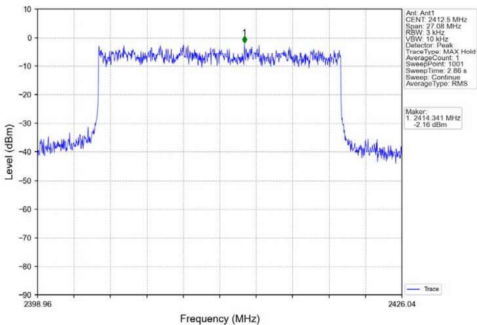
16QAM 20MHz_LCH_2412.5MHz_Ant1_NTNV
