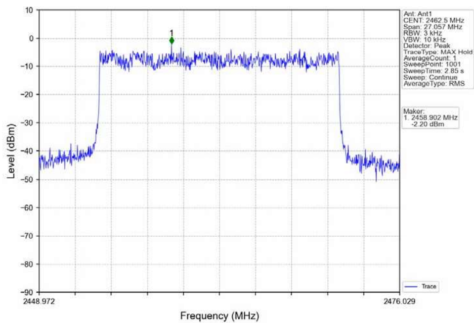
16QAM 20MHz_HCH_2462.5MHz_Ant1_NTNV
