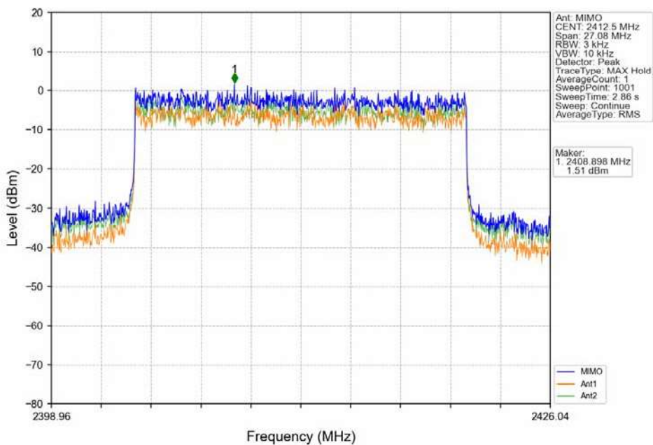
16QAM 20MHz_LCH_2412.5MHz_MIMO_NTNV
