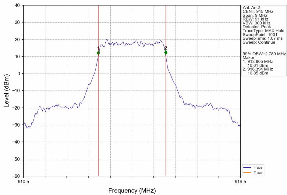
QPSK_MCH_915MHz_Ant2_NTNV
