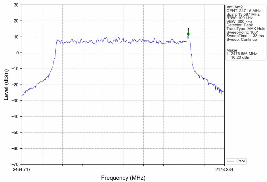
QPSK_HCH_2471.5MHz_Ant2_NTNV
