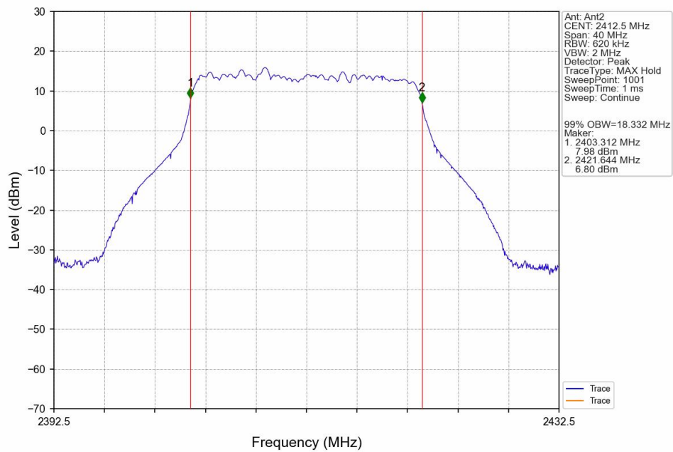
16QAM_LCH_2412.5MHz_Ant2_NTNV
