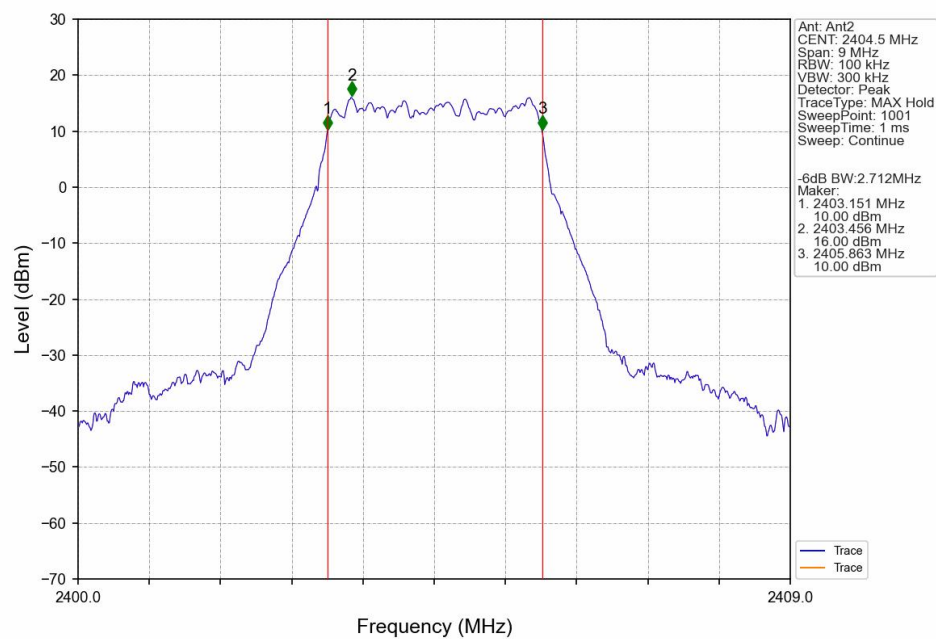
QPSK_LCH_2404.5MHz_Ant2_NTNV
