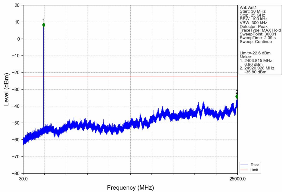
QPSK_LCH_2405.5MHz_Ant1_NTNV
