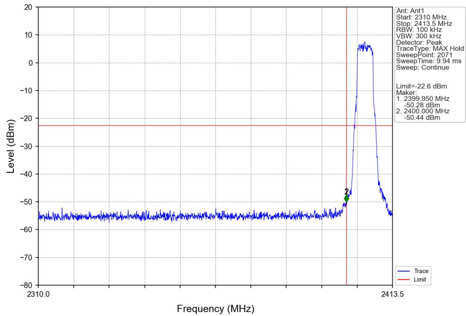
QPSK_LCH_2405.5MHz_Ant1_NTNV
