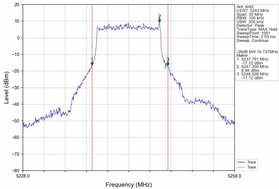
16QAM_HCH_5243MHz_Ant2_NTNV
