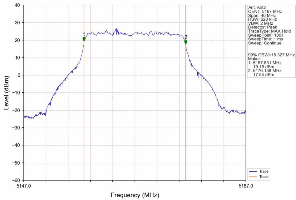
16QAM_LCH_5167MHz_Ant2_NTNV
