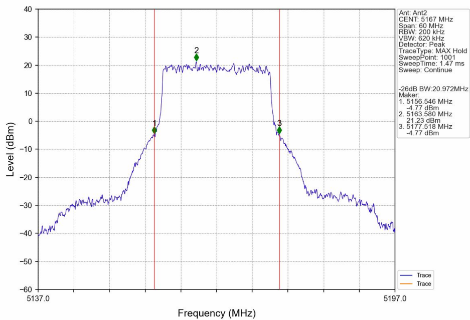
16QAM_LCH_5167MHz_Ant2_NTNV
