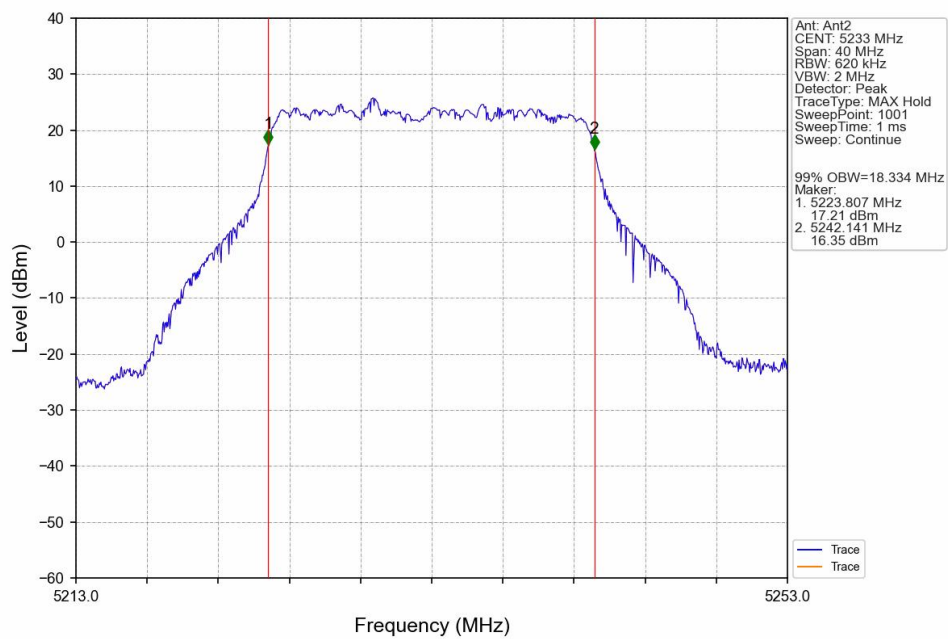
16QAM_HCH_5233MHz_Ant2_NTNV
