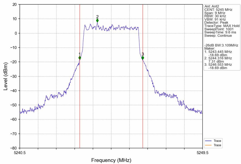
16QAM_HCH_5245MHz_Ant2_NTNV
