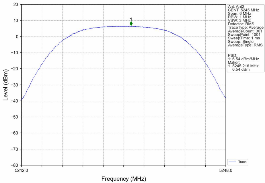
QPSK_HCH_5245MHz_Ant2_NTNV
