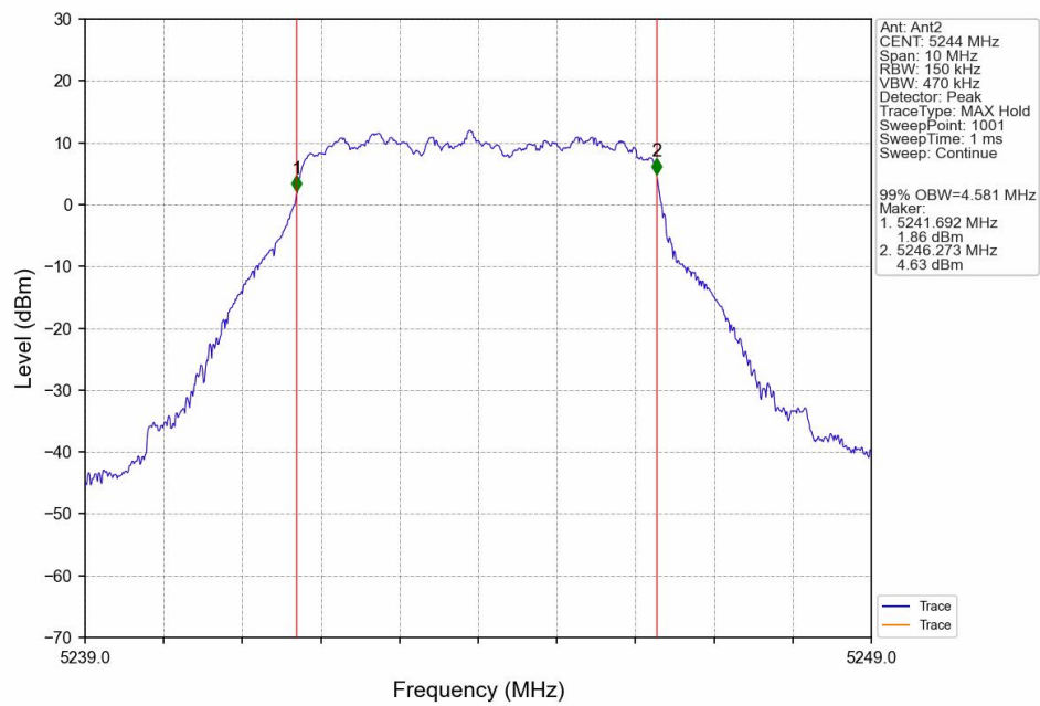
16QAM_HCH_5244MHz_Ant2_NTNV
