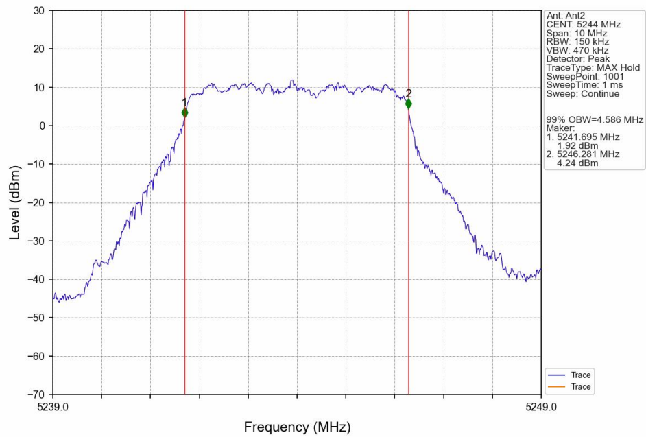
QPSK_HCH_5244MHz_Ant2_NTNV
