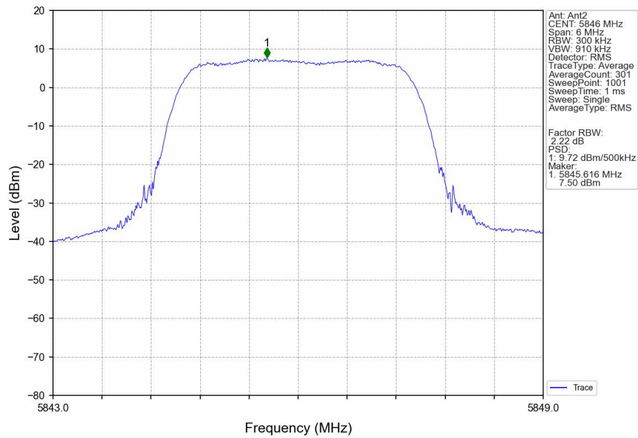
QPSK_HCH_5846MHz_Ant2_NTNV
