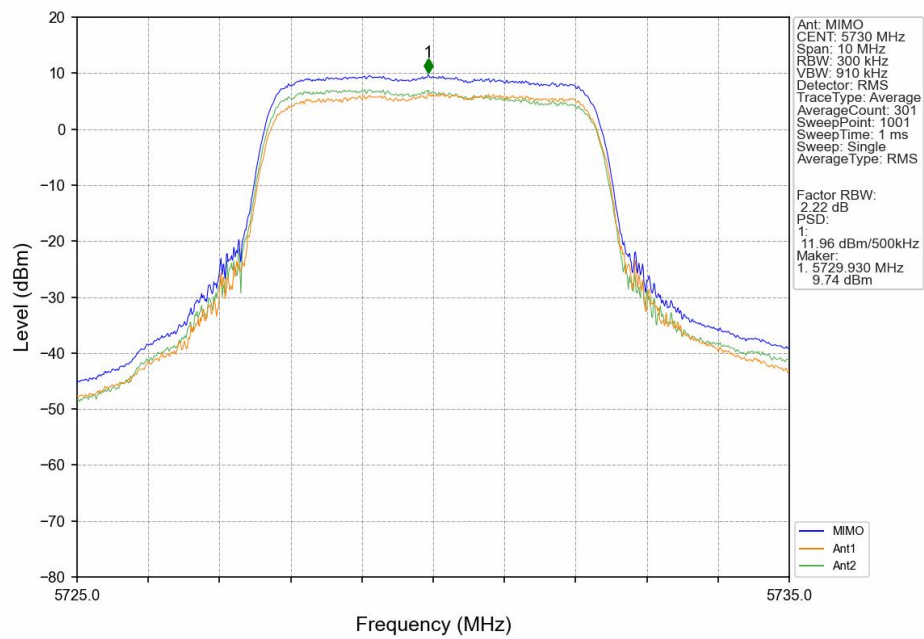
16QAM_LCH_5730MHz_MIMO_NTNV
