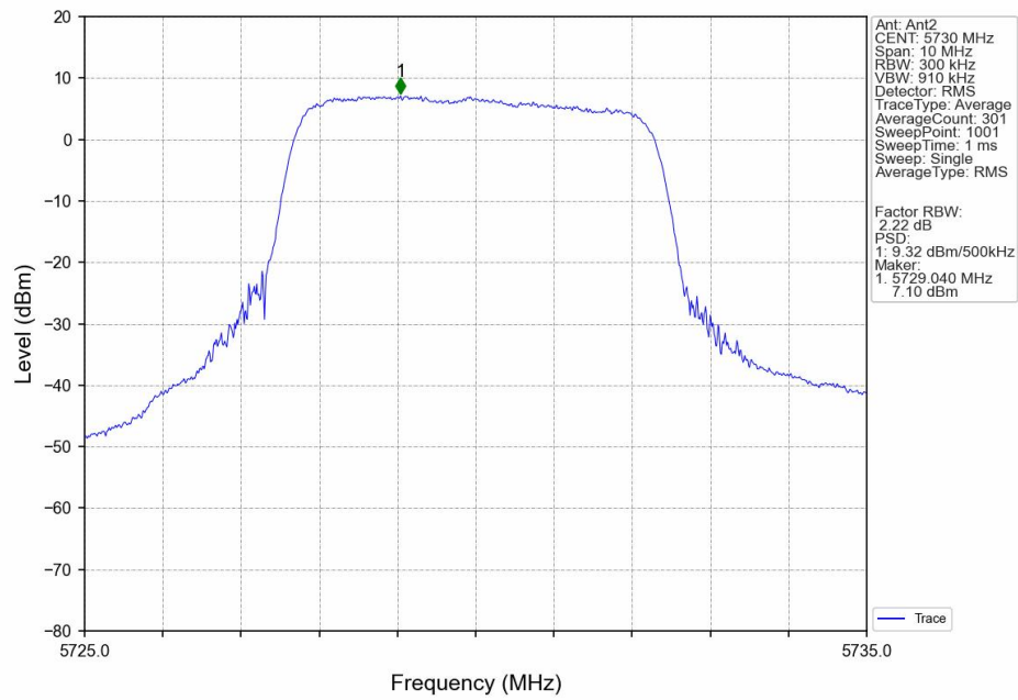
16QAM_LCH_5730MHz_MIMO_NTNV
