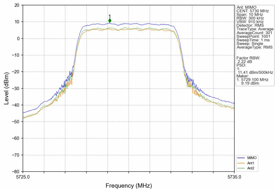
16QAM_LCH_5730MHz_MIMO_NTNV
