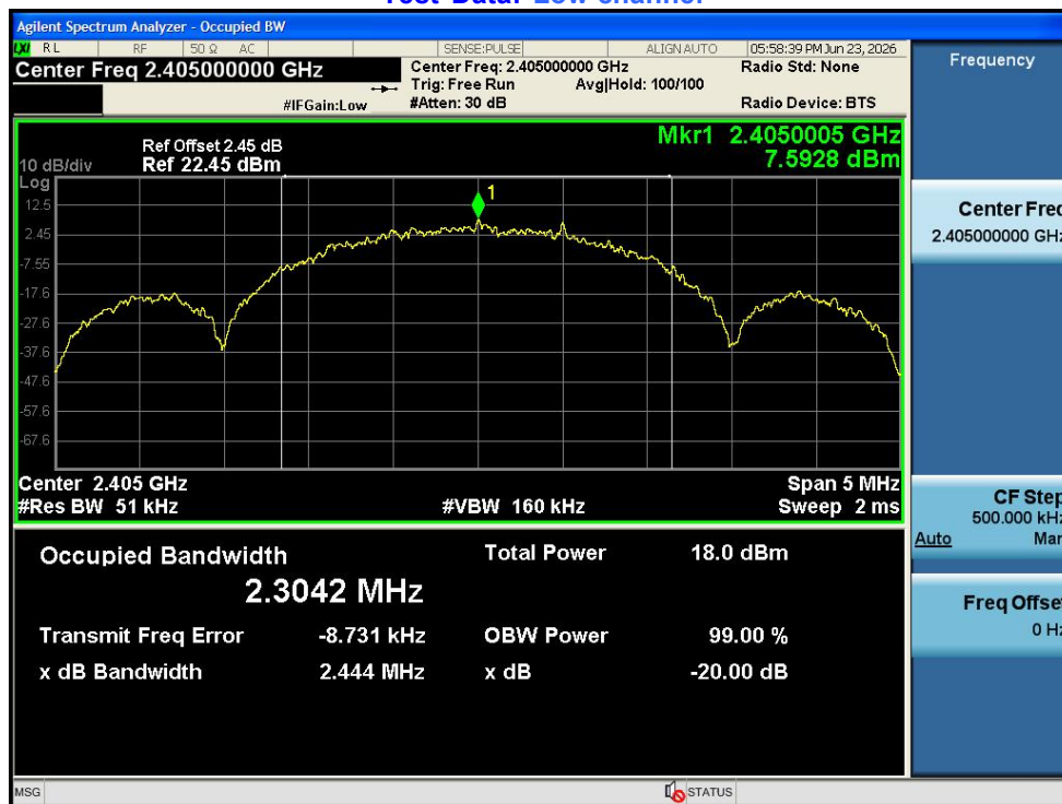
Test Data: Low channel
