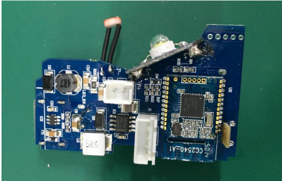
Figure 5. Bottom view of PCB
