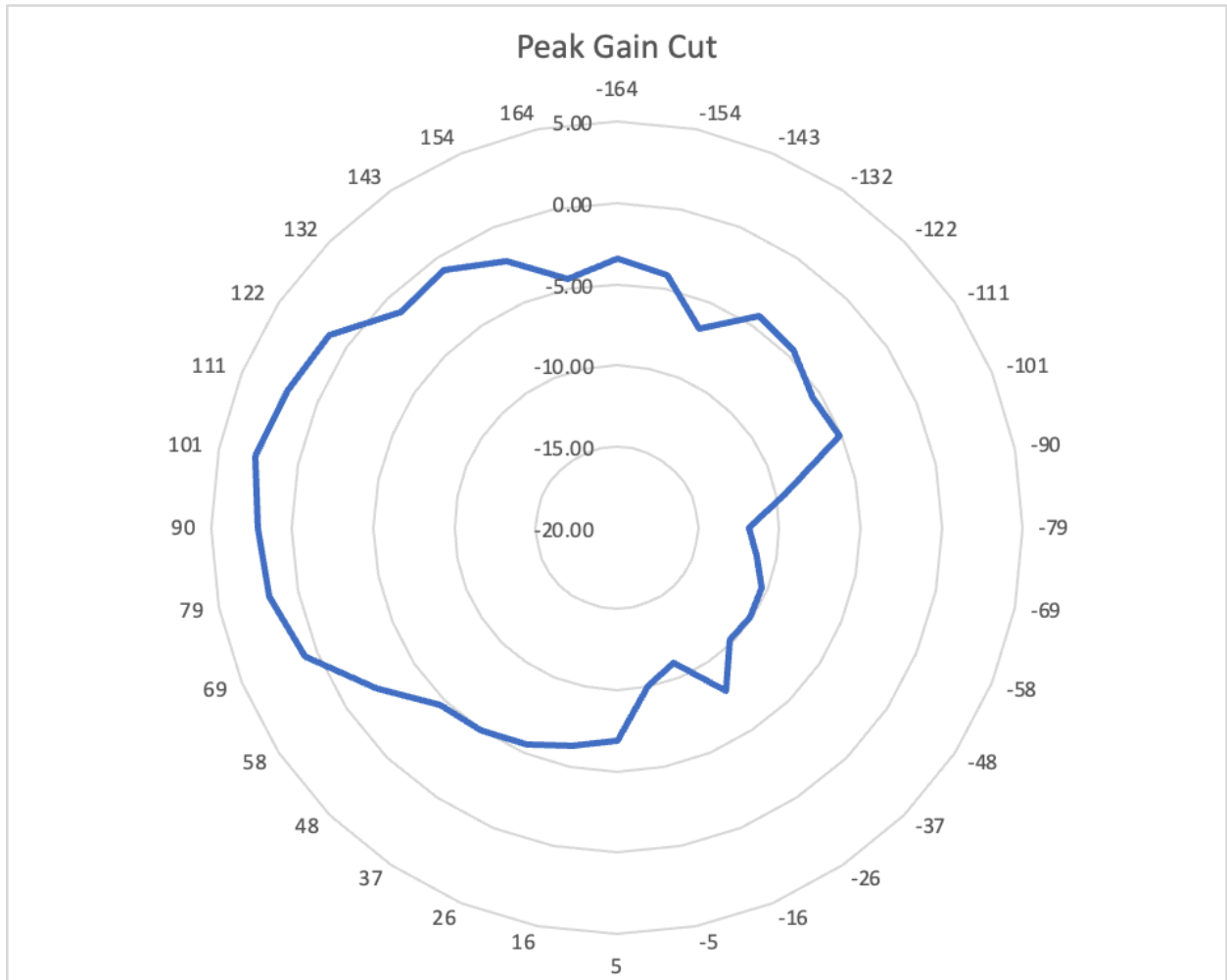
Wifi UNII-2C
