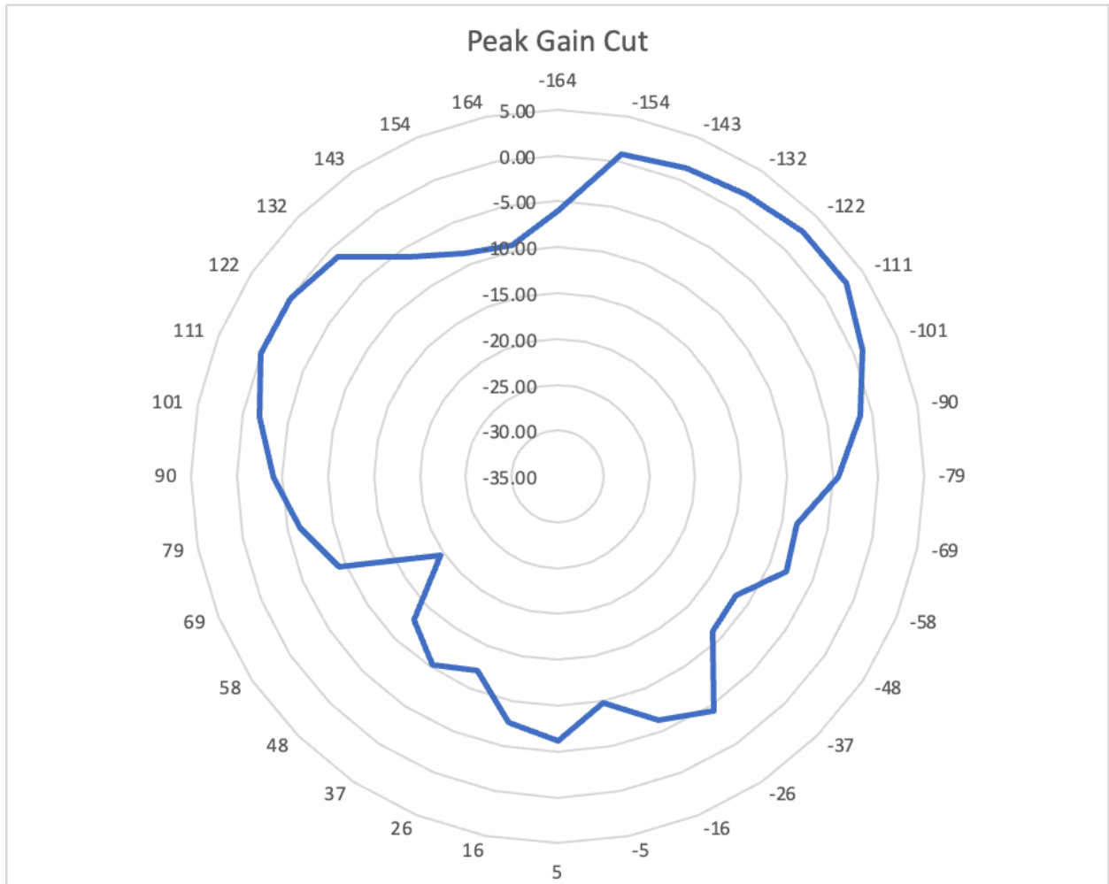
Wifi UNII-7
