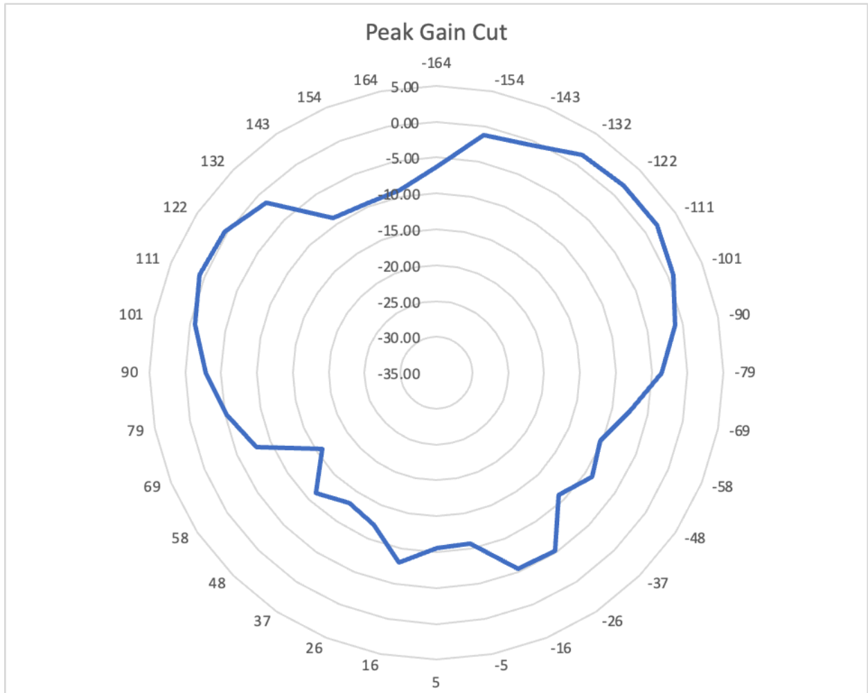
Wifi UNII-8
