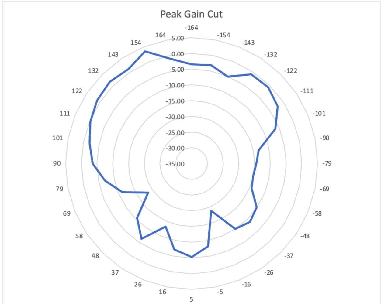
Wifi UNII-5
