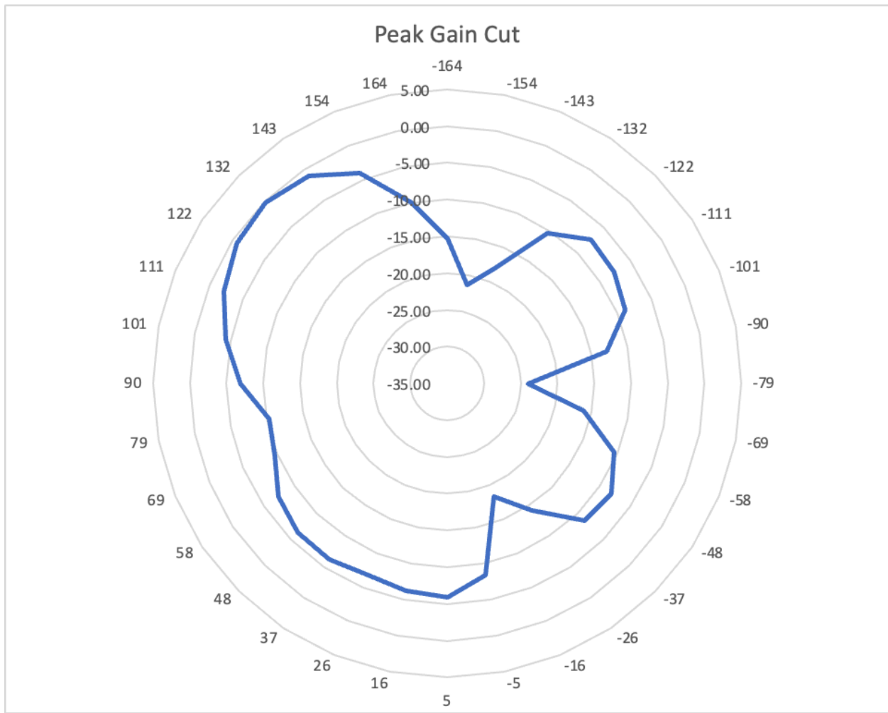
Antenna 2D Total Gain Plots (Phi cut with peak gain): Wifi/BT 2.4GHz
