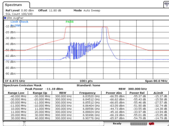
Plot on Channel 6875MHz 26RU8
