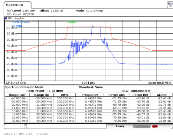
Plot on Channel 6475MHz 52RU39
