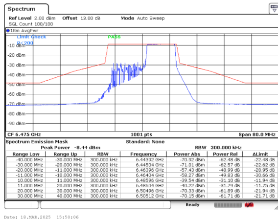
Plot on Channel 6475MHz 106RU54
