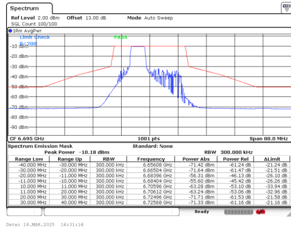
Plot on Channel 6695MHz 52RU38
