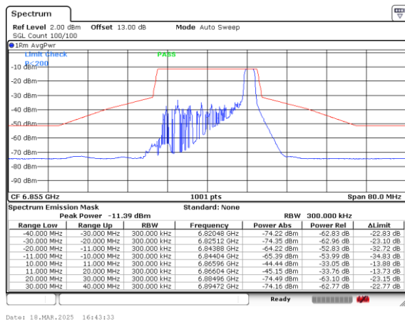
Plot on Channel 6855MHz 26RU8
