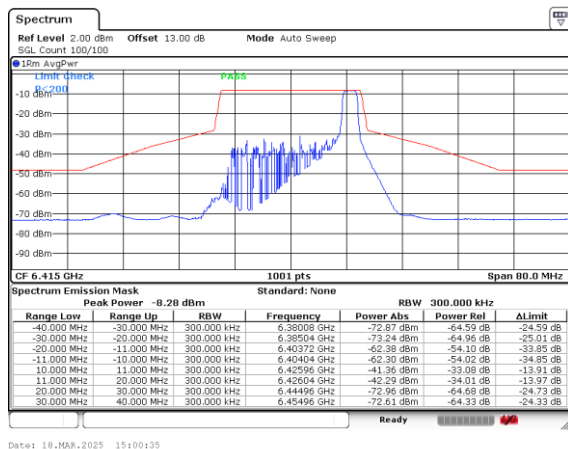
Plot on Channel 6415MHz 26RU8
