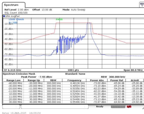
Plot on Channel 6515MHz 26RU8
