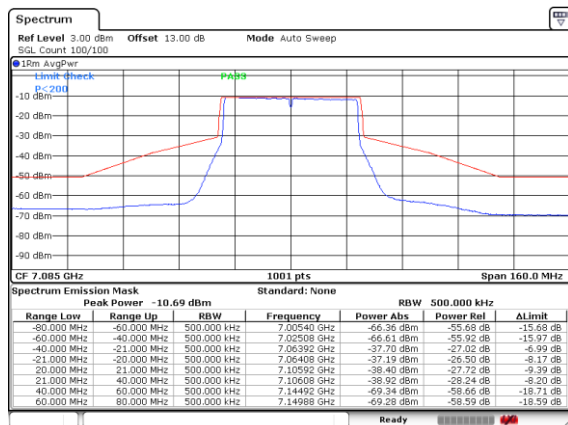
Plot on Channel 7085MHz
