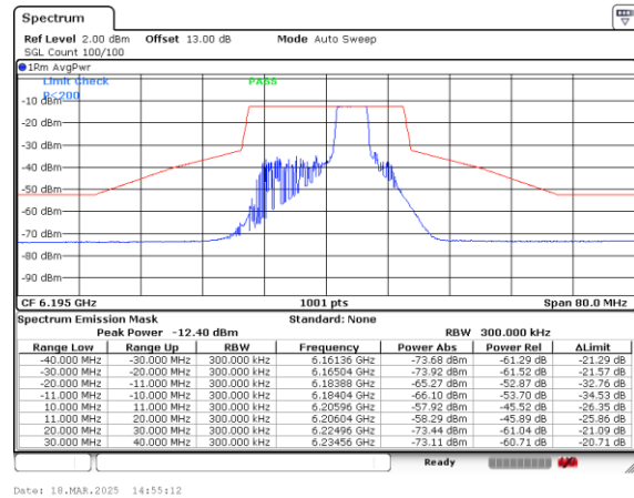
Plot on Channel 6195MHz 52RU39
