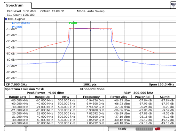
Plot on Channel 7005MHz
