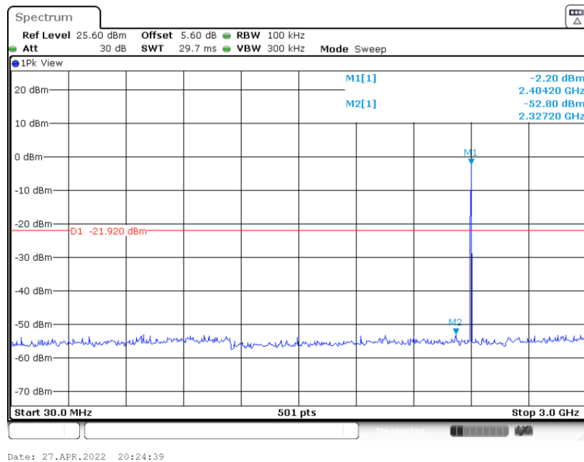
Conducted Spurious Emission Plot on Channel 00
