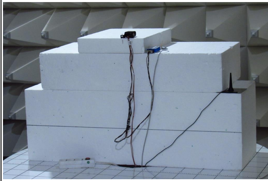
Setup EUT view above 1 GHz pre measurements
