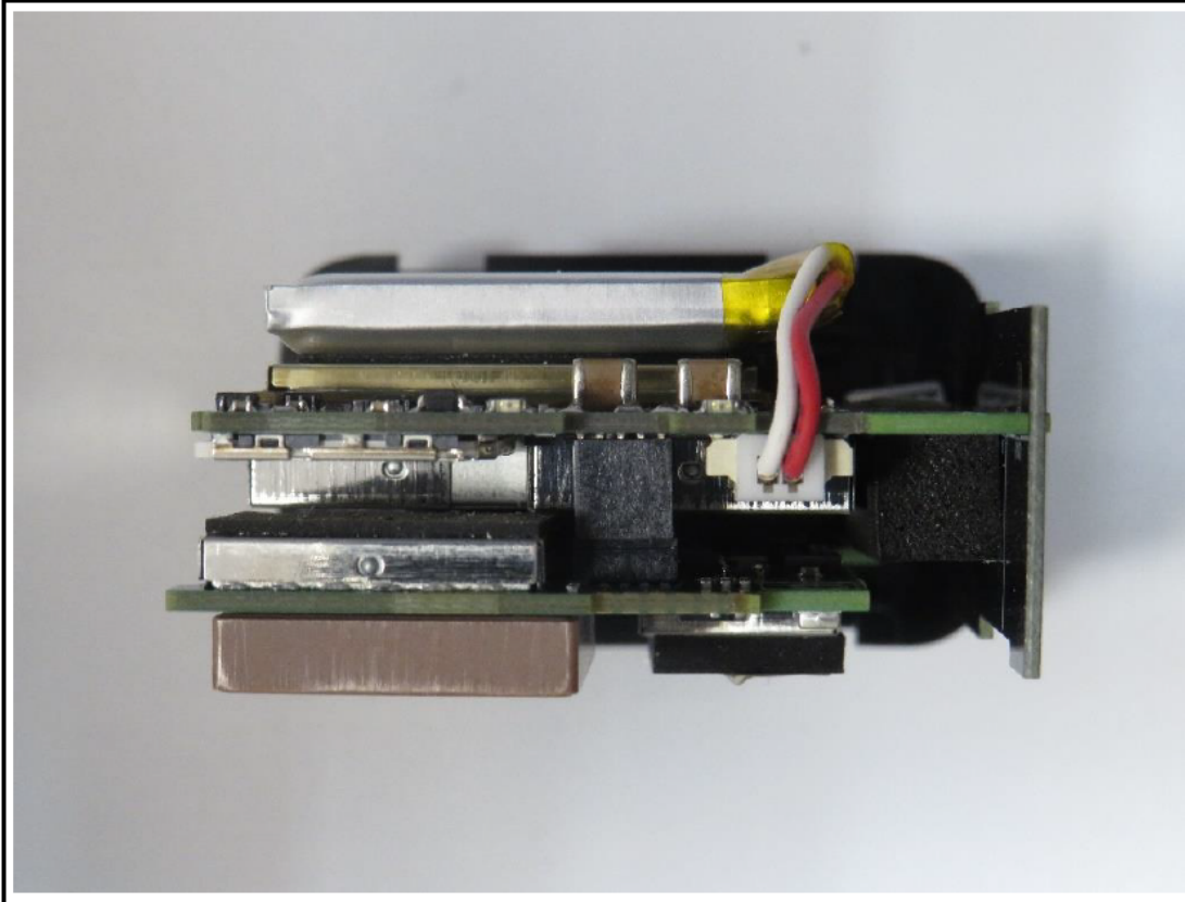
L0245 PCB FRONT SIDE
