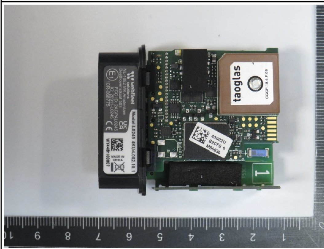
L0245 PCB BOTTOM SIDE
