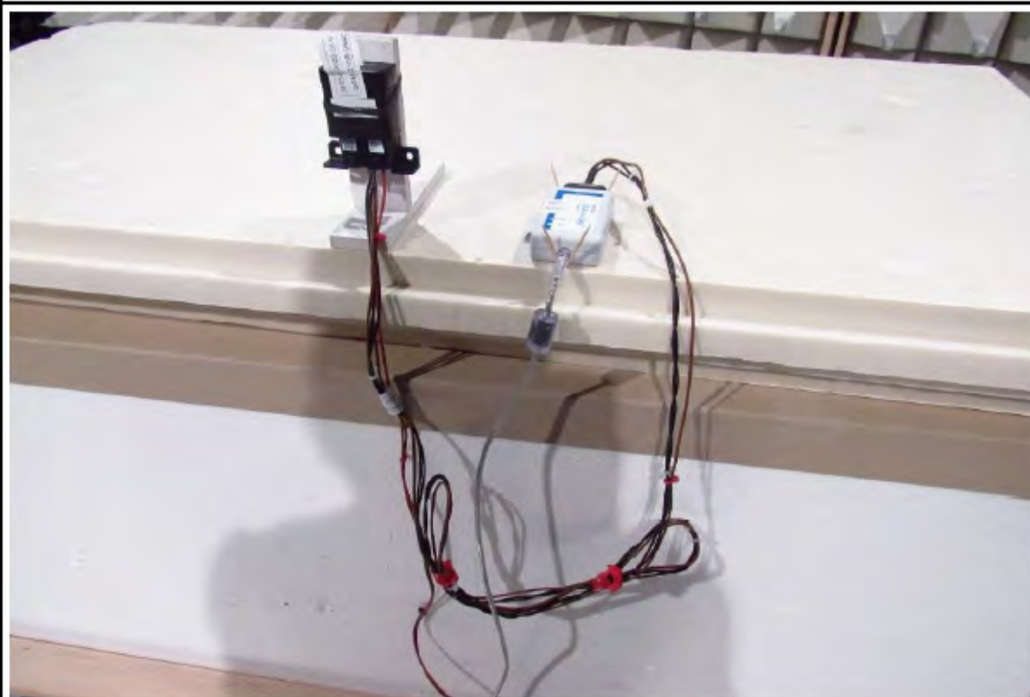
EUT Setup below 1 GHz
