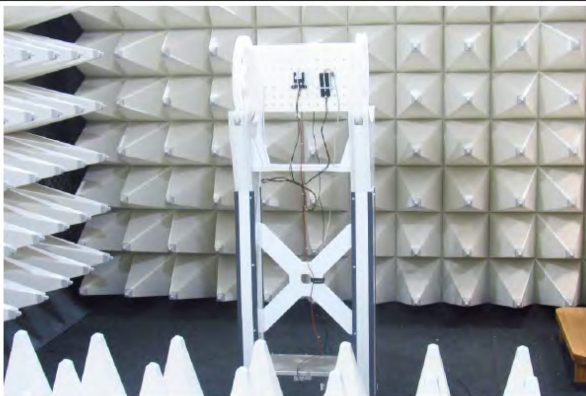
EUT Setup above 1 GHz
