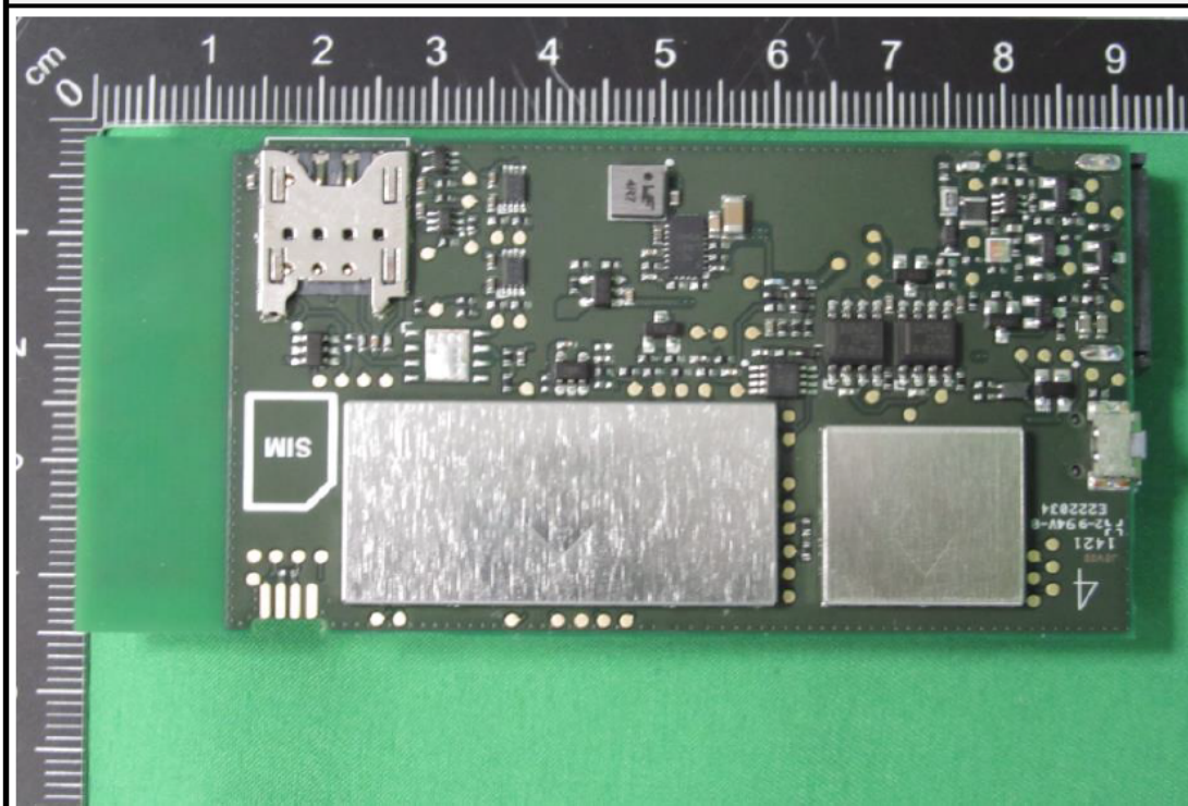
PCB back view
