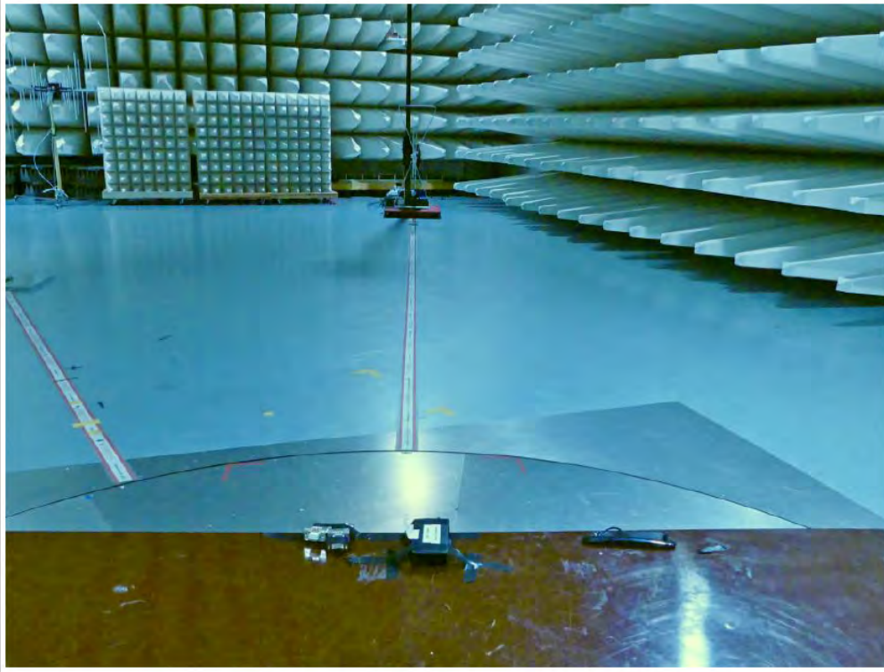
Test setup up to 1 GHz vertical polarization
