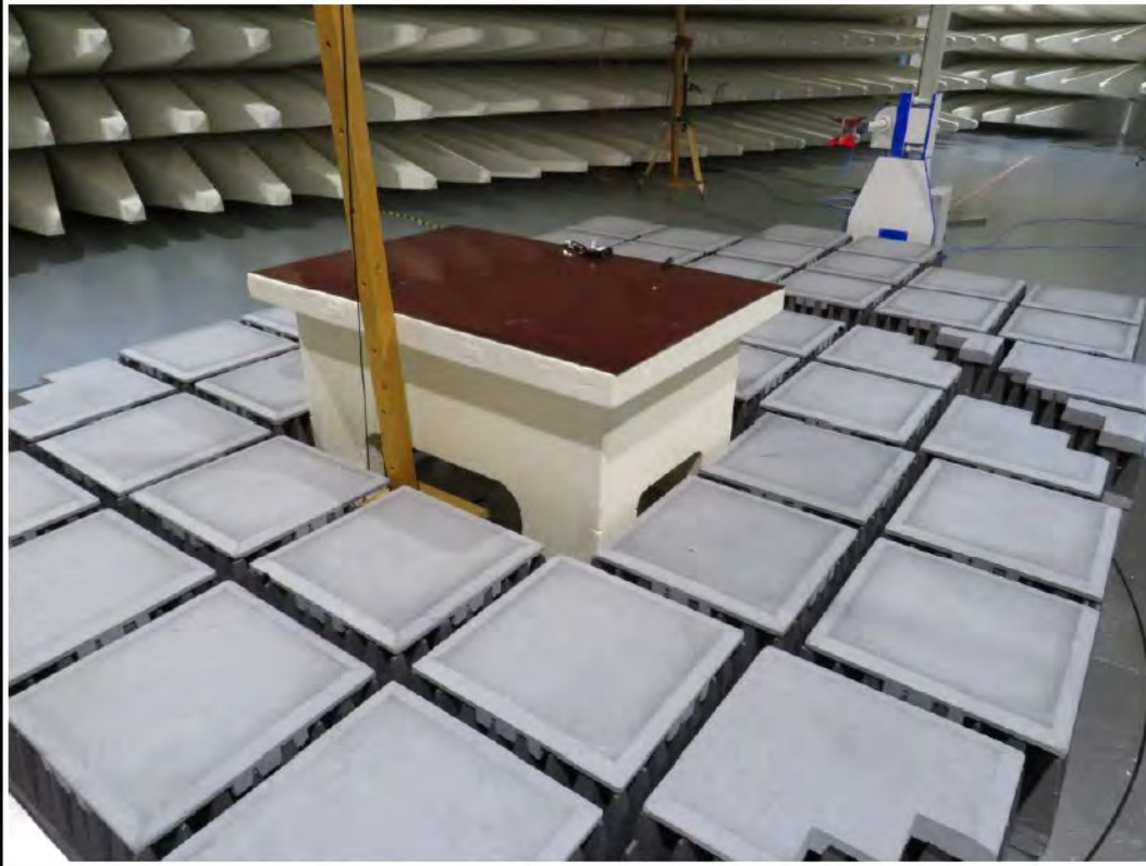
Test setup up above 1 GHz vertical polarization
