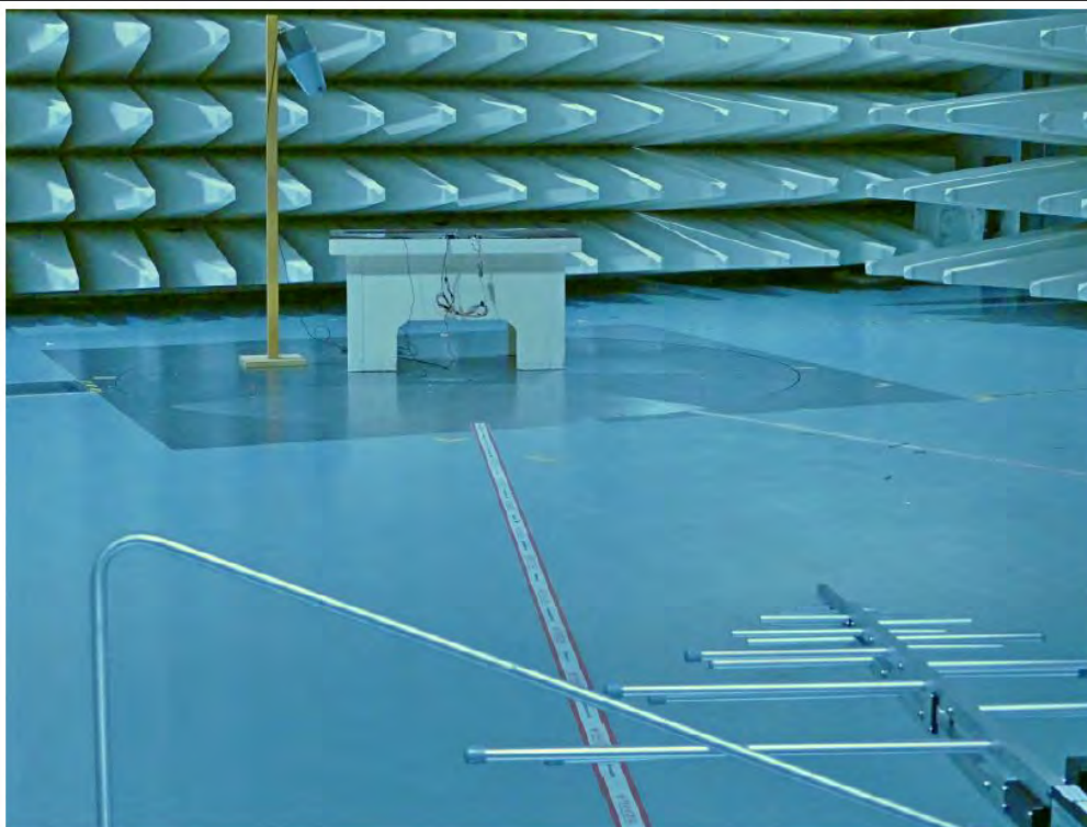
Test setup up to 1 GHz horizontal polarization
