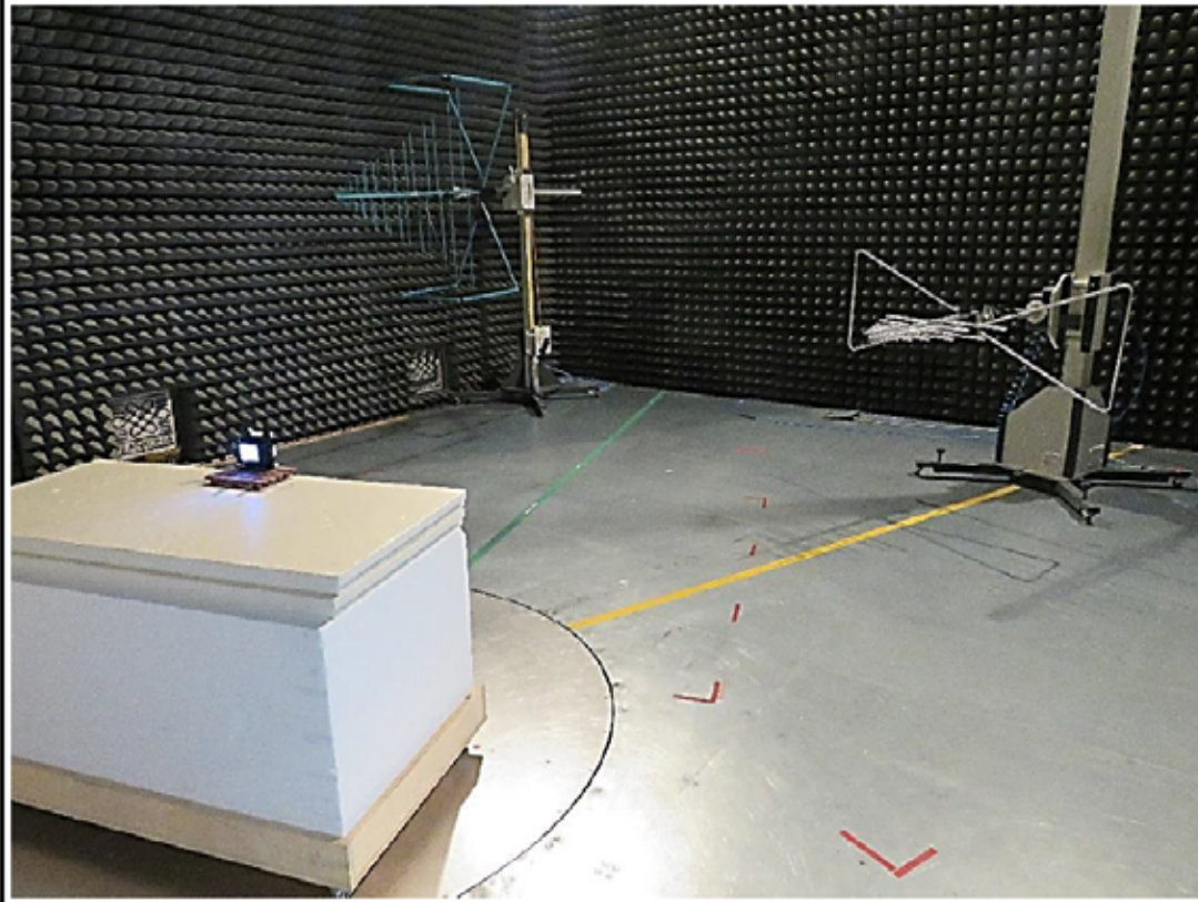
Test setup above 30 MHz - view 1
