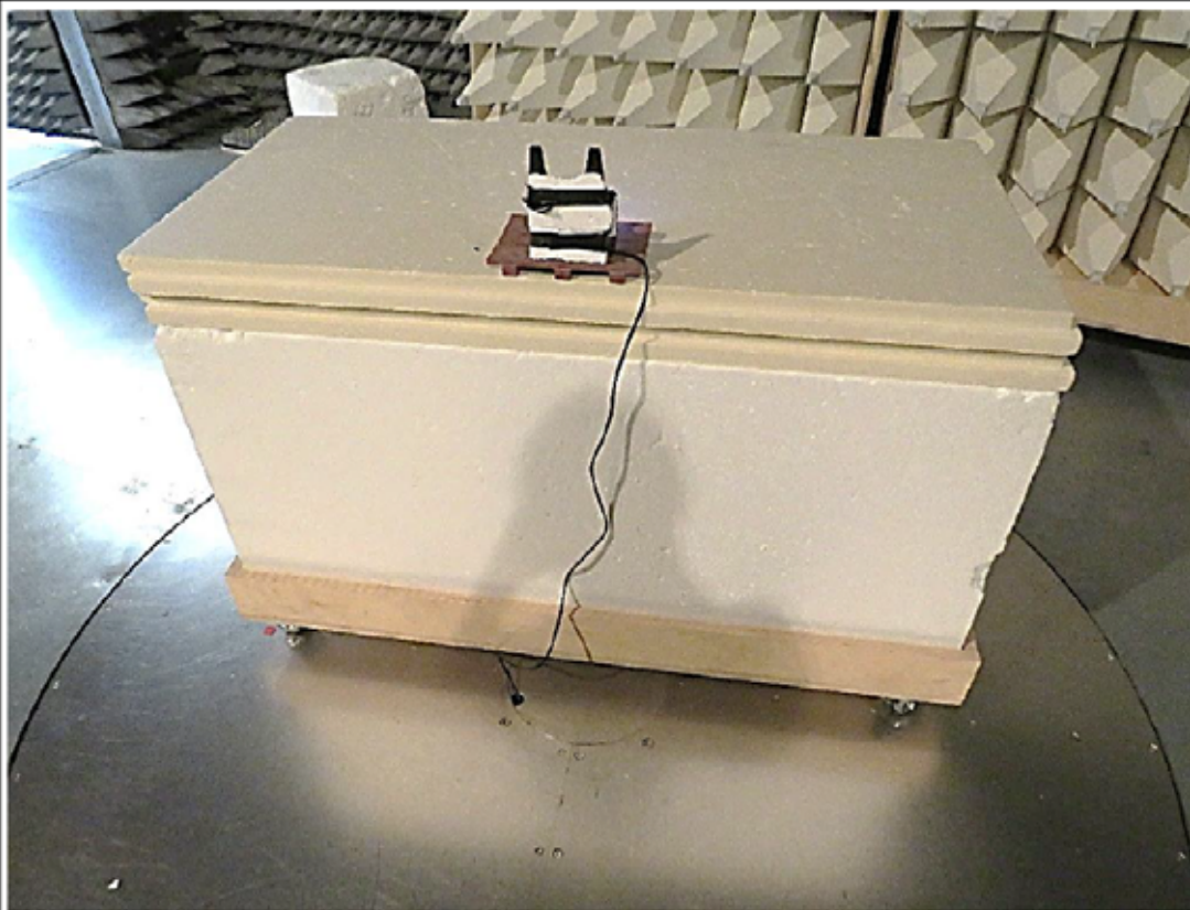
Test setup above 30 MHz - view 2
