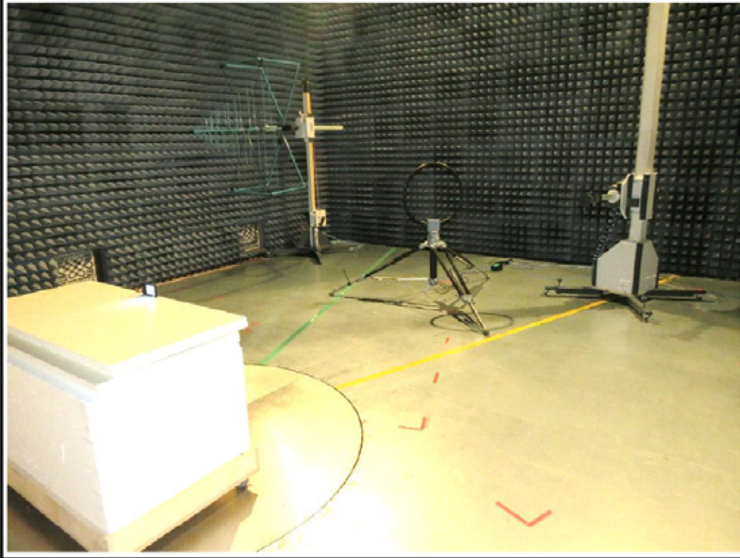
Test setup below 30 MHz - view 1
