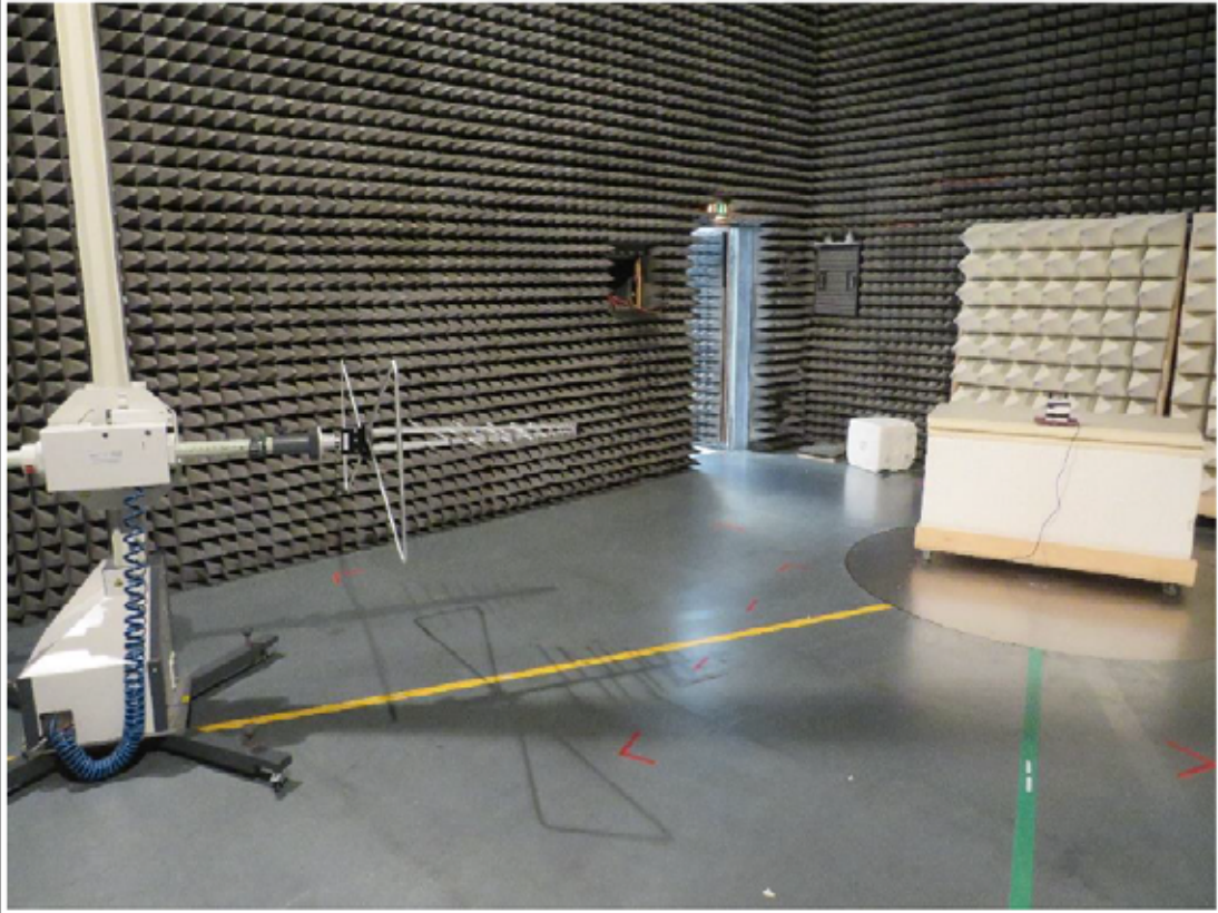
Test setup 30 MHz - 1000 MHz
