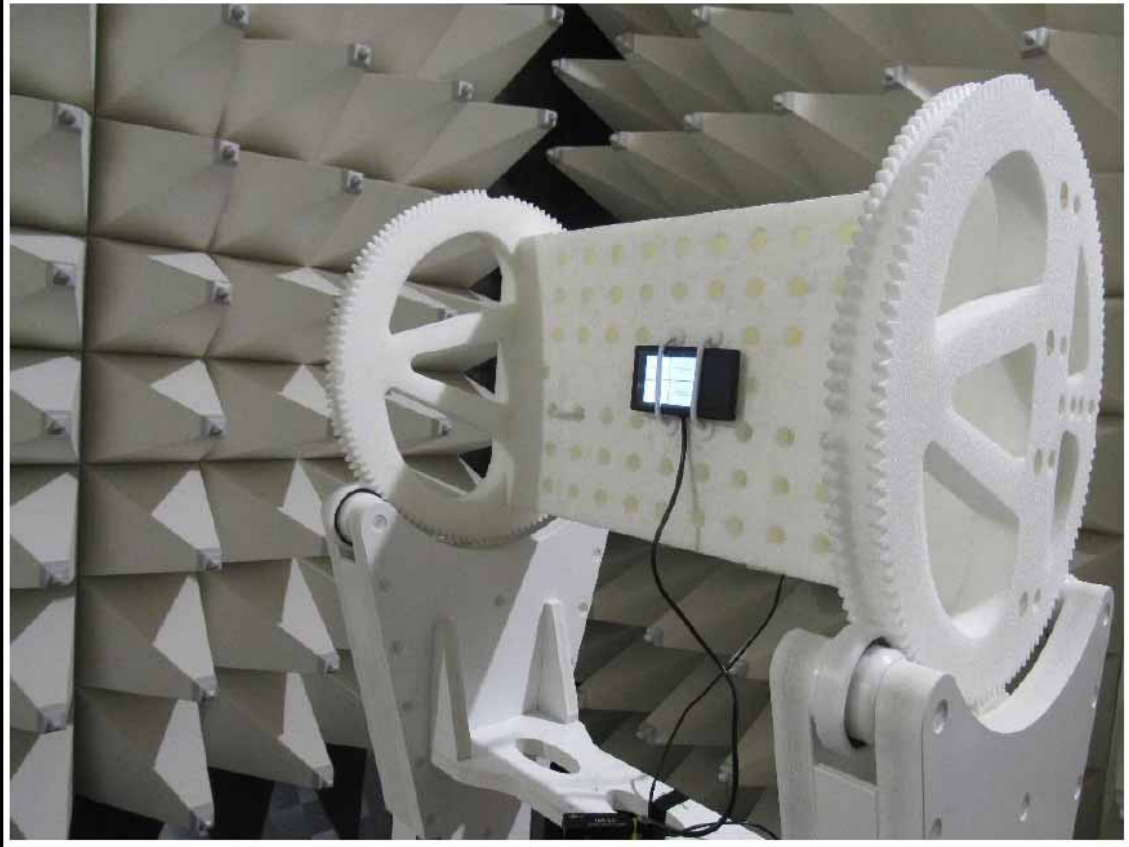
Test setup > 1 GHz
