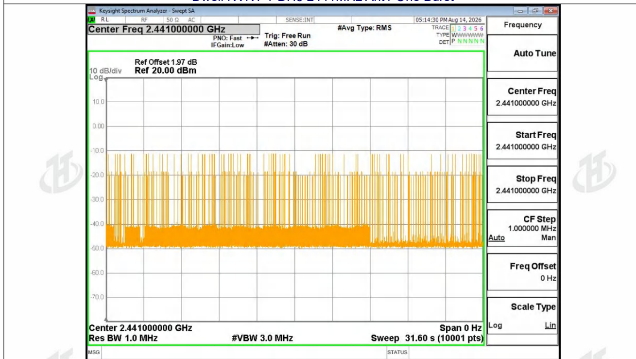
Dwell NVNT 1-DH5 2441MHz Ant1 Accumulated
