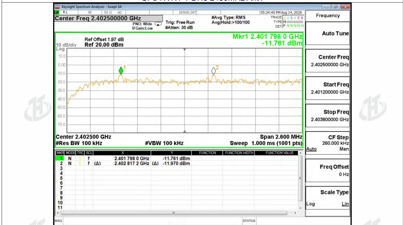
CFS NVNT 2-DH5 2402MHz Ant1
