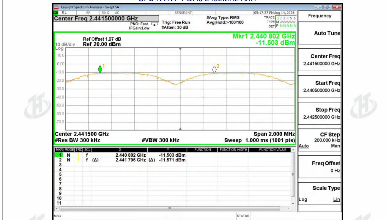
CFS NVNT 1-DH5 2441MHz Ant1
