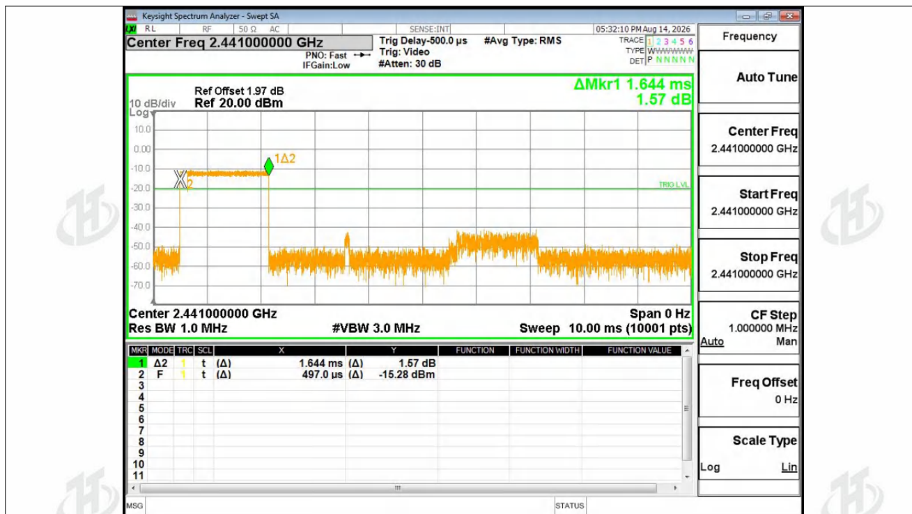
Dwell NVNT 2-DH3 2441MHz Ant1 One Burst
