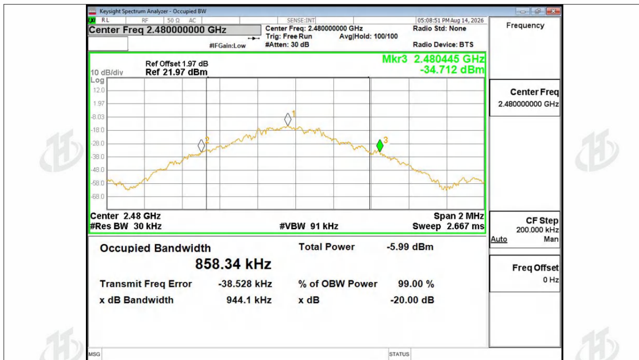
-20dB Bandwidth NVNT 1-DH5 2480MHz Ant1
