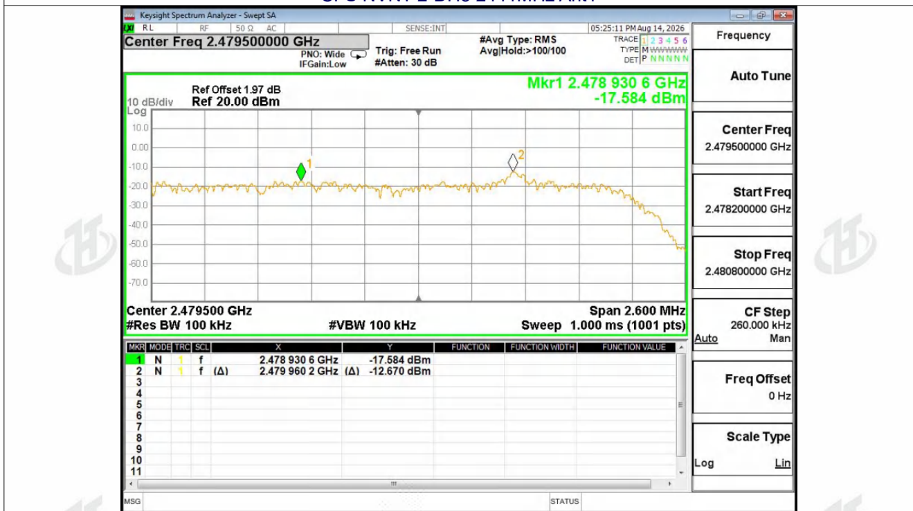
CFS NVNT 2-DH5 2480MHz Ant1
