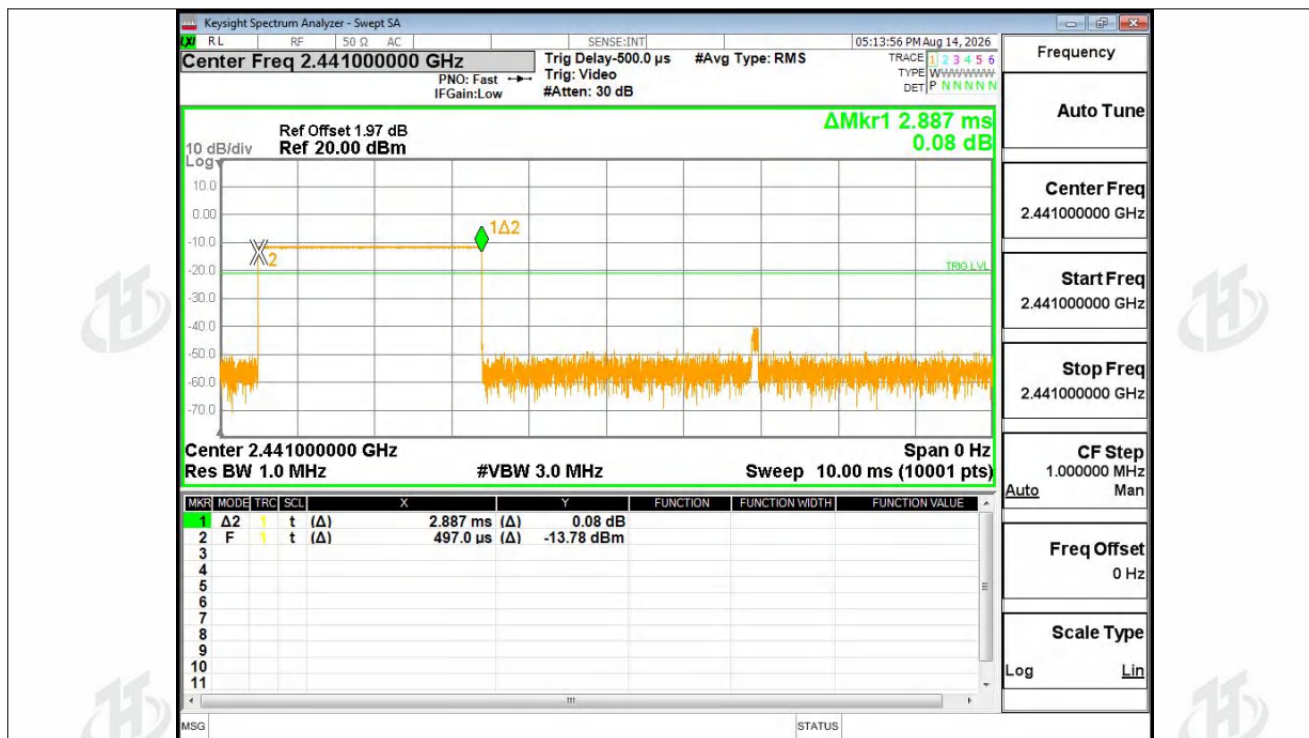
Dwell NVNT 1-DH5 2441MHz Ant1 One Burst
