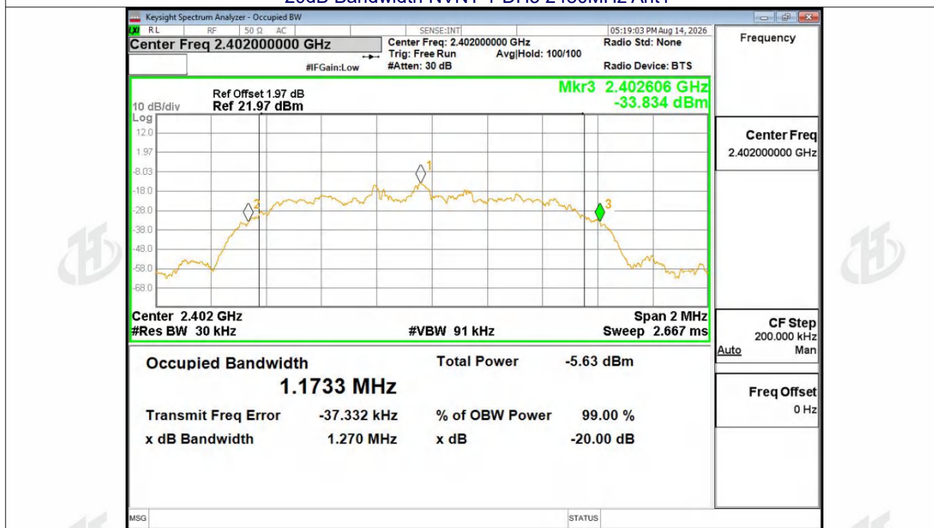
-20dB Bandwidth NVNT 2-DH5 2402MHz Ant1
