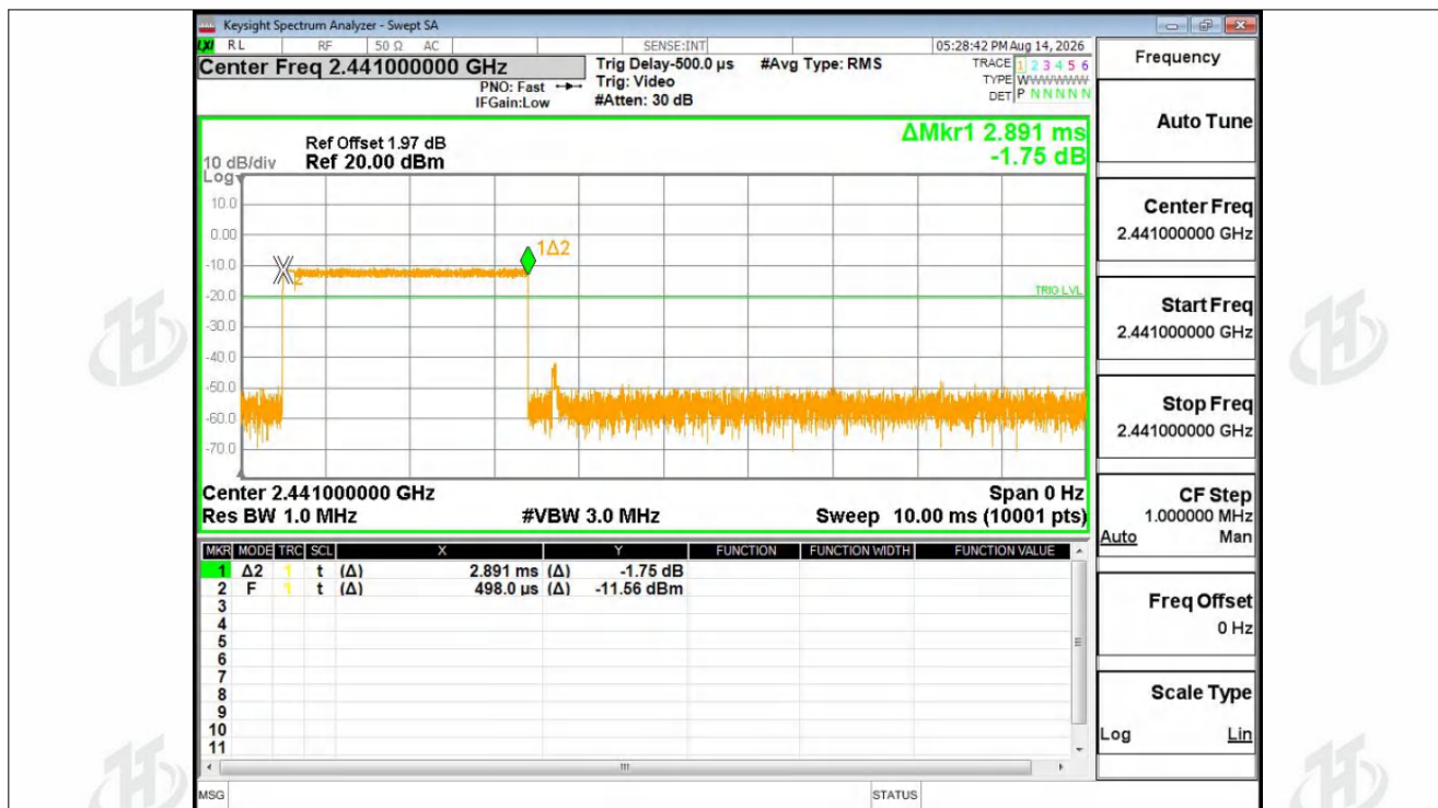
Dwell NVNT 2-DH5 2441MHz Ant1 One Burst
