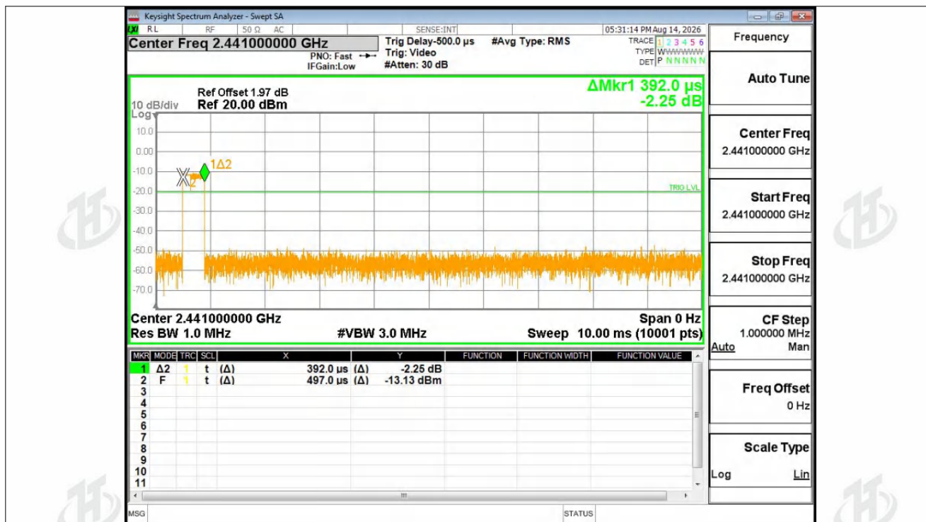
Dwell NVNT 2-DH1 2441MHz Ant1 One Burst
