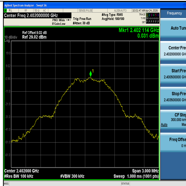
BLE_1M-Ant1-2402-0~Reference-PASS
