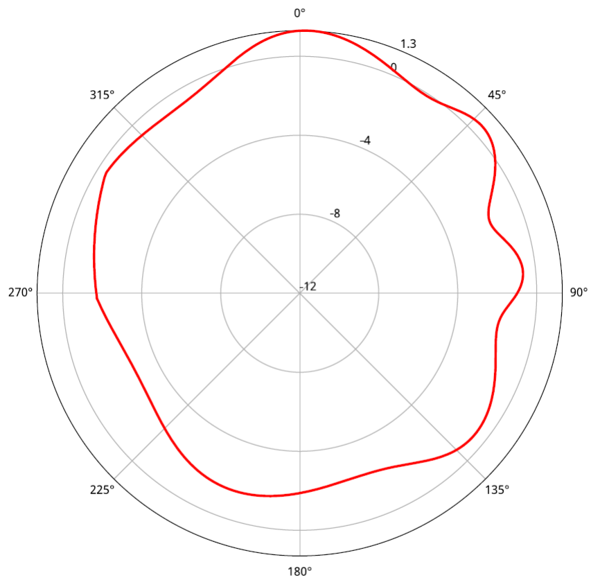
462.5500MHz Realized Gain (Non - Normalized), Max=1.3 dBi
