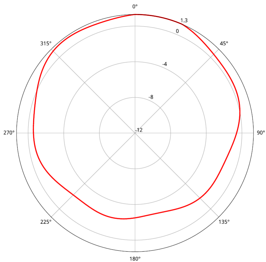
467.5625MHz Realized Gain (Non - Normalized), Max=1.3 dBi
