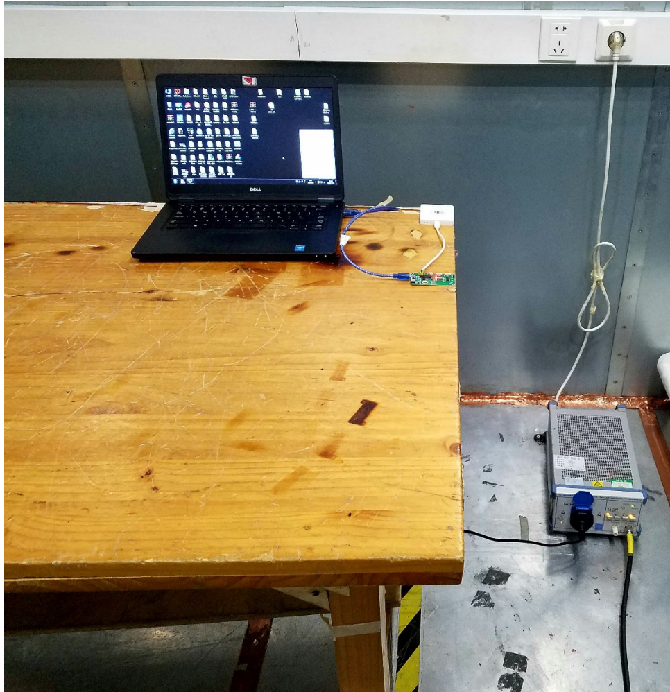
Picture 2 Conducted Emission Test Setup
