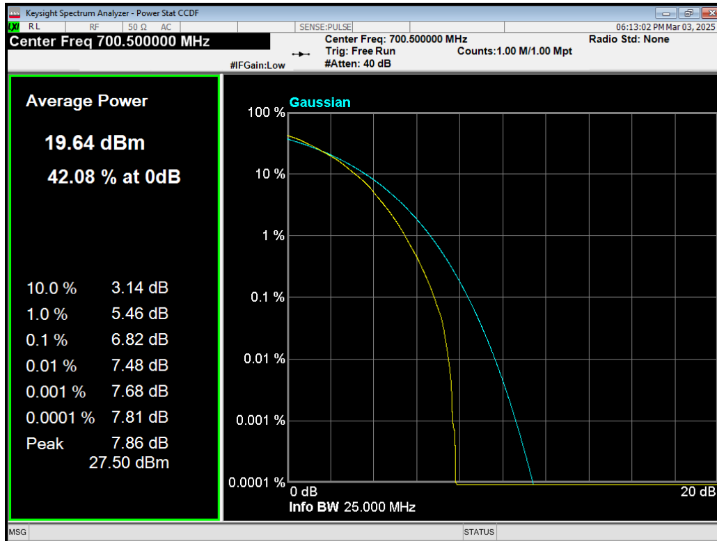
Band12 64QAM BW=3MHz Channel=23025 RB Size=15 Position=#0.png
