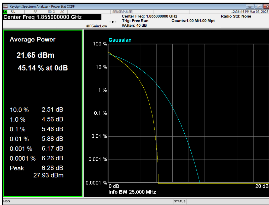
Band2 QPSK BW=10MHz Channel=18650 RB Size=50 Position=#0.png
