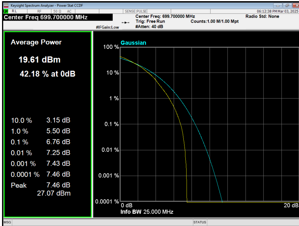
Band12 64QAM BW=1.4MHz Channel=23017 RB Size=6 Position=#0.png
