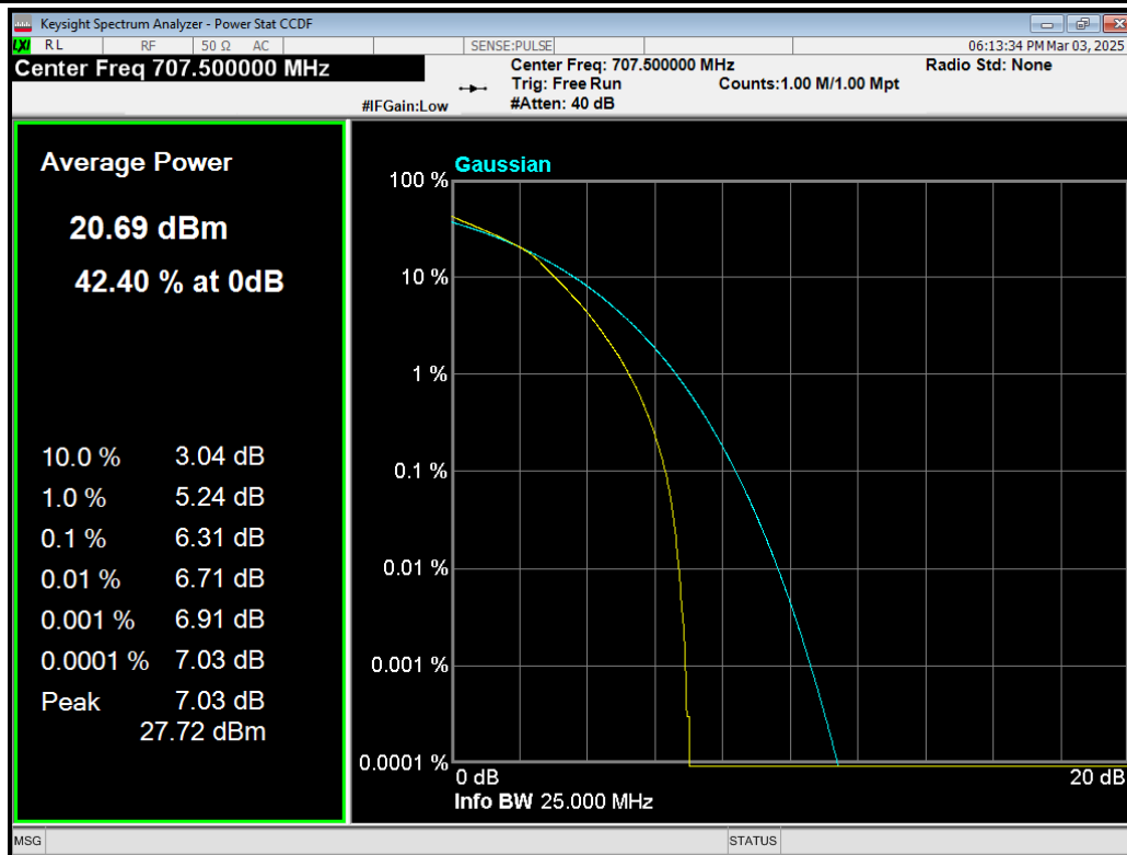
Band12 16QAM BW=5MHz Channel=23095 RB Size=25 Position=#0.png
