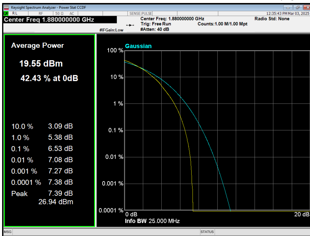
Band2 64QAM BW=1.4MHz Channel=18900 RB Size=6 Position=#0.png
