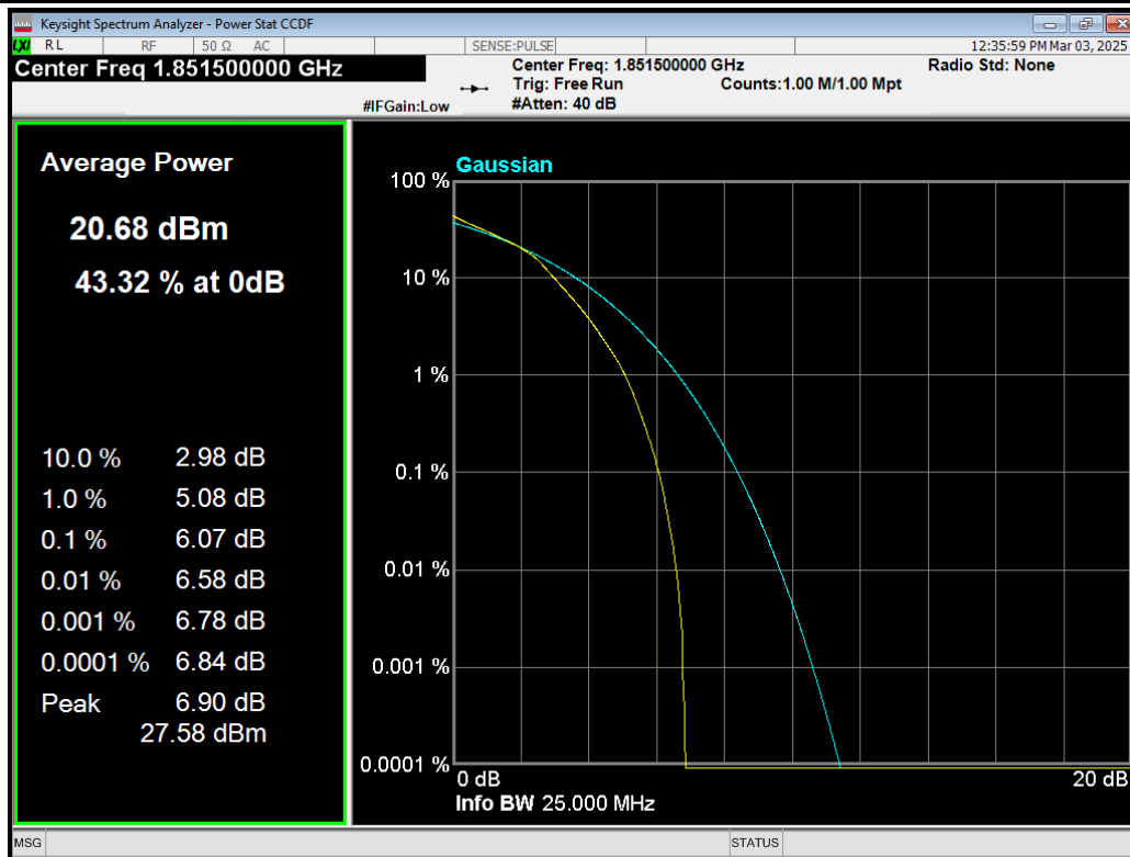
Band2 16QAM BW=3MHz Channel=18615 RB Size=15 Position=#0.png
