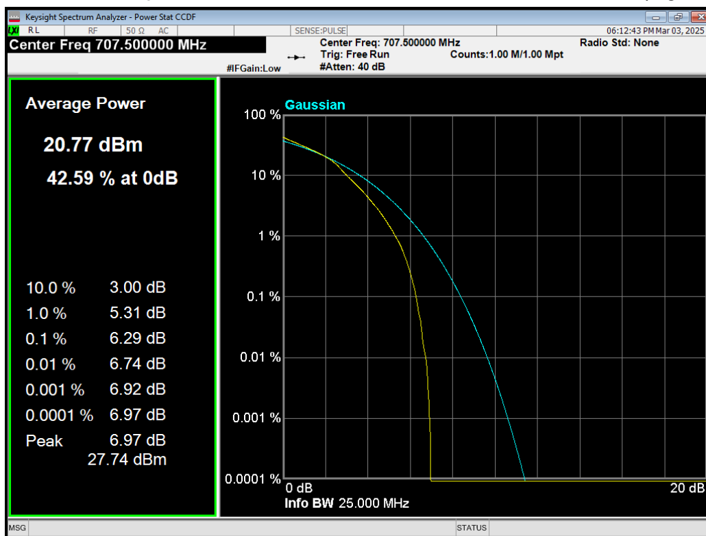
Band12 16QAM BW=1.4MHz Channel=23095 RB Size=6 Position=#0.png
