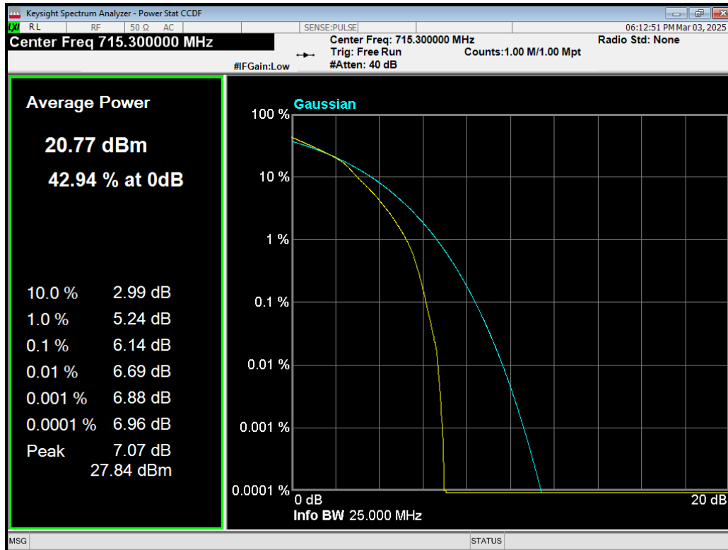
Band12 16QAM BW=1.4MHz Channel=23173 RB Size=6 Position=#0.png
