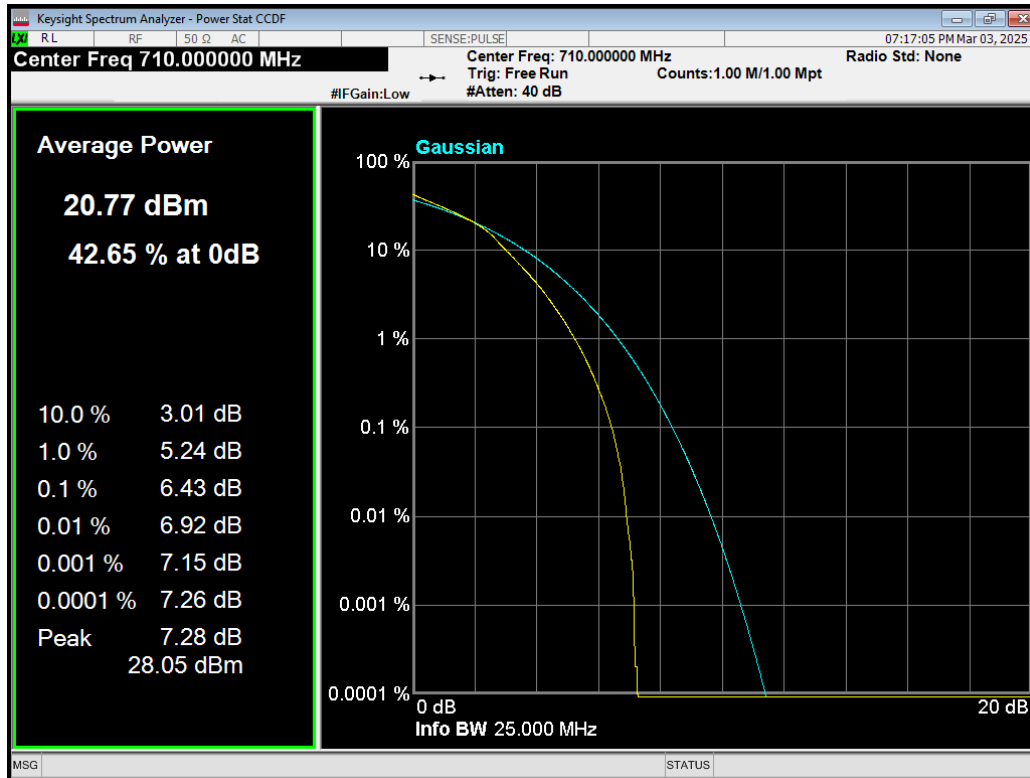
Band17 16QAM BW=5MHz Channel=23790 RB Size=25 Position=#0.png
