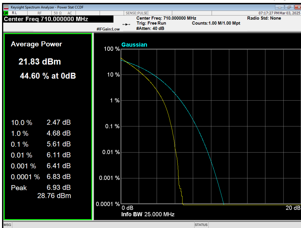
Band17 QPSK BW=10MHz Channel=23790 RB Size=50 Position=#0.png
