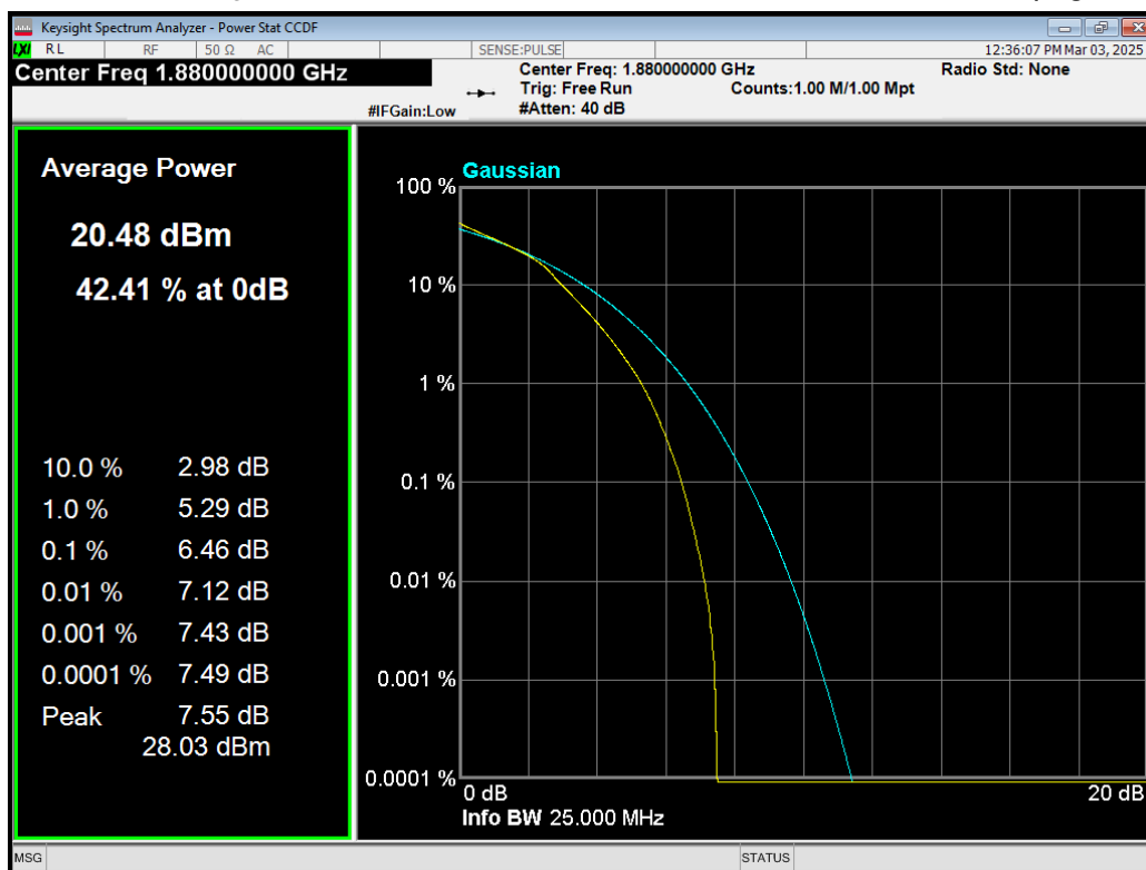
Band2 16QAM BW=3MHz Channel=18900 RB Size=15 Position=#0.png
