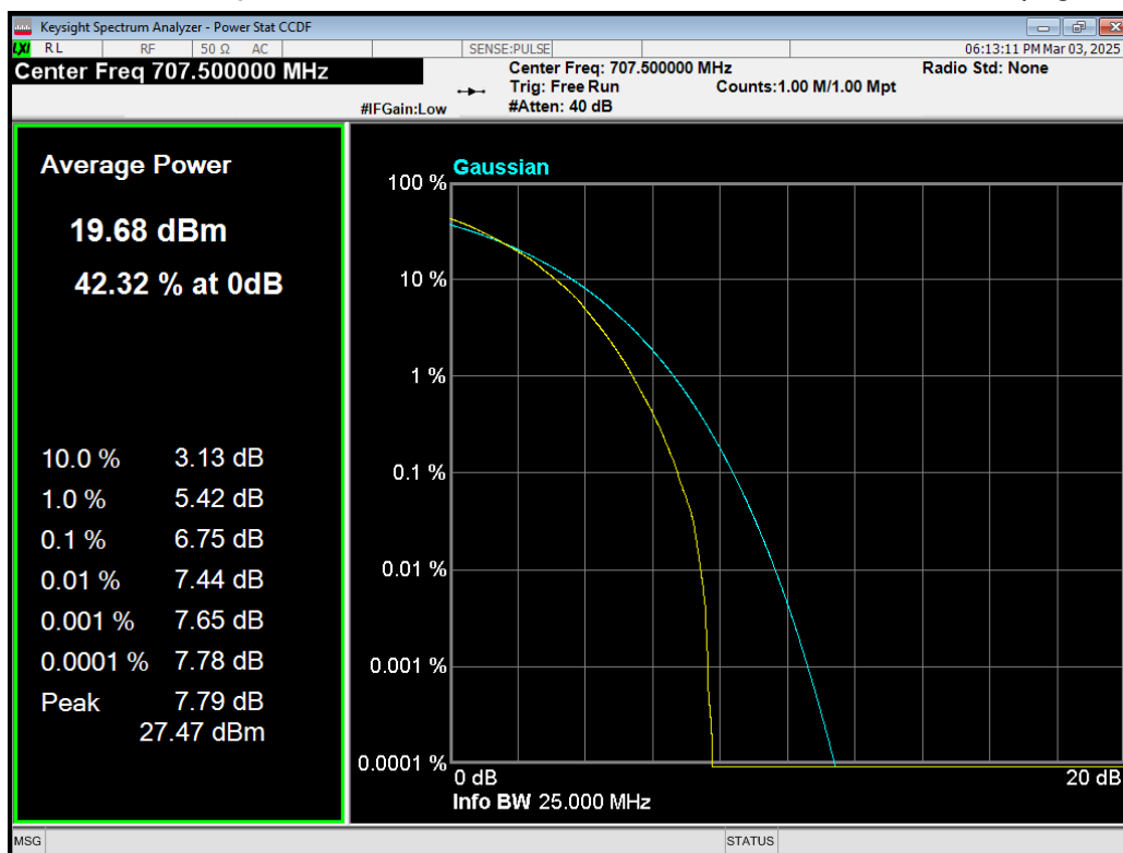
Band12 64QAM BW=3MHz Channel=23095 RB Size=15 Position=#0.png
