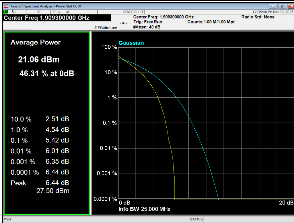
Band2 QPSK BW=1.4MHz Channel=19193 RB Size=6 Position=#0.png
