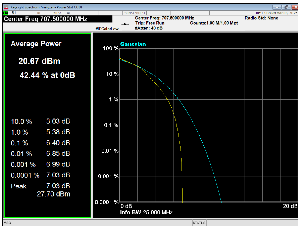
Band12 16QAM BW=3MHz Channel=23095 RB Size=15 Position=#0.png
