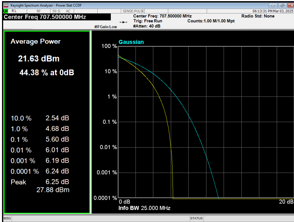
Band12 QPSK BW=5MHz Channel=23095 RB Size=25 Position=#0.png
