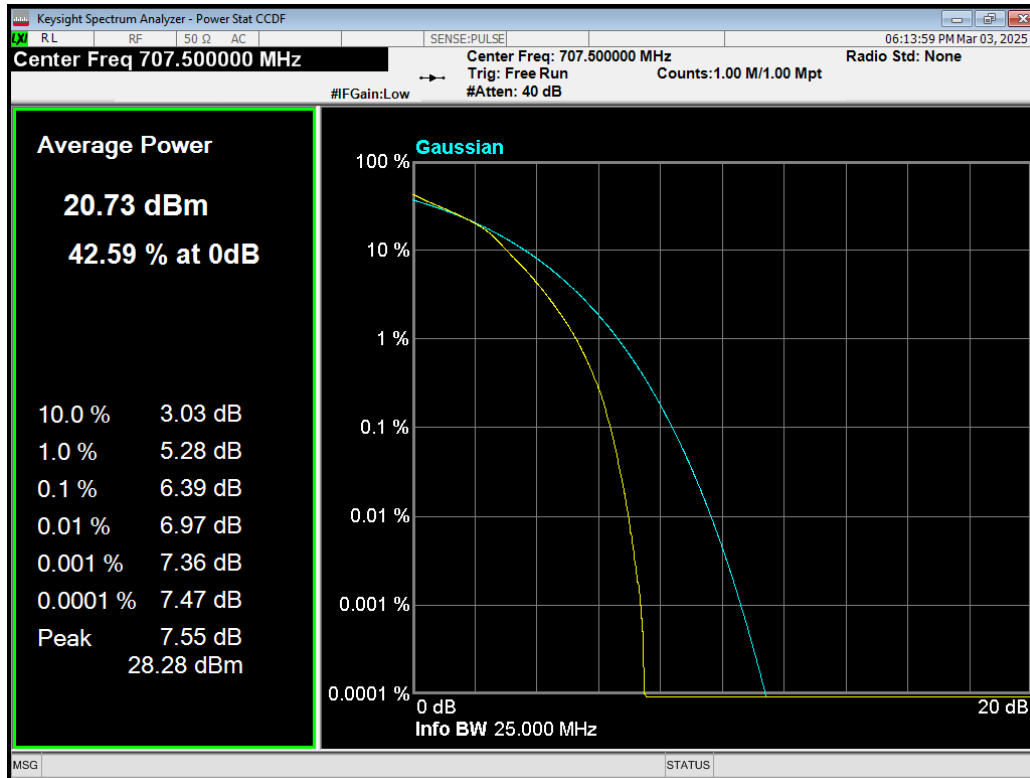
Band12 16QAM BW=10MHz Channel=23095 RB Size=50 Position=#0.png
