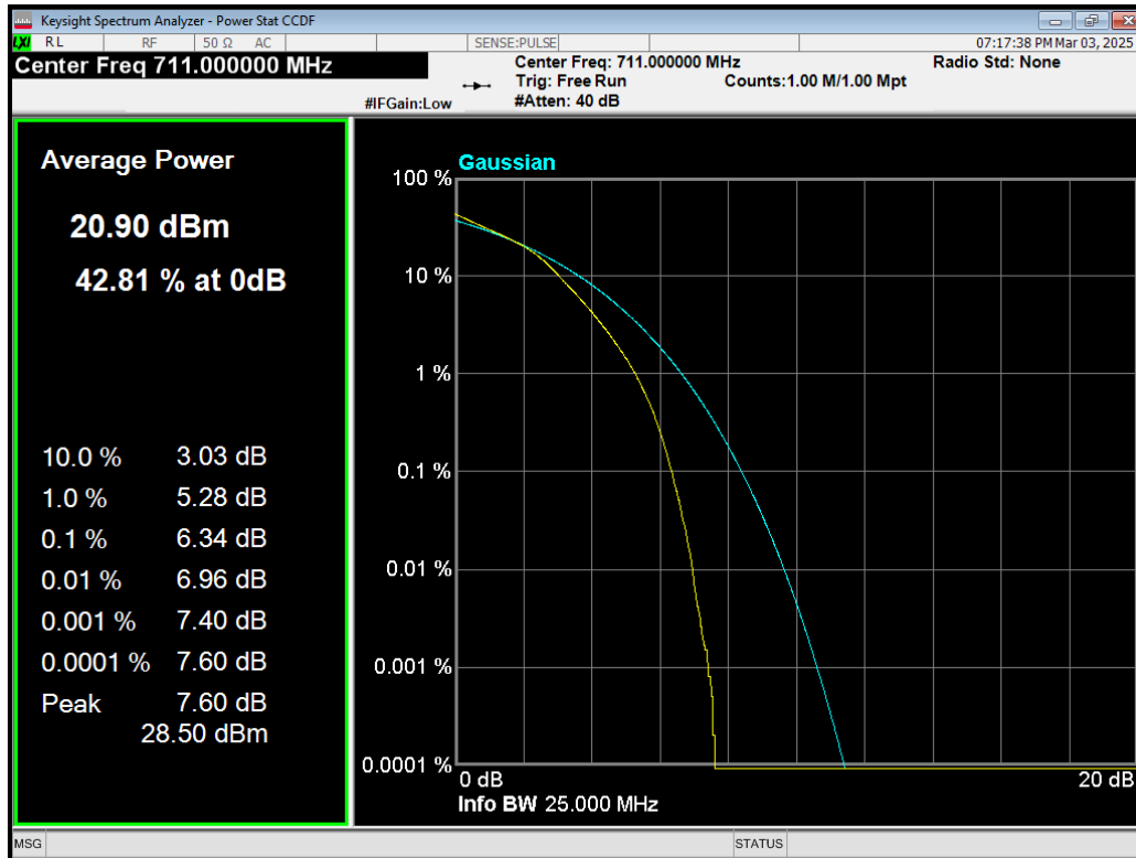
Band17 16QAM BW=10MHz Channel=23800 RB Size=50 Position=#0.png
