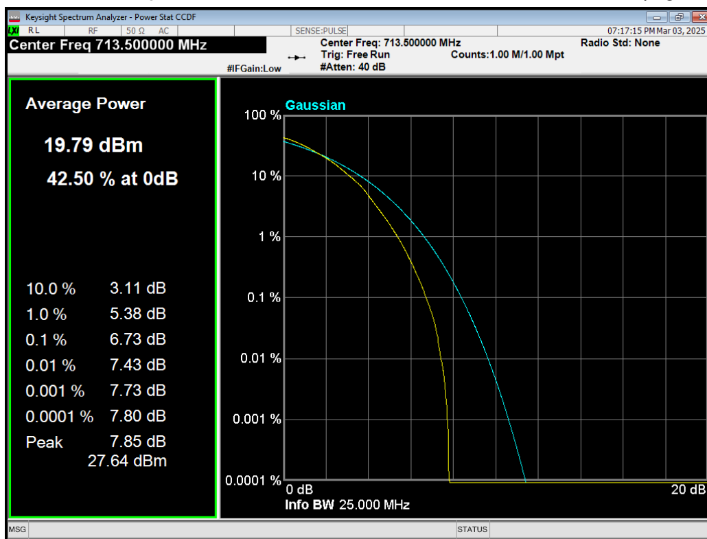
Band17 64QAM BW=5MHz Channel=23825 RB Size=25 Position=#0.png
