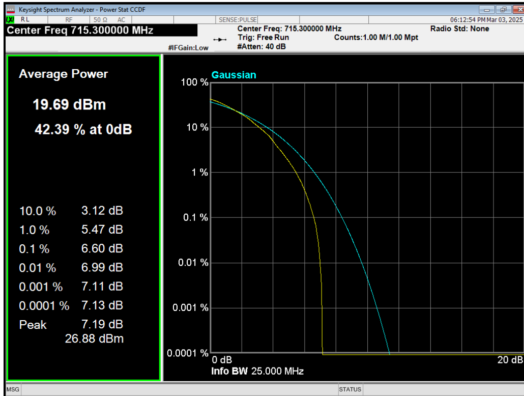
Band12 64QAM BW=1.4MHz Channel=23173 RB Size=6 Position=#0.png
