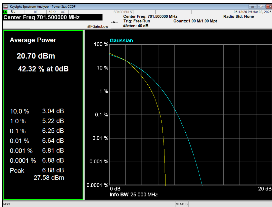
Band12 16QAM BW=5MHz Channel=23035 RB Size=25 Position=#0.png
