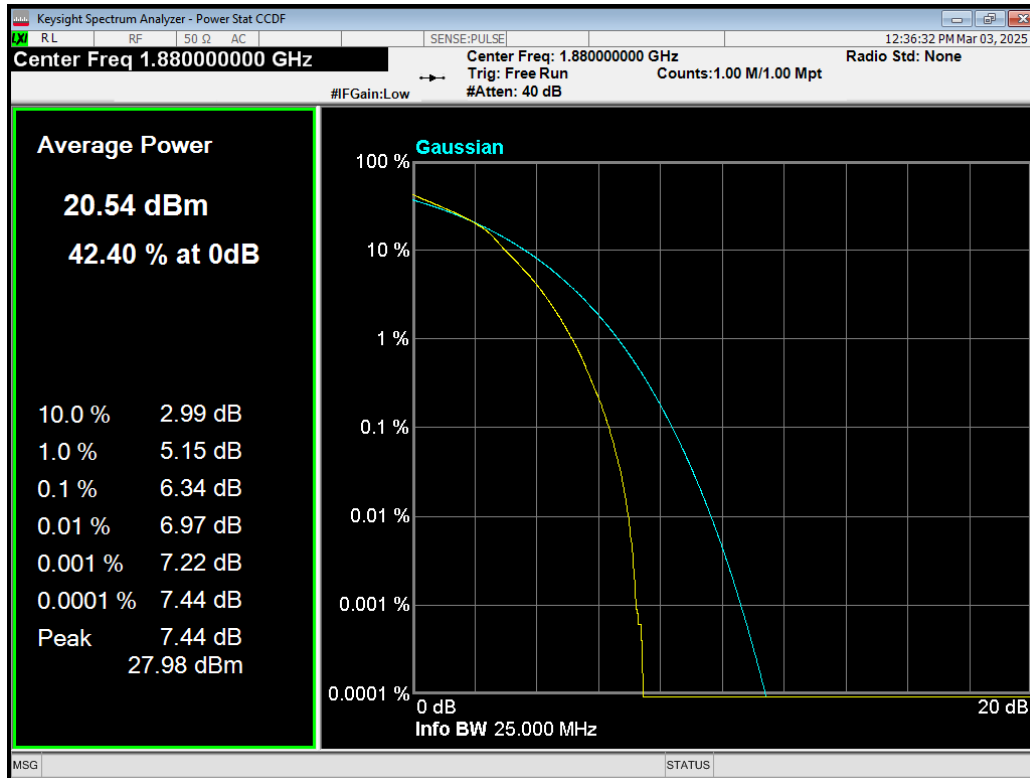
Band2 16QAM BW=5MHz Channel=18900 RB Size=25 Position=#0.png
