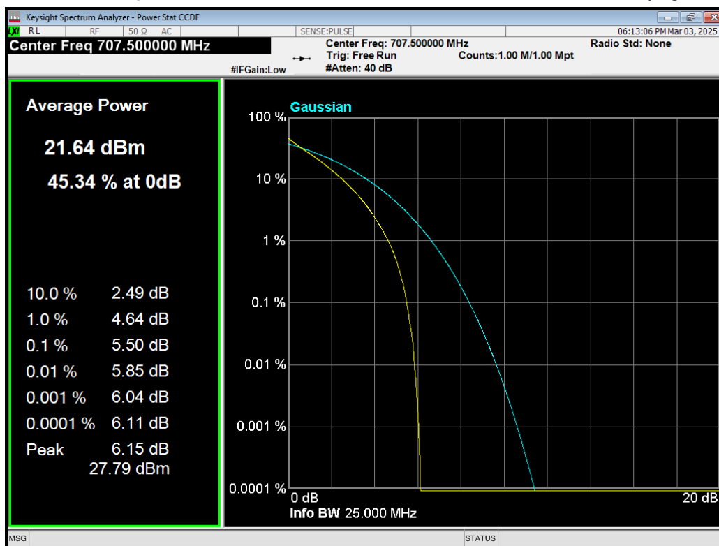
Band12 QPSK BW=3MHz Channel=23095 RB Size=15 Position=#0.png
