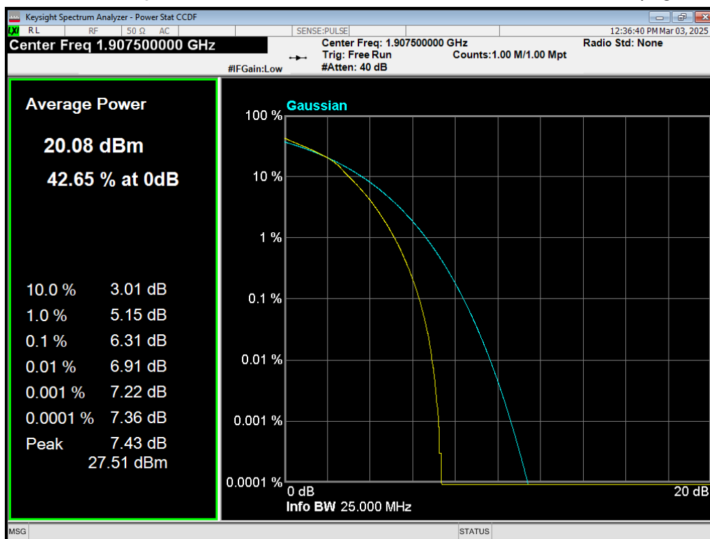
Band2 16QAM BW=5MHz Channel=19175 RB Size=25 Position=#0.png
