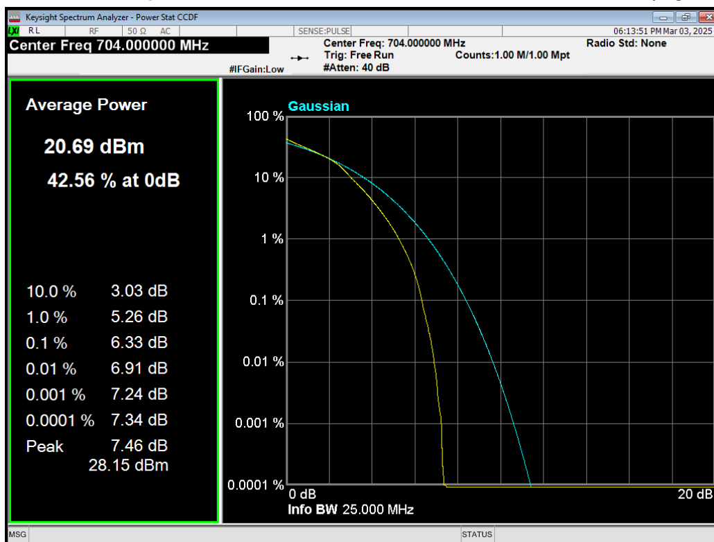
Band12 16QAM BW=10MHz Channel=23060 RB Size=50 Position=#0.png
