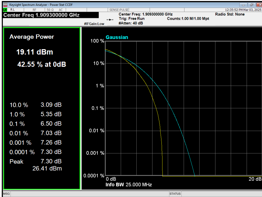
Band2 64QAM BW=1.4MHz Channel=19193 RB Size=6 Position=#0.png
