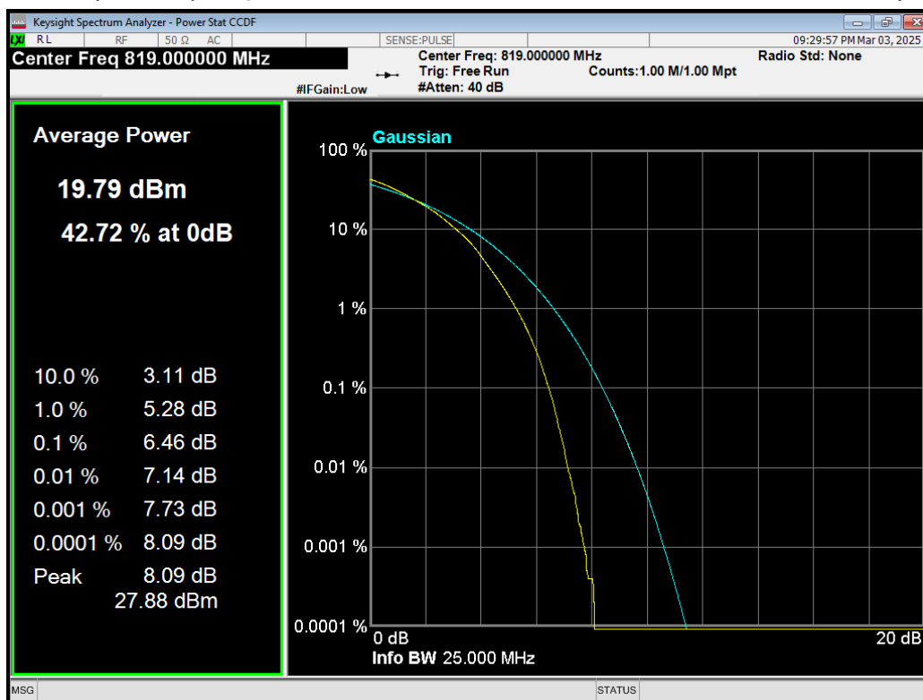
Band26(814-824) 64QAM BW=10MHz Channel=26740 RB Size=50 Position=#0.png
