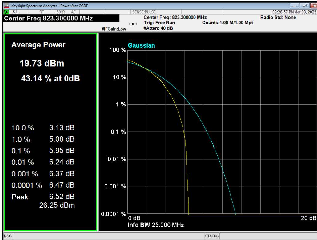
Band26(814-824) 64QAM BW=1.4MHz Channel=26783 RB Size=6 Position=#0.png
