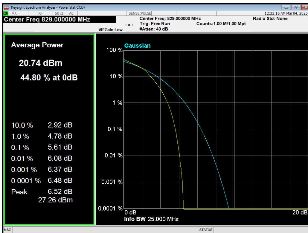
Band26(824-849) 16QAM BW=10MHz Channel=26840 RB Size=50 Position=#0.png
