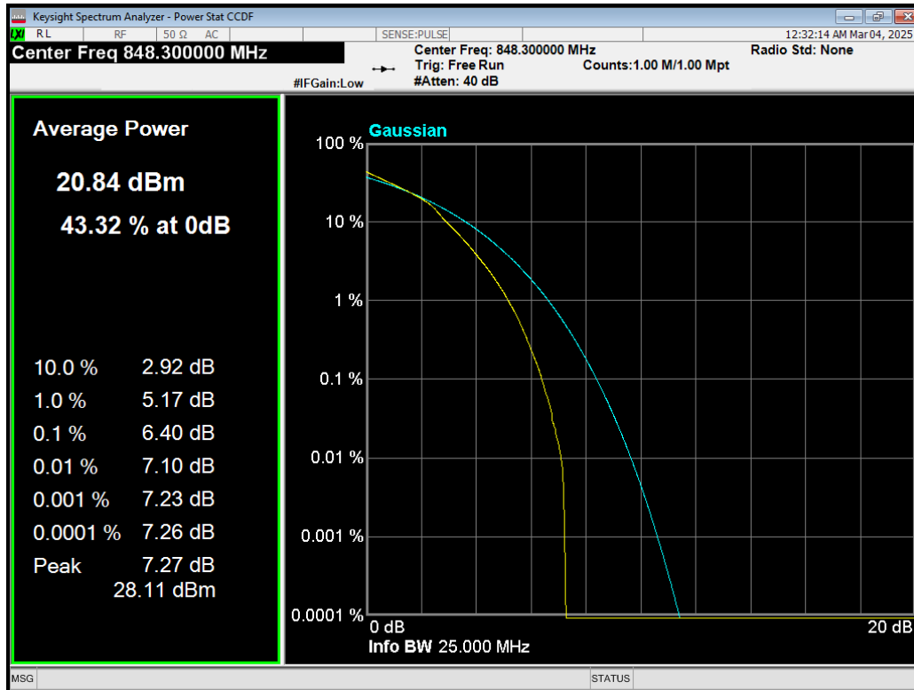
Band26(824-849) 16QAM BW=1.4MHz Channel=27033 RB Size=6 Position=#0.png
