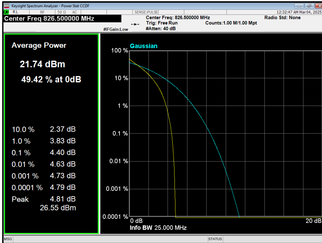
Band26(824-849) QPSK BW=5MHz Channel=26815 RB Size=25 Position=#0.png
