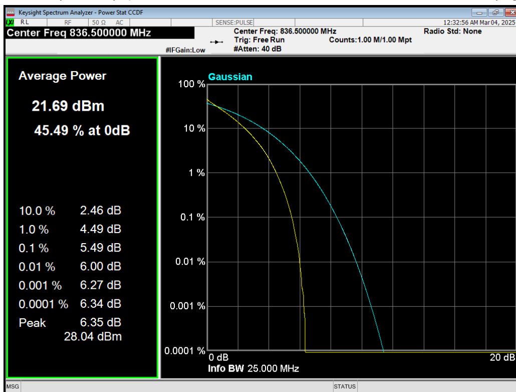
Band26(824-849) QPSK BW=5MHz Channel=26915 RB Size=25 Position=#0.png
