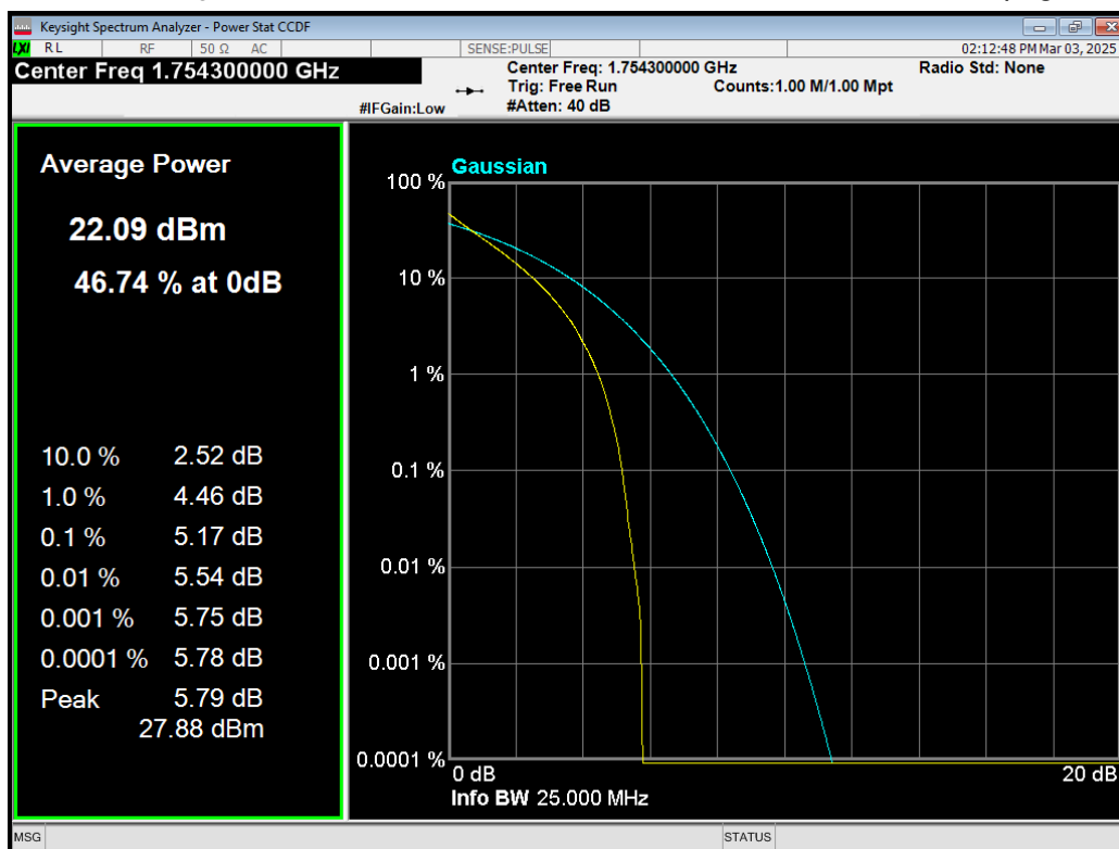
Band4 QPSK BW=1.4MHz Channel=20393 RB Size=6 Position=#0.png
