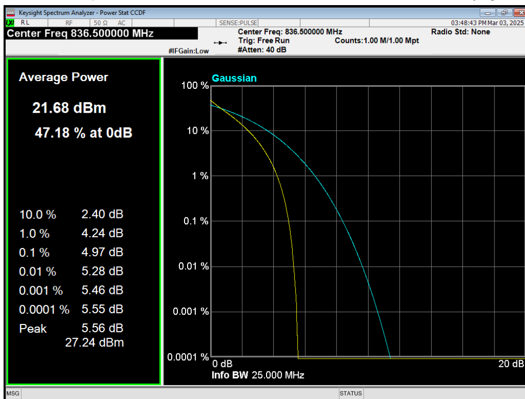
Band5 QPSK BW=10MHz Channel=20525 RB Size=50 Position=#0.png
