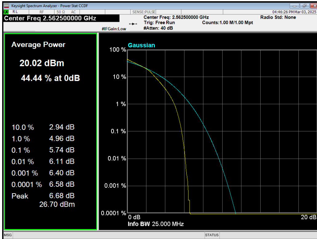
Band7 16QAM BW=15MHz Channel=21375 RB Size=75 Position=#0.png
