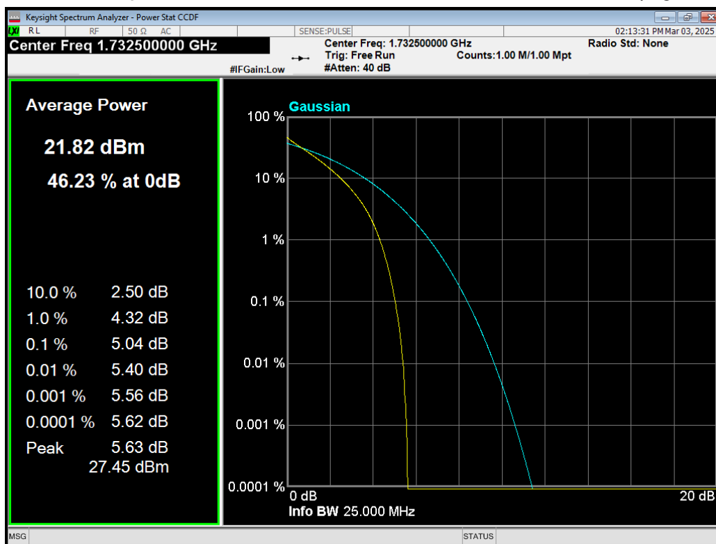
Band4 QPSK BW=5MHz Channel=20175 RB Size=25 Position=#0.png
