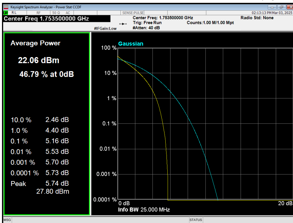
Band4 QPSK BW=3MHz Channel=20385 RB Size=15 Position=#0.png
