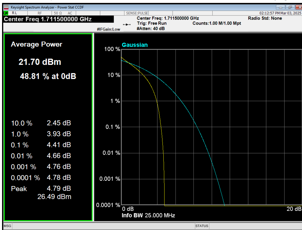
Band4 QPSK BW=3MHz Channel=19965 RB Size=15 Position=#0.png
