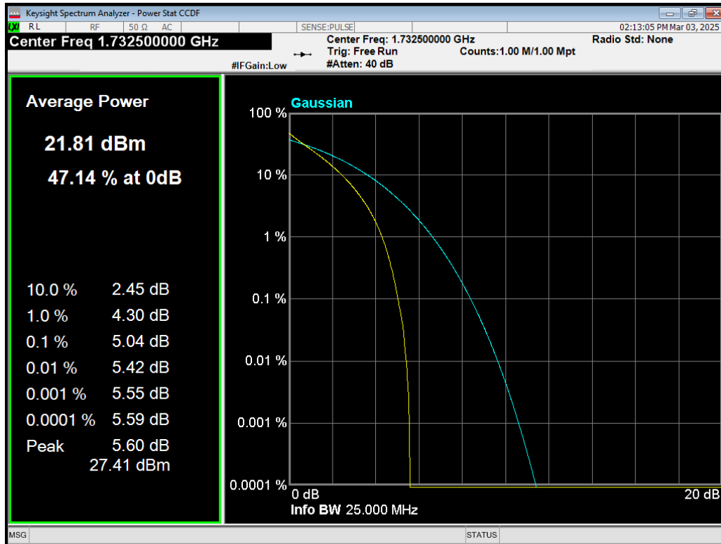
Band4 QPSK BW=3MHz Channel=20175 RB Size=15 Position=#0.png
