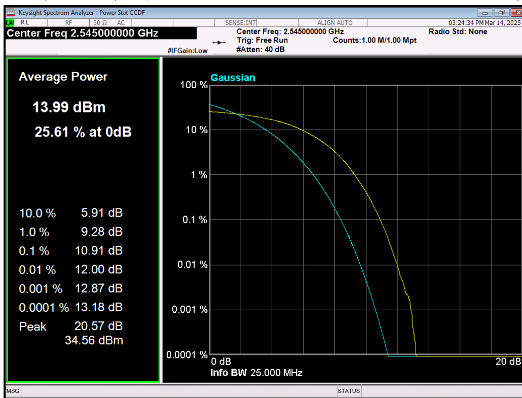
Band41(2535-2655) 64QAM BW=20MHz Channel=40140 RB Size=100 Position=#0.png
