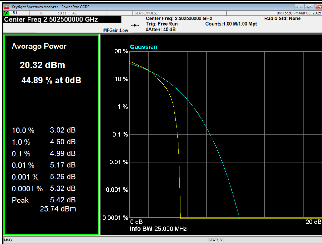
Band7 16QAM BW=5MHz Channel=20775 RB Size=25 Position=#0.png
