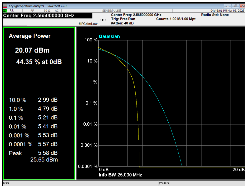
Band7 16QAM BW=10MHz Channel=21400 RB Size=50 Position=#0.png
