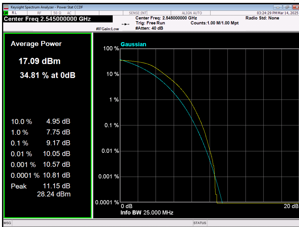
Band41(2535-2655) QPSK BW=20MHz Channel=40140 RB Size=100 Position=#0.png
