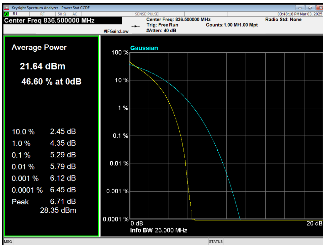
Band5 QPSK BW=5MHz Channel=20525 RB Size=25 Position=#0.png
