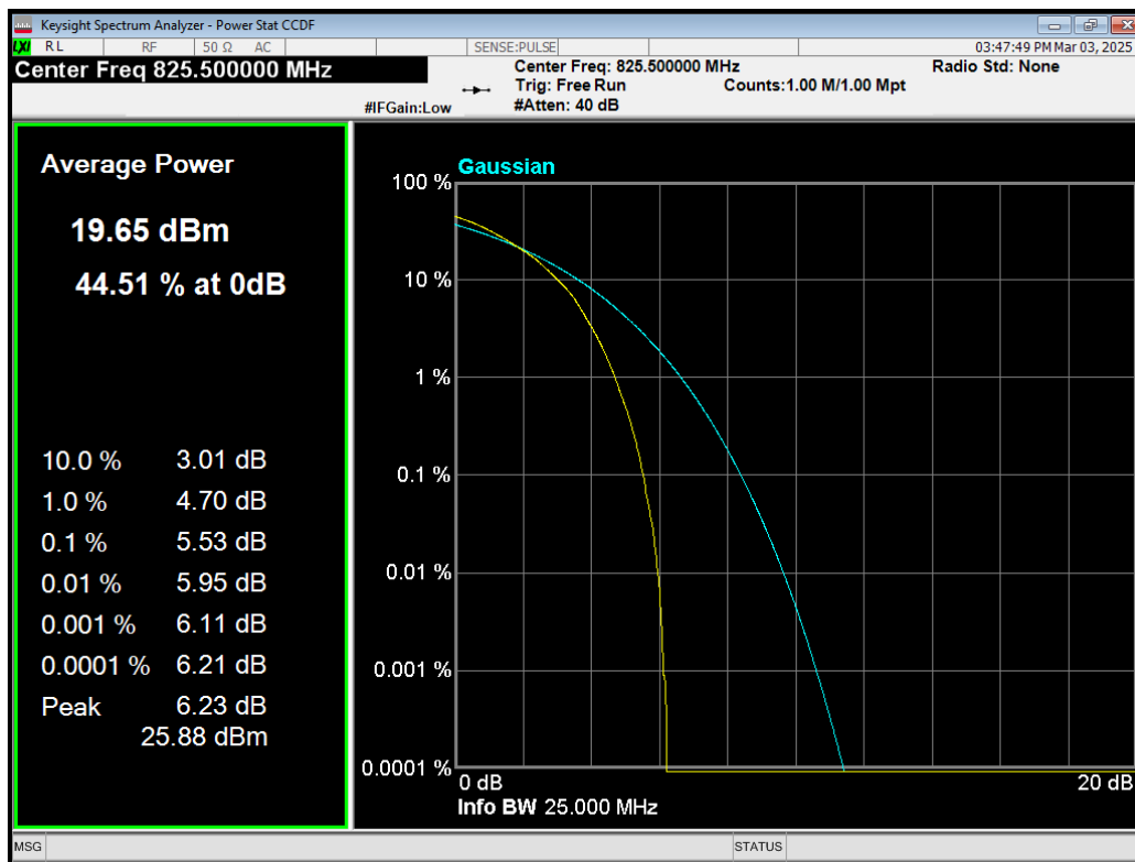
Band5 64QAM BW=3MHz Channel=20415 RB Size=15 Position=#0.png
