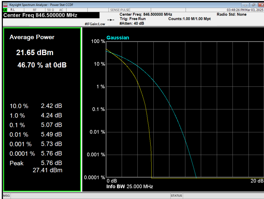
Band5 QPSK BW=5MHz Channel=20625 RB Size=25 Position=#0.png
