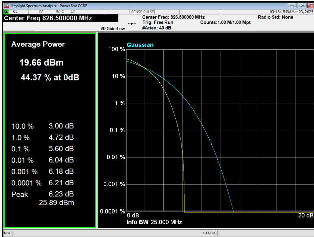
Band5 64QAM BW=5MHz Channel=20425 RB Size=25 Position=#0.png
