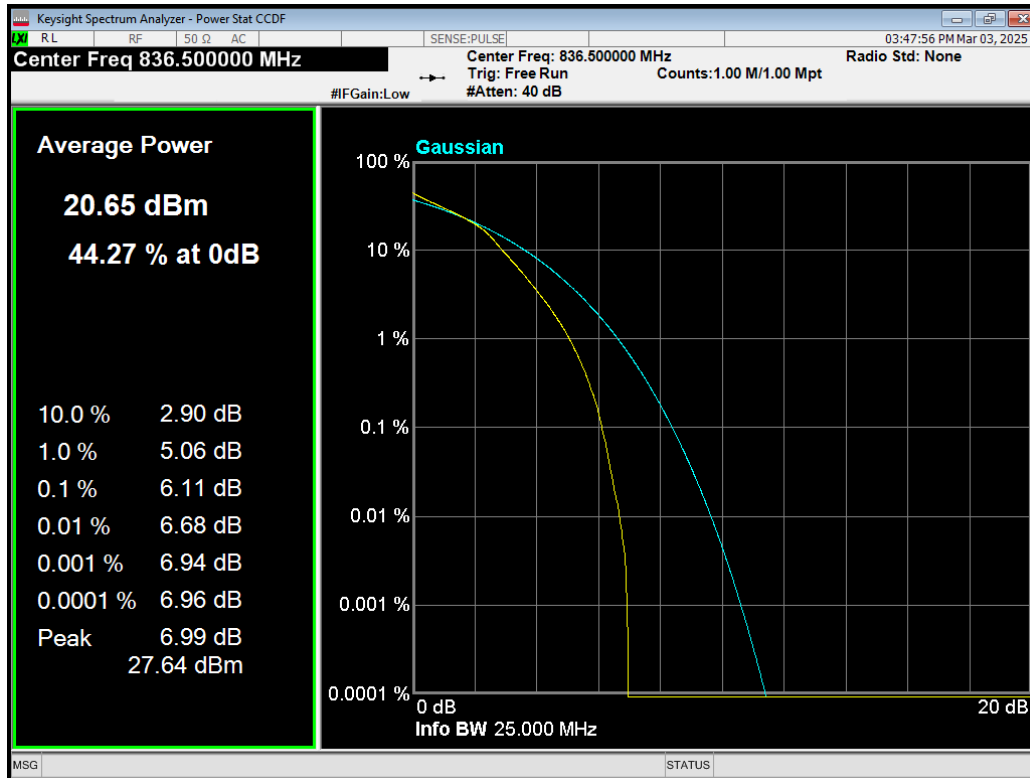
Band5 16QAM BW=3MHz Channel=20525 RB Size=15 Position=#0.png
