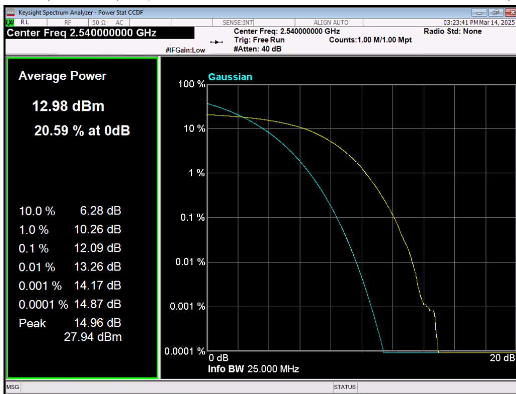
Band41(2535-2655) 64QAM BW=10MHz Channel=40090 RB Size=50 Position=#0.png
