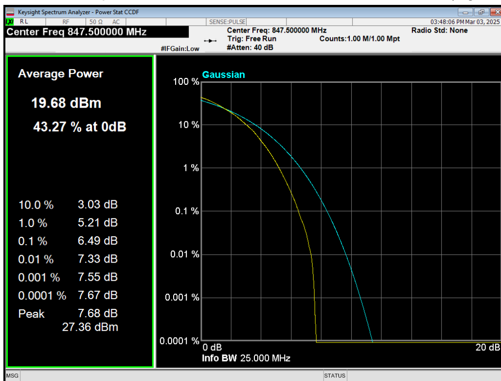
Band5 64QAM BW=3MHz Channel=20635 RB Size=15 Position=#0.png
