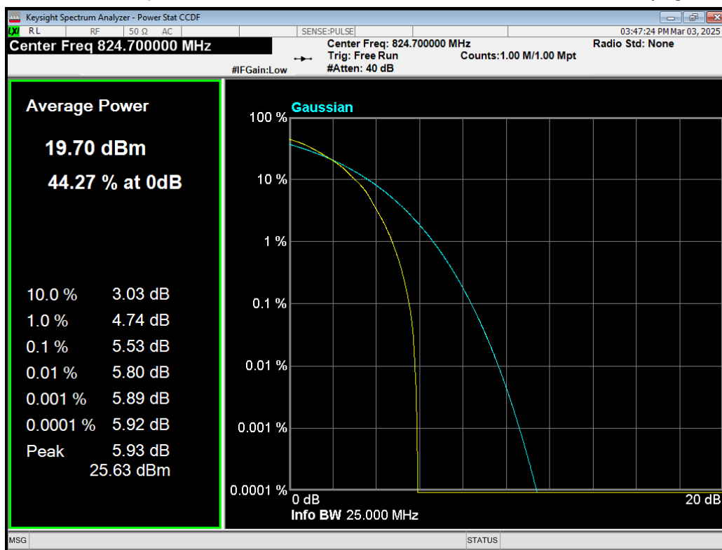
Band5 64QAM BW=1.4MHz Channel=20407 RB Size=6 Position=#0.png
