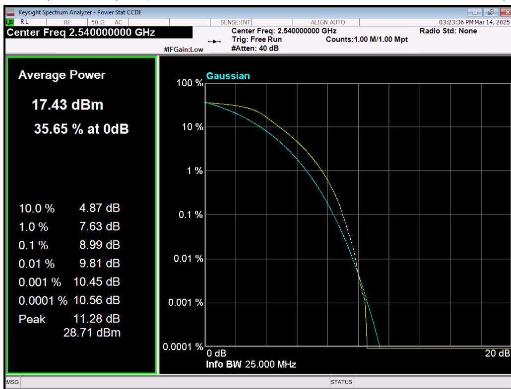
Band41(2535-2655) QPSK BW=10MHz Channel=40090 RB Size=50 Position=#0.png
