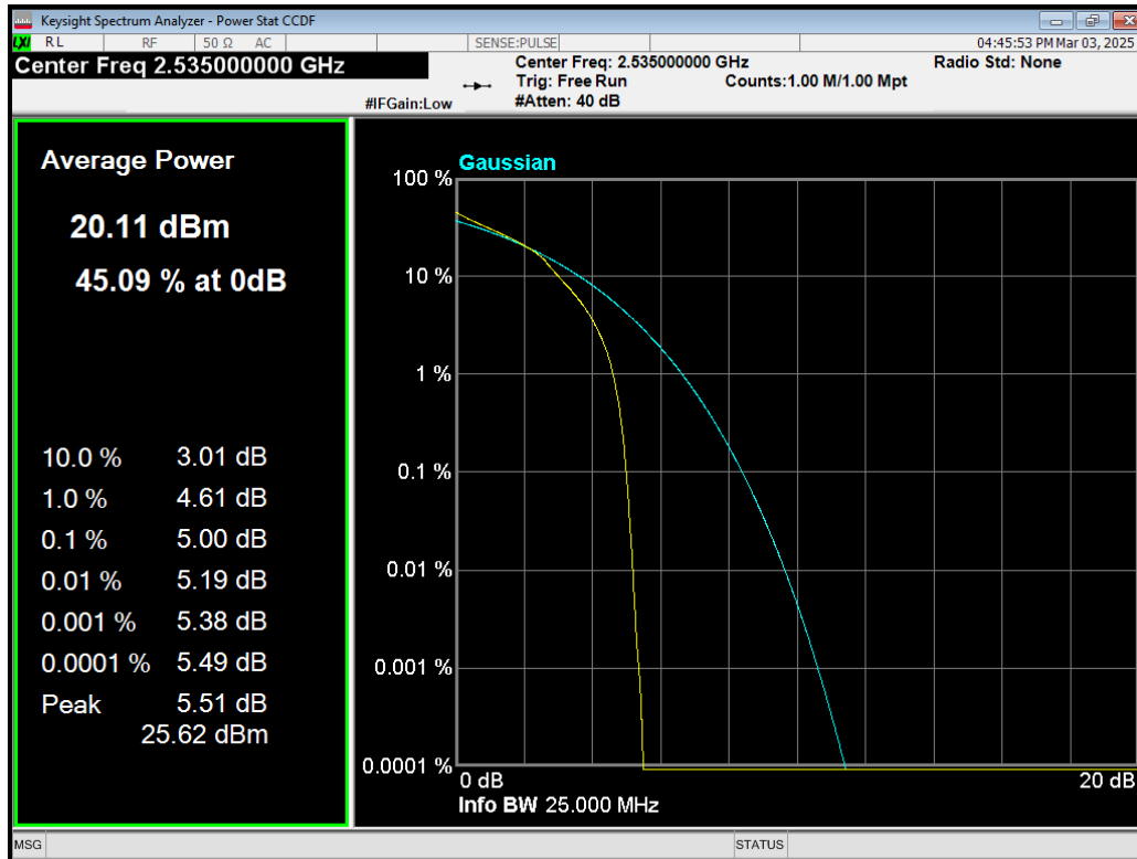
Band7 16QAM BW=10MHz Channel=21100 RB Size=50 Position=#0.png
