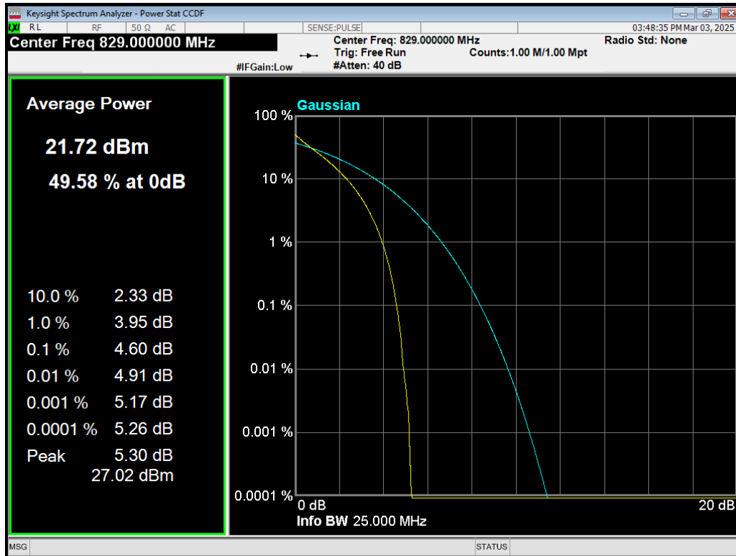
Band5 QPSK BW=10MHz Channel=20450 RB Size=50 Position=#0.png
