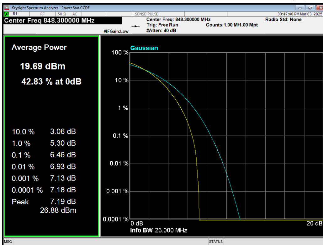
Band5 64QAM BW=1.4MHz Channel=20643 RB Size=6 Position=#0.png
