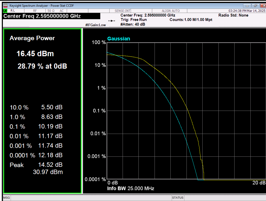
Band41(2535-2655) QPSK BW=20MHz Channel=40640 RB Size=100 Position=#0.png
