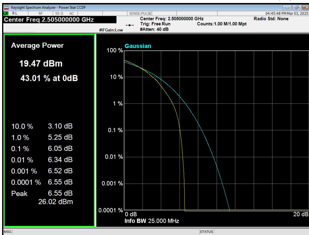
Band7 64QAM BW=10MHz Channel=20800 RB Size=50 Position=#0.png
