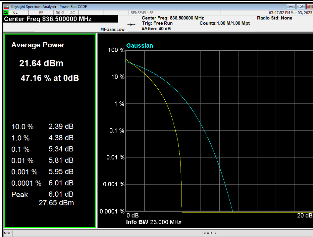
Band5 QPSK BW=3MHz Channel=20525 RB Size=15 Position=#0.png
