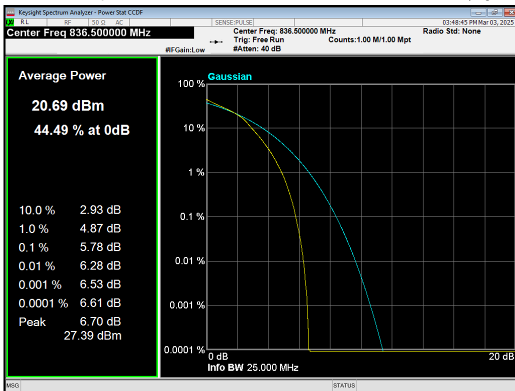
Band5 16QAM BW=10MHz Channel=20525 RB Size=50 Position=#0.png
