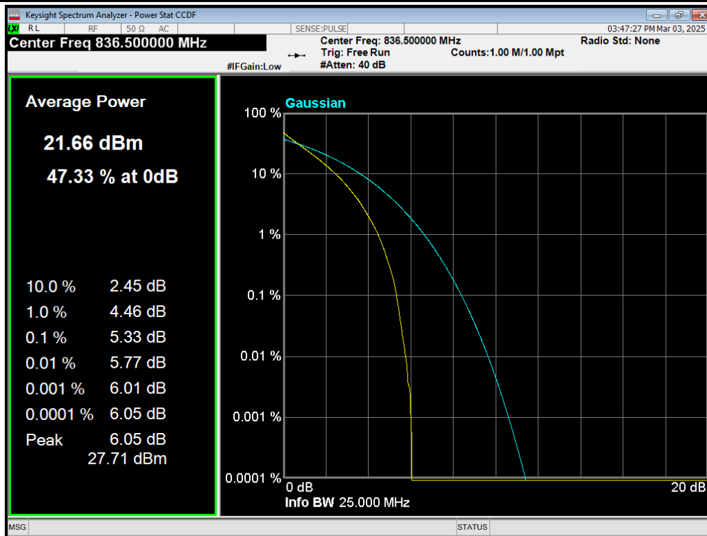
Band5 QPSK BW=1.4MHz Channel=20525 RB Size=6 Position=#0.png
