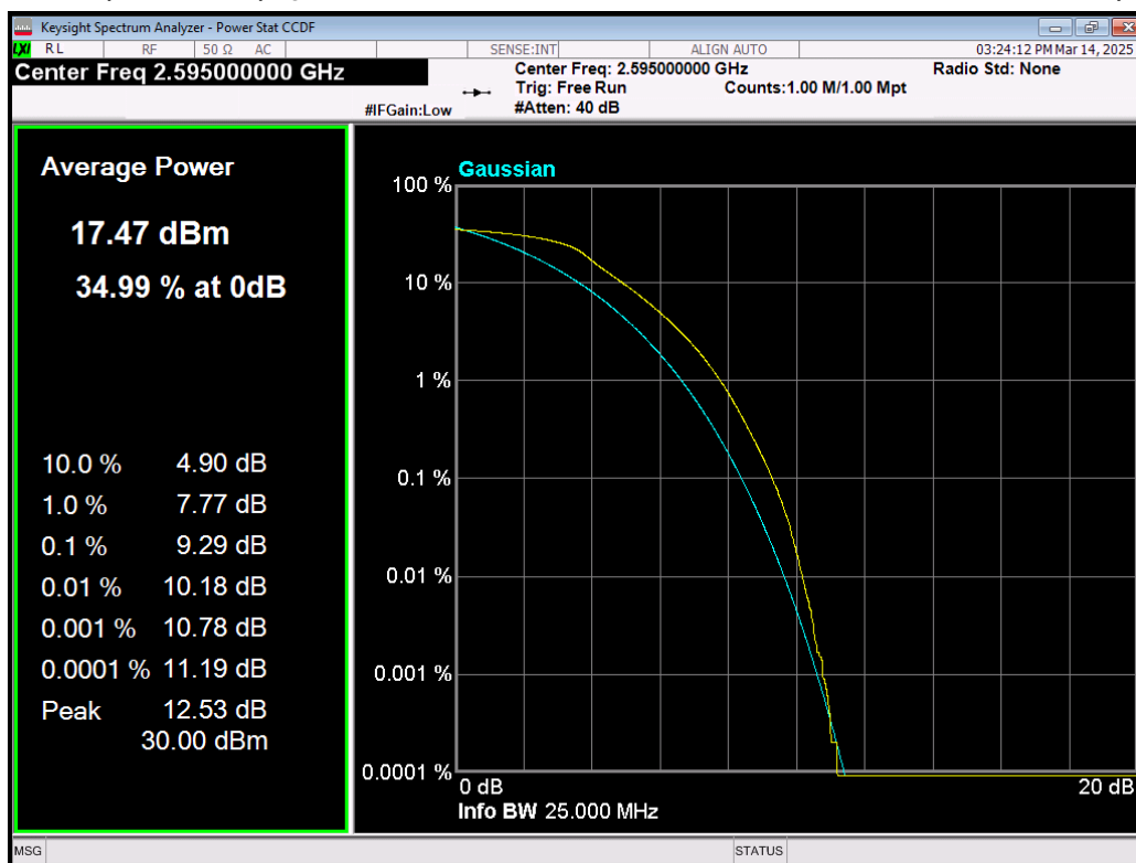
Band41(2535-2655) QPSK BW=15MHz Channel=40640 RB Size=75 Position=#0.png
