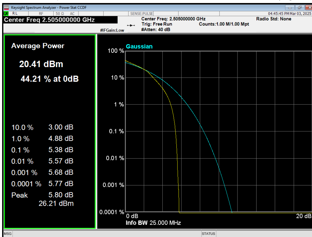
Band7 16QAM BW=10MHz Channel=20800 RB Size=50 Position=#0.png
