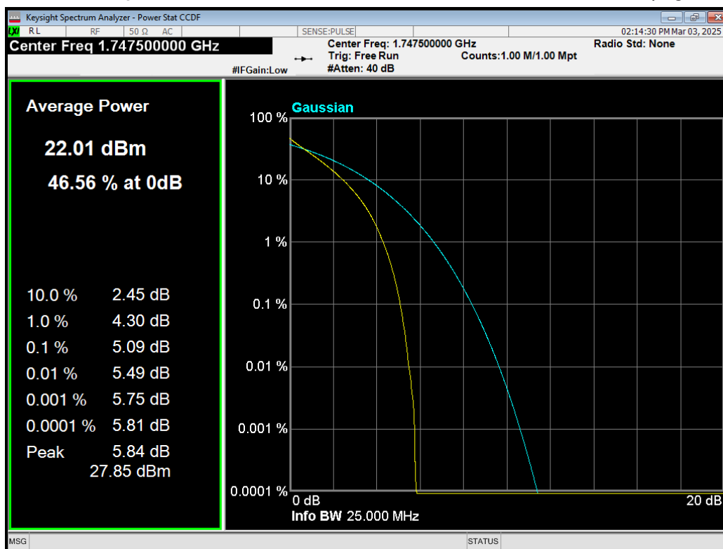
Band4 QPSK BW=15MHz Channel=20325 RB Size=75 Position=#0.png
