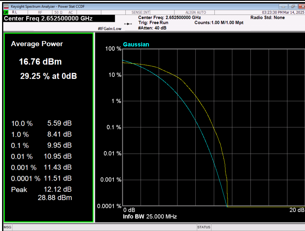
Band41(2535-2655) 16QAM BW=5MHz Channel=41215 RB Size=25 Position=#0.png
