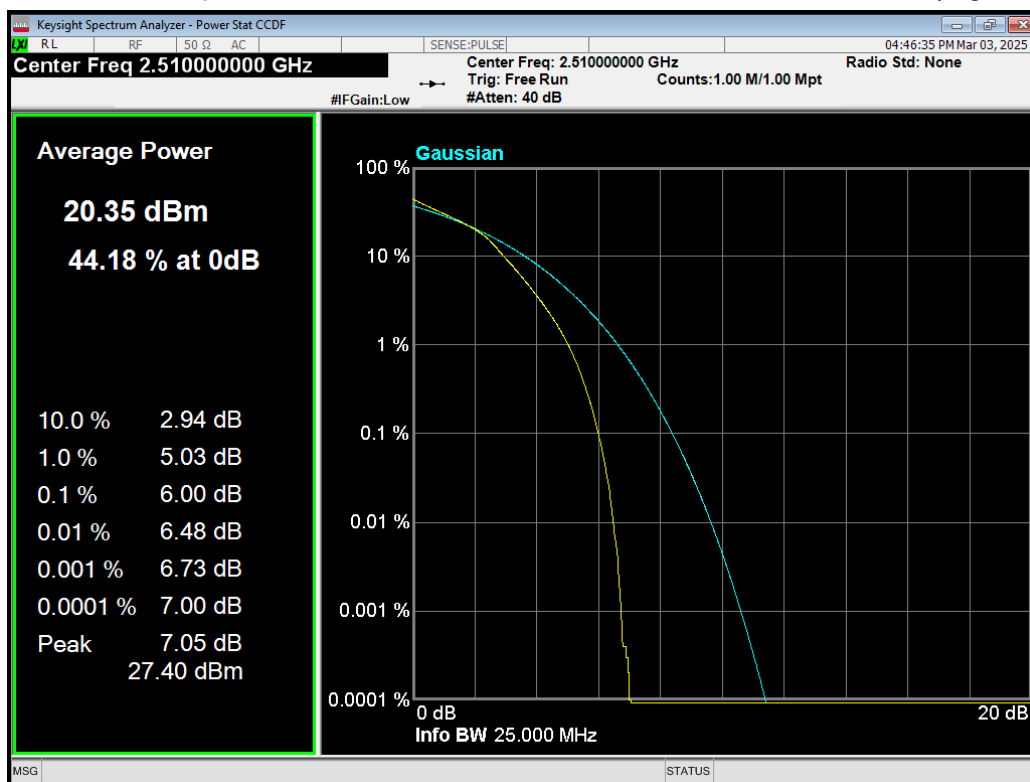
Band7 16QAM BW=20MHz Channel=20850 RB Size=100 Position=#0.png
