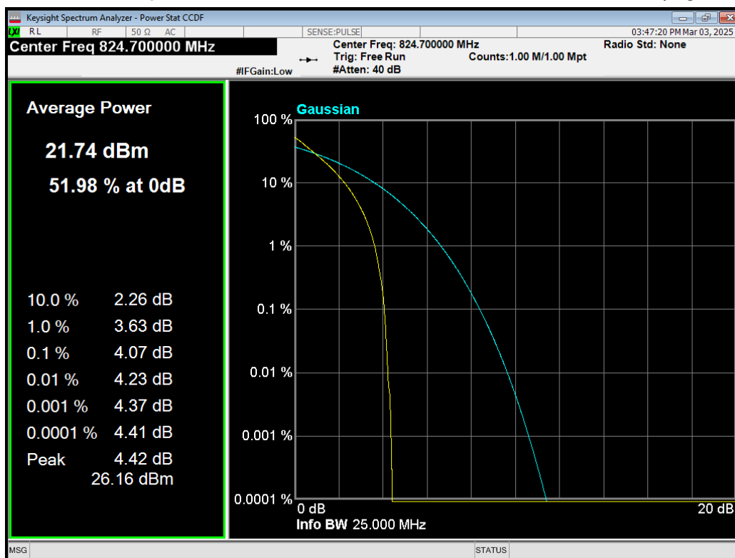
Band5 QPSK BW=1.4MHz Channel=20407 RB Size=6 Position=#0.png
