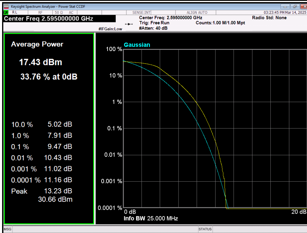
Band41(2535-2655) QPSK BW=10MHz Channel=40640 RB Size=50 Position=#0.png
