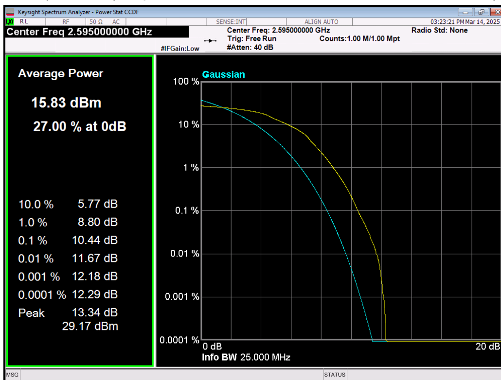
Band41(2535-2655) 16QAM BW=5MHz Channel=40640 RB Size=25 Position=#0.png
