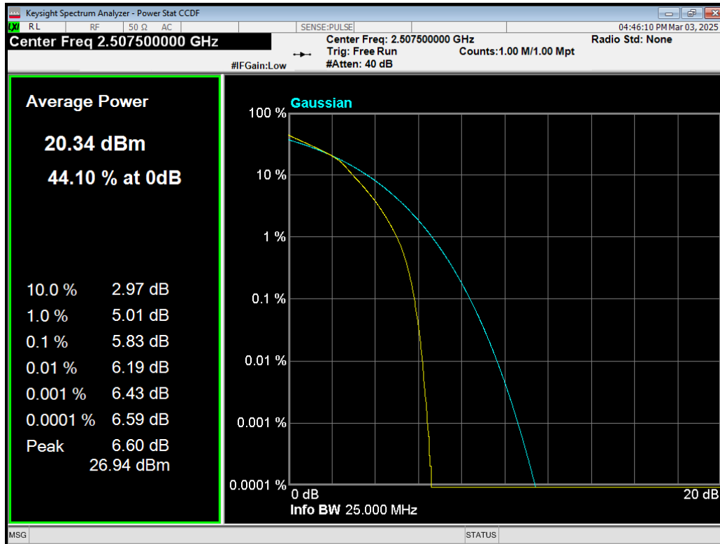
Band7 16QAM BW=15MHz Channel=20825 RB Size=75 Position=#0.png
