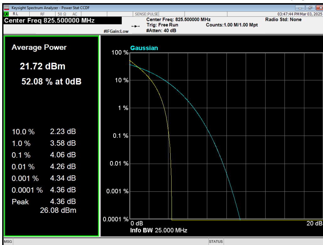
Band5 QPSK BW=3MHz Channel=20415 RB Size=15 Position=#0.png
