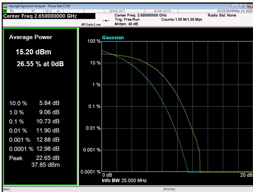
Band41(2535-2655) 64QAM BW=10MHz Channel=41190 RB Size=50 Position=#0.png
