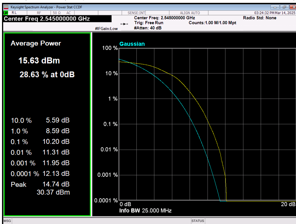
Band41(2535-2655) 16QAM BW=20MHz Channel=40140 RB Size=100 Position=#0.png
