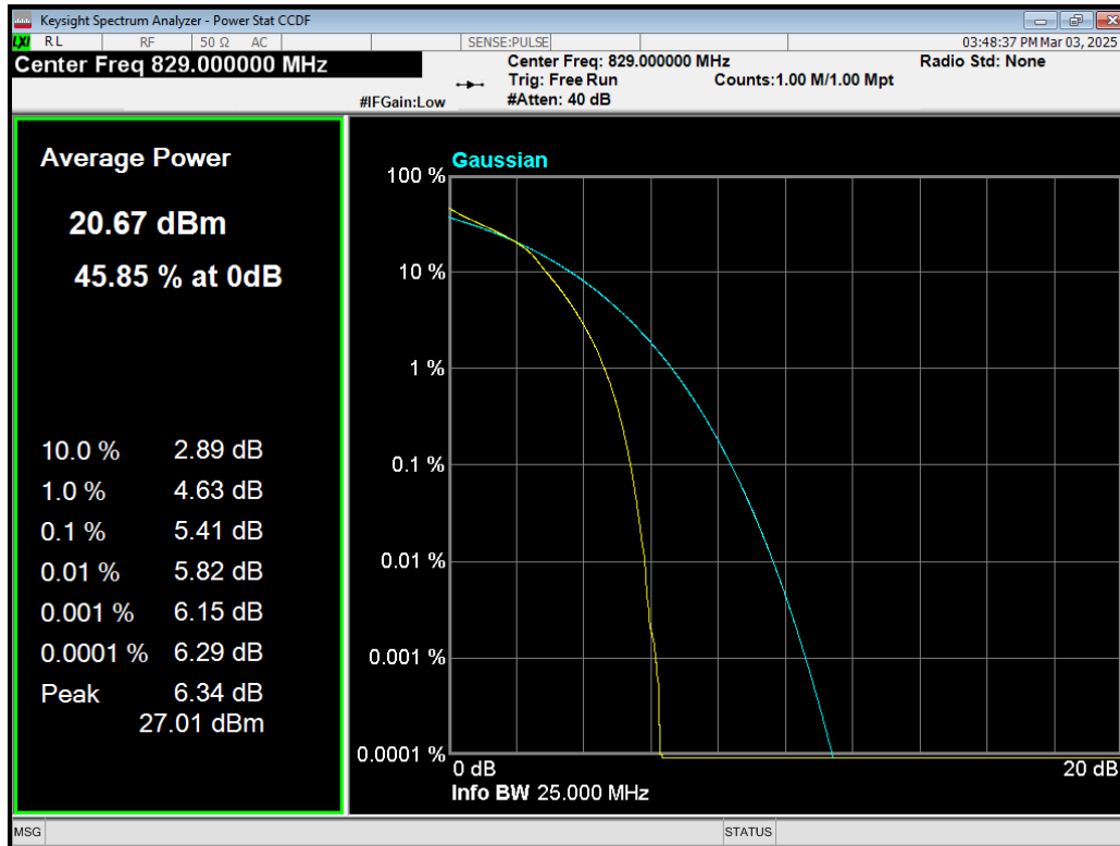
Band5 16QAM BW=10MHz Channel=20450 RB Size=50 Position=#0.png
