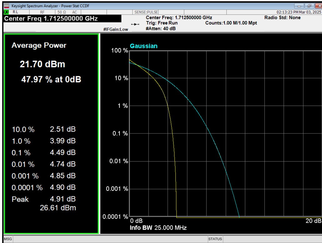
Band4 QPSK BW=5MHz Channel=19975 RB Size=25 Position=#0.png
