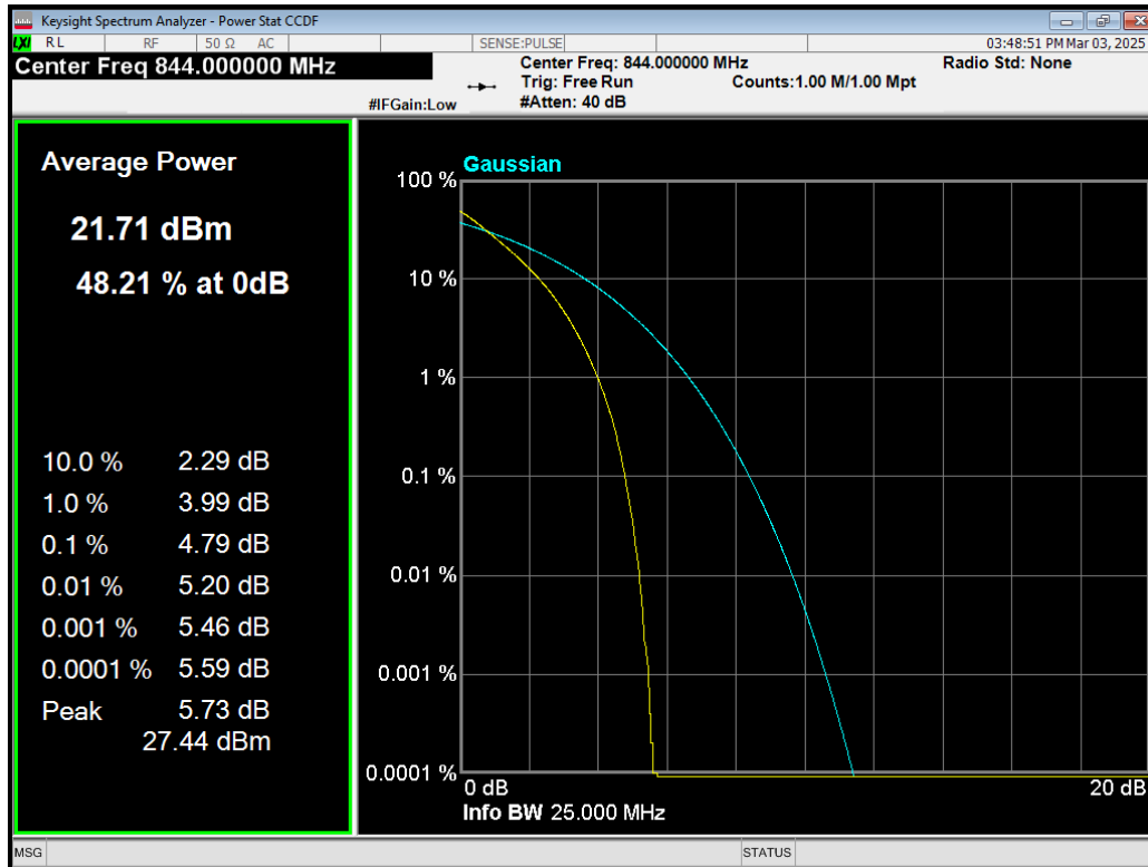
Band5 QPSK BW=10MHz Channel=20600 RB Size=50 Position=#0.png
