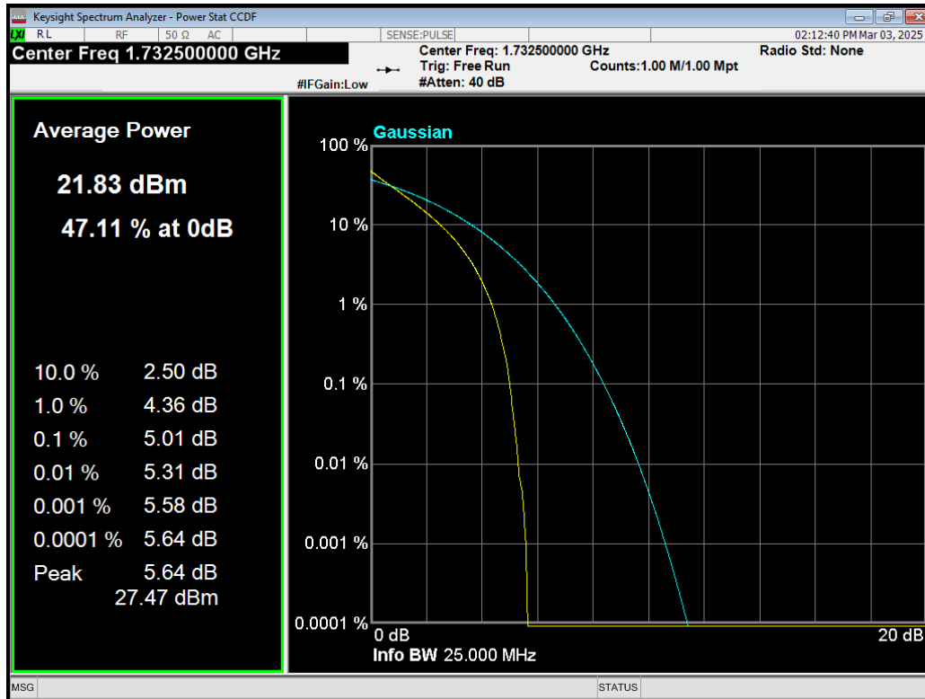
Band4 QPSK BW=1.4MHz Channel=20175 RB Size=6 Position=#0.png
