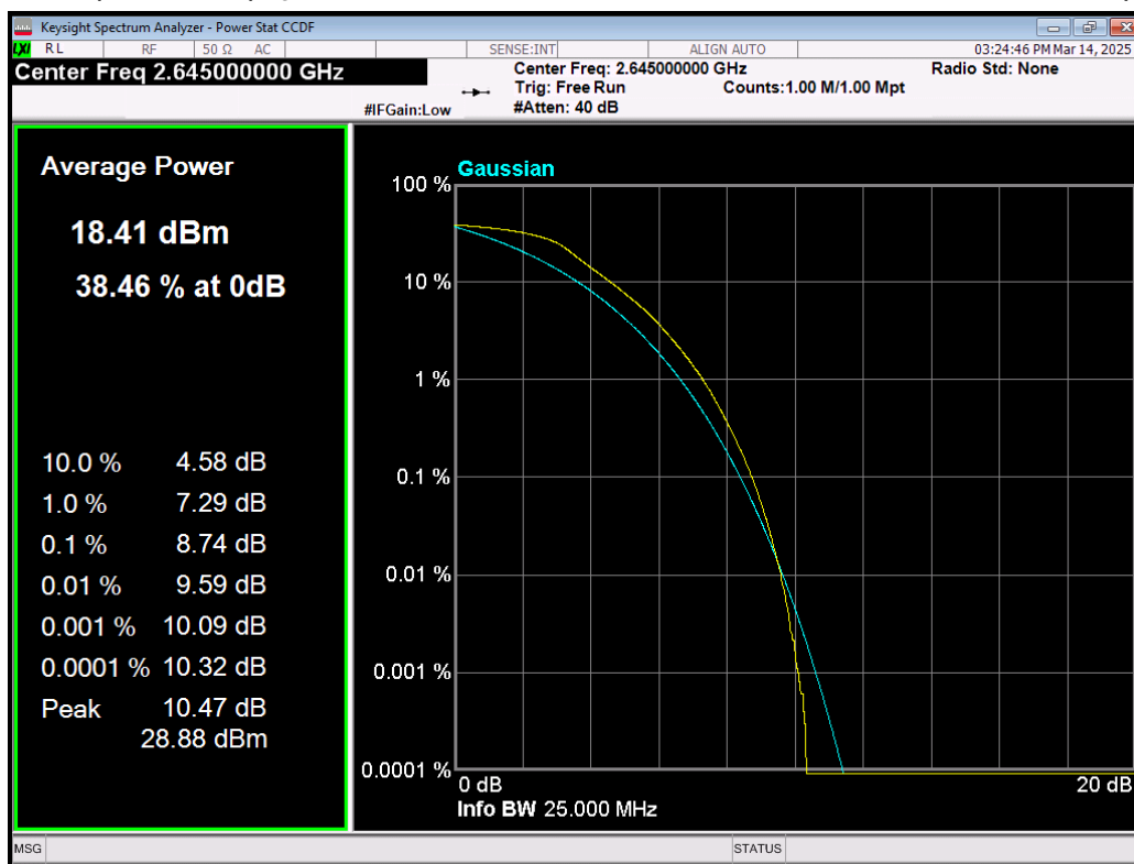
Band41(2535-2655) QPSK BW=20MHz Channel=41140 RB Size=100 Position=#0.png
