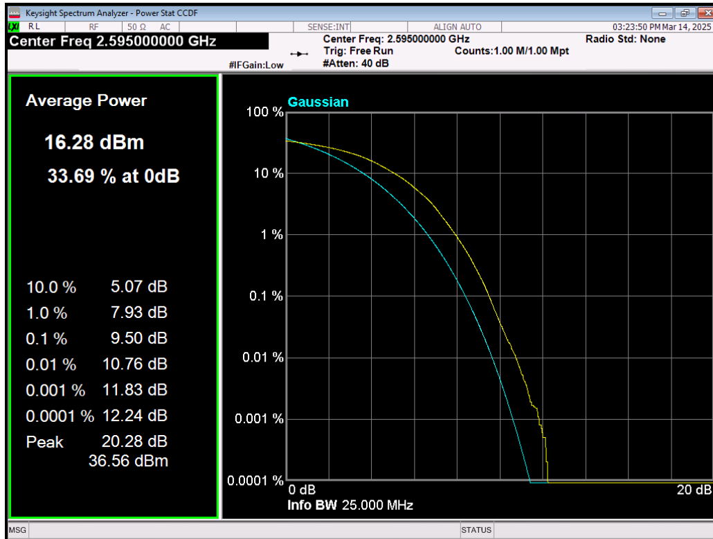
Band41(2535-2655) 64QAM BW=10MHz Channel=40640 RB Size=50 Position=#0.png
