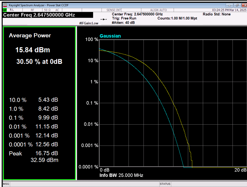
Band41(2535-2655) 64QAM BW=15MHz Channel=41165 RB Size=75 Position=#0.png
