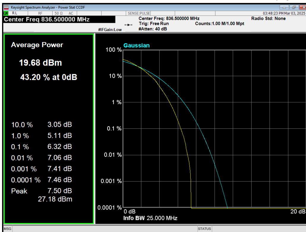
Band5 64QAM BW=5MHz Channel=20525 RB Size=25 Position=#0.png
