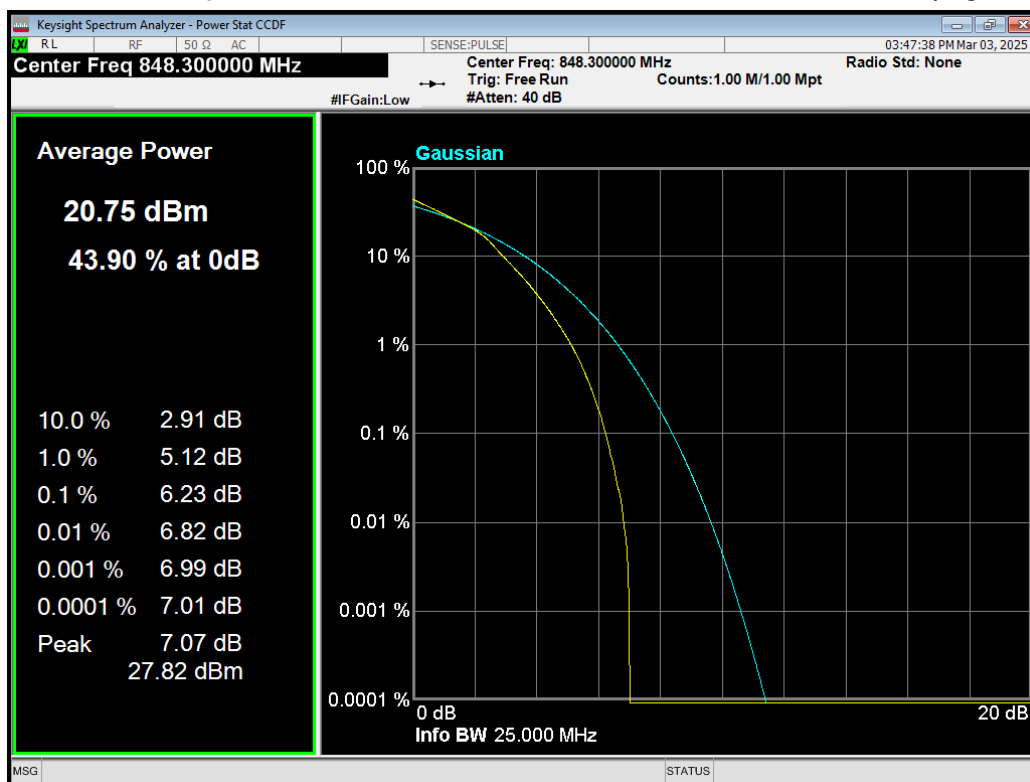
Band5 16QAM BW=1.4MHz Channel=20643 RB Size=6 Position=#0.png
