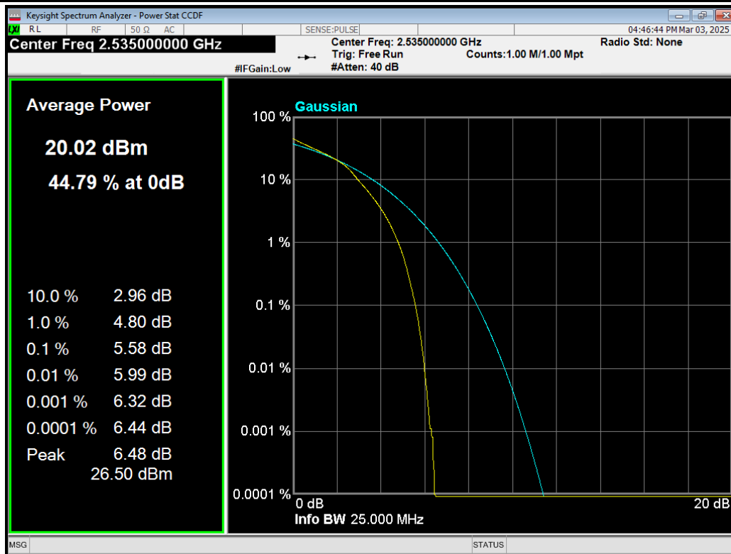
Band7 16QAM BW=20MHz Channel=21100 RB Size=100 Position=#0.png
