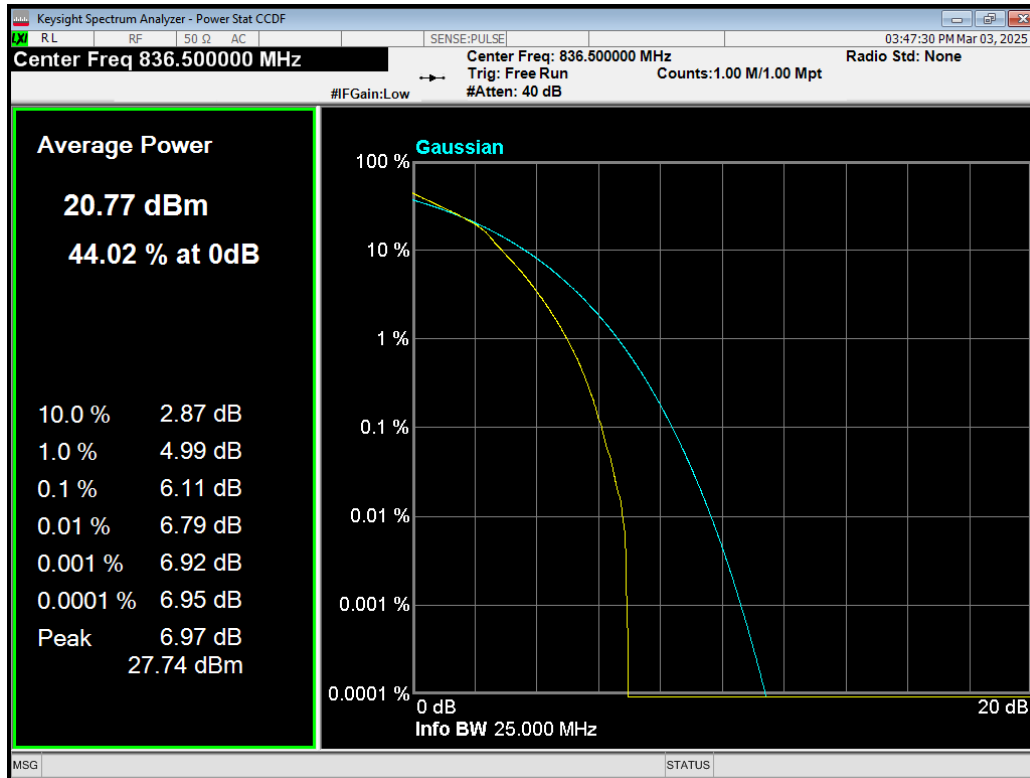
Band5 16QAM BW=1.4MHz Channel=20525 RB Size=6 Position=#0.png
