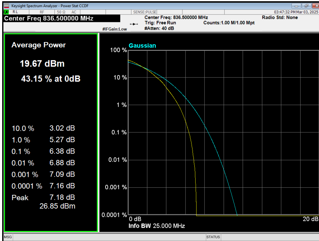
Band5 64QAM BW=1.4MHz Channel=20525 RB Size=6 Position=#0.png
