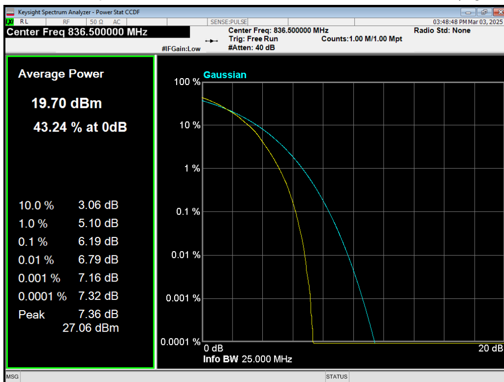
Band5 64QAM BW=10MHz Channel=20525 RB Size=50 Position=#0.png
