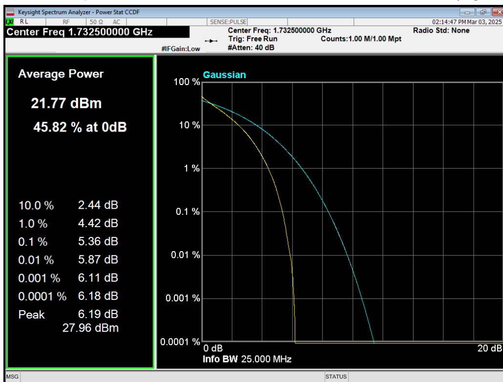
Band4 QPSK BW=20MHz Channel=20175 RB Size=100 Position=#0.png
