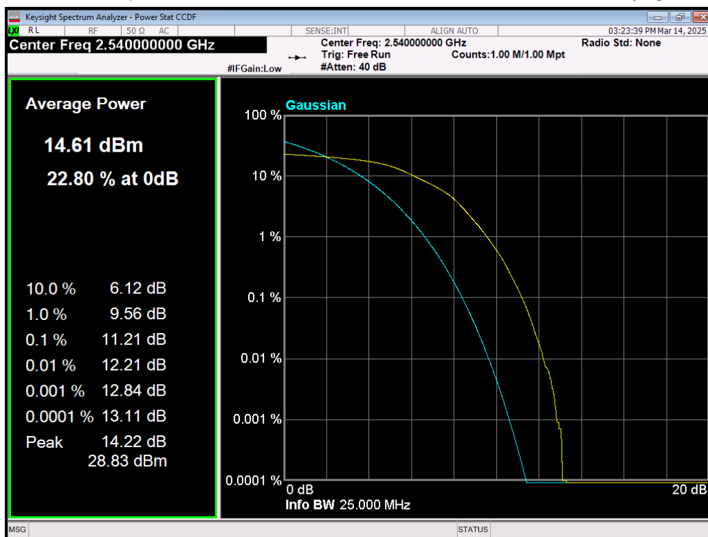
Band41(2535-2655) 16QAM BW=10MHz Channel=40090 RB Size=50 Position=#0.png
