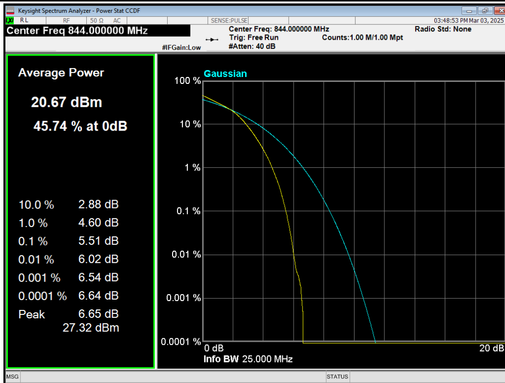
Band5 16QAM BW=10MHz Channel=20600 RB Size=50 Position=#0.png
