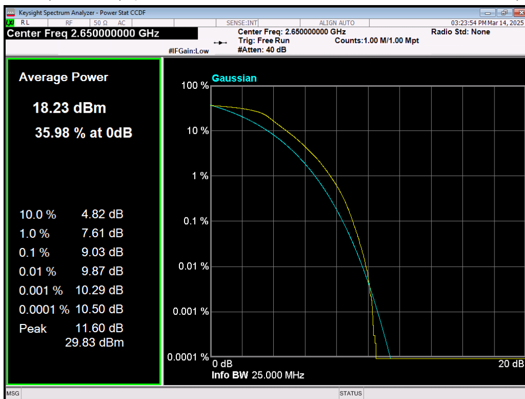
Band41(2535-2655) QPSK BW=10MHz Channel=41190 RB Size=50 Position=#0.png
