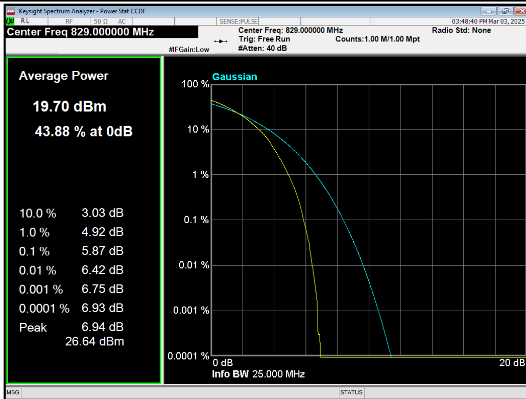
Band5 64QAM BW=10MHz Channel=20450 RB Size=50 Position=#0.png
