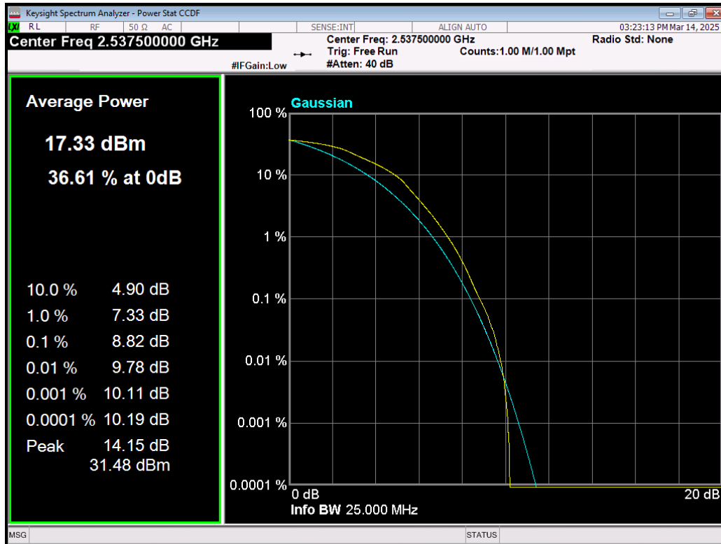
Band41(2535-2655) 16QAM BW=5MHz Channel=40065 RB Size=25 Position=#0.png
