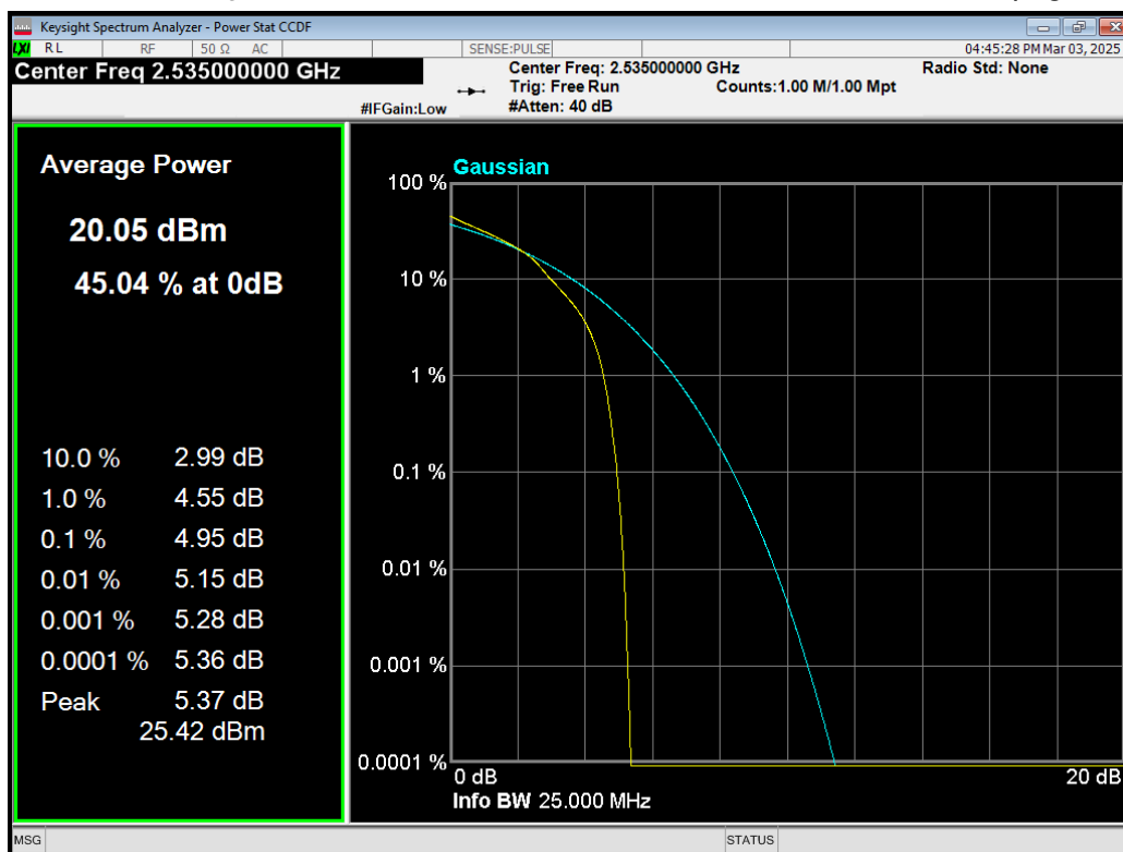
Band7 16QAM BW=5MHz Channel=21100 RB Size=25 Position=#0.png
