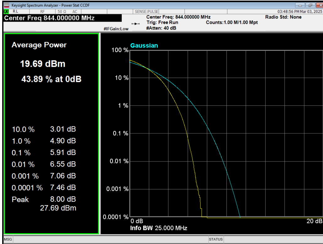
Band5 64QAM BW=10MHz Channel=20600 RB Size=50 Position=#0.png
