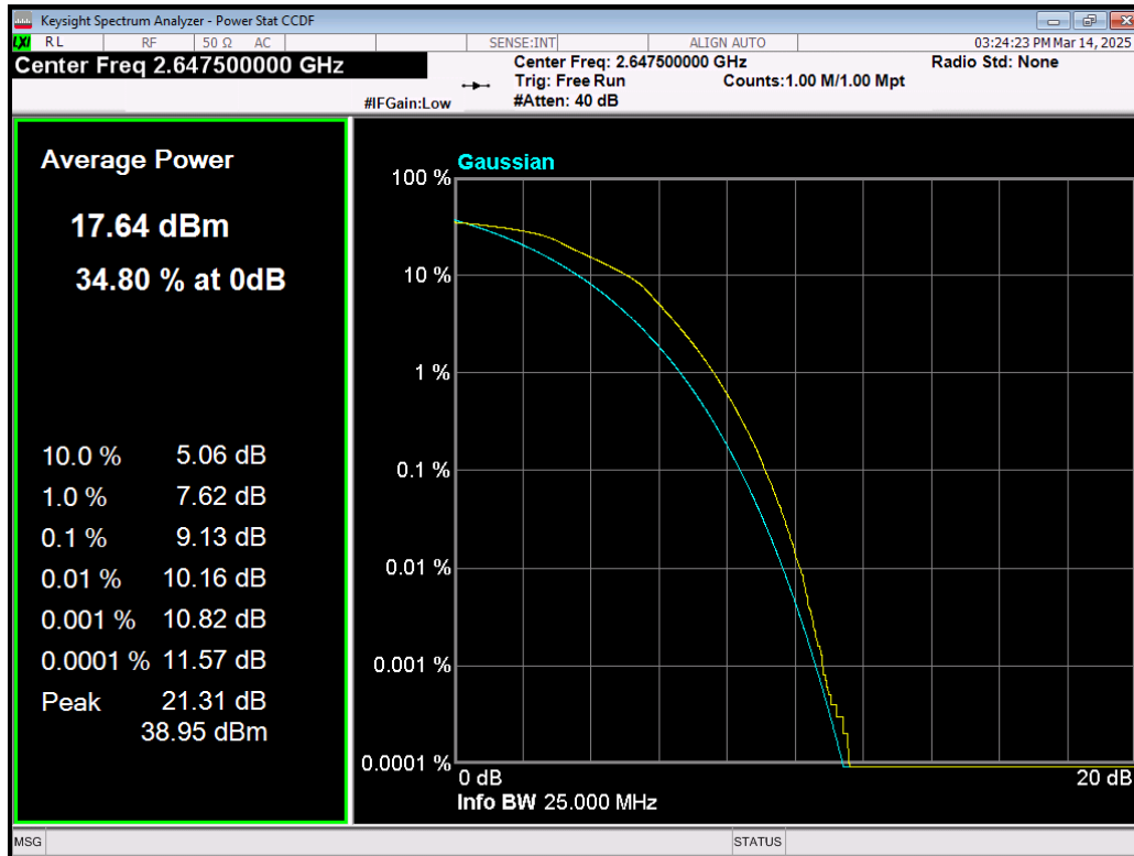
Band41(2535-2655) 16QAM BW=15MHz Channel=41165 RB Size=75 Position=#0.png
