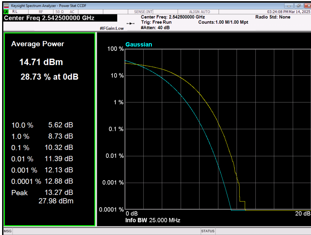
Band41(2535-2655) 64QAM BW=15MHz Channel=40115 RB Size=75 Position=#0.png
