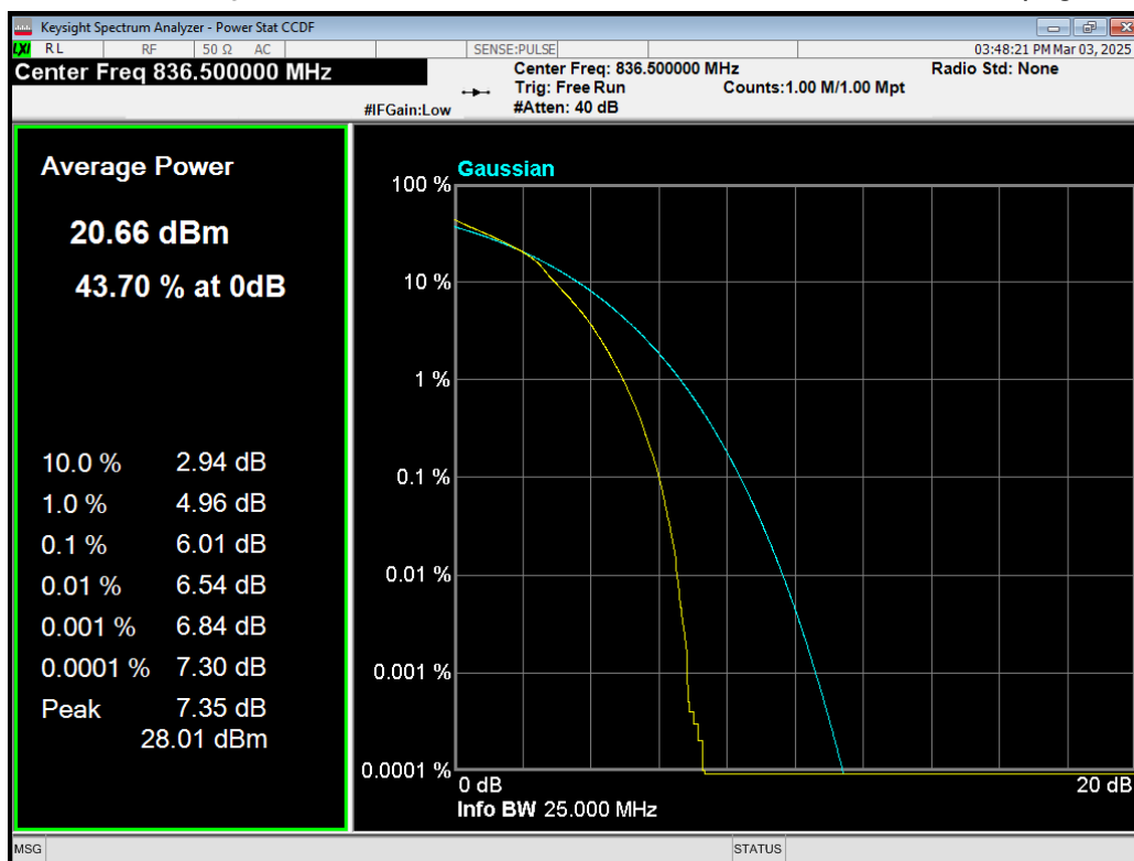
Band5 16QAM BW=5MHz Channel=20525 RB Size=25 Position=#0.png
