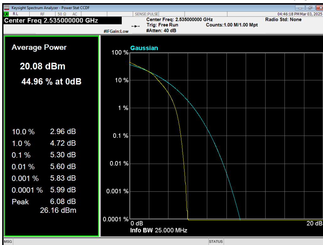
Band7 16QAM BW=15MHz Channel=21100 RB Size=75 Position=#0.png
