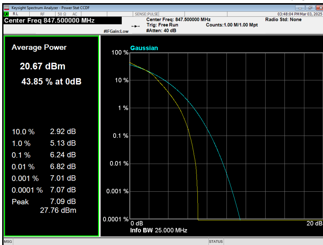
Band5 16QAM BW=3MHz Channel=20635 RB Size=15 Position=#0.png
