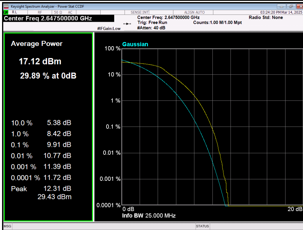
Band41(2535-2655) QPSK BW=15MHz Channel=41165 RB Size=75 Position=#0.png
