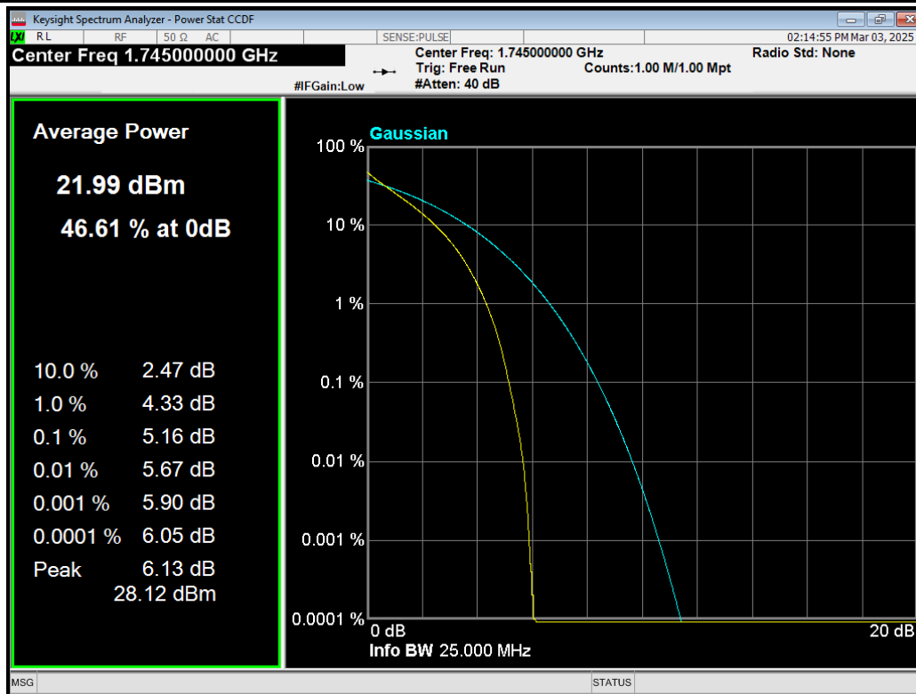
Band4 QPSK BW=20MHz Channel=20300 RB Size=100 Position=#0.png
