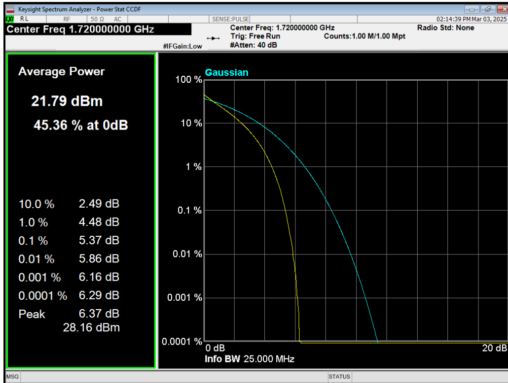
Band4 QPSK BW=20MHz Channel=20050 RB Size=100 Position=#0.png
