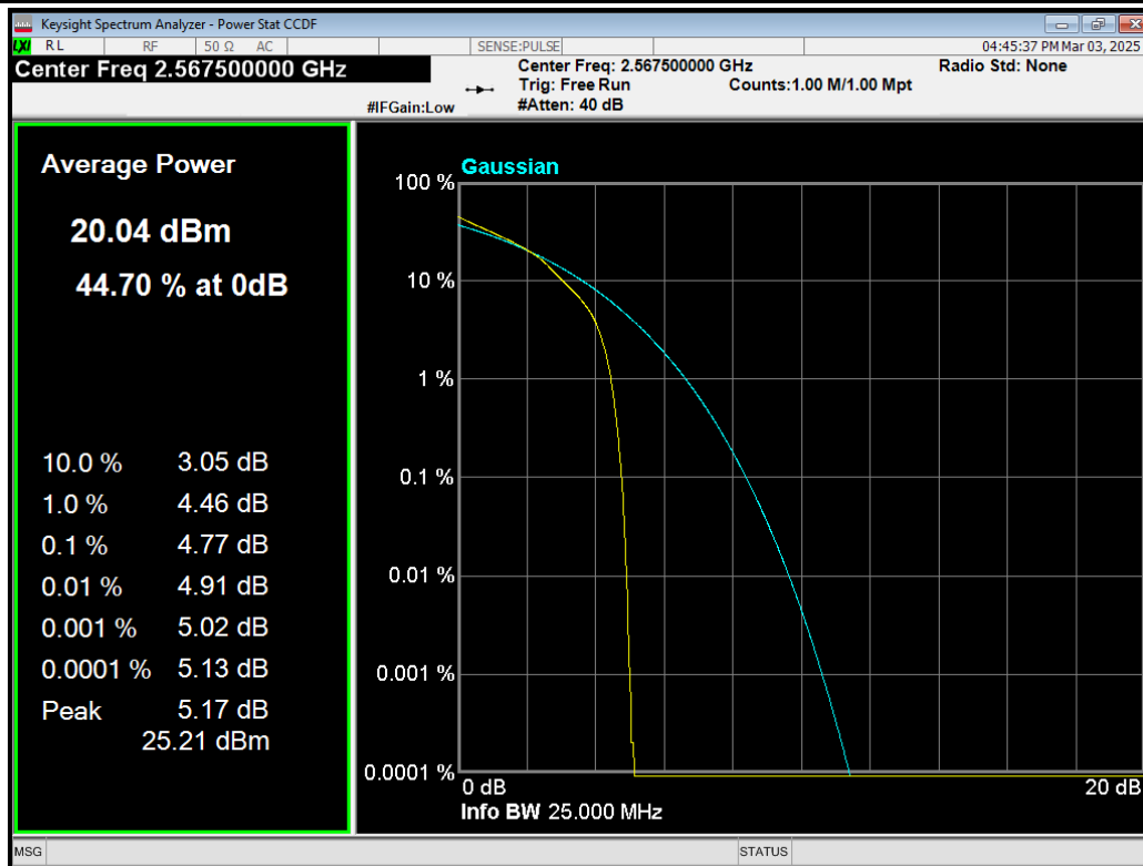
Band7 16QAM BW=5MHz Channel=21425 RB Size=25 Position=#0.png
