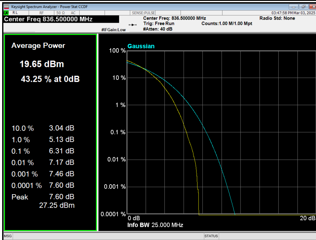
Band5 64QAM BW=3MHz Channel=20525 RB Size=15 Position=#0.png
