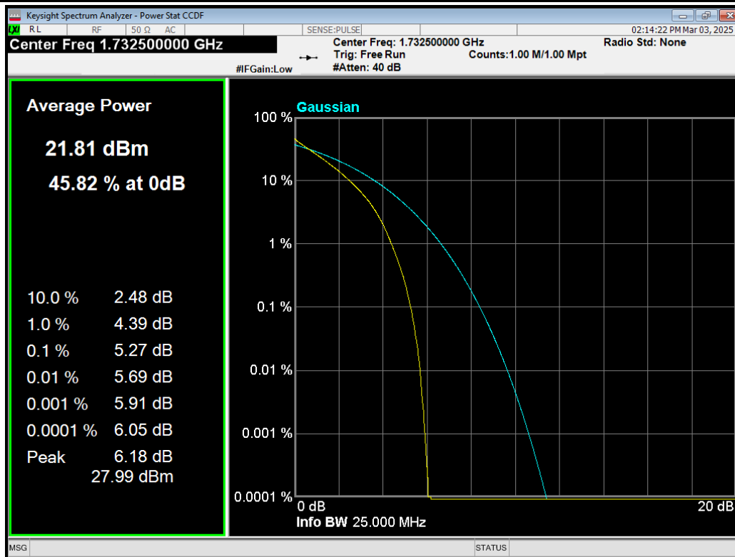
Band4 QPSK BW=15MHz Channel=20175 RB Size=75 Position=#0.png
