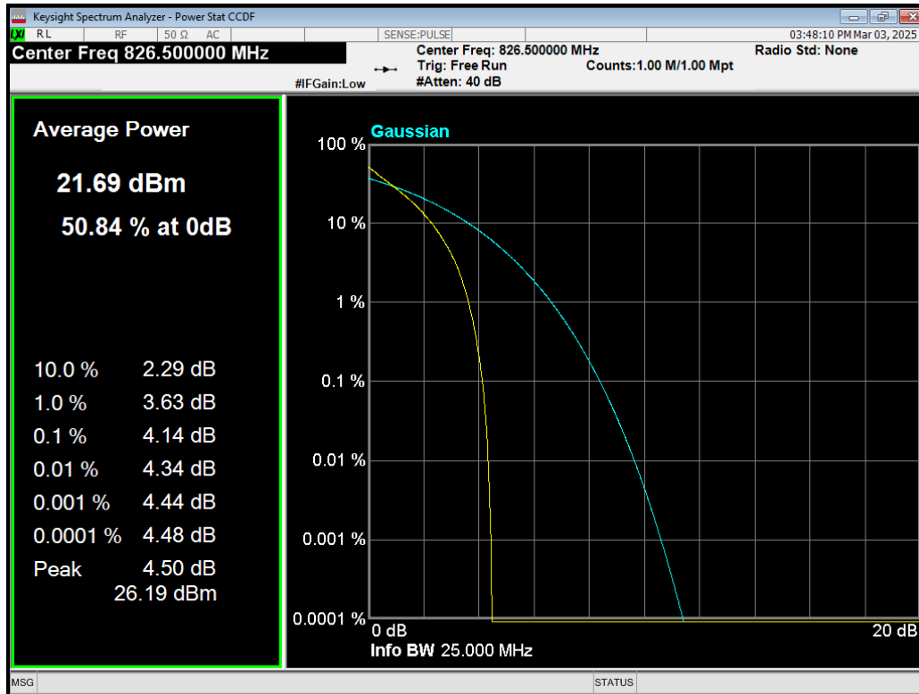
Band5 QPSK BW=5MHz Channel=20425 RB Size=25 Position=#0.png
