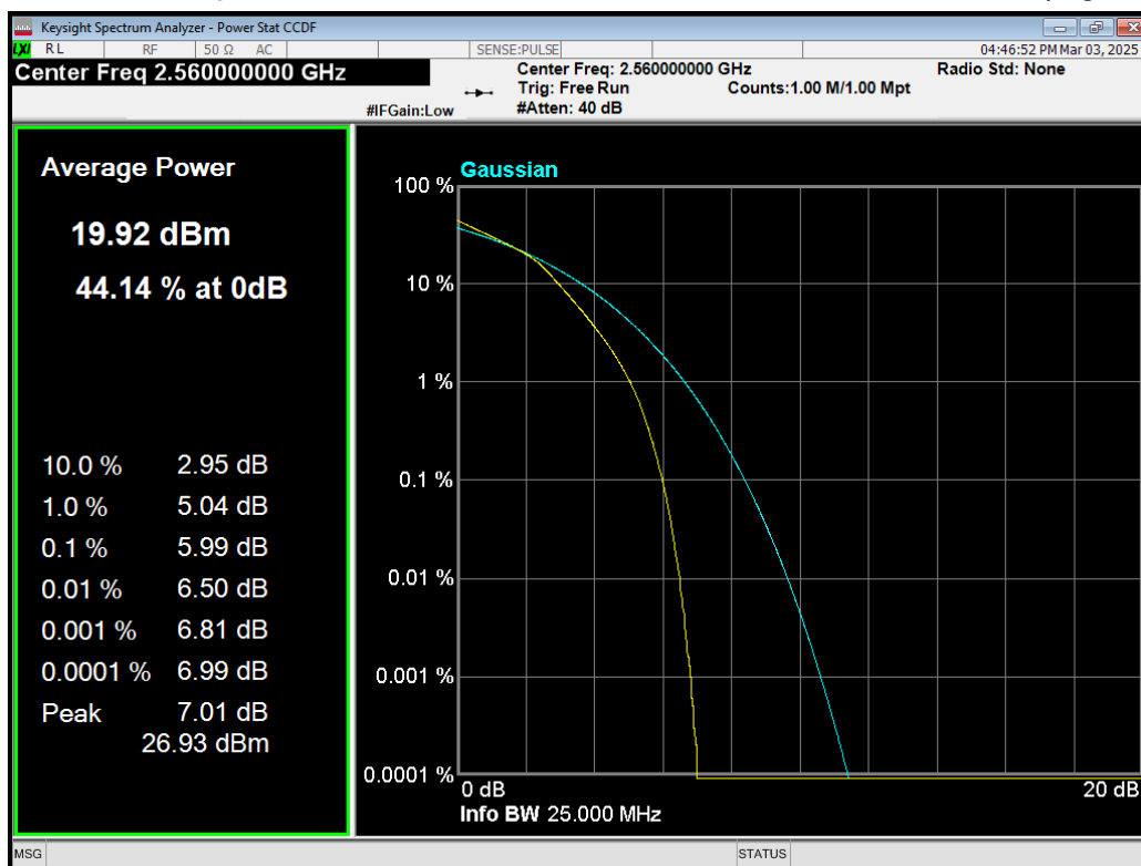
Band7 16QAM BW=20MHz Channel=21350 RB Size=100 Position=#0.png
