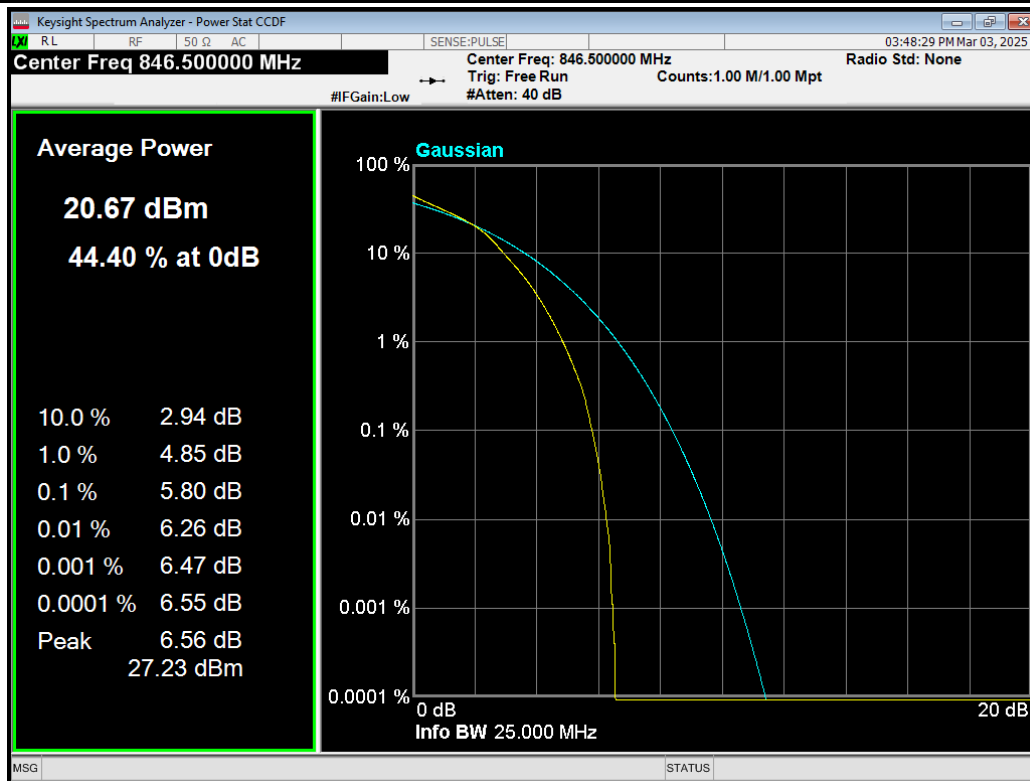
Band5 16QAM BW=5MHz Channel=20625 RB Size=25 Position=#0.png
