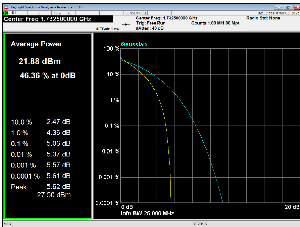
Band4 QPSK BW=10MHz Channel=20175 RB Size=50 Position=#0.png
