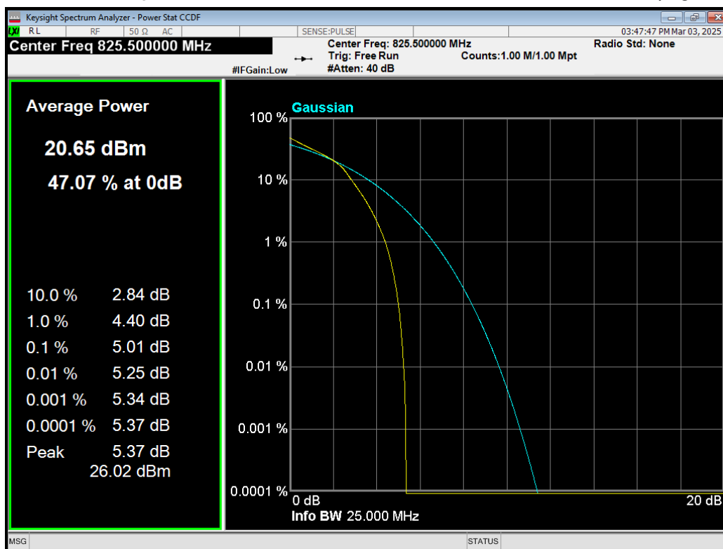
Band5 16QAM BW=3MHz Channel=20415 RB Size=15 Position=#0.png
