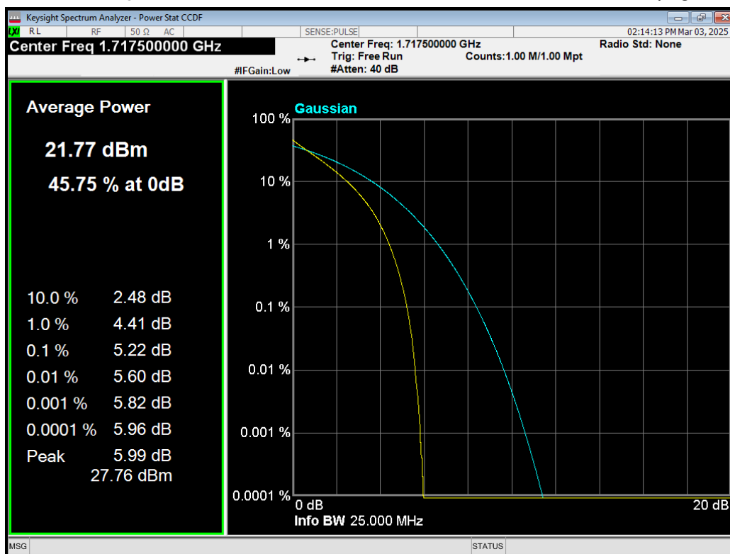
Band4 QPSK BW=15MHz Channel=20025 RB Size=75 Position=#0.png
