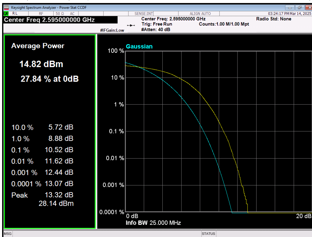
Band41(2535-2655) 64QAM BW=15MHz Channel=40640 RB Size=75 Position=#0.png
