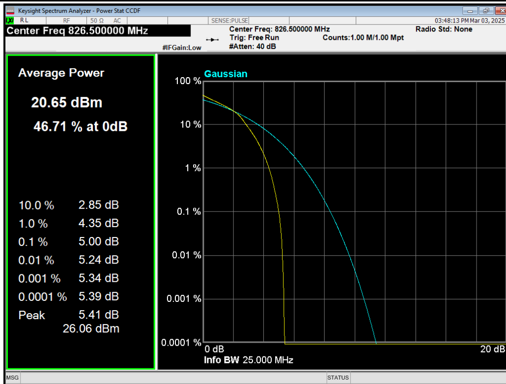
Band5 16QAM BW=5MHz Channel=20425 RB Size=25 Position=#0.png
