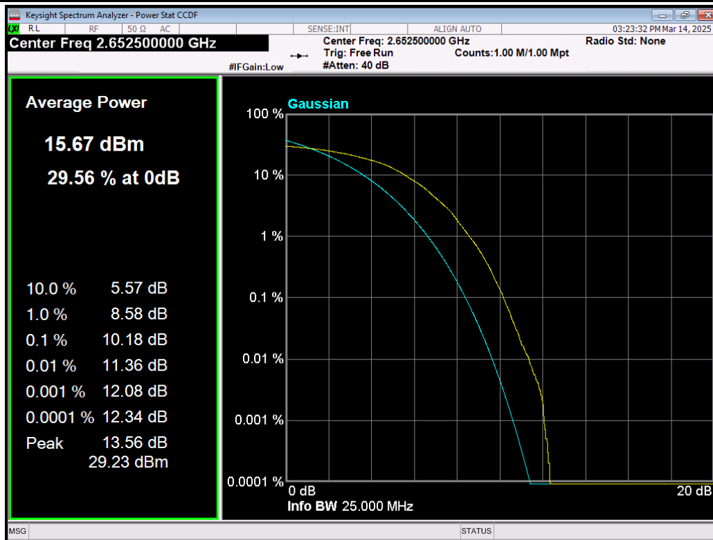
Band41(2535-2655) 64QAM BW=5MHz Channel=41215 RB Size=25 Position=#0.png
