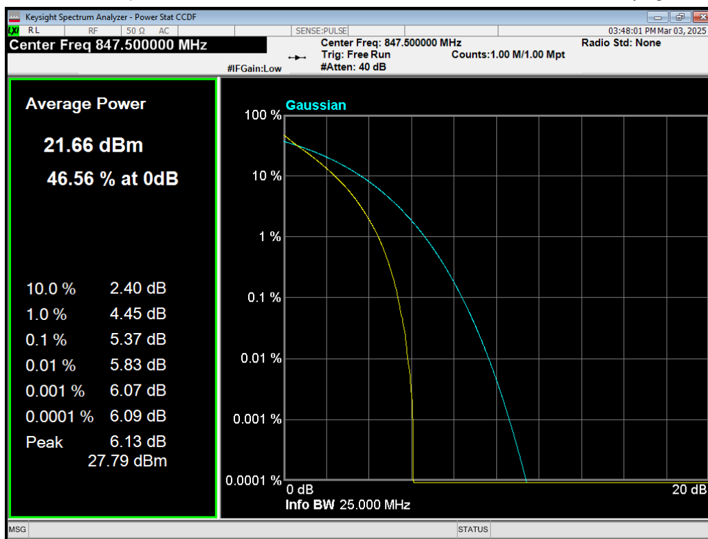
Band5 QPSK BW=3MHz Channel=20635 RB Size=15 Position=#0.png
