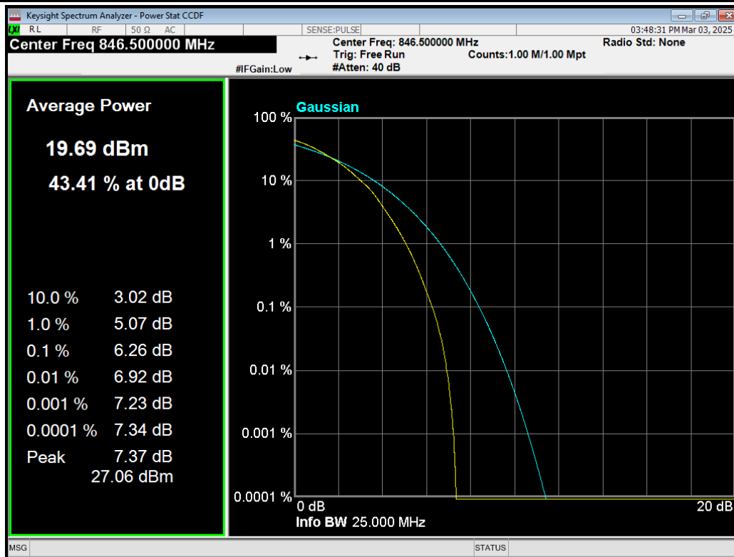
Band5 64QAM BW=5MHz Channel=20625 RB Size=25 Position=#0.png
