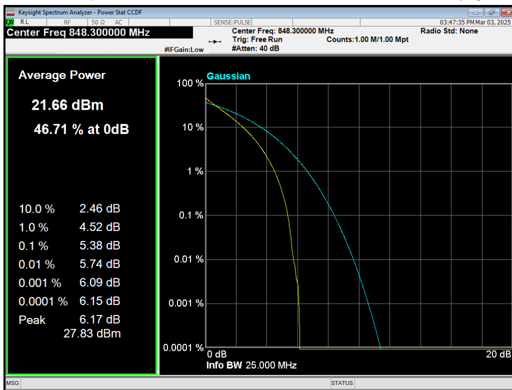
Band5 QPSK BW=1.4MHz Channel=20643 RB Size=6 Position=#0.png
