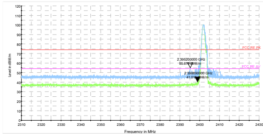
DH5-Channel 0: Peak + Average
