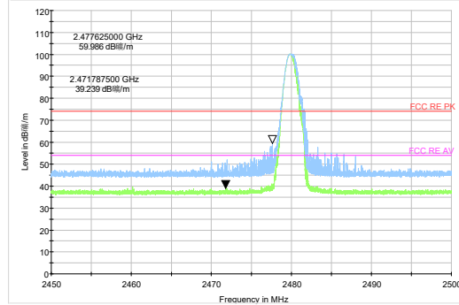
DH5-Channel 78: Peak + Average
