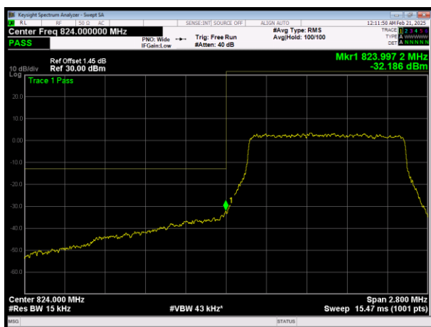
L\LTE Band26 (824-849) QAM16 BW=1.4MHz Channel=26797 RB Size=6 Position=#0
