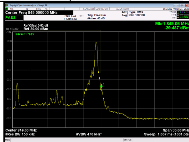
HLTE Band26 (824-849) QAM64 BW=15MHz Channel=26965 RB Size=1 Position=#Max
