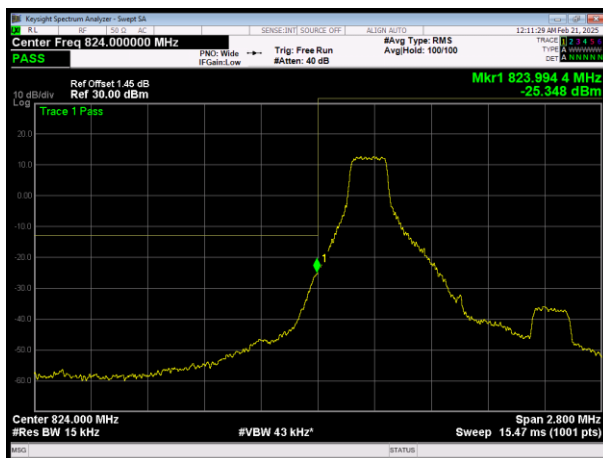
L\LTE Band26 (824-849) QPSK BW=1.4MHz Channel=26797 RB Size=1 Position=#0
