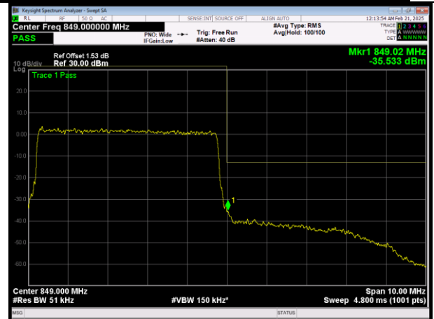
H\LTE Band26 (824-849) QAM16 BW=5MHz Channel=27015 RB Size=25 Position=#0
