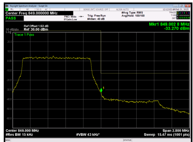
H\LTE Band26 (824-849) QPSK BW=1.4MHz Channel=27033 RB Size=6 Position=#0
