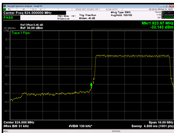
L\LTE Band26 (824-849) QAM64 BW=5MHz Channel=26815 RB Size=25 Position=#0
