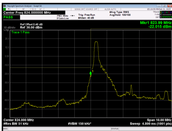
L\LTE Band26 (824-849) QAM64 BW=5MHz Channel=26815 RB Size=1 Position=#0
