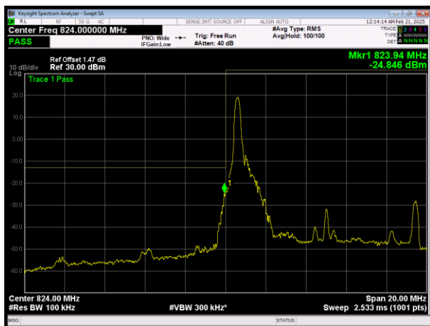
L\LTE Band26 (824-849) QAM16 BW=10MHz Channel=26840 RB Size=1 Position=#0
