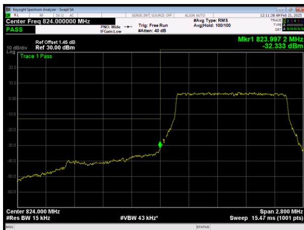
L\LTE Band26 (824-849) QPSK BW=1.4MHz Channel=26797 RB Size=6 Position=#0
