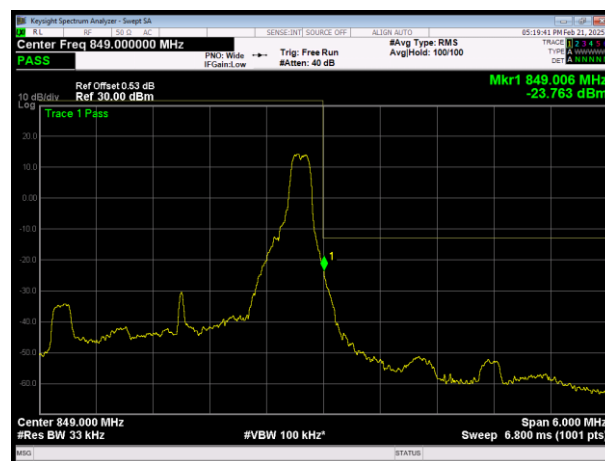
HLTE Band26 (824-849) QAM64 BW=3MHz Channel=27025 RB Size=1 Position=#Max
