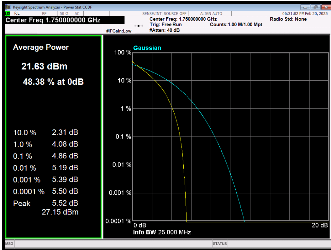
LTE Band4 QPSK BW=10MHz Channel=20350 RB Size=50 Position=#0
