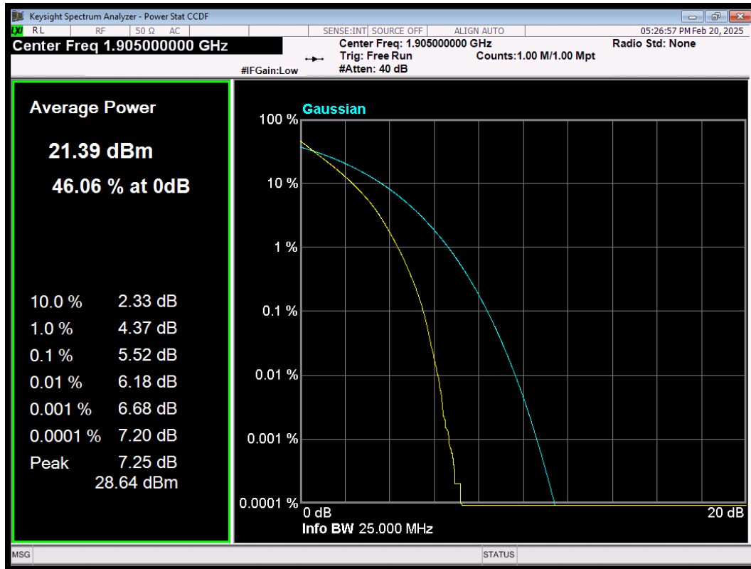
LTE Band2 QPSK BW=10MHz Channel=19150 RB Size=50 Position=#0
