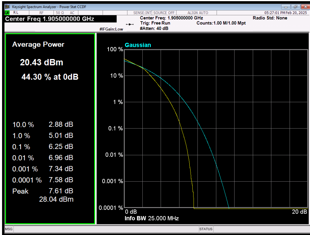
LTE Band2 QAM16 BW=10MHz Channel=19150 RB Size=50 Position=#0
