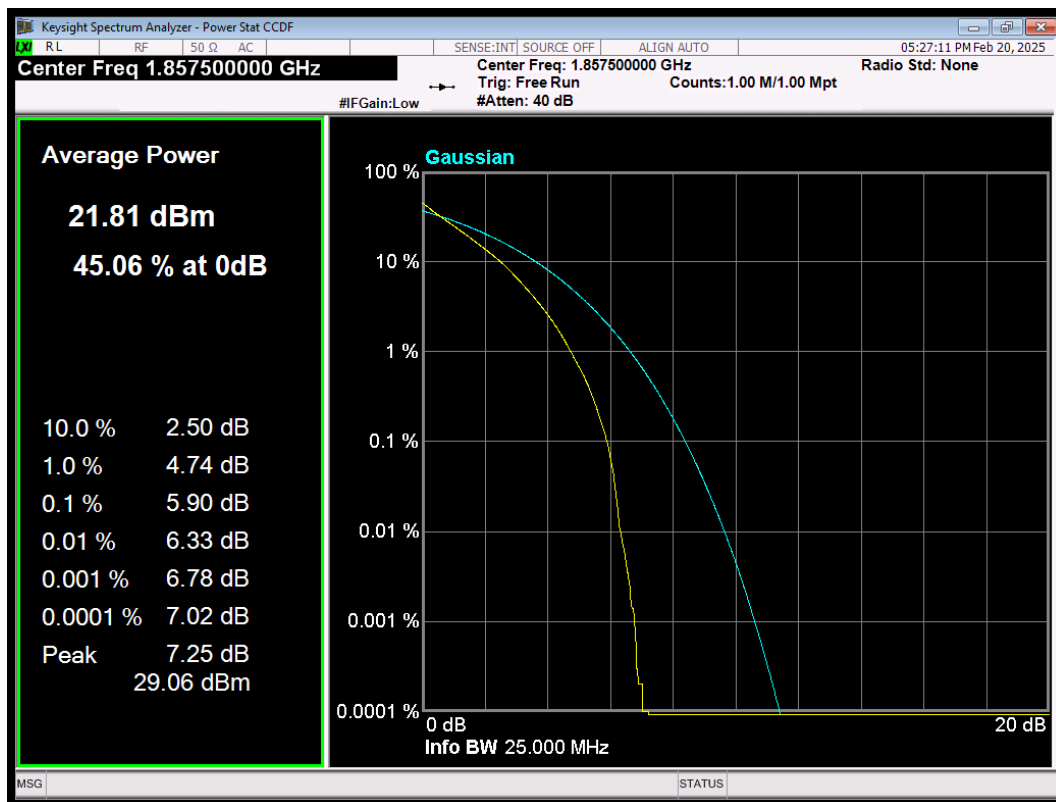
LTE Band2 QPSK BW=15MHz Channel=18675 RB Size=75 Position=#0
