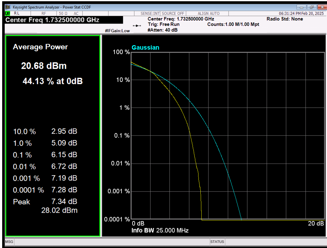
LTE Band4 QAM16 BW=15MHz Channel=20175 RB Size=75 Position=#0
