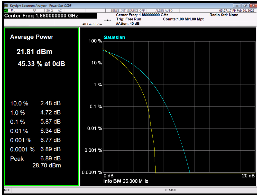
LTE Band2 QPSK BW=15MHz Channel=18900 RB Size=75 Position=#0
