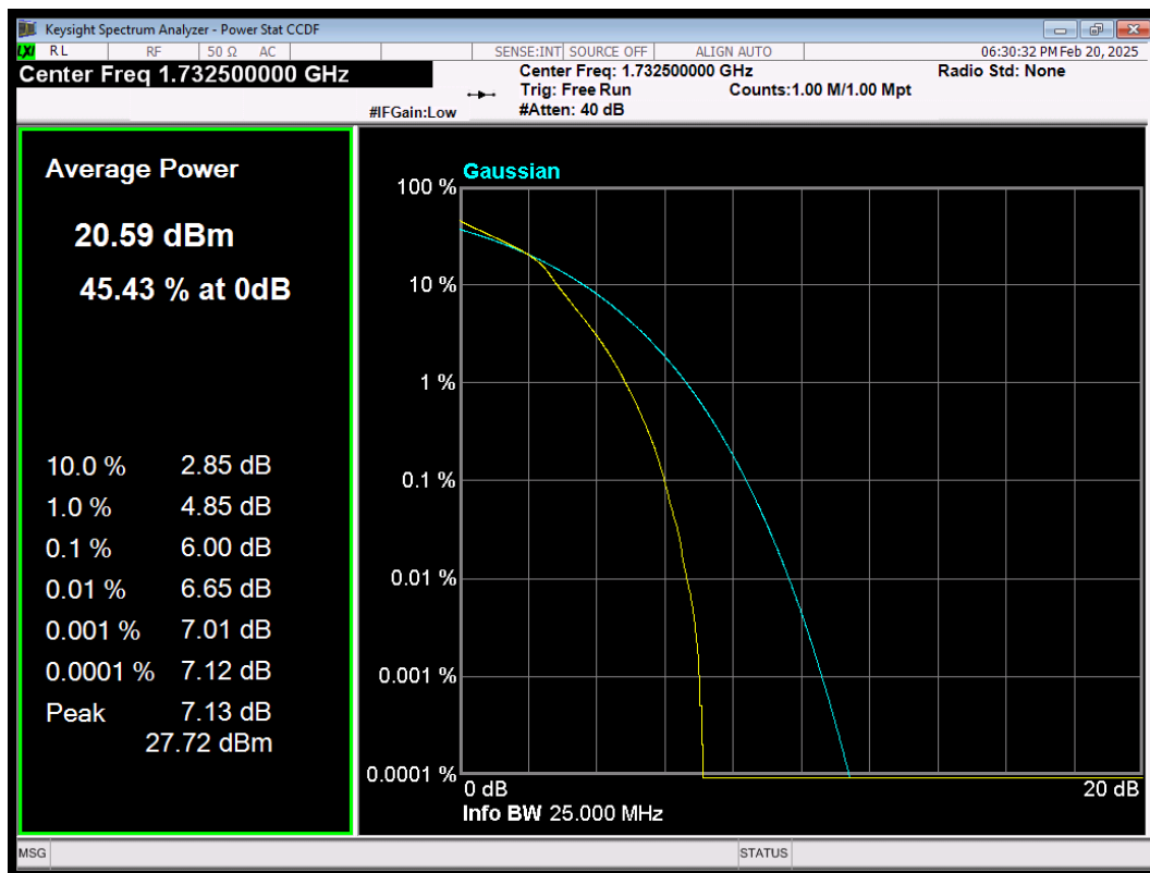
LTE Band4 QAM16 BW=5MHz Channel=20175 RB Size=25 Position=#0
