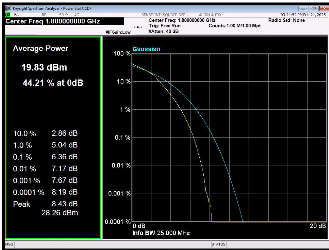
LTE Band2 QAM64 BW=20MHz Channel=18900 RB Size=100 Position=#0
