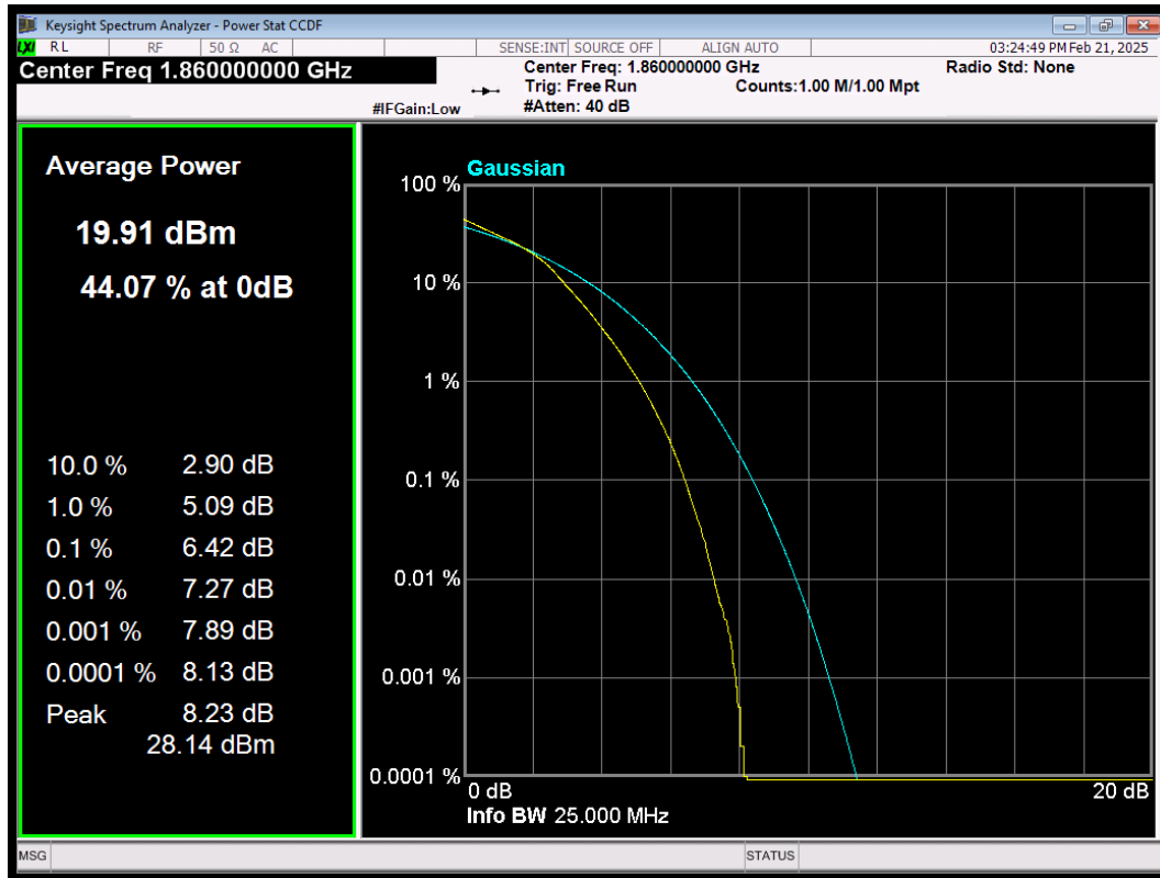
LTE Band2 QAM64 BW=20MHz Channel=18700 RB Size=100 Position=#0
