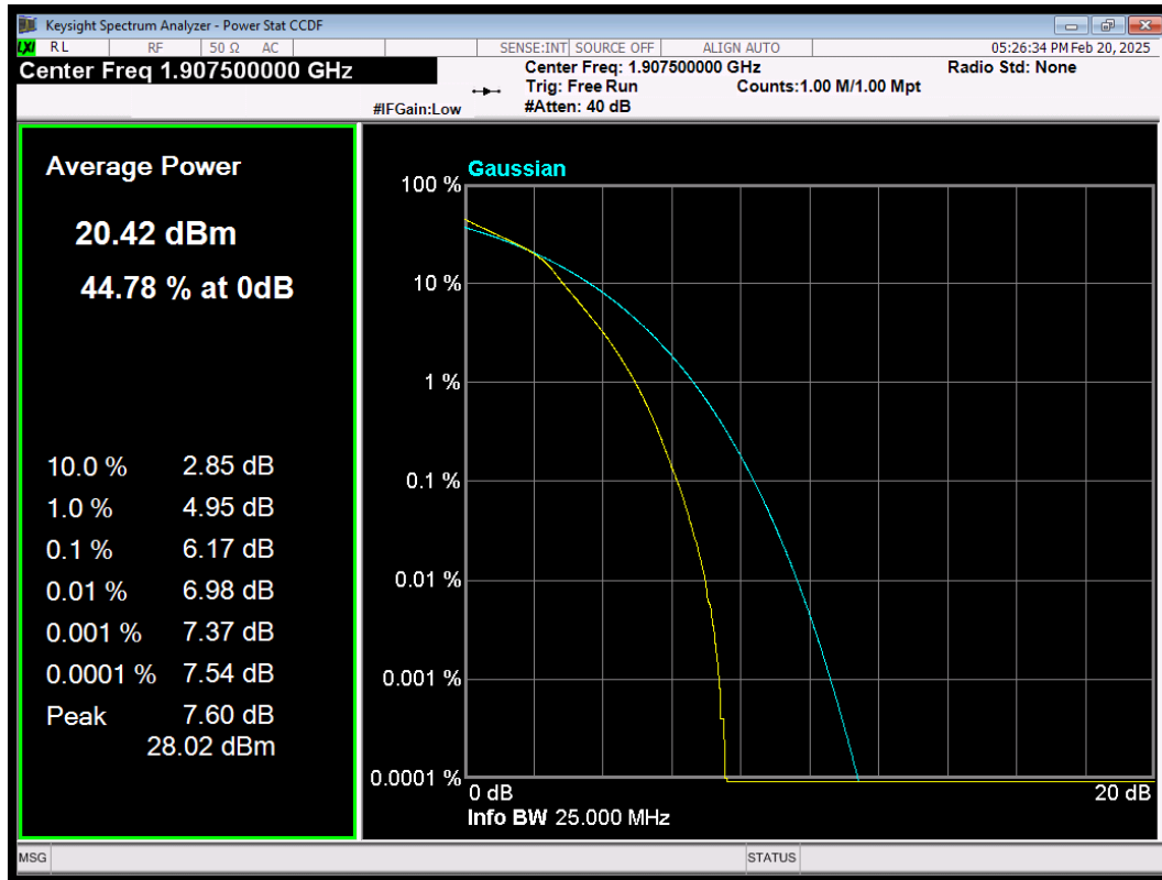
LTE Band2 QAM16 BW=5MHz Channel=19175 RB Size=25 Position=#0
