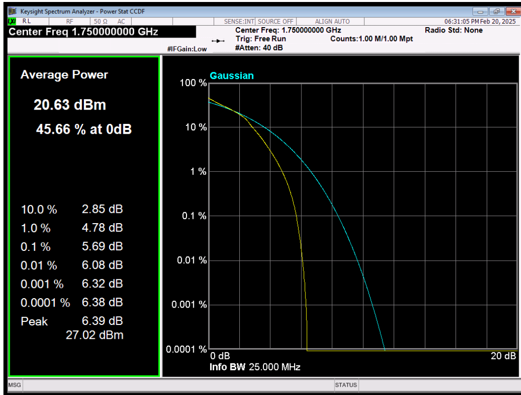
LTE Band4 QAM16 BW=10MHz Channel=20350 RB Size=50 Position=#0
