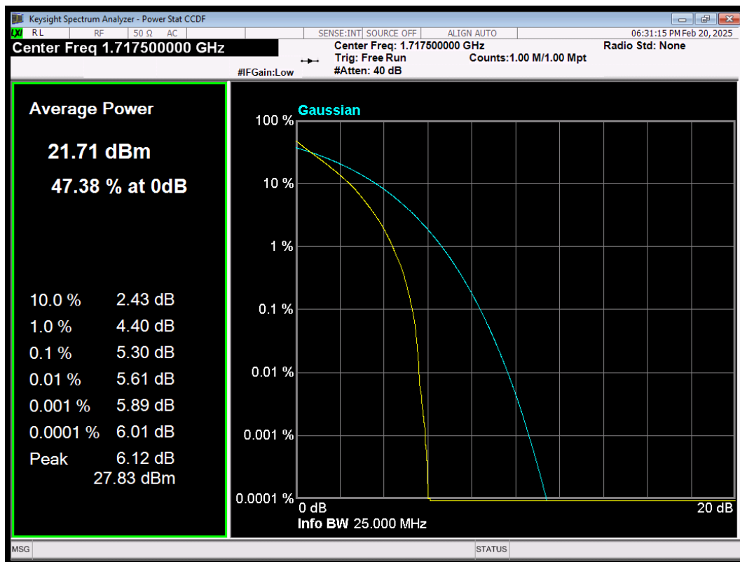
LTE Band4 QPSK BW=15MHz Channel=20025 RB Size=75 Position=#0
