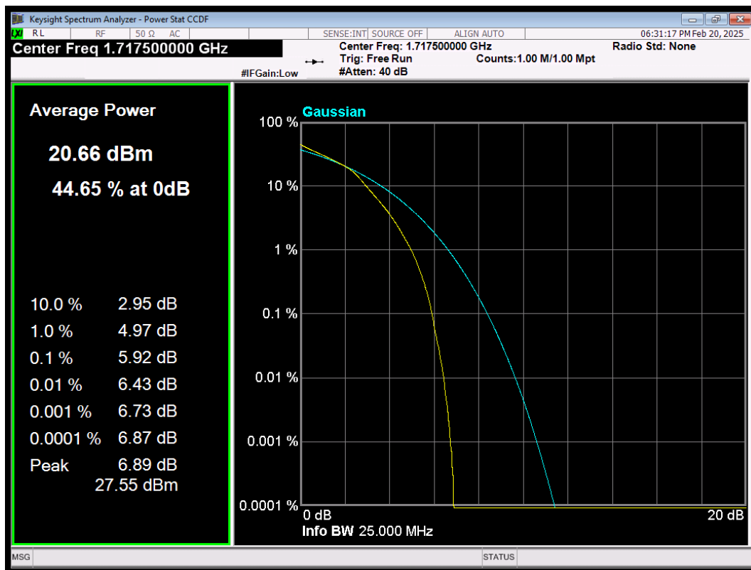
LTE Band4 QAM16 BW=15MHz Channel=20025 RB Size=75 Position=#0
