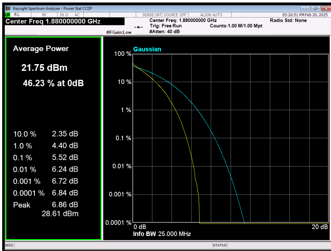
LTE Band2 QPSK BW=10MHz Channel=18900 RB Size=50 Position=#0
