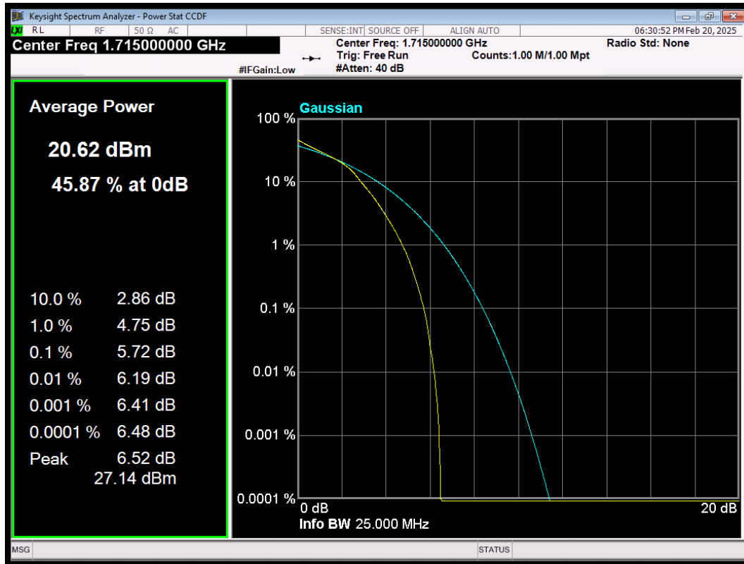
LTE Band4 QAM16 BW=10MHz Channel=20000 RB Size=50 Position=#0
