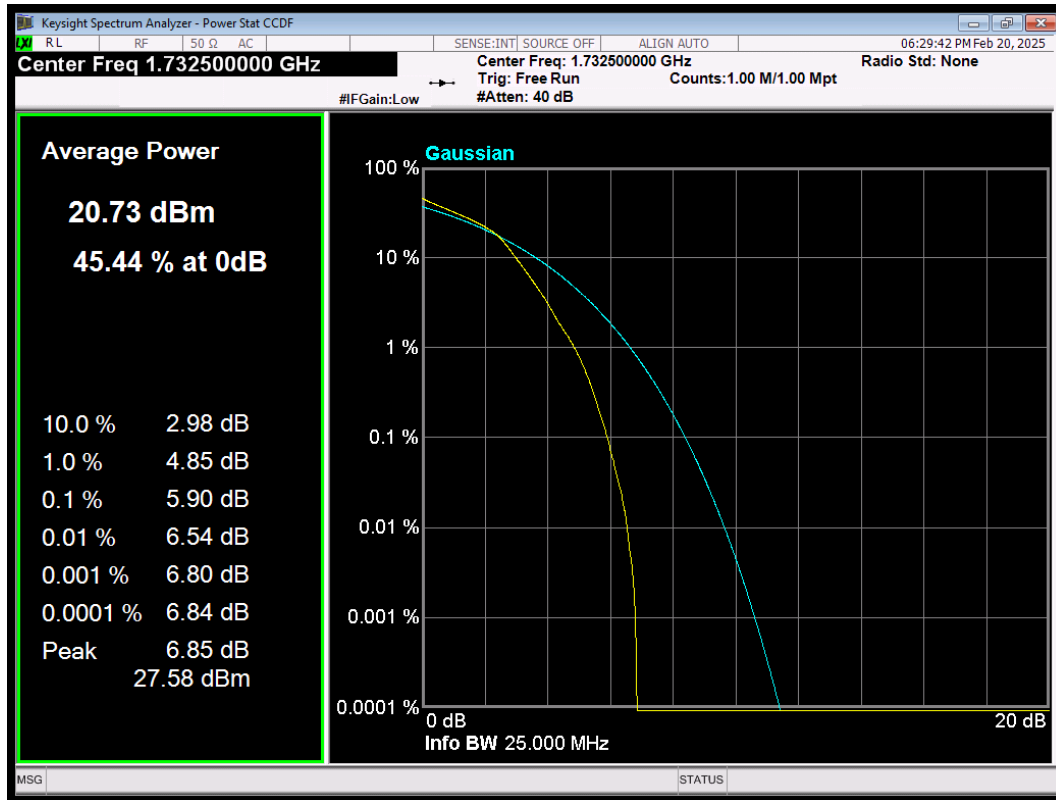
LTE Band4 QAM16 BW=1.4MHz Channel=20175 RB Size=6 Position=#0
