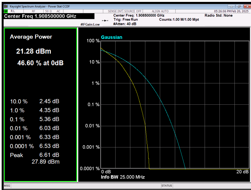
LTE Band2 QPSK BW=3MHz Channel=19185 RB Size=15 Position=#0
