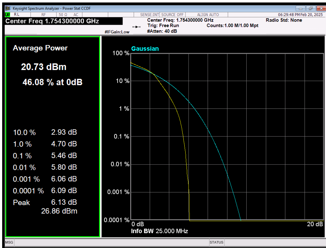
LTE Band4 QAM16 BW=1.4MHz Channel=20393 RB Size=6 Position=#0
