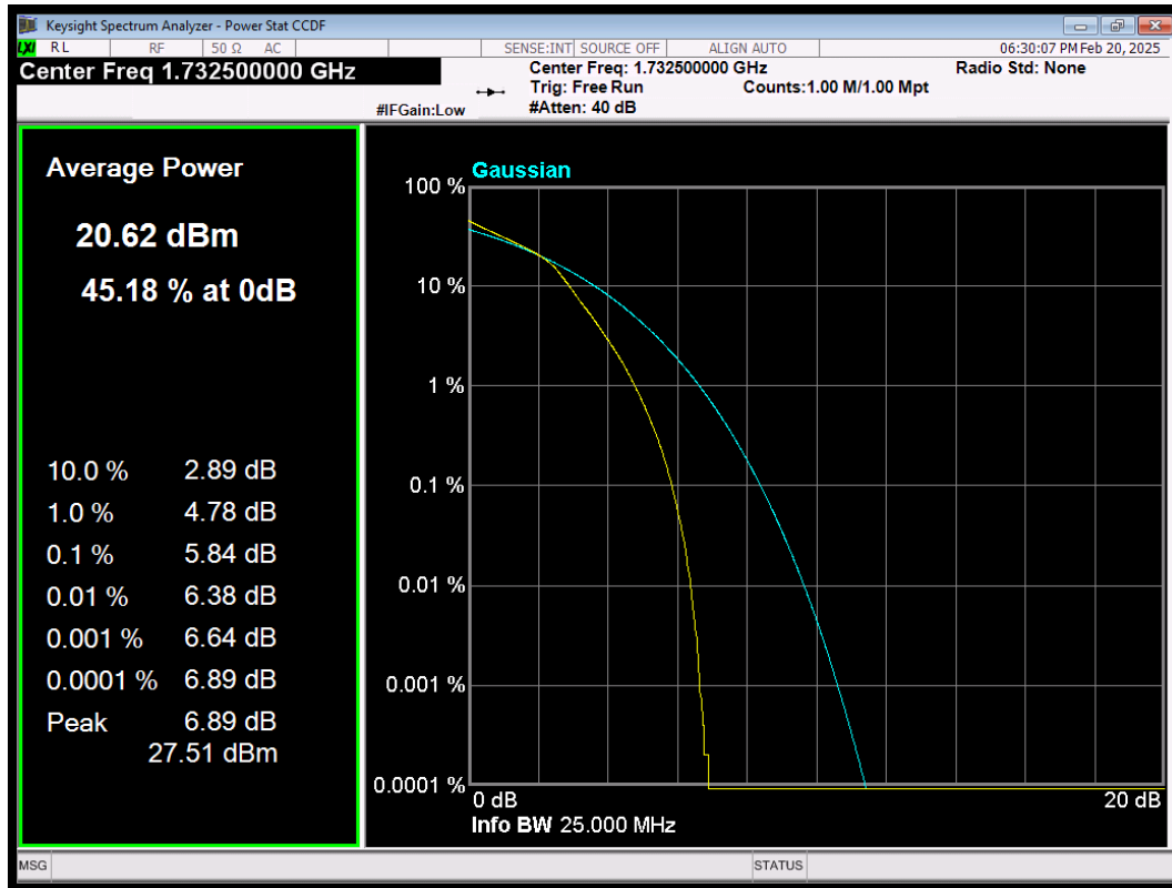
LTE Band4 QAM16 BW=3MHz Channel=20175 RB Size=15 Position=#0
