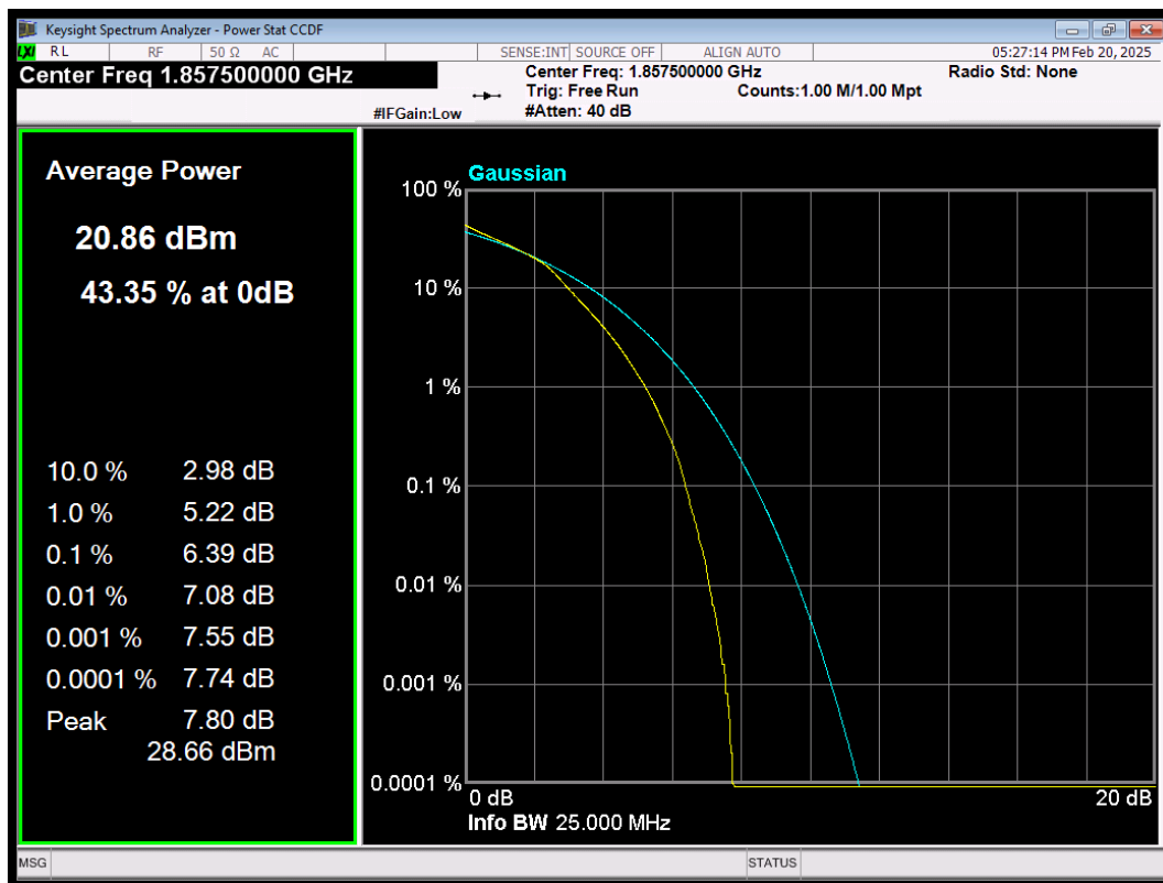
LTE Band2 QAM16 BW=15MHz Channel=18675 RB Size=75 Position=#0
