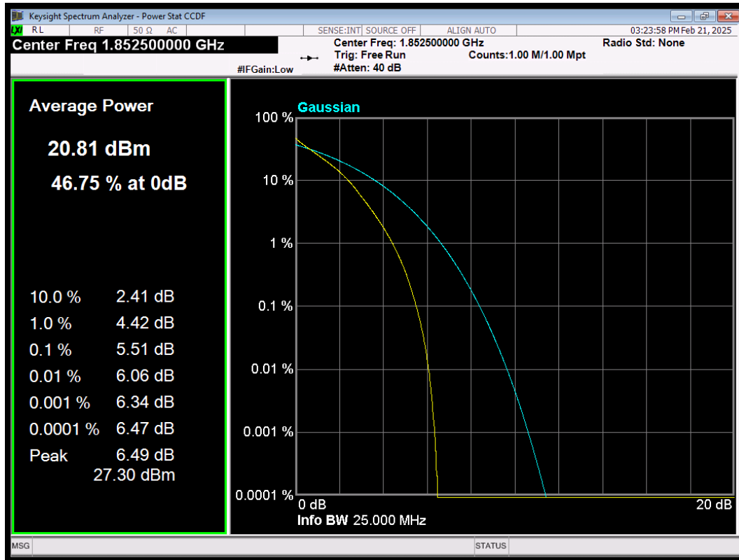
LTE Band2 QAM64 BW=5MHz Channel=18625 RB Size=25 Position=#0
