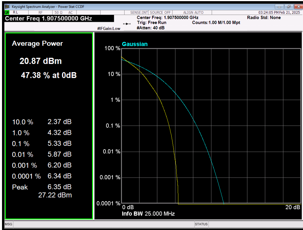
LTE Band2 QAM64 BW=5MHz Channel=19175 RB Size=25 Position=#0
