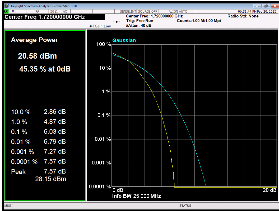
LTE Band4 QAM16 BW=20MHz Channel=20050 RB Size=100 Position=#0
