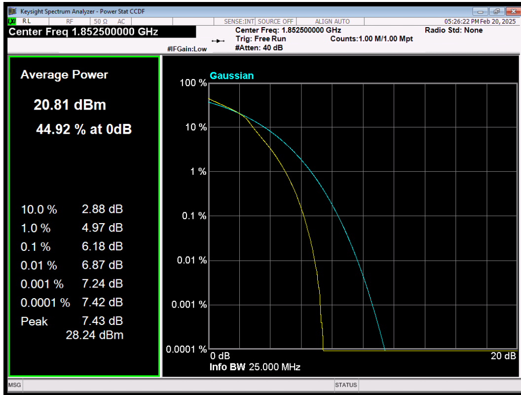
LTE Band2 QAM16 BW=5MHz Channel=18625 RB Size=25 Position=#0
