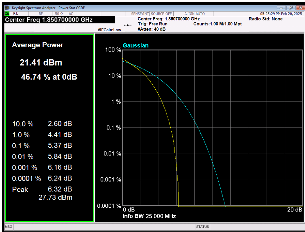
LTE Band2 QPSK BW=1.4MHz Channel=18607 RB Size=6 Position=#0
