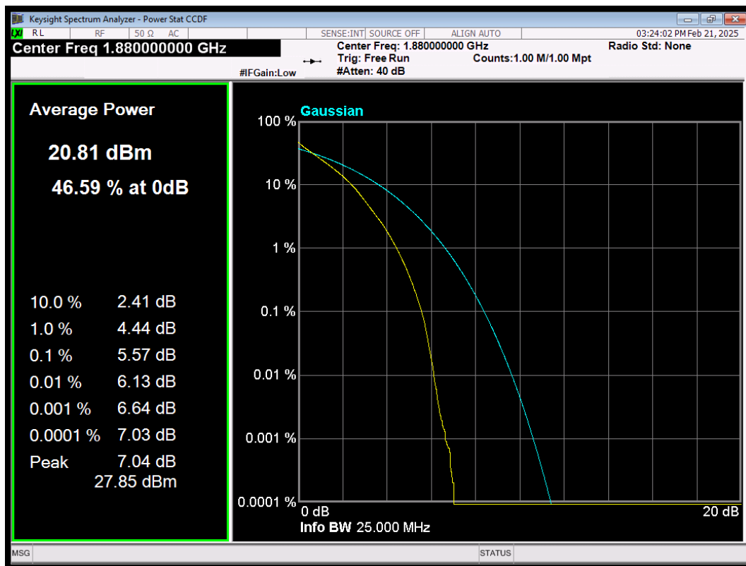
LTE Band2 QAM64 BW=5MHz Channel=18900 RB Size=25 Position=#0
