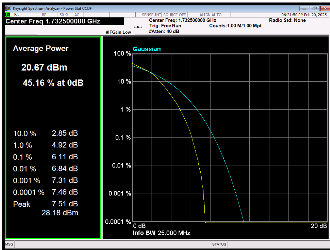
LTE Band4 QAM16 BW=20MHz Channel=20175 RB Size=100 Position=#0
