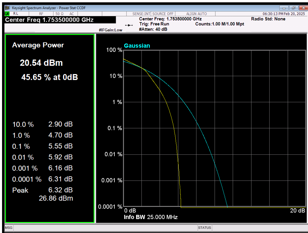
LTE Band4 QAM16 BW=3MHz Channel=20385 RB Size=15 Position=#0
