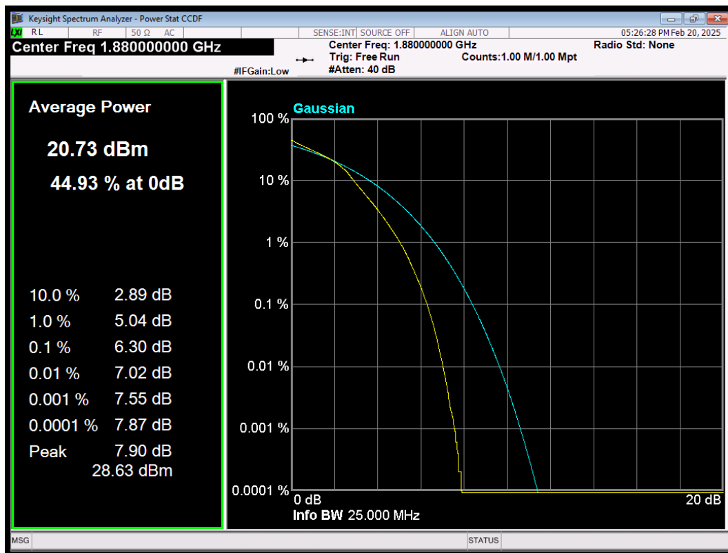
LTE Band2 QAM16 BW=5MHz Channel=18900 RB Size=25 Position=#0
