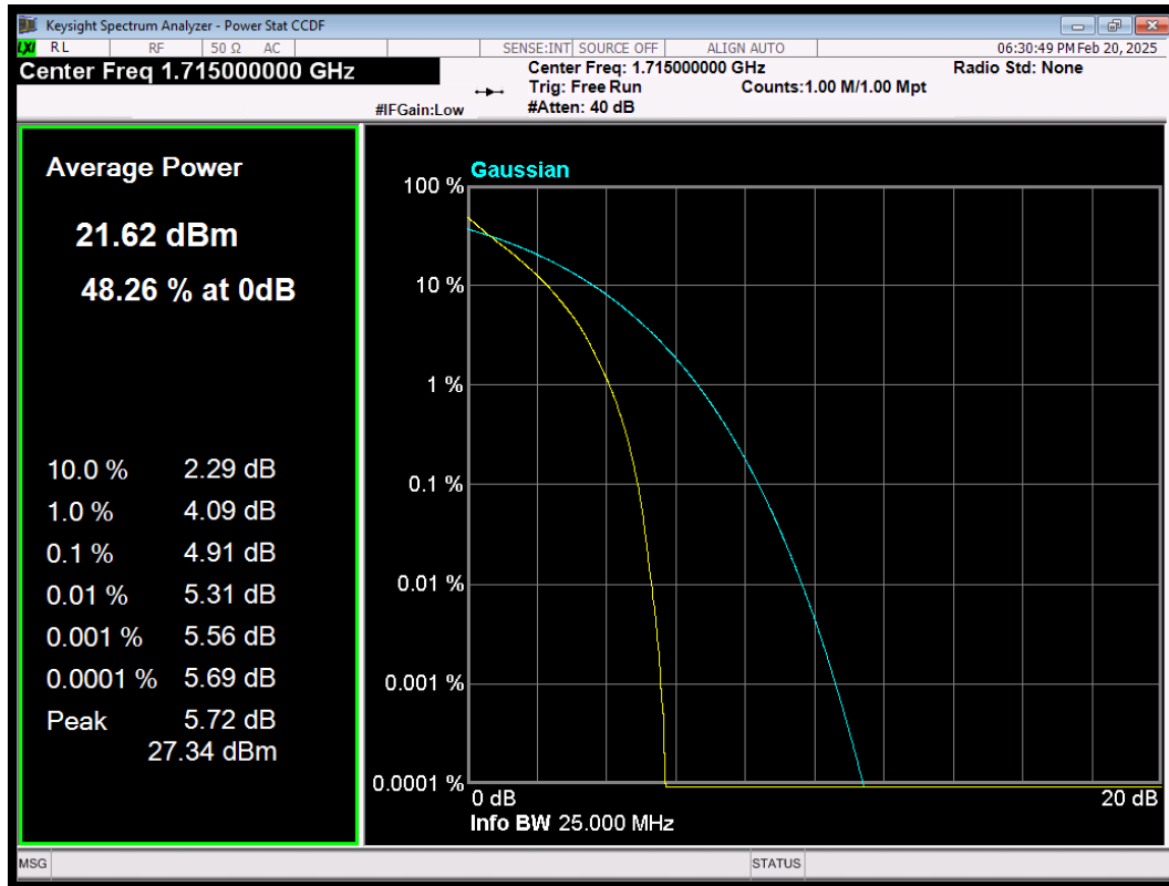
LTE Band4 QPSK BW=10MHz Channel=20000 RB Size=50 Position=#0
