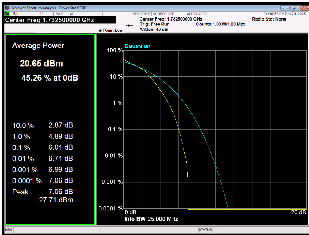
LTE Band4 QAM16 BW=10MHz Channel=20175 RB Size=50 Position=#0
