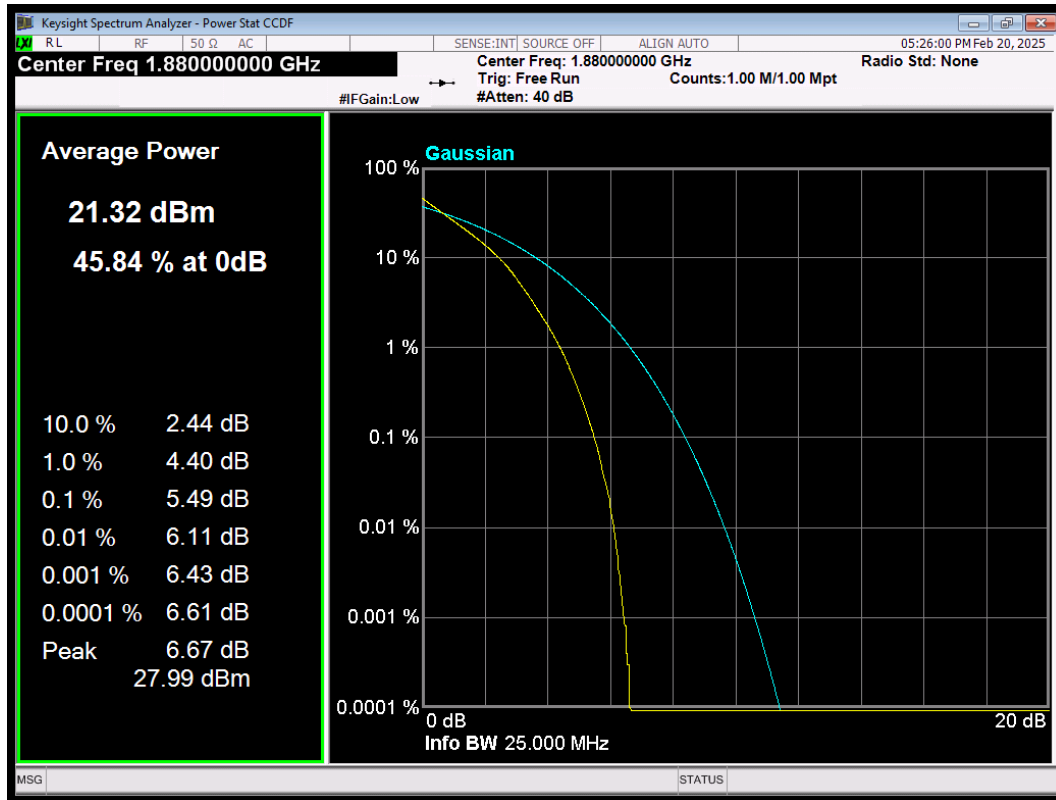
LTE Band2 QPSK BW=3MHz Channel=18900 RB Size=15 Position=#0
