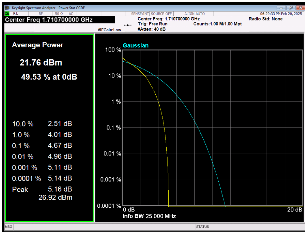
LTE Band4 QPSK BW=1.4MHz Channel=19957 RB Size=6 Position=#0
