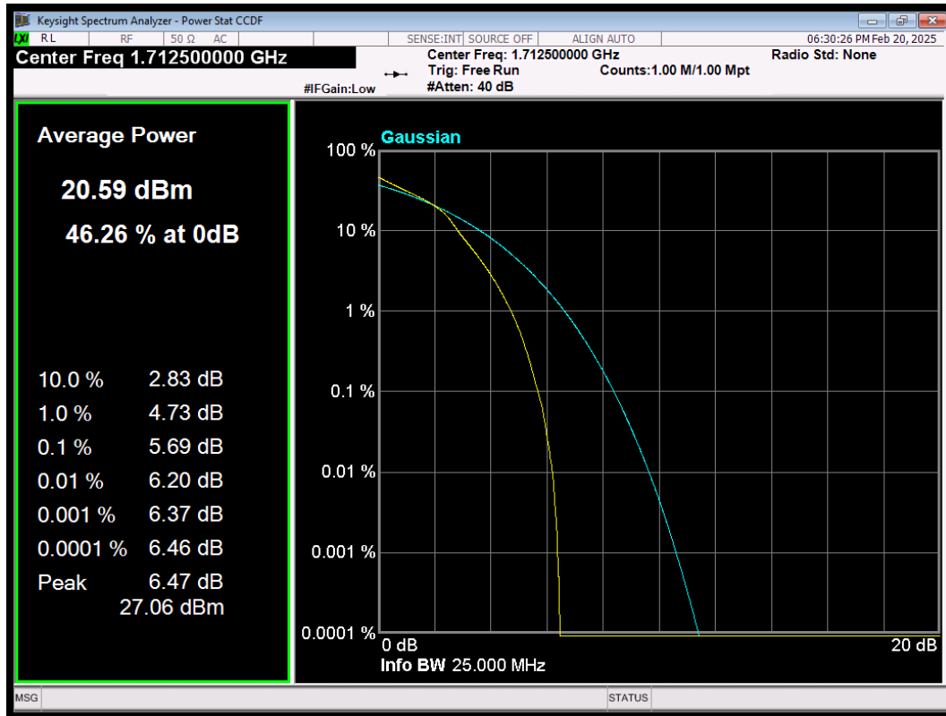
LTE Band4 QAM16 BW=5MHz Channel=19975 RB Size=25 Position=#0
