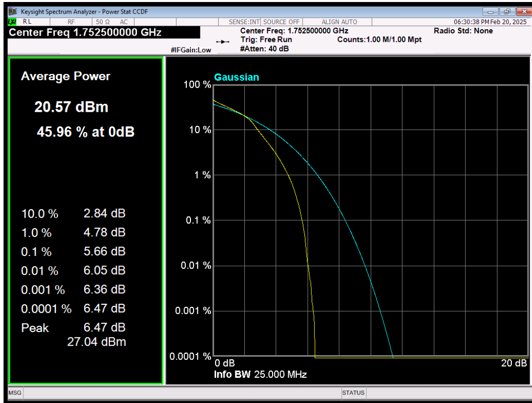
LTE Band4 QAM16 BW=5MHz Channel=20375 RB Size=25 Position=#0
