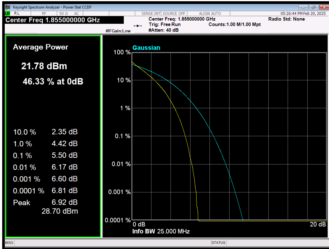
LTE Band2 QPSK BW=10MHz Channel=18650 RB Size=50 Position=#0
