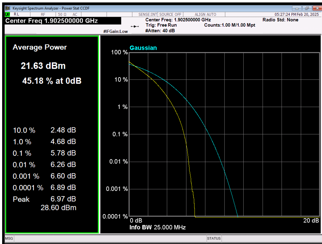
LTE Band2 QPSK BW=15MHz Channel=19125 RB Size=75 Position=#0
