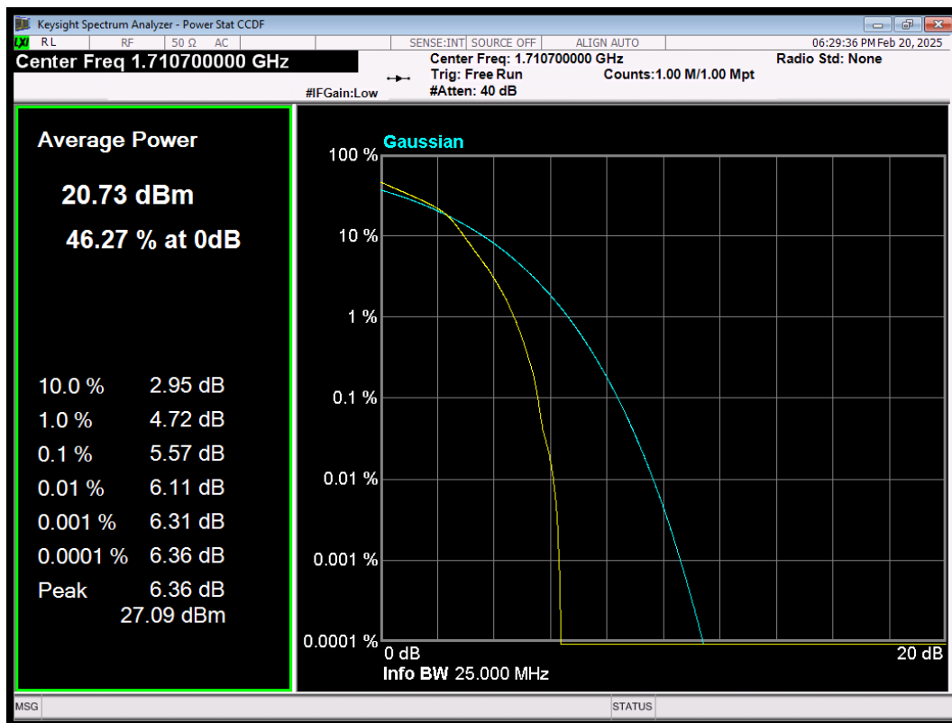
LTE Band4 QAM16 BW=1.4MHz Channel=19957 RB Size=6 Position=#0
