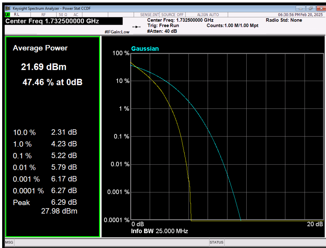
LTE Band4 QPSK BW=10MHz Channel=20175 RB Size=50 Position=#0
