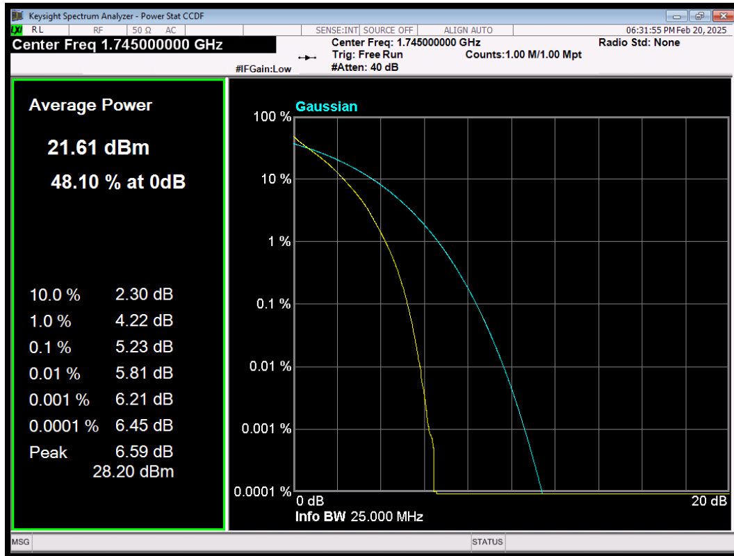
LTE Band4 QPSK BW=20MHz Channel=20300 RB Size=100 Position=#0
