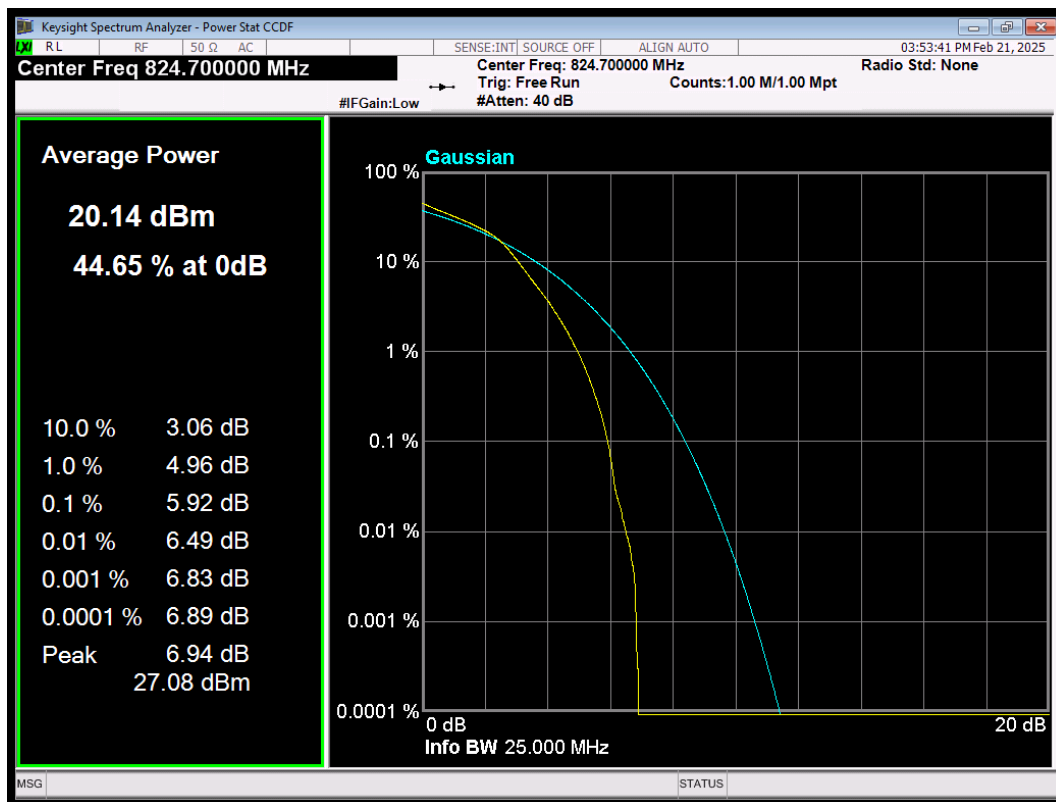
LTE Band5 QAM64 BW=1.4MHz Channel=20407 RB Size=6 Position=#0
