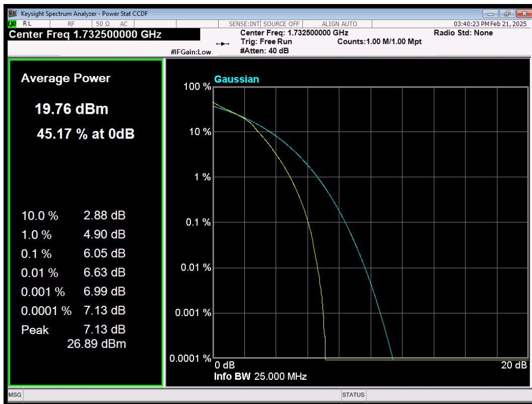
LTE Band4 QAM64 BW=10MHz Channel=20175 RB Size=50 Position=#0
