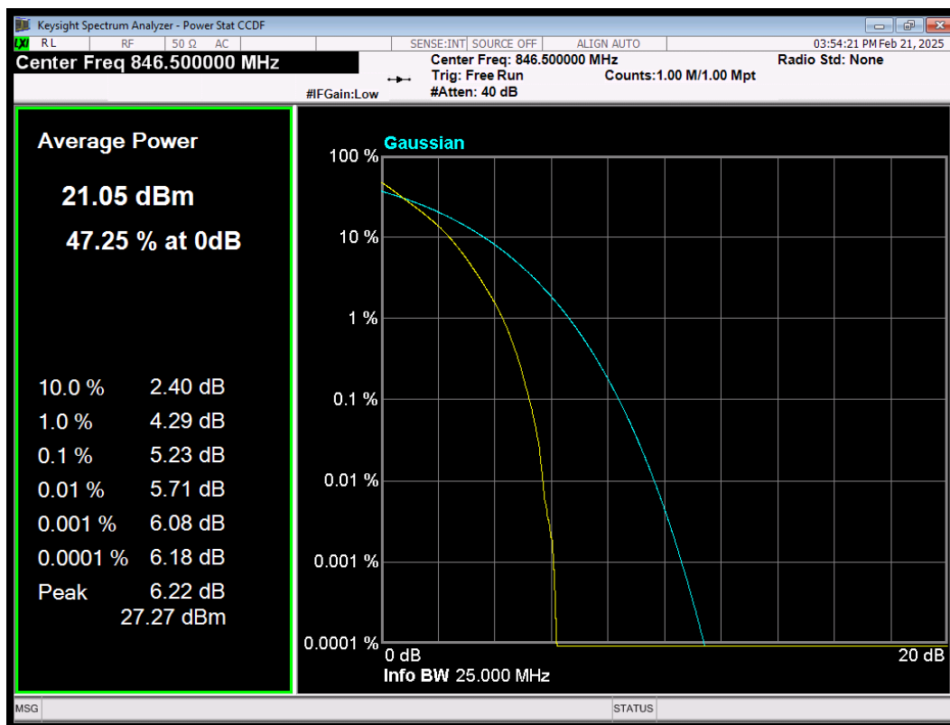
LTE Band5 QAM64 BW=5MHz Channel=20625 RB Size=25 Position=#0
