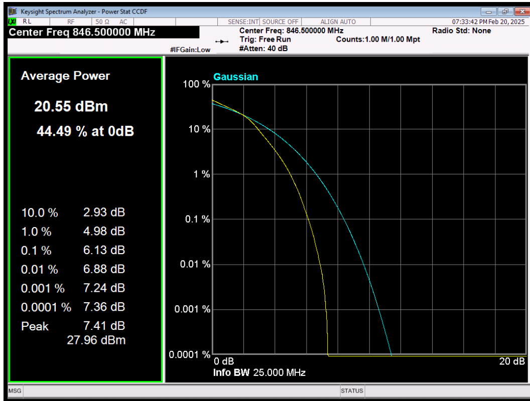
LTE Band5 QAM16 BW=5MHz Channel=20625 RB Size=25 Position=#0
