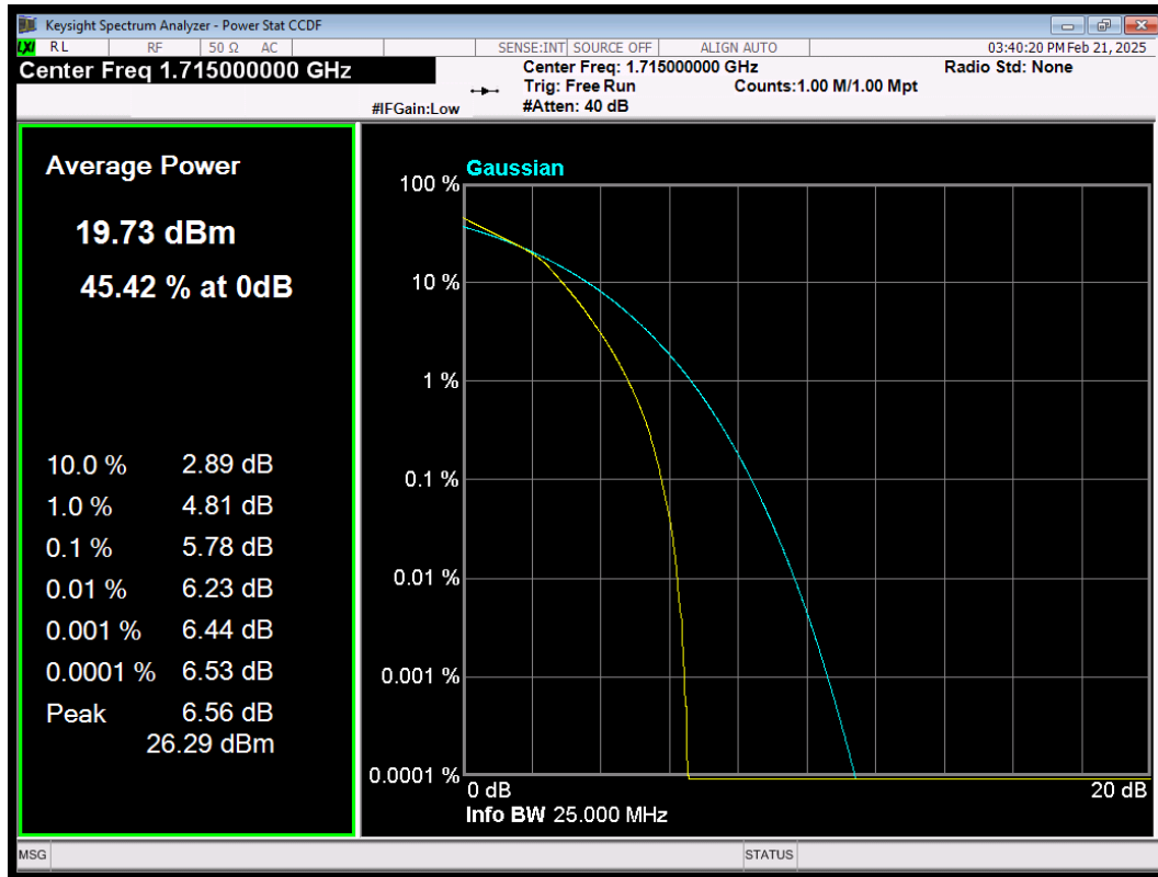
LTE Band4 QAM64 BW=10MHz Channel=20000 RB Size=50 Position=#0
