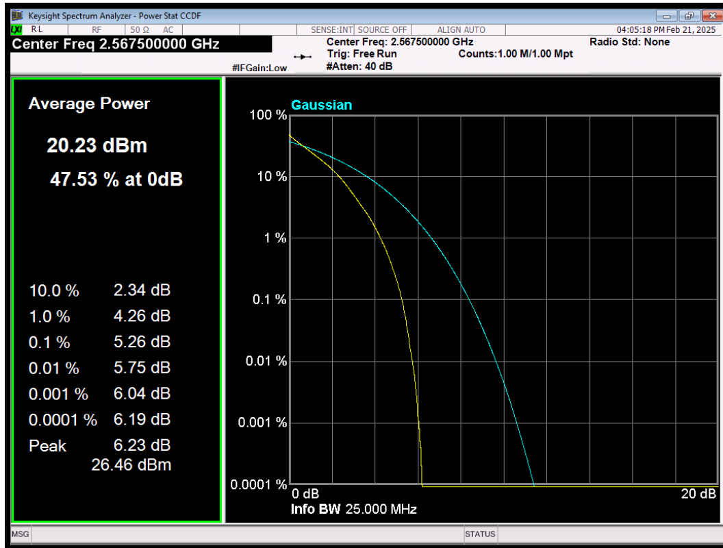
LTE Band7 QAM64 BW=5MHz Channel=21425 RB Size=25 Position=#0
