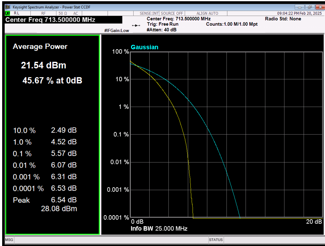
LTE Band12 QPSK BW=5MHz Channel=23155 RB Size=25 Position=#0
