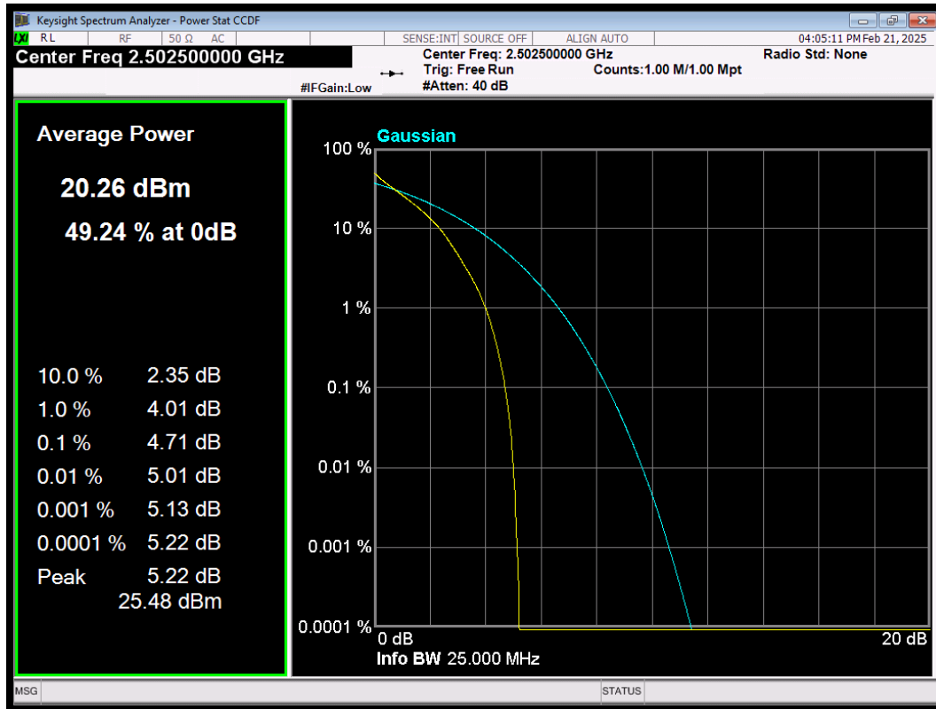
LTE Band7 QAM64 BW=5MHz Channel=20775 RB Size=25 Position=#0
