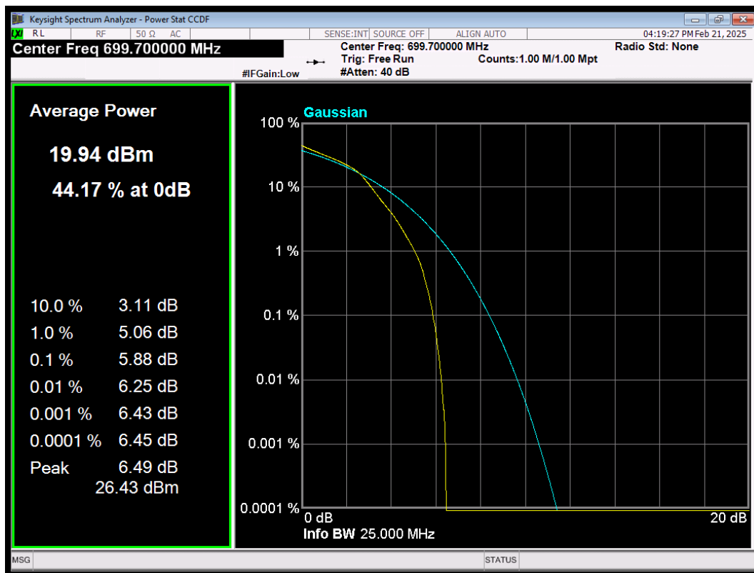
LTE Band12 QAM64 BW=1.4MHz Channel=23017 RB Size=6 Position=#0
