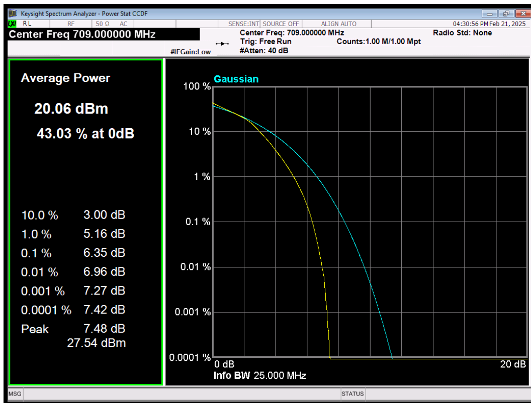
LTE Band17 QAM64 BW=10MHz Channel=23780 RB Size=50 Position=#0
