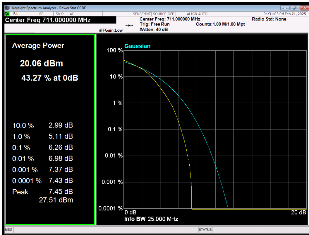
LTE Band17 QAM64 BW=10MHz Channel=23800 RB Size=50 Position=#0
