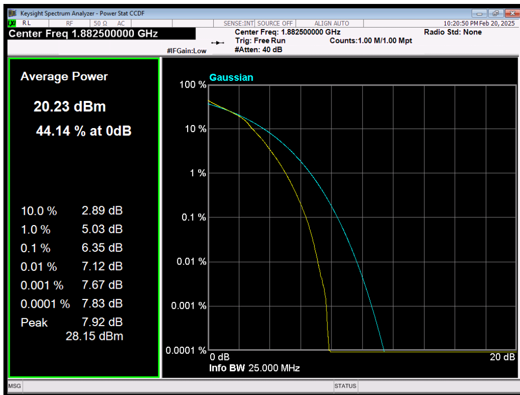
LTE Band25 QAM16 BW=10MHz Channel=26365 RB Size=50 Position=#0
