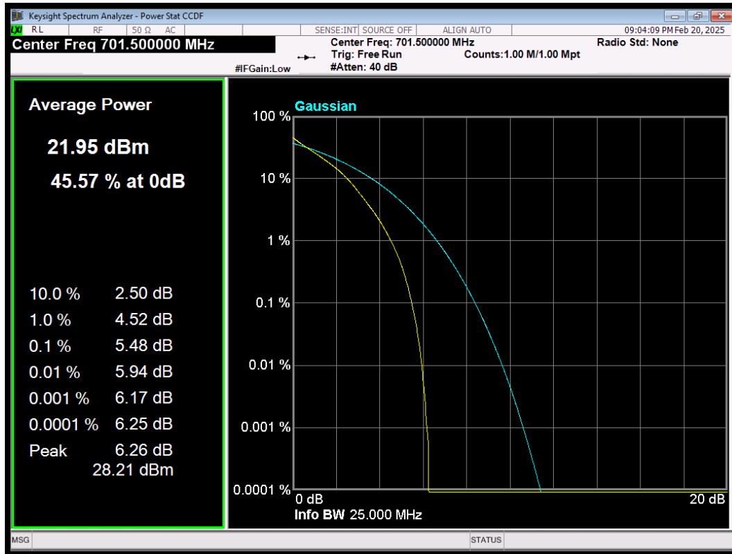
LTE Band12 QPSK BW=5MHz Channel=23035 RB Size=25 Position=#0
