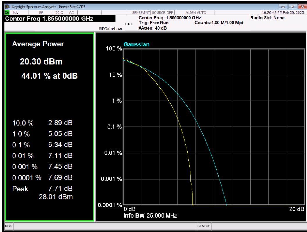
LTE Band25 QAM16 BW=10MHz Channel=26090 RB Size=50 Position=#0
