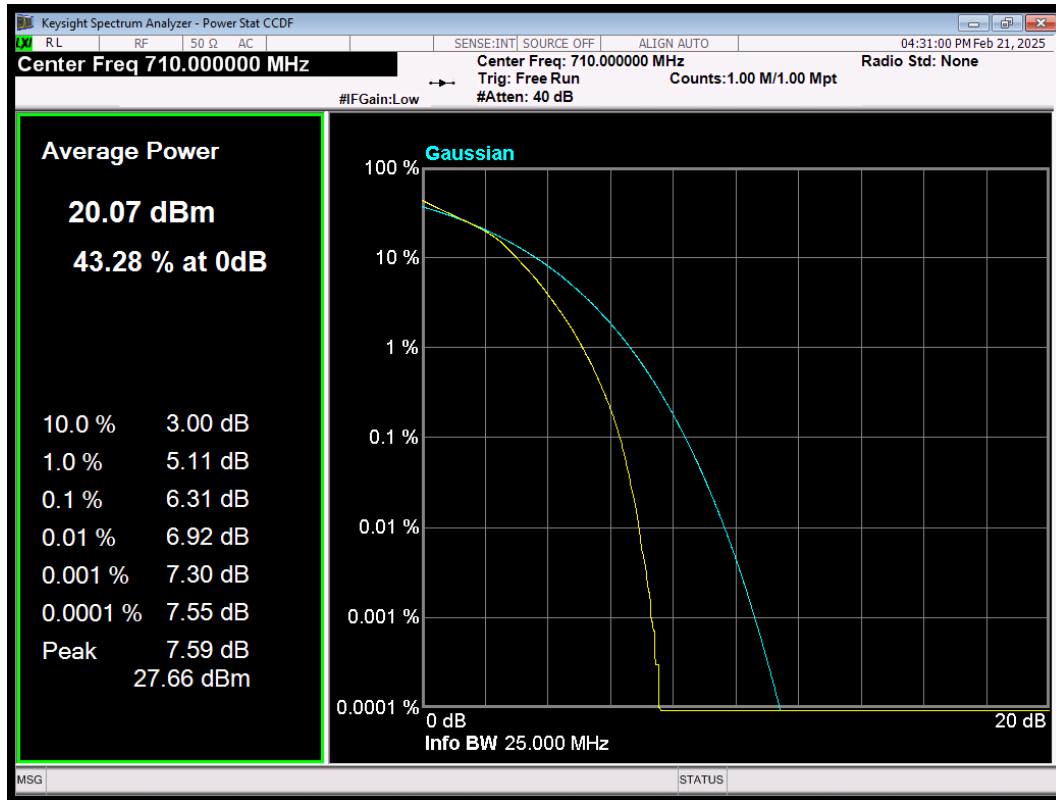
LTE Band17 QAM64 BW=10MHz Channel=23790 RB Size=50 Position=#0
