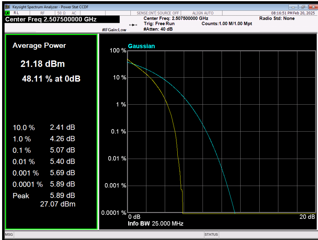
LTE Band7 QPSK BW=15MHz Channel=20825 RB Size=75 Position=#0
