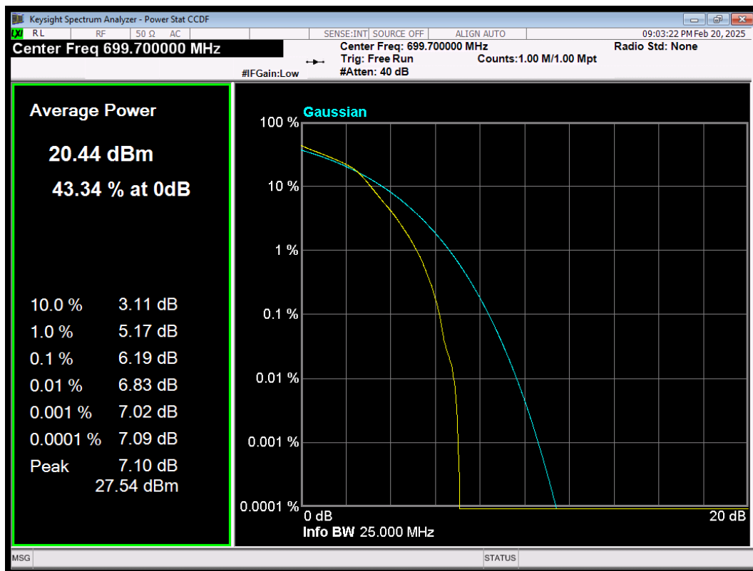
LTE Band12 QAM16 BW=1.4MHz Channel=23017 RB Size=6 Position=#0
