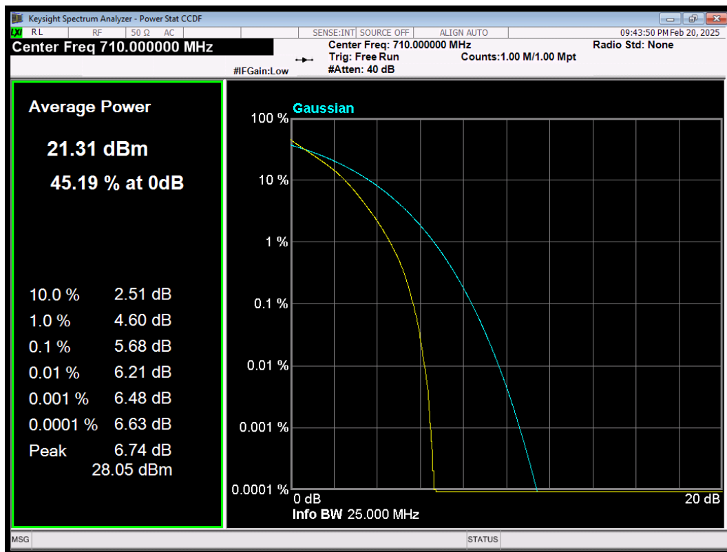
LTE Band17 QPSK BW=5MHz Channel=23790 RB Size=25 Position=#0
