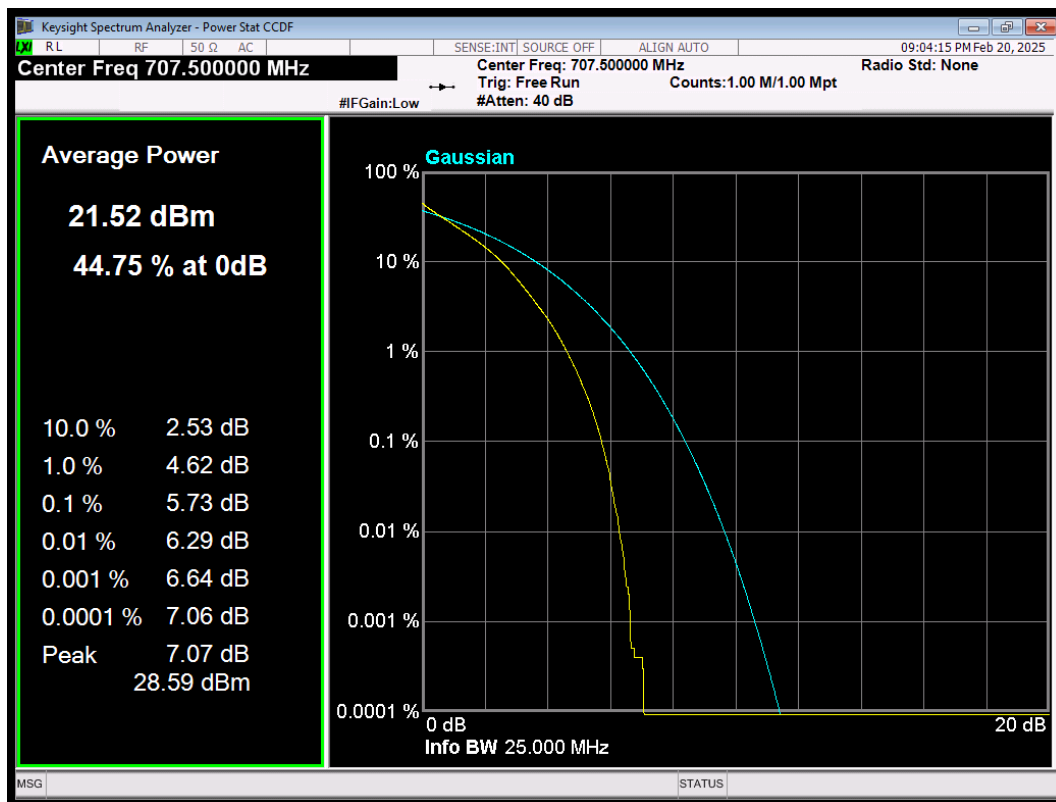
LTE Band12 QPSK BW=5MHz Channel=23095 RB Size=25 Position=#0
