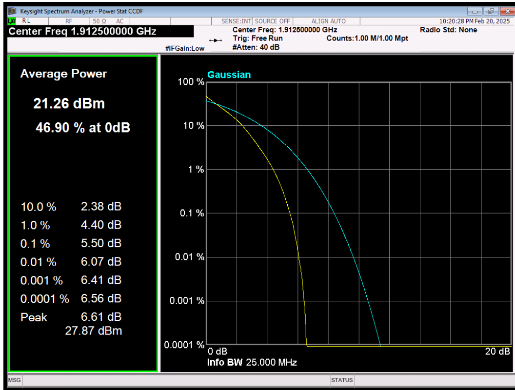
LTE Band25 QPSK BW=5MHz Channel=26665 RB Size=25 Position=#0
