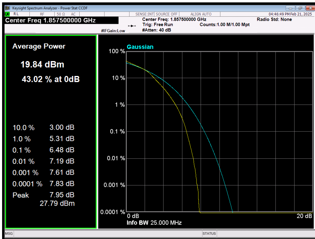
LTE Band25 QAM64 BW=15MHz Channel=26115 RB Size=75 Position=#0
