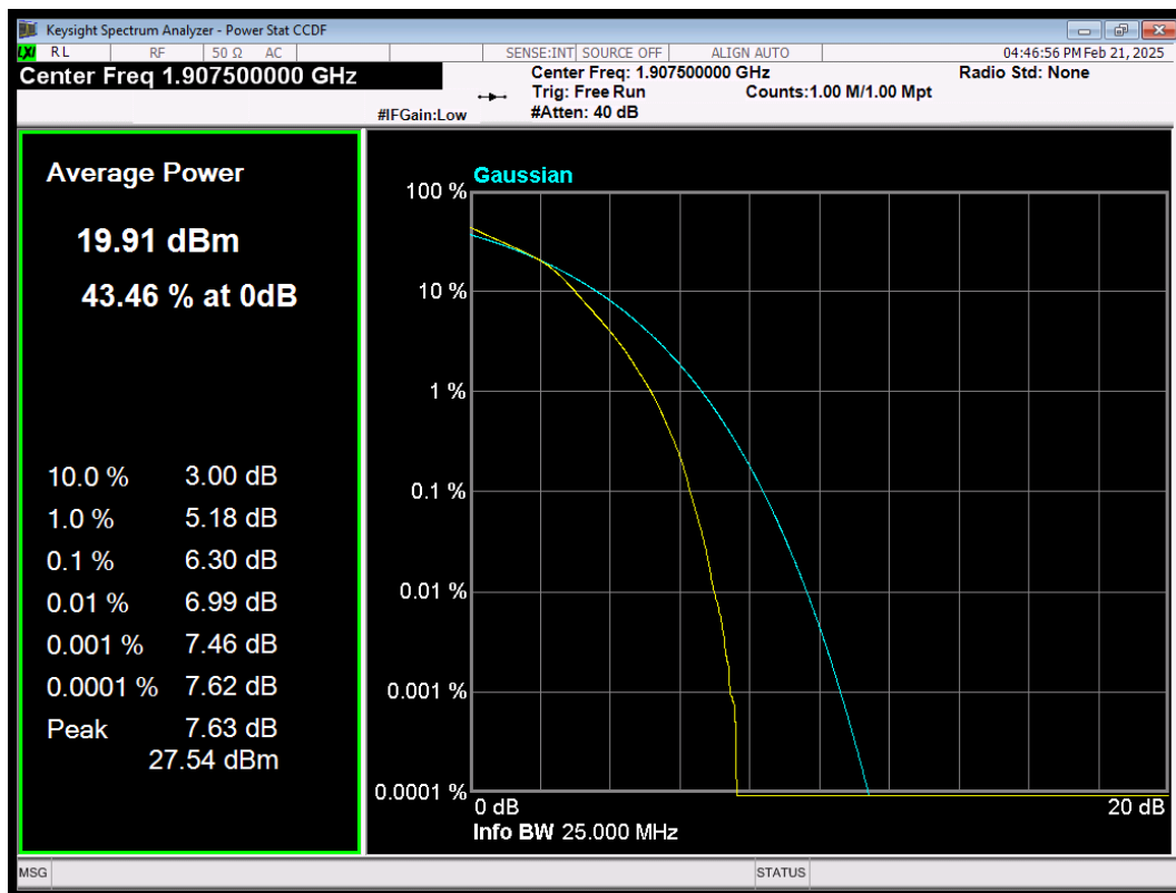
LTE Band25 QAM64 BW=15MHz Channel=26615 RB Size=75 Position=#0
