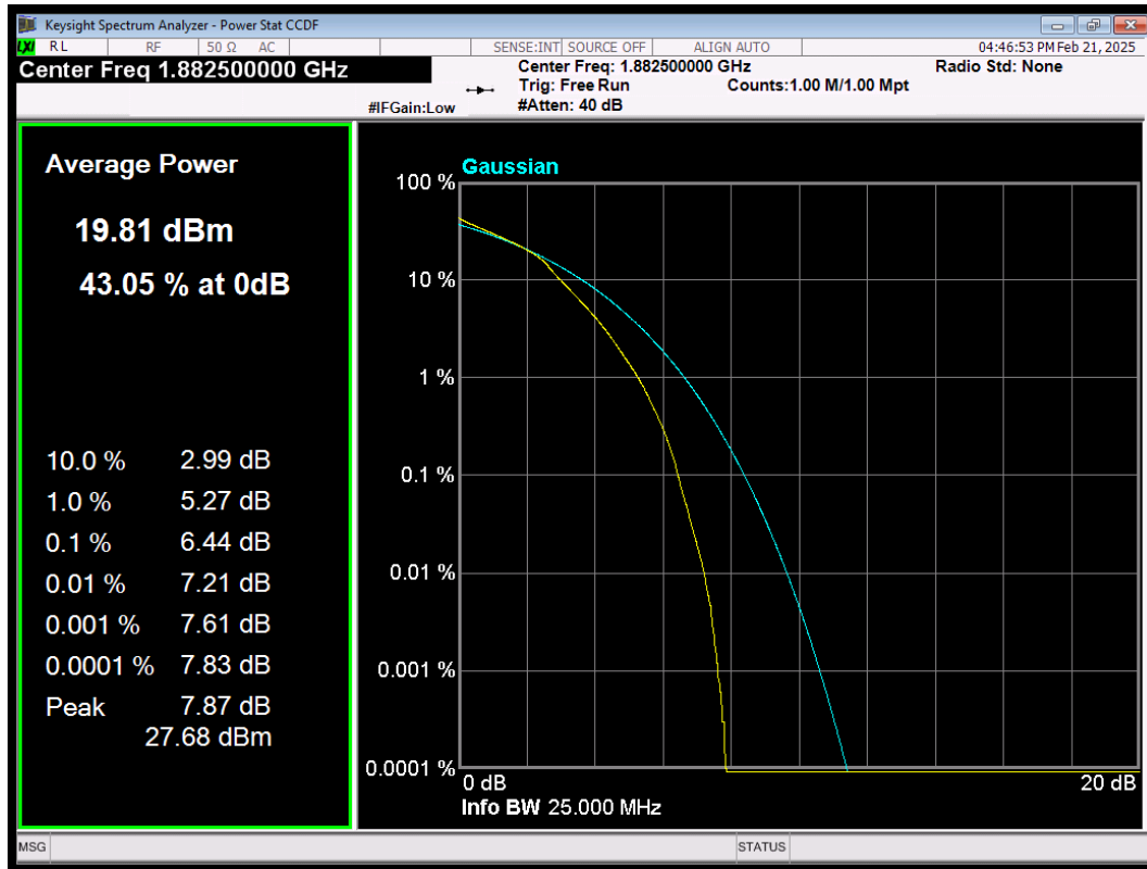
LTE Band25 QAM64 BW=15MHz Channel=26365 RB Size=75 Position=#0
