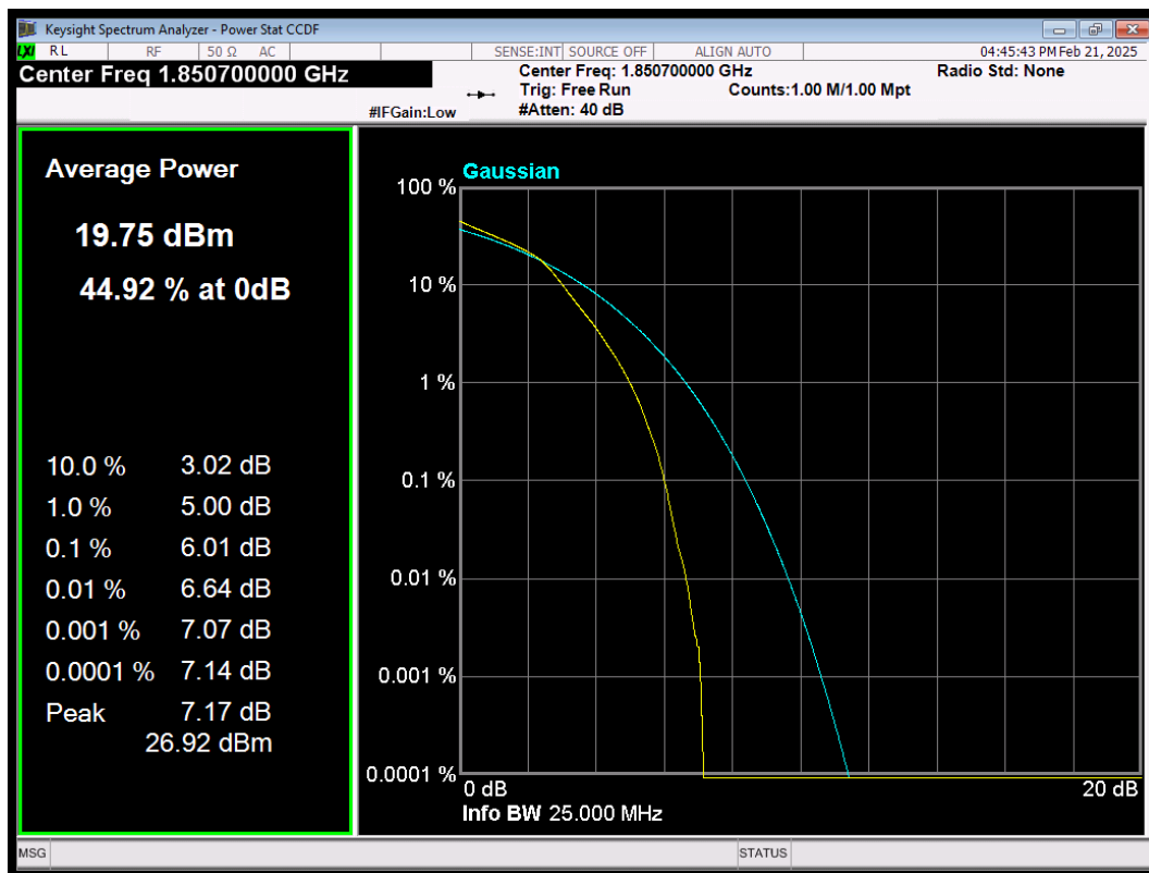
LTE Band25 QAM64 BW=1.4MHz Channel=26047 RB Size=6 Position=#0
