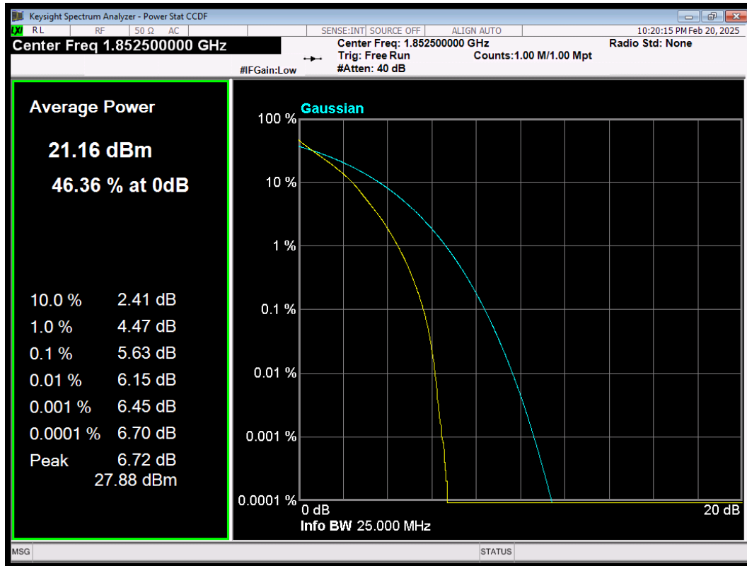
LTE Band25 QPSK BW=5MHz Channel=26065 RB Size=25 Position=#0
