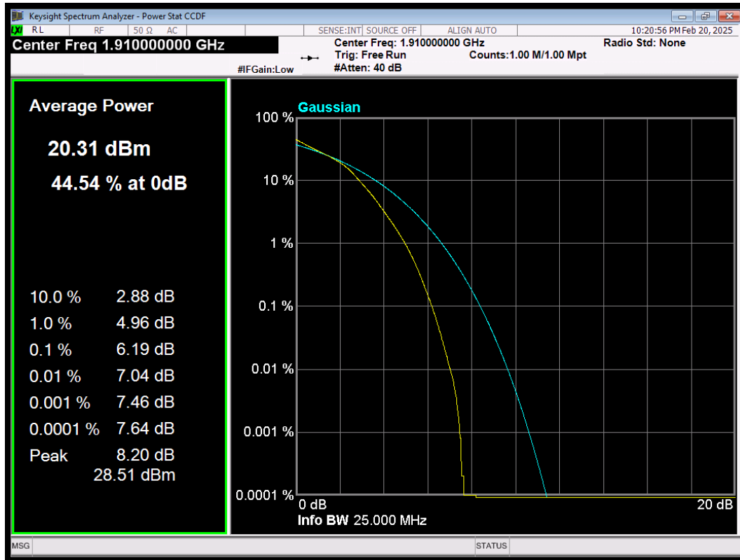
LTE Band25 QAM16 BW=10MHz Channel=26640 RB Size=50 Position=#0
