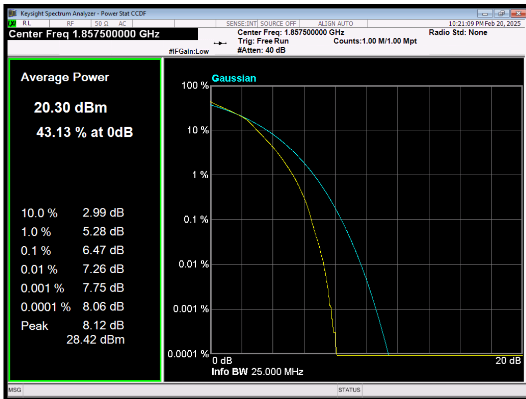
LTE Band25 QAM16 BW=15MHz Channel=26115 RB Size=75 Position=#0
