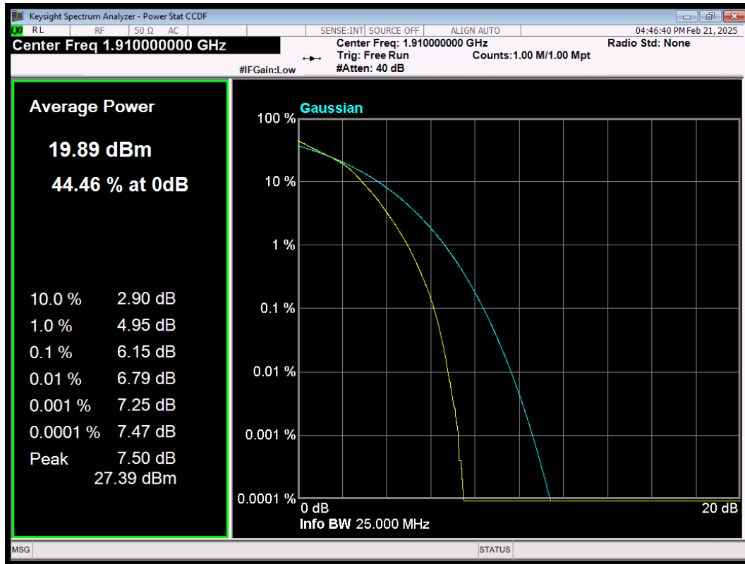
LTE Band25 QAM64 BW=10MHz Channel=26640 RB Size=50 Position=#0
