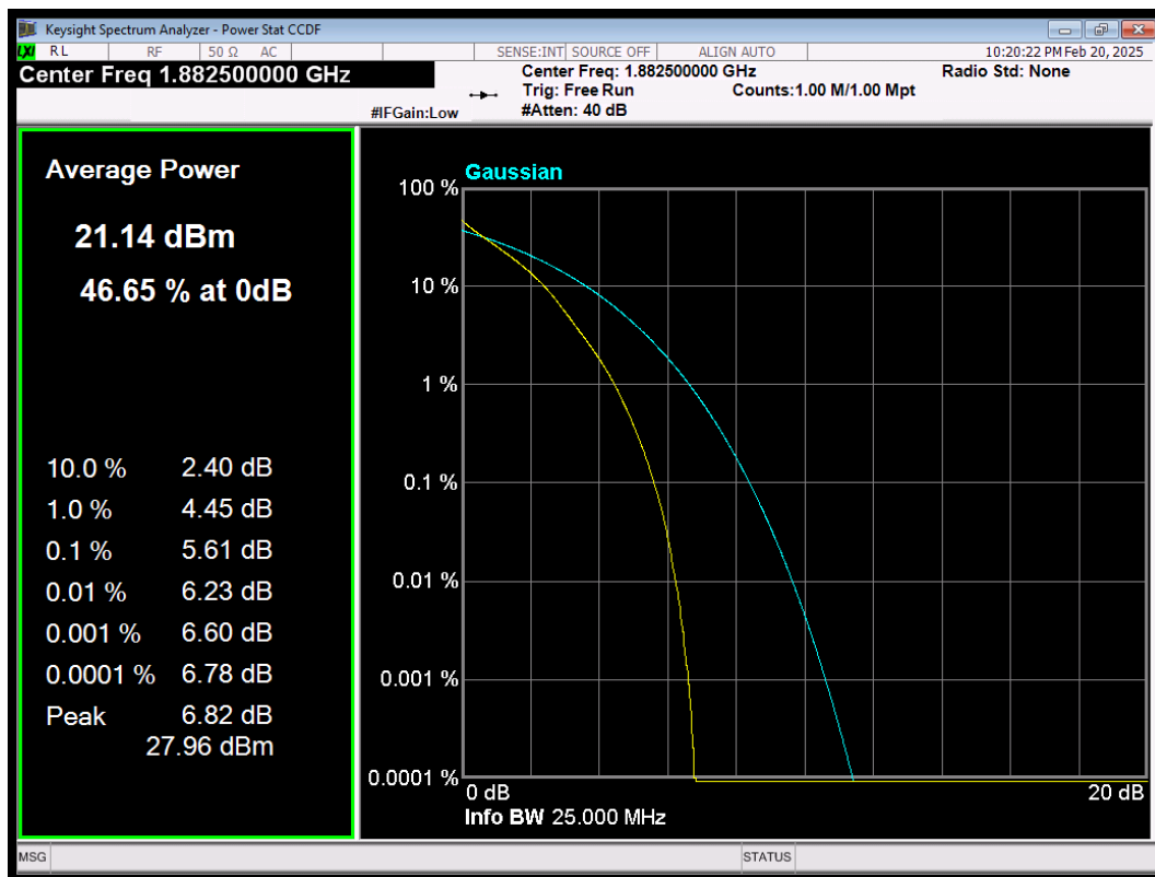
LTE Band25 QPSK BW=5MHz Channel=26365 RB Size=25 Position=#0
