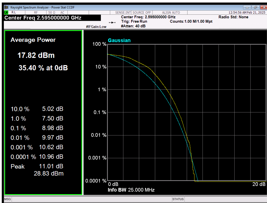
LTE Band38 QAM16 BW=20MHz Channel=38000 RB Size=100 Position=#0
