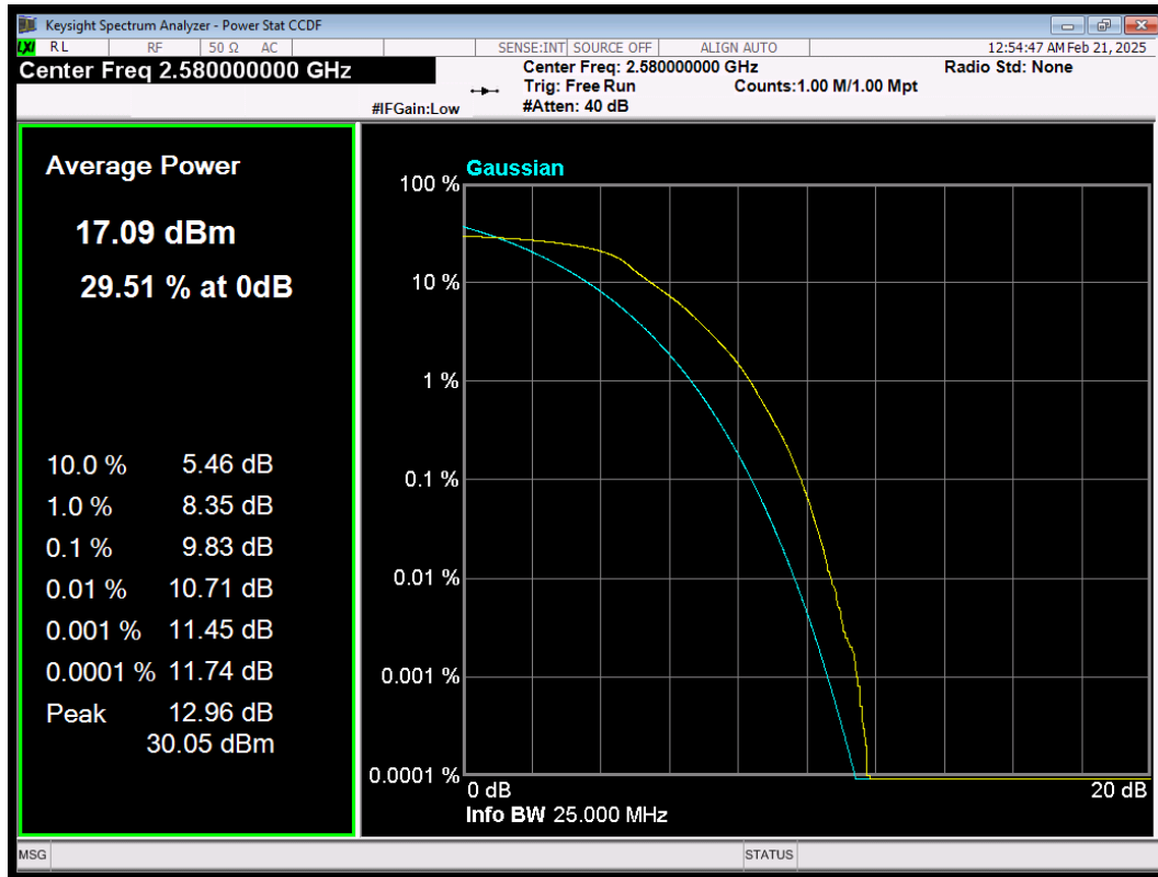
LTE Band38 QPSK BW=20MHz Channel=37850 RB Size=100 Position=#0
