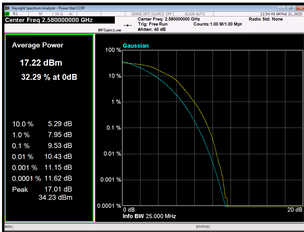
LTE Band38 QAM16 BW=20MHz Channel=37850 RB Size=100 Position=#0
