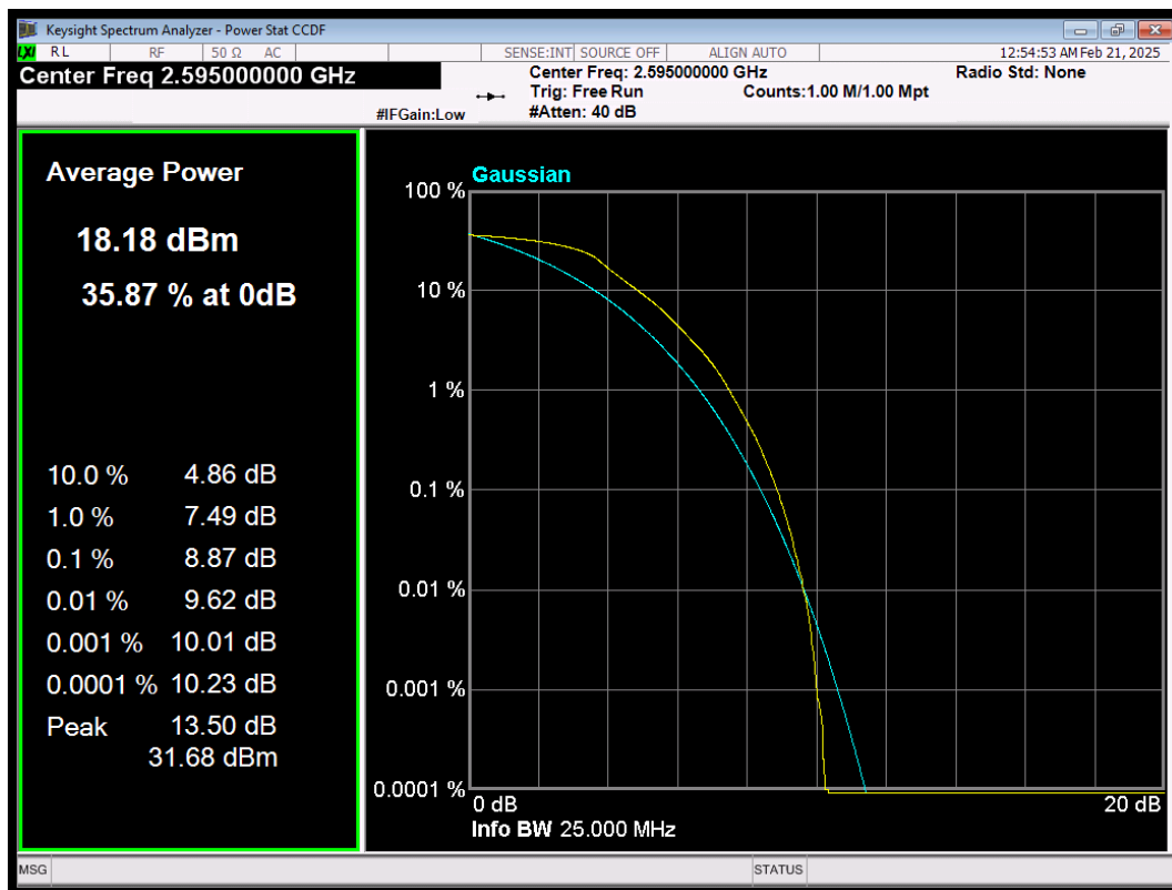
LTE Band38 QPSK BW=20MHz Channel=38000 RB Size=100 Position=#0
