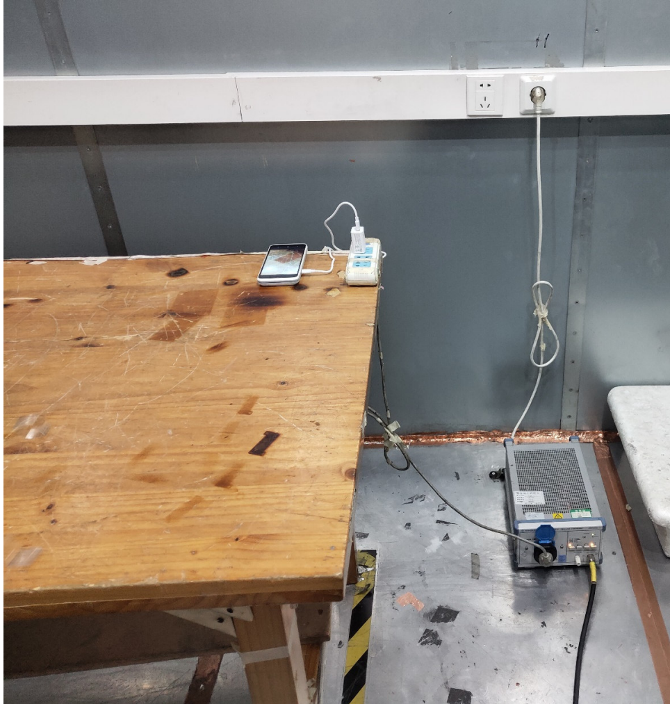
Picture 1: Radiated Emission Test Setup
