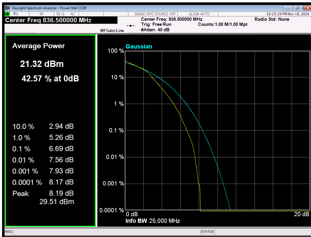
LTE Band5 16QAM BW=3MHz Channel=20525 RB Size=15 Position=#0
