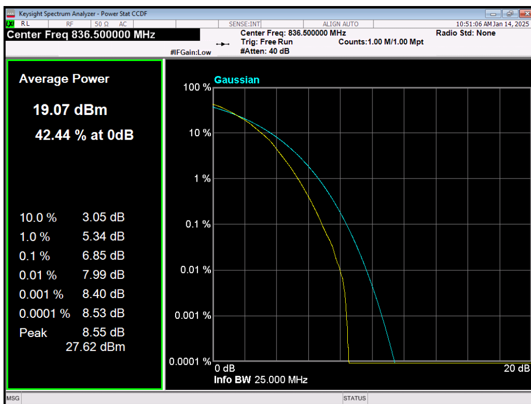
LTE Band5 64QAM BW=5MHz Channel=20525 RB Size=25 Position=#0
