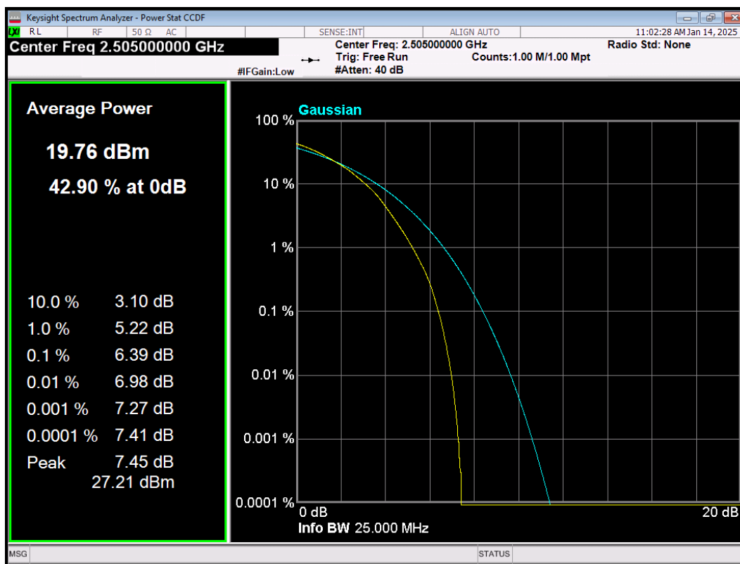
LTE Band7 64QAM BW=10MHz Channel=20800 RB Size=50 Position=#0
