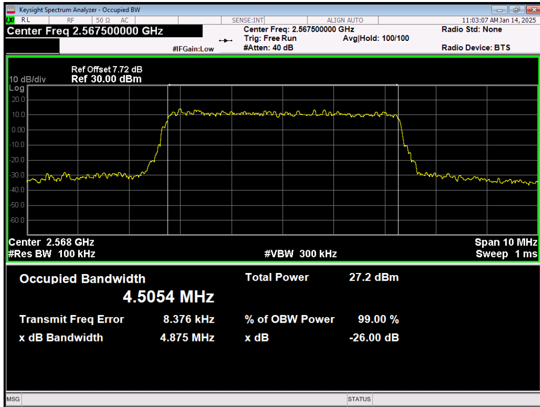
LTE Band7 64QAM BW=5MHz Channel=21425 RB Size=25 Position=#0
