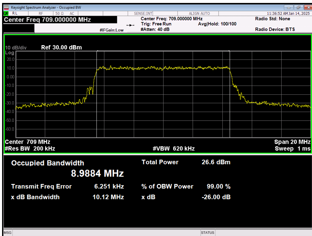
LTE Band17 64QAM BW=10MHz Channel=23780 RB Size=50 Position=#0
