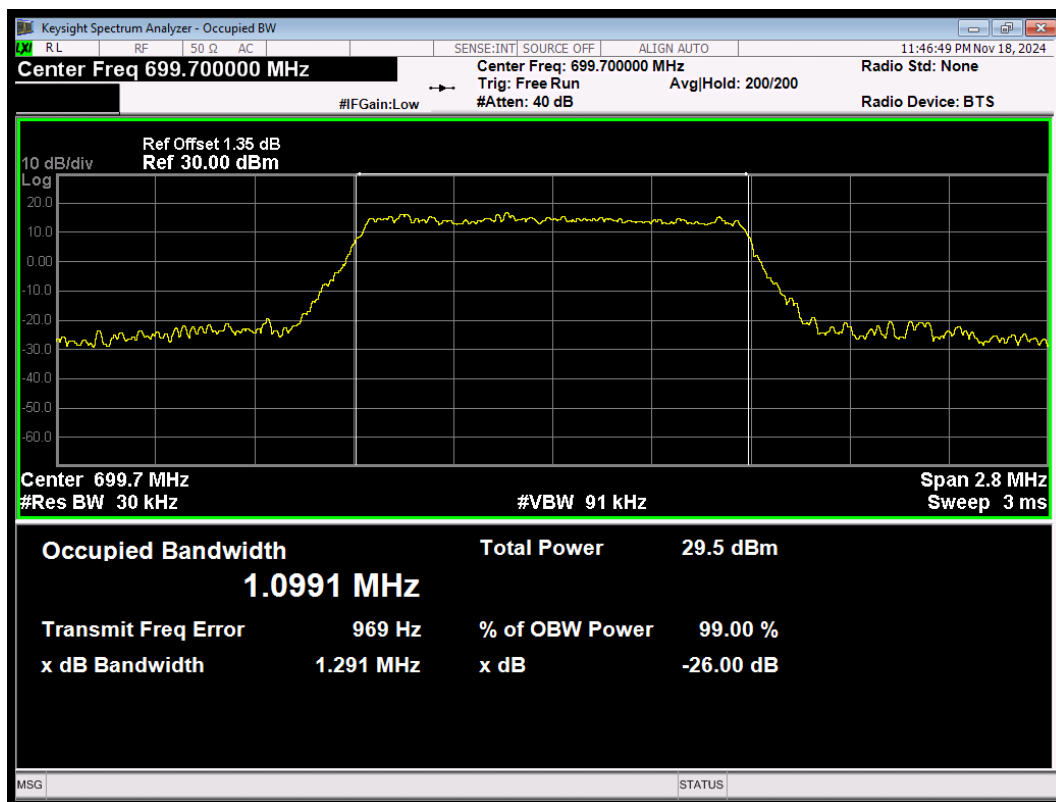
LTE Band12 16QAM BW=1.4MHz Channel=23017 RB Size=6 Position=#0
