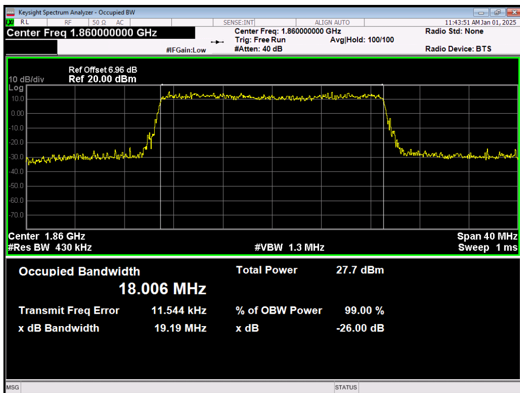
LTE Band25 16QAM BW=20MHz Channel=26140 RB Size=100 Position=#0
