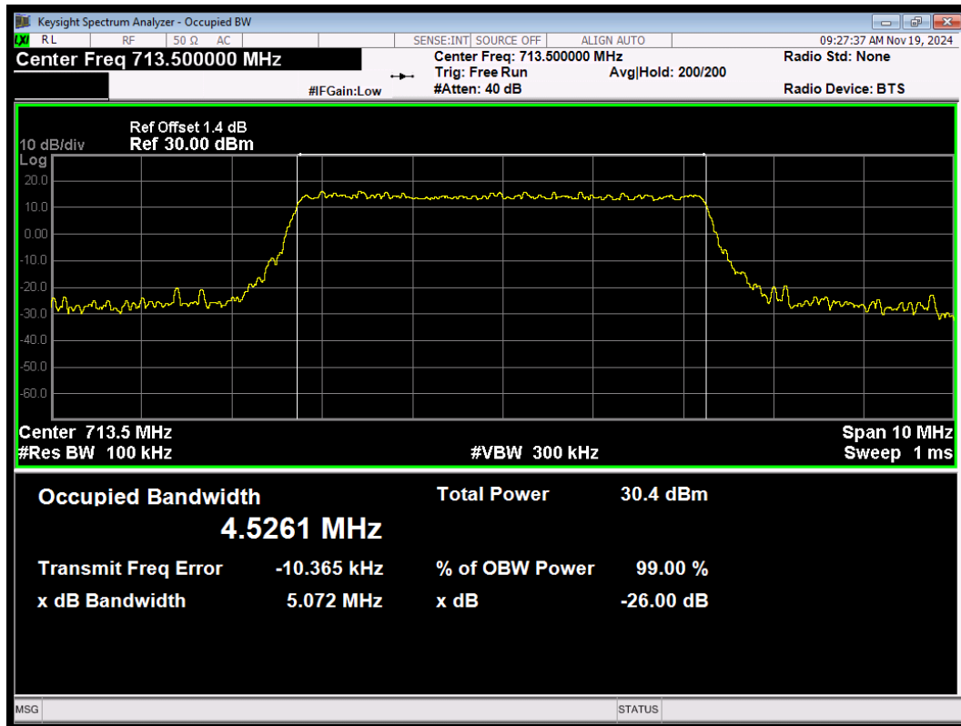
LTE Band17 QPSK BW=5MHz Channel=23825 RB Size=25 Position=#0
