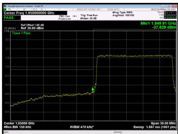
LTE Band2 16QAM BW=15MHz Channel=18675 RB Size=75 Position=#0
