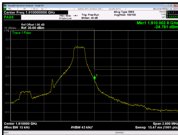
LTE Band2 16QAM BW=1.4MHz Channel=19193 RB Size=1 Position=#Max
