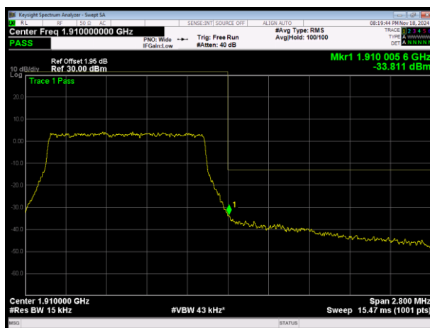
LTE Band2 16QAM BW=1.4MHz Channel=19193 RB Size=6 Position=#0
