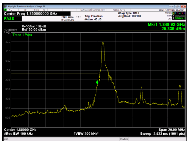
LTE Band2 16QAM BW=10MHz Channel=18650 RB Size=1 Position=#0
