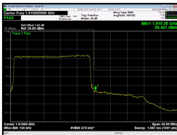
LTE Band2 16QAM BW=15MHz Channel=19125 RB Size=75 Position=#0
