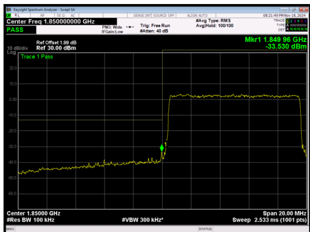
LTE Band2 16QAM BW=10MHz Channel=18650 RB Size=50 Position=#0
