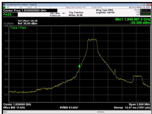
LTE Band2 16QAM BW=1.4MHz Channel=18607 RB Size=1 Position=#0
