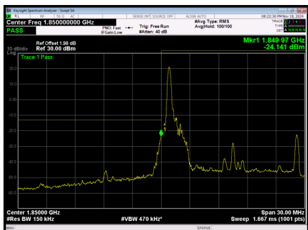
LTE Band2 16QAM BW=15MHz Channel=18675 RB Size=1 Position=#0
