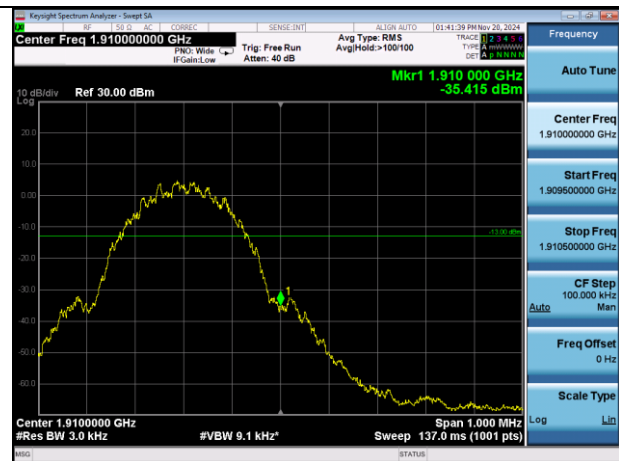
EGPRS1900H
