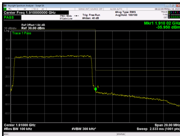
LTE Band2 16QAM BW=10MHz Channel=19150 RB Size=50 Position=#0
