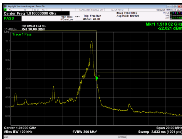
LTE Band2 16QAM BW=10MHz Channel=19150 RB Size=1 Position=#Max
