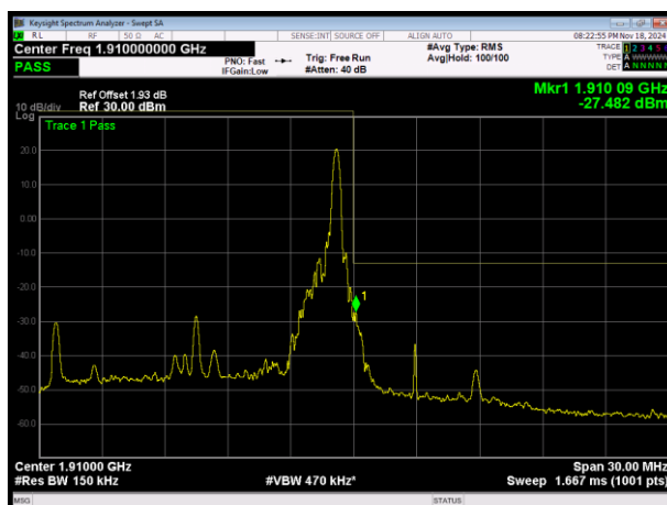
LTE Band2 16QAM BW=15MHz Channel=19125 RB Size=1 Position=#Max
