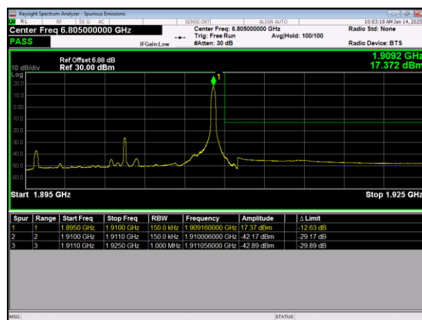
LTE Band2 64QAM BW=15MHz HighChannel=19125 RB Size=1 Position=#Max
