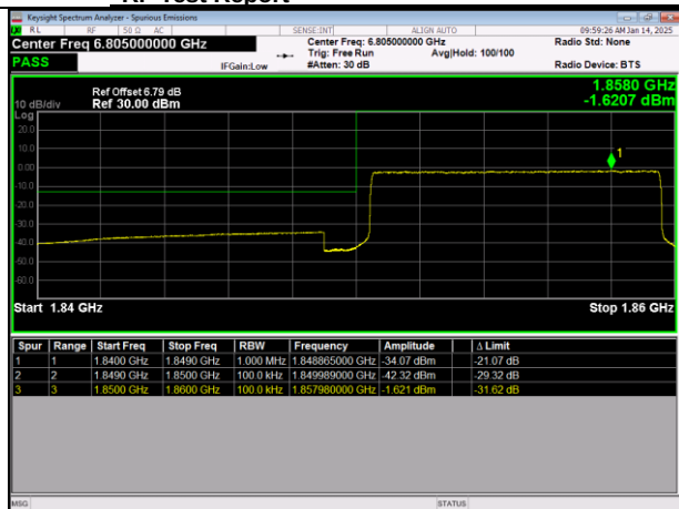
LTE Band2 64QAM BW=10MHz LowChannel=18650 RB Size=50 Position=#0
