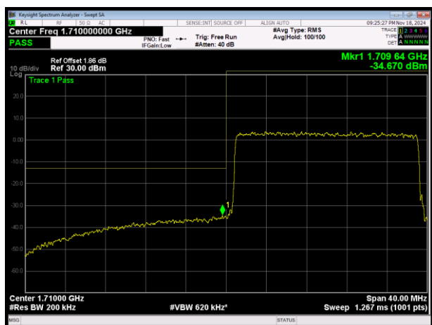
LTE Band4 16QAM BW=20MHz Channel=20050 RB Size=100 Position=#0
