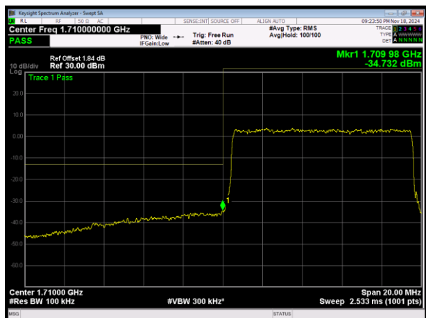
LTE Band4 16QAM BW=10MHz Channel=20000 RB Size=50 Position=#0
