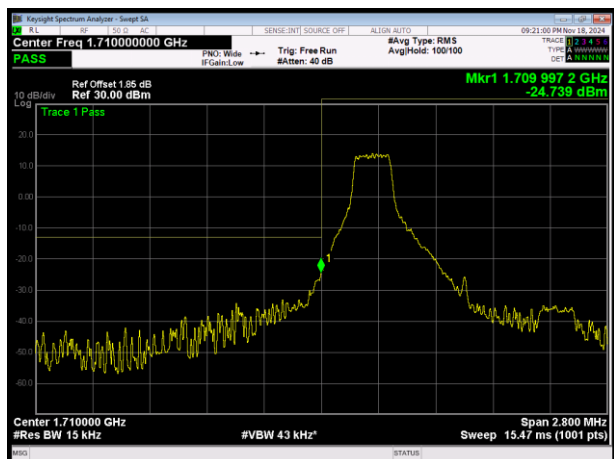
LTE Band4 QPSK BW=1.4MHz Channel=19957 RB Size=1 Position=#0
