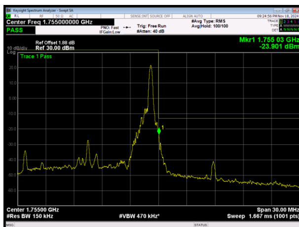
LTE Band4 16QAM BW=15MHz Channel=20325 RB Size=1 Position=#Max
