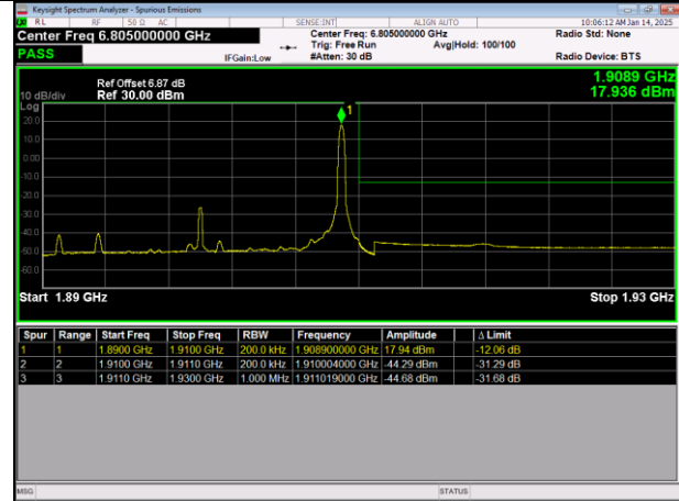
LTE Band2 64QAM BW=20MHz HighChannel=19100 RB Size=1 Position=#Max
