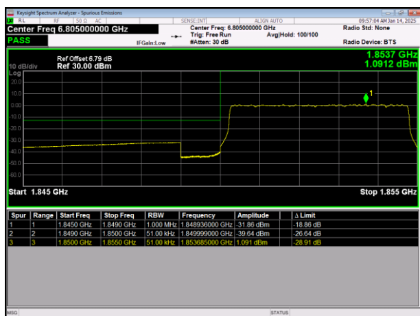
LTE Band2 64QAM BW=5MHz LowChannel=18625 RB Size=25 Position=#0
