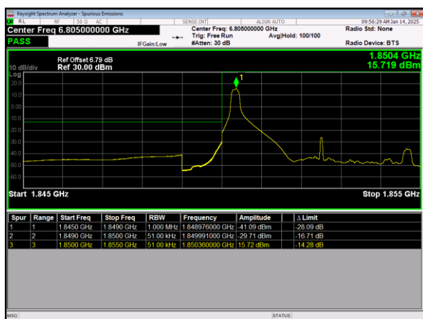
LTE Band2 64QAM BW=5MHz LowChannel=18625 RB Size=1 Position=#0
