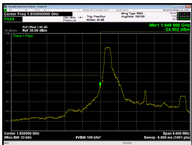
LTE Band2 16QAM BW=3MHz Channel=18615 RB Size=1 Position=#0
