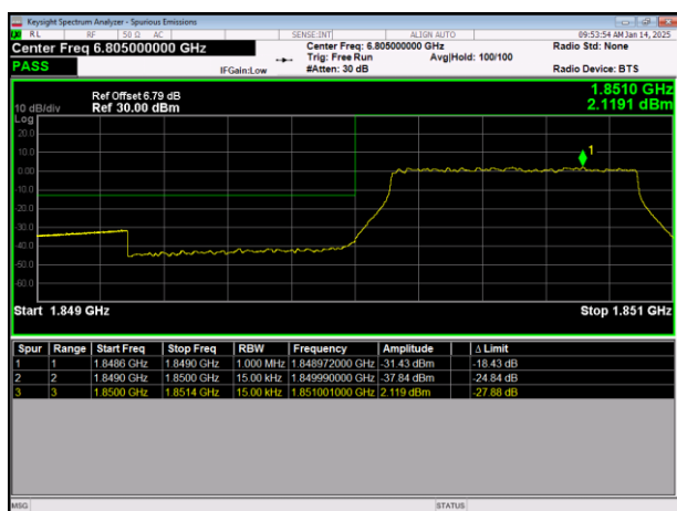
LTE Band2 64QAM BW=1.4MHz LowChannel=18607 RB Size=6 Position=#0
