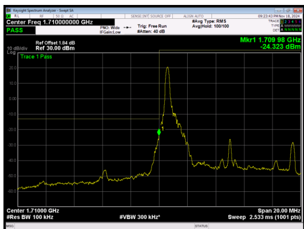
LTE Band4 16QAM BW=10MHz Channel=20000 RB Size=1 Position=#0
