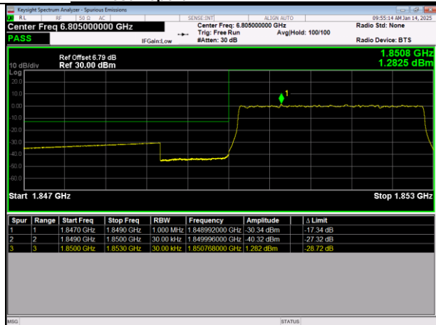
LTE Band2 64QAM BW=3MHz LowChannel=18615 RB Size=15 Position=#0
