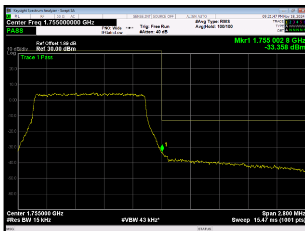
LTE Band4 16QAM BW=1.4MHz Channel=20393 RB Size=6 Position=#0
