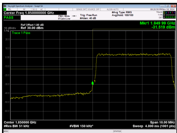
LTE Band2 QPSK BW=5MHz Channel=18625 RB Size=25 Position=#0
