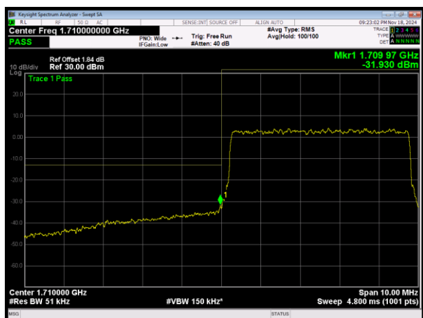
LTE Band4 16QAM BW=5MHz Channel=19975 RB Size=25 Position=#0
