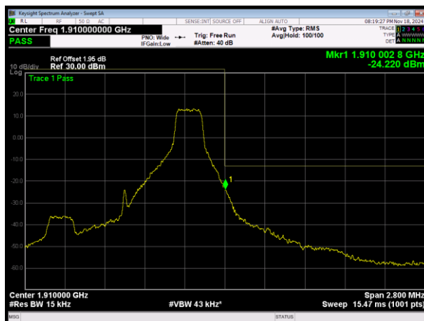
LTE Band2 QPSK BW=1.4MHz Channel=19193 RB Size=1 Position=#Max
