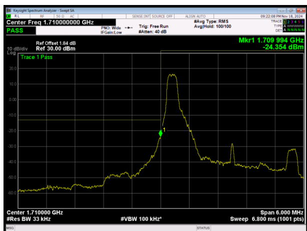
LTE Band4 16QAM BW=3MHz Channel=19965 RB Size=1 Position=#0
