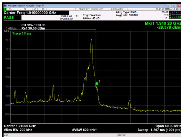
LTE Band2 16QAM BW=20MHz Channel=19100 RB Size=1 Position=#Max
