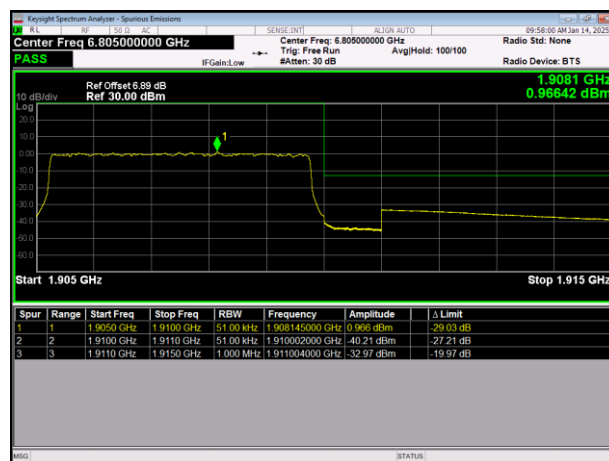
LTE Band2 64QAM BW=5MHz HighChannel=19175 RB Size=25 Position=#0
