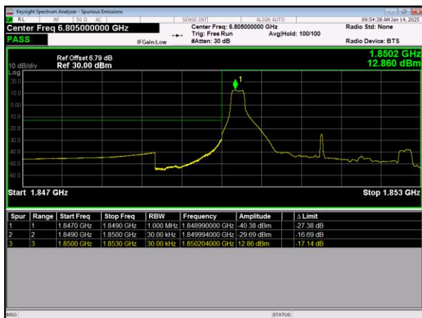
LTE Band2 64QAM BW=3MHz LowChannel=18615 RB Size=1 Position=#0
