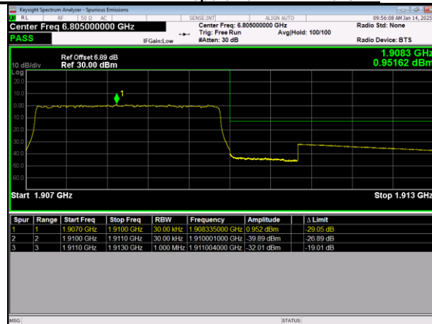
LTE Band2 64QAM BW=3MHz HighChannel=19185 RB Size=15 Position=#0
