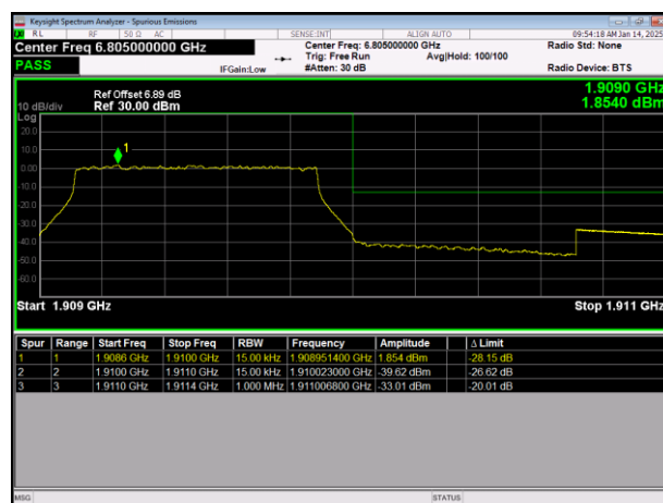
LTE Band2 64QAM BW=1.4MHz HighChannel=19193 RB Size=6 Position=#0
