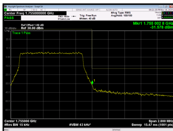
LTE Band4 QPSK BW=1.4MHz Channel=20393 RB Size=6 Position=#0
