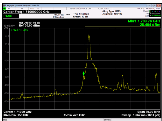
LTE Band4 16QAM BW=15MHz Channel=20025 RB Size=1 Position=#0
