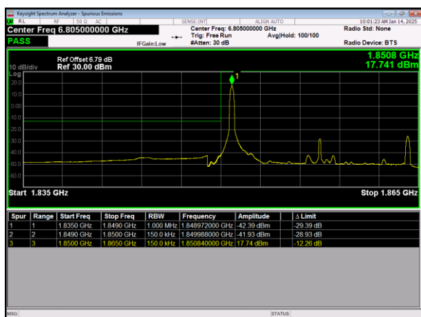
LTE Band2 64QAM BW=15MHz LowChannel=18675 RB Size=1 Position=#0
