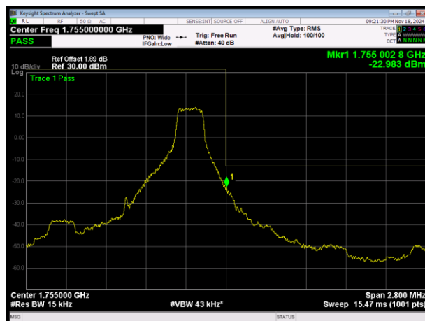
LTE Band4 QPSK BW=1.4MHz Channel=20393 RB Size=1 Position=#Max
