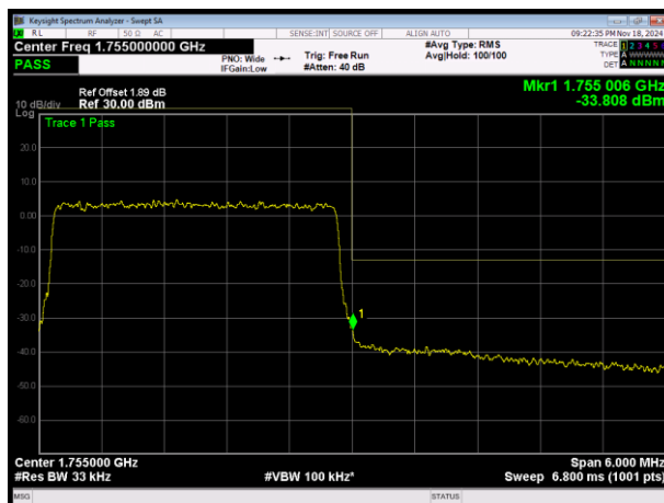
LTE Band4 16QAM BW=3MHz Channel=20385 RB Size=15 Position=#0
