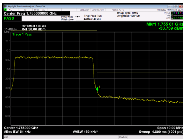
LTE Band4 16QAM BW=5MHz Channel=20375 RB Size=25 Position=#0
