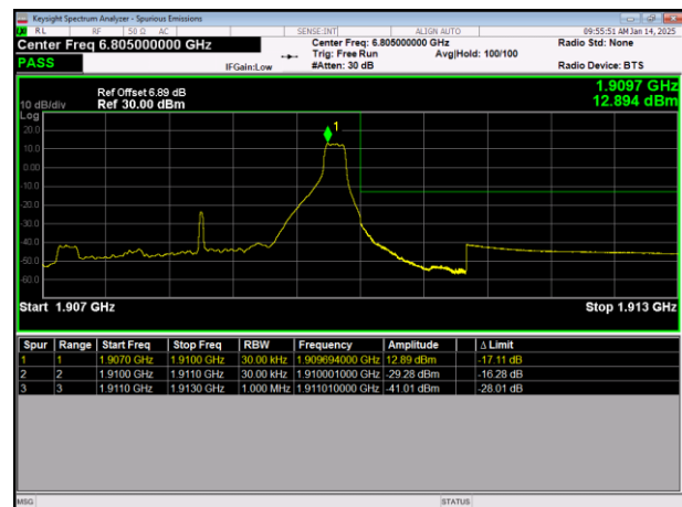
LTE Band2 64QAM BW=3MHz HighChannel=19185 RB Size=1 Position=#Max
