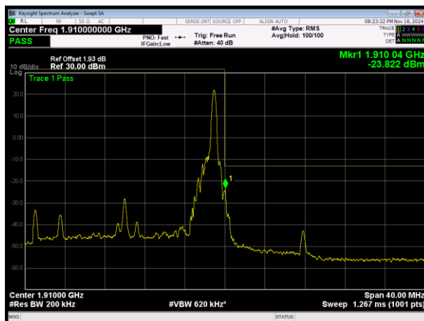
LTE Band2 QPSK BW=20MHz Channel=19100 RB Size=1 Position=#Max
