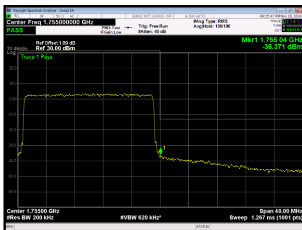
LTE Band4 16QAM BW=20MHz Channel=20300 RB Size=100 Position=#0
