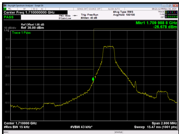
LTE Band4 16QAM BW=1.4MHz Channel=19957 RB Size=1 Position=#0
