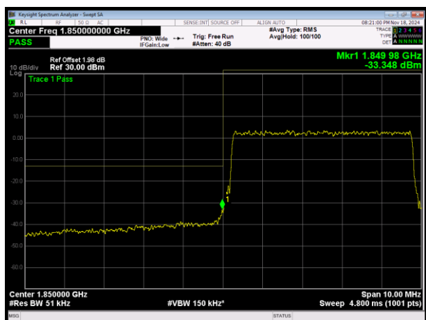
LTE Band2 16QAM BW=5MHz Channel=18625 RB Size=25 Position=#0
