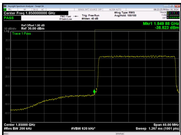
LTE Band2 16QAM BW=20MHz Channel=18700 RB Size=100 Position=#0
