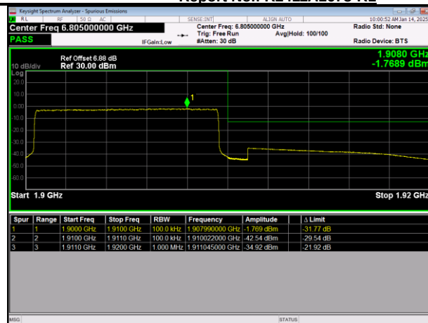
LTE Band2 64QAM BW=10MHz HighChannel=19150 RB Size=50 Position=#0
