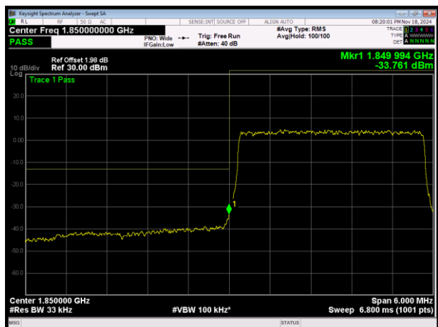
LTE Band2 QPSK BW=3MHz Channel=18615 RB Size=15 Position=#0
