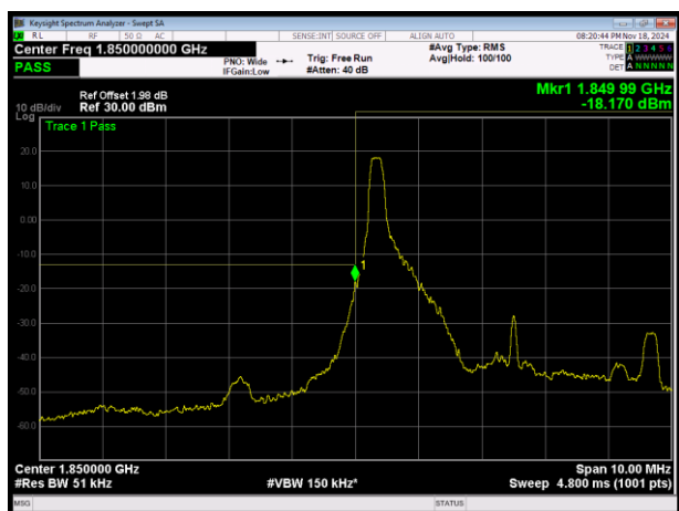
LTE Band2 QPSK BW=5MHz Channel=18625 RB Size=1 Position=#0
