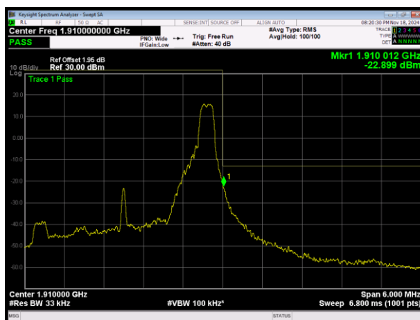
LTE Band2 16QAM BW=3MHz Channel=19185 RB Size=1 Position=#Max
