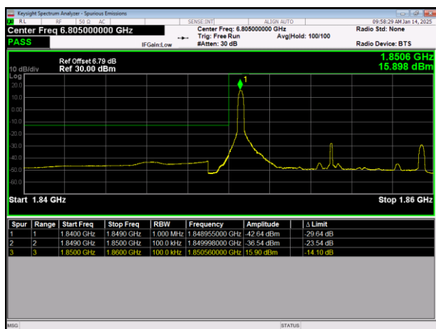
LTE Band2 64QAM BW=10MHz LowChannel=18650 RB Size=1 Position=#0
