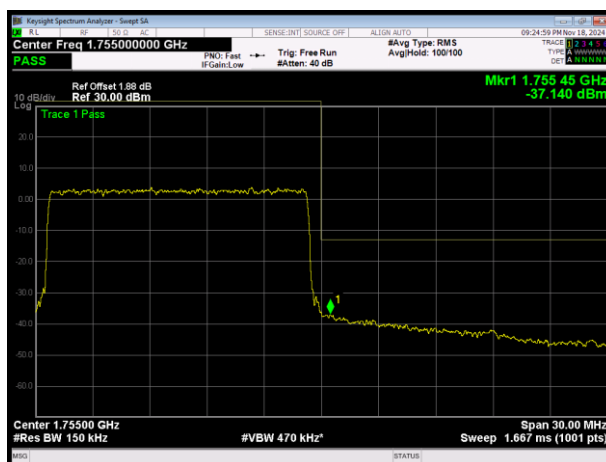
LTE Band4 16QAM BW=15MHz Channel=20325 RB Size=75 Position=#0
