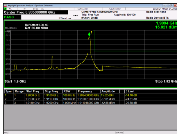
LTE Band2 64QAM BW=10MHz HighChannel=19150 RB Size=1 Position=#Max
