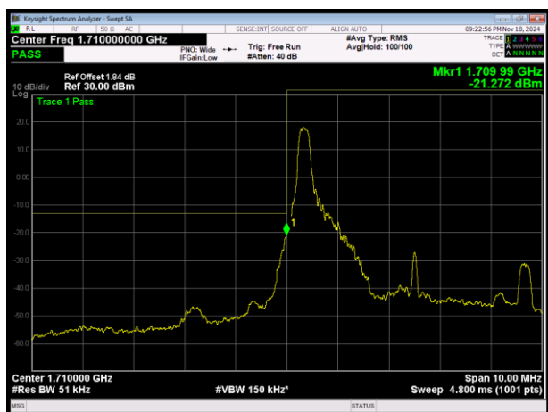
LTE Band4 16QAM BW=5MHz Channel=19975 RB Size=1 Position=#0
