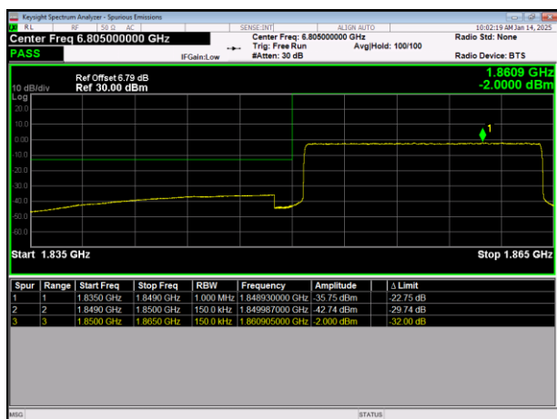
LTE Band2 64QAM BW=15MHz LowChannel=18675 RB Size=75 Position=#0
