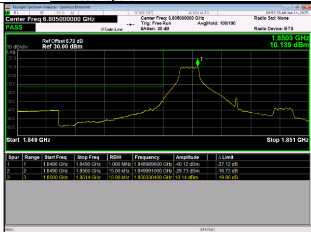
LTE Band2 64QAM BW=1.4MHz LowChannel=18607 RB Size=1 Position=#0
