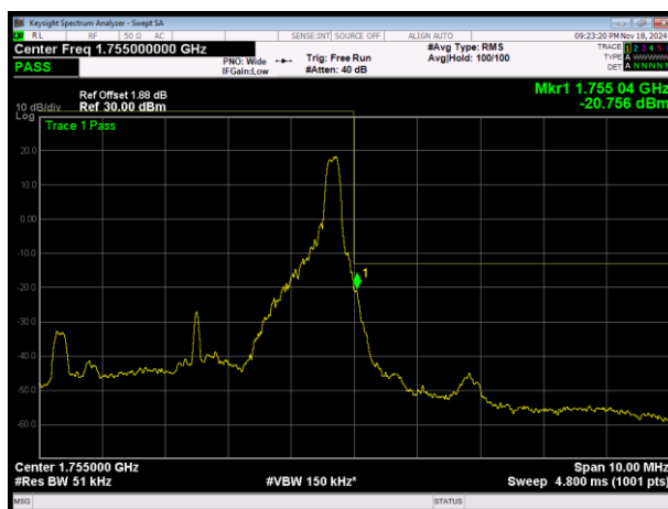
LTE Band4 16QAM BW=5MHz Channel=20375 RB Size=1 Position=#Max
