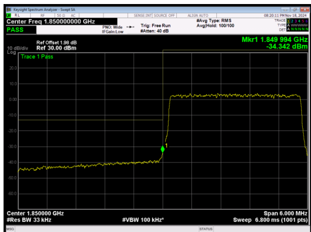
LTE Band2 16QAM BW=3MHz Channel=18615 RB Size=15 Position=#0
