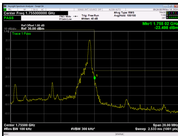
LTE Band4 16QAM BW=10MHz Channel=20350 RB Size=1 Position=#Max
