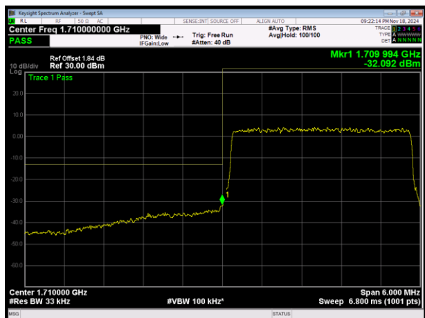
LTE Band4 16QAM BW=3MHz Channel=19965 RB Size=15 Position=#0
