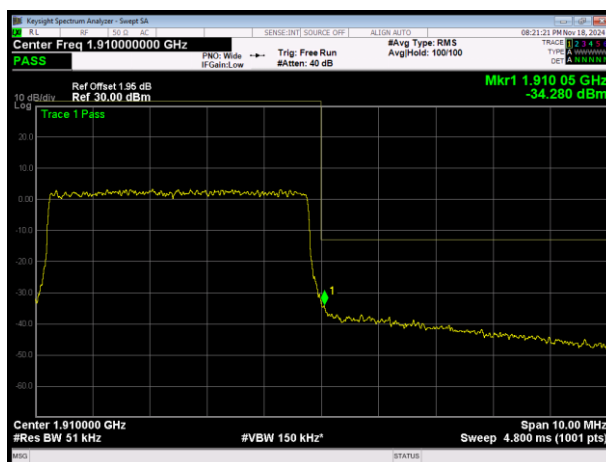
LTE Band2 16QAM BW=5MHz Channel=19175 RB Size=25 Position=#0
