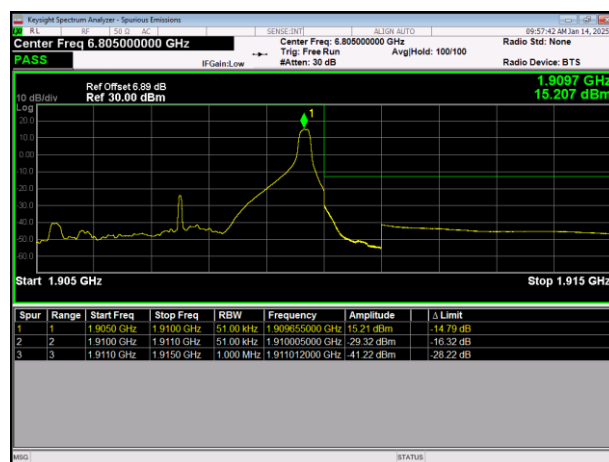
LTE Band2 64QAM BW=5MHz HighChannel=19175 RB Size=1 Position=#Max
