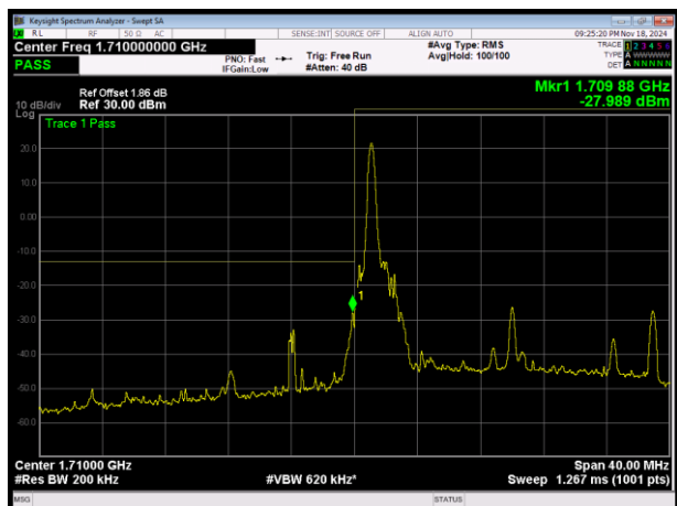
LTE Band4 16QAM BW=20MHz Channel=20050 RB Size=1 Position=#0
