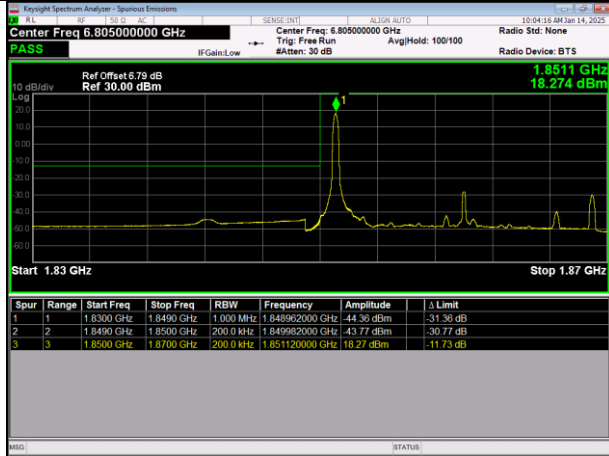
LTE Band2 64QAM BW=20MHz LowChannel=18700 RB Size=1 Position=#0
