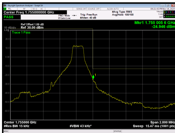
LTE Band4 16QAM BW=1.4MHz Channel=20393 RB Size=1 Position=#Max
