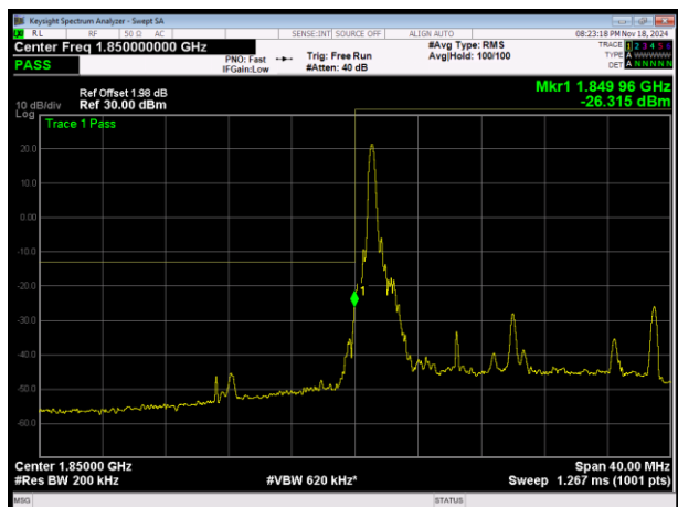
LTE Band2 16QAM BW=20MHz Channel=18700 RB Size=1 Position=#0
