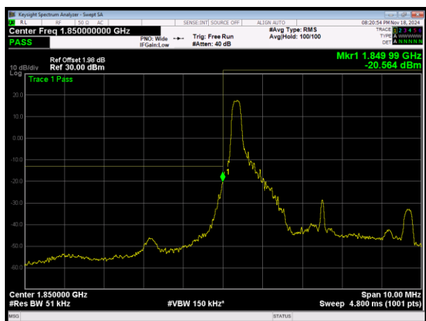
LTE Band2 16QAM BW=5MHz Channel=18625 RB Size=1 Position=#0
