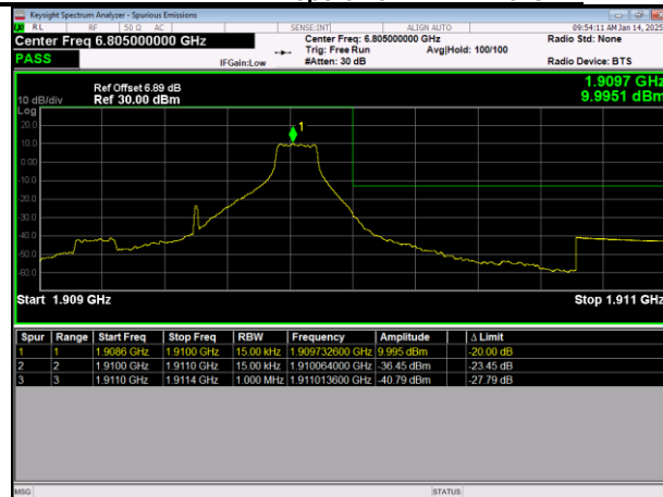
LTE Band2 64QAM BW=1.4MHz HighChannel=19193 RB Size=1 Position=#Max
