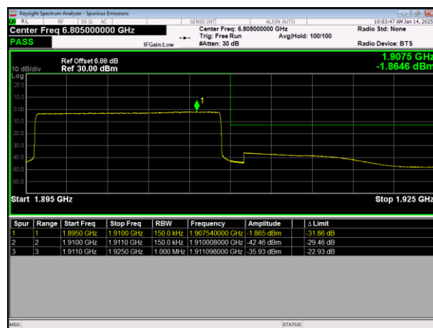
LTE Band2 64QAM BW=15MHz HighChannel=19125 RB Size=75 Position=#0
