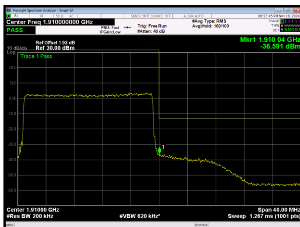
LTE Band2 16QAM BW=20MHz Channel=19100 RB Size=100 Position=#0
