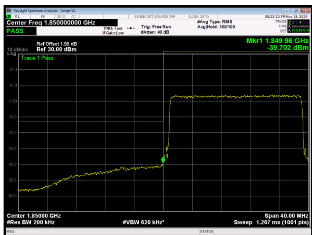
LTE Band2 QPSK BW=20MHz Channel=18700 RB Size=100 Position=#0
