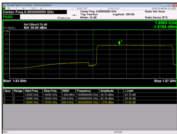
LTE Band2 64QAM BW=20MHz LowChannel=18700 RB Size=100 Position=#0
