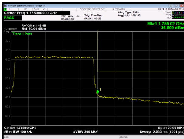
LTE Band4 16QAM BW=10MHz Channel=20350 RB Size=50 Position=#0
