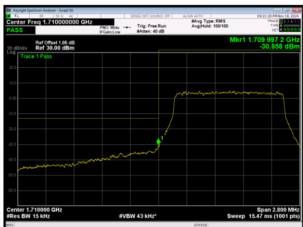
LTE Band4 16QAM BW=1.4MHz Channel=19957 RB Size=6 Position=#0
