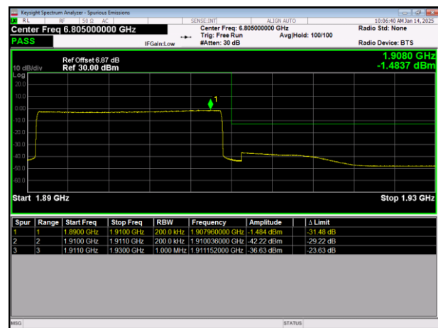
LTE Band2 64QAM BW=20MHz HighChannel=19100 RB Size=100 Position=#0
