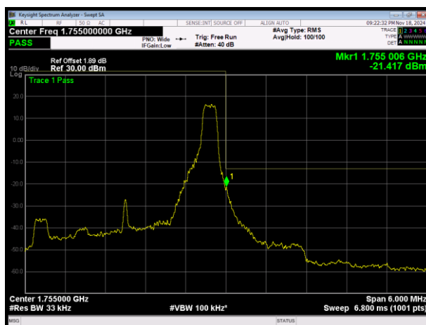
LTE Band4 16QAM BW=3MHz Channel=20385 RB Size=1 Position=#Max
