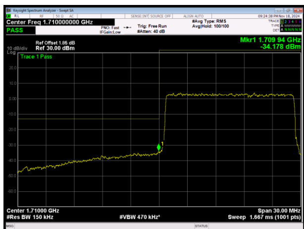
LTE Band4 16QAM BW=15MHz Channel=20025 RB Size=75 Position=#0
