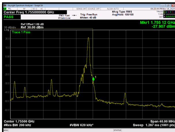
LTE Band4 16QAM BW=20MHz Channel=20300 RB Size=1 Position=#Max
