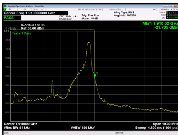
LTE Band2 16QAM BW=5MHz Channel=19175 RB Size=1 Position=#Max
