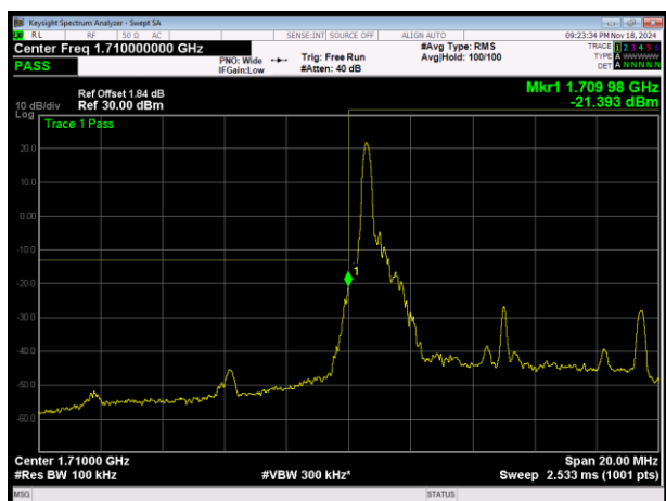
LTE Band4 QPSK BW=10MHz Channel=20000 RB Size=1 Position=#0
