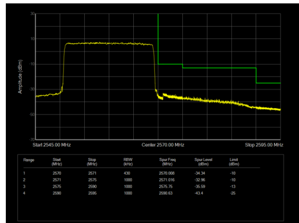
LTE Band7 QPSK BW=20MHz Channel=21350 RB Size=100 Position=#0
