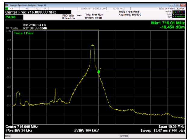
LTE Band12 16QAM BW=5MHz Channel=23155 RB Size=1 Position=#Max
