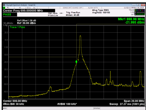
LTE Band12 QPSK BW=10MHz Channel=23060 RB Size=1 Position=#0
