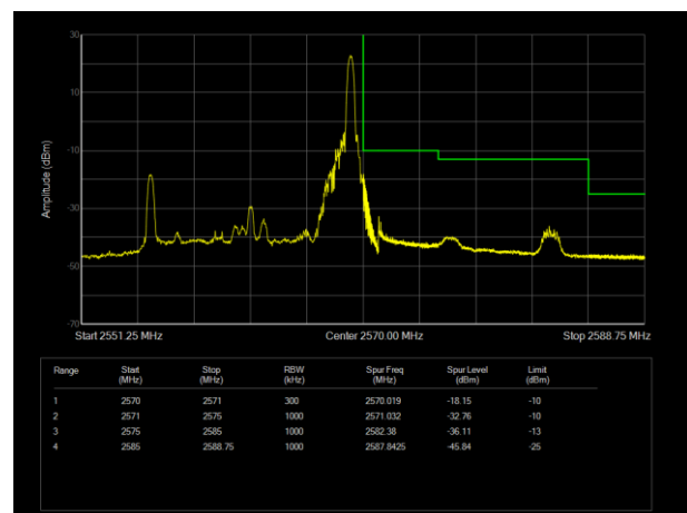
LTE Band7 16QAM BW=15MHz Channel=21375 RB Size=1 Position=#Max
