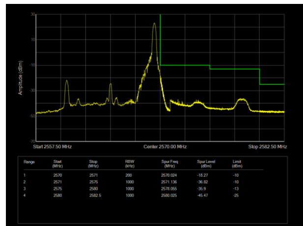
LTE Band7 QPSK BW=10MHz Channel=21400 RB Size=1 Position=#Max
