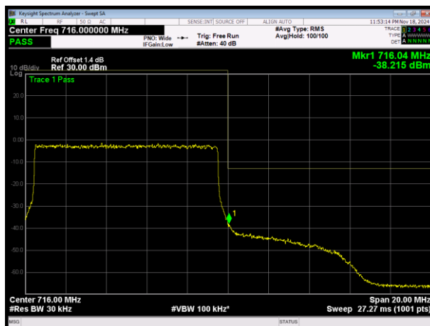
LTE Band12 16QAM BW=10MHz Channel=23130 RB Size=50 Position=#0
