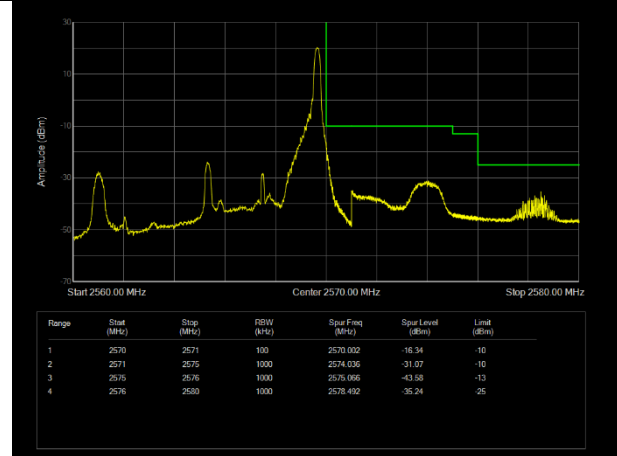
LTE Band7 16QAM BW=5MHz Channel=21425 RB Size=1 Position=#Max
