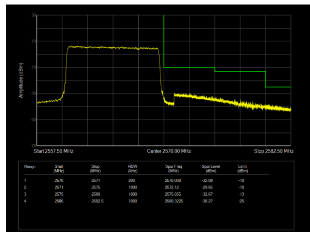
LTE Band7 16QAM BW=10MHz Channel=21400 RB Size=50 Position=#0
