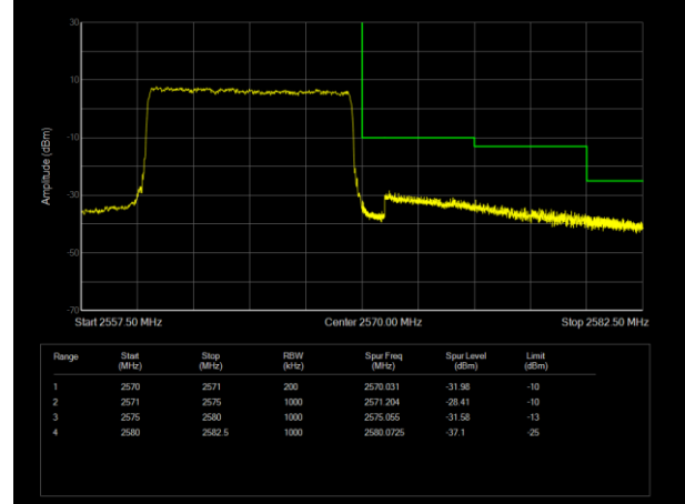
LTE Band7 QPSK BW=10MHz Channel=21400 RB Size=50 Position=#0
