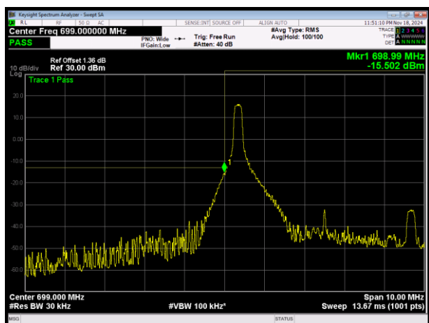
LTE Band12 QPSK BW=5MHz Channel=23035 RB Size=1 Position=#0
