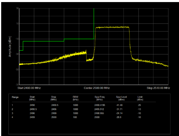
LTE Band7 16QAM BW=5MHz Channel=20775 RB Size=25 Position=#0
