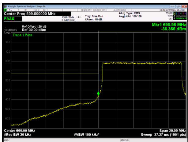
LTE Band12 QPSK BW=10MHz Channel=23060 RB Size=50 Position=#0
