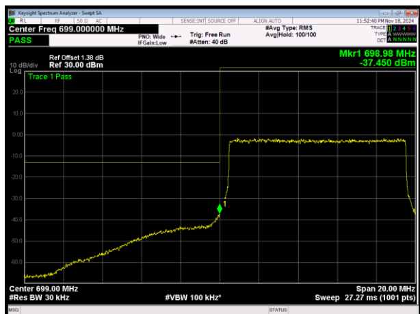
LTE Band12 16QAM BW=10MHz Channel=23060 RB Size=50 Position=#0
