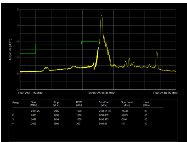
LTE Band7 16QAM BW=15MHz Channel=20825 RB Size=1 Position=#0
