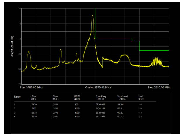
LTE Band7 QPSK BW=5MHz Channel=21425 RB Size=1 Position=#Max
