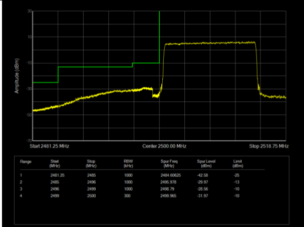
LTE Band7 16QAM BW=15MHz Channel=20825 RB Size=75 Position=#0
