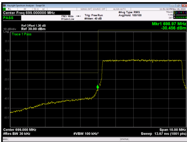
LTE Band12 16QAM BW=5MHz Channel=23035 RB Size=25 Position=#0
