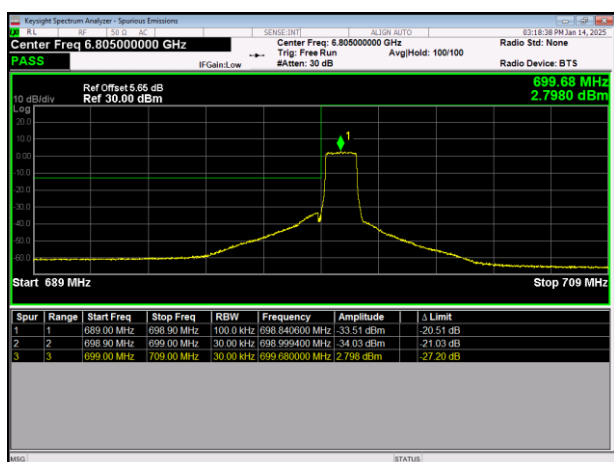
LTE Band12 64QAM BW=1.4MHz LowChannel=23017 RB Size=6 Position=#0
