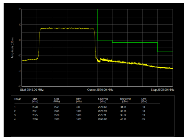
LTE Band7 16QAM BW=20MHz Channel=21350 RB Size=100 Position=#0
