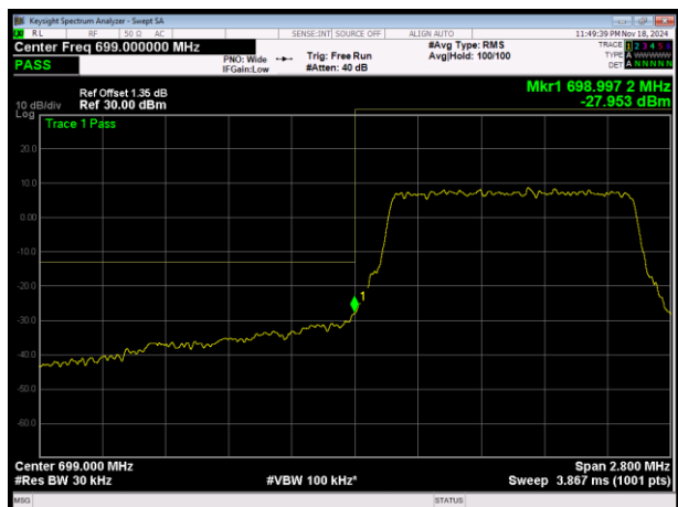
LTE Band12 QPSK BW=1.4MHz Channel=23017 RB Size=6 Position=#0
