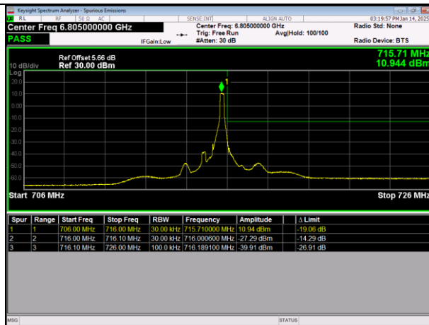
LTE Band12 64QAM BW=1.4MHz HighChannel=23173 RB Size=1 Position=#Max
