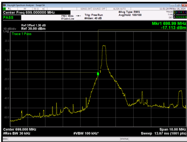
LTE Band12 16QAM BW=5MHz Channel=23035 RB Size=1 Position=#0
