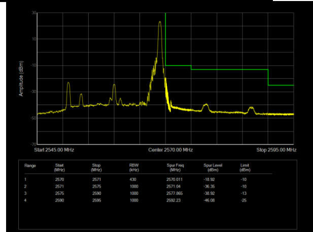
LTE Band7 QPSK BW=20MHz Channel=21350 RB Size=1 Position=#Max
