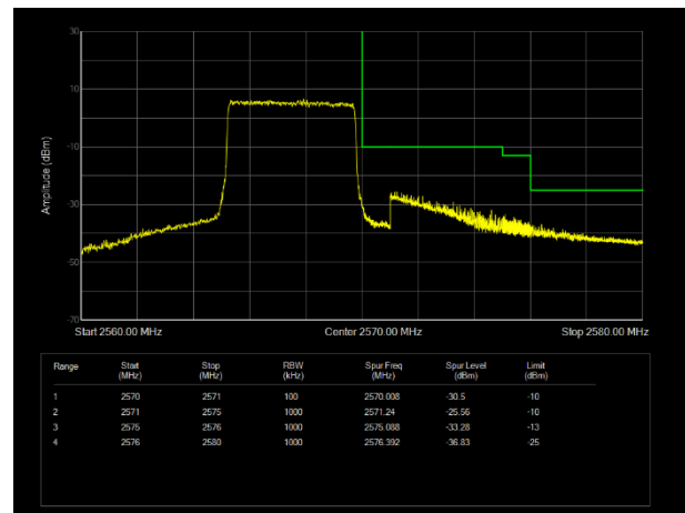
LTE Band7 16QAM BW=5MHz Channel=21425 RB Size=25 Position=#0
