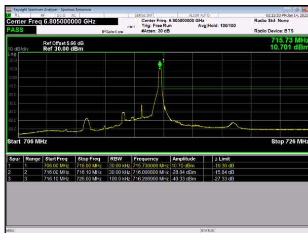
LTE Band12 64QAM BW=3MHz HighChannel=23165 RB Size=1 Position=#Max
