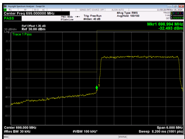
LTE Band12 QPSK BW=3MHz Channel=23025 RB Size=15 Position=#0
