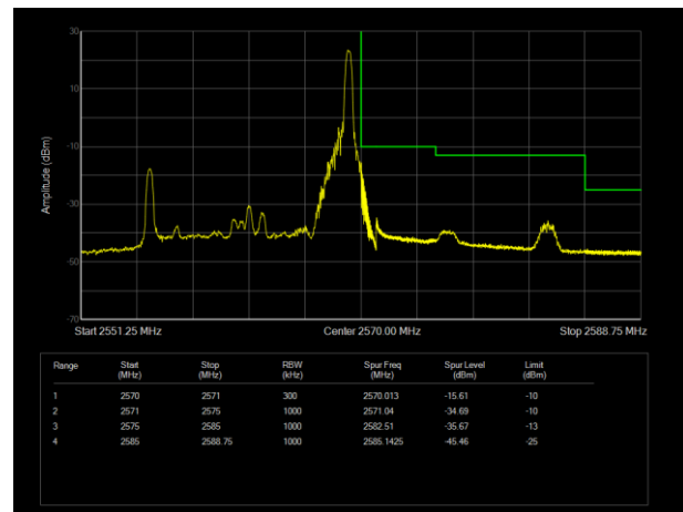
LTE Band7 QPSK BW=15MHz Channel=21375 RB Size=1 Position=#Max
