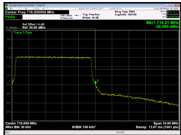
LTE Band12 16QAM BW=5MHz Channel=23155 RB Size=25 Position=#0
