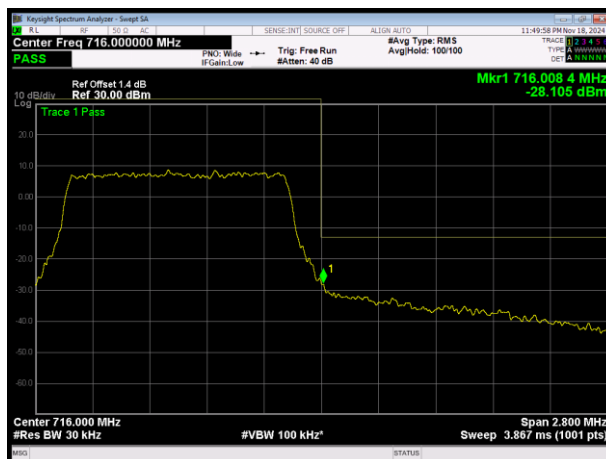
LTE Band12 QPSK BW=1.4MHz Channel=23173 RB Size=6 Position=#0
