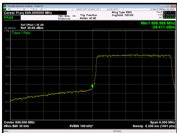
LTE Band12 16QAM BW=3MHz Channel=23025 RB Size=15 Position=#0
