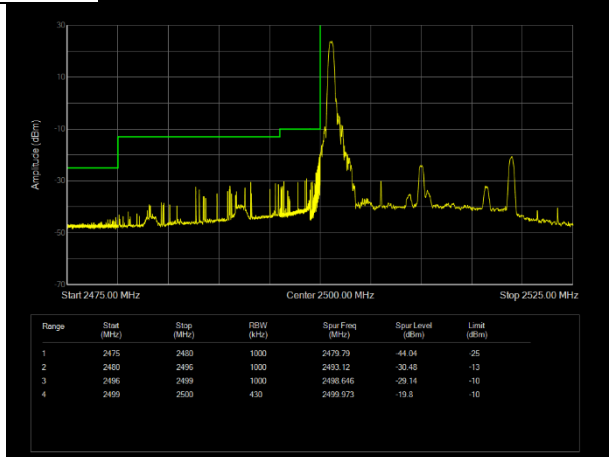
LTE Band7 QPSK BW=20MHz Channel=20850 RB Size=1 Position=#0
