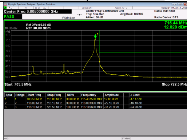
LTE Band12 64QAM BW=10MHz HighChannel=23130 RB Size=1 Position=#Max
