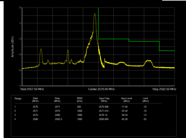
LTE Band7 16QAM BW=10MHz Channel=21400 RB Size=1 Position=#Max
