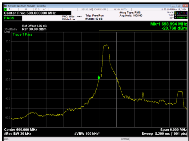
LTE Band12 QPSK BW=3MHz Channel=23025 RB Size=1 Position=#0
