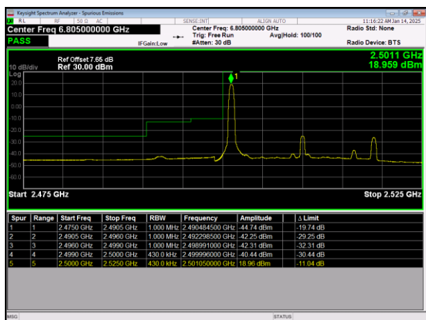
LTE Band7 64QAM BW=20MHz LowChannel=20850 RB Size=1 Position=#0
