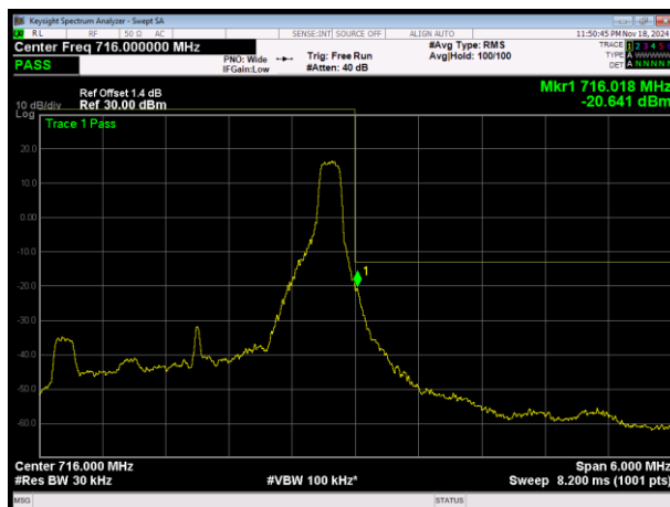
LTE Band12 QPSK BW=3MHz Channel=23165 RB Size=1 Position=#Max
