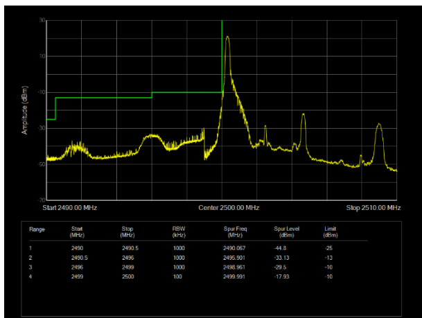
LTE Band7 QPSK BW=5MHz Channel=20775 RB Size=1 Position=#0
