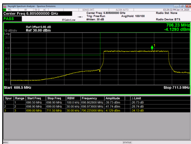
LTE Band12 64QAM BW=10MHz LowChannel=23060 RB Size=50 Position=#0
