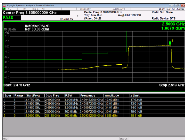
LTE Band7 64QAM BW=10MHz LowChannel=20800 RB Size=50 Position=#0
