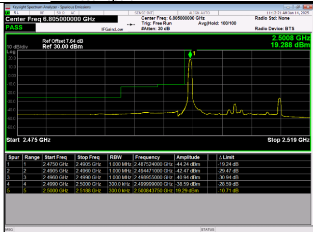
LTE Band7 64QAM BW=15MHz LowChannel=20825 RB Size=1 Position=#0
