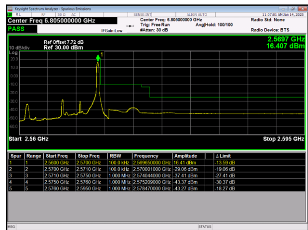
LTE Band7 64QAM BW=5MHz HighChannel=21425 RB Size=1 Position=#Max
