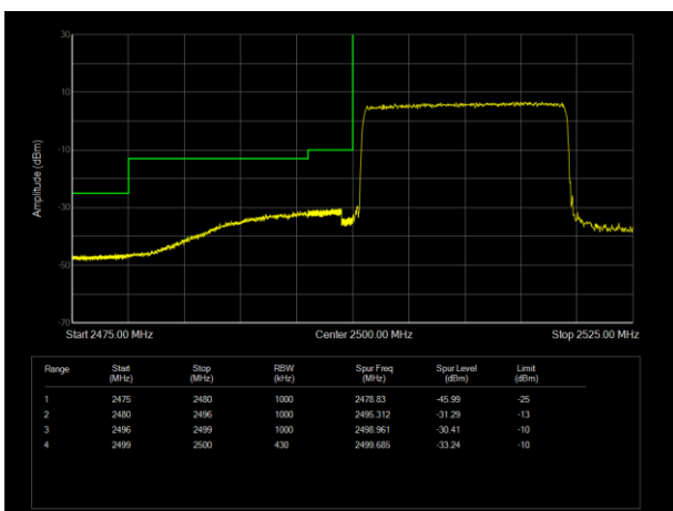
LTE Band7 16QAM BW=20MHz Channel=20850 RB Size=100 Position=#0
