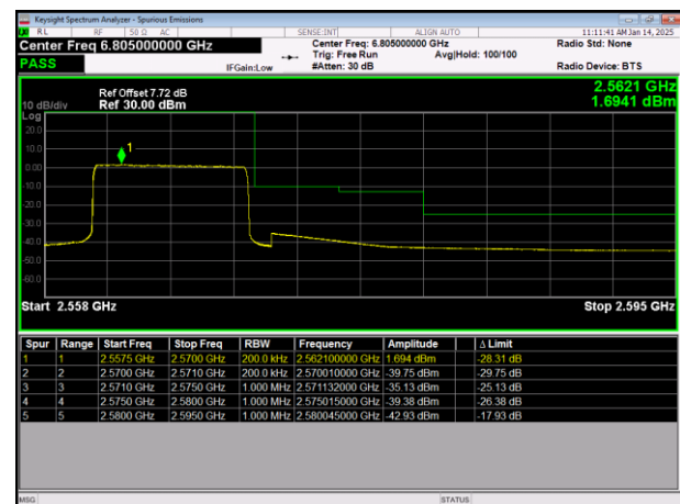
LTE Band7 64QAM BW=10MHz HighChannel=21400 RB Size=50 Position=#0
