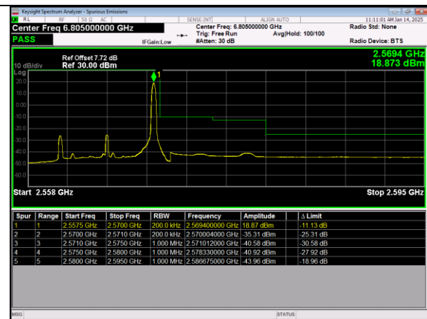
LTE Band7 64QAM BW=10MHz HighChannel=21400 RB Size=1 Position=#Max
