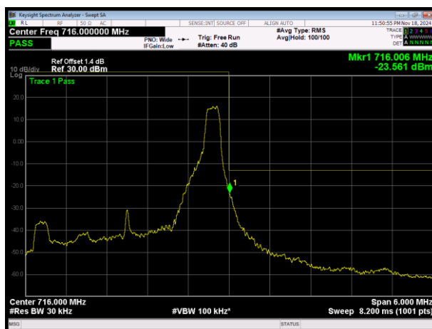
LTE Band12 16QAM BW=3MHz Channel=23165 RB Size=1 Position=#Max
