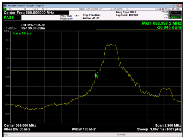
LTE Band12 16QAM BW=1.4MHz Channel=23017 RB Size=1 Position=#0
