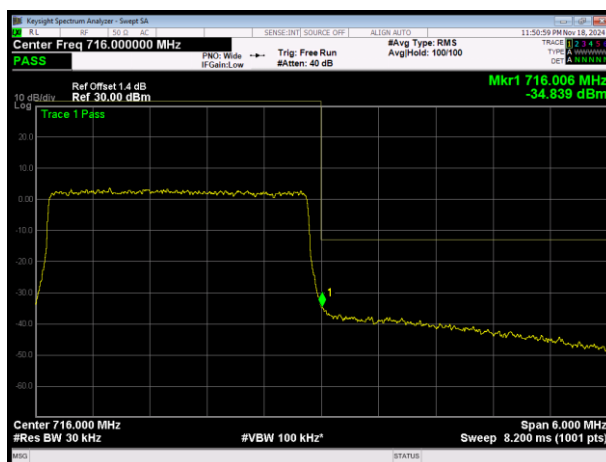
LTE Band12 16QAM BW=3MHz Channel=23165 RB Size=15 Position=#0
