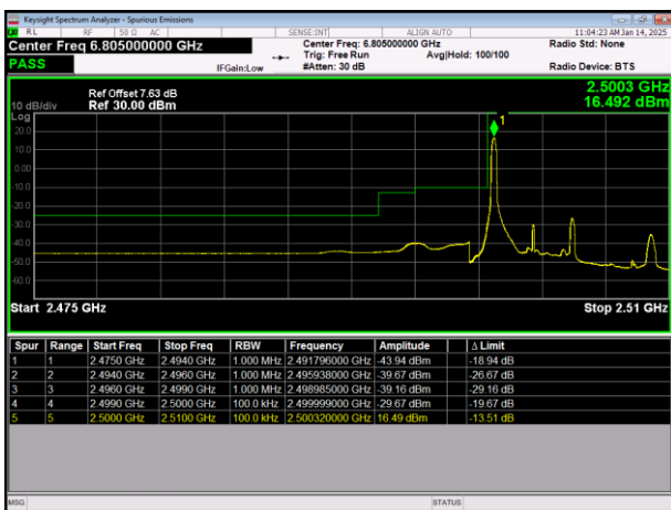
LTE Band7 64QAM BW=5MHz LowChannel=20775 RB Size=1 Position=#0
