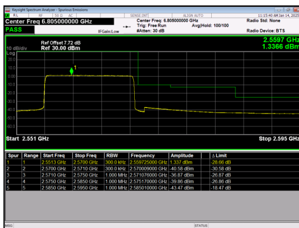
LTE Band7 64QAM BW=15MHz HighChannel=21375 RB Size=75 Position=#0
