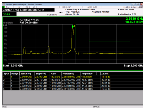
LTE Band7 64QAM BW=20MHz HighChannel=21350 RB Size=1 Position=#Max
