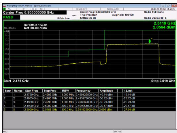
LTE Band7 64QAM BW=15MHz LowChannel=20825 RB Size=75 Position=#0
