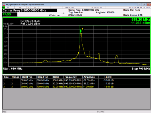
LTE Band12 64QAM BW=3MHz LowChannel=23025 RB Size=1 Position=#0
