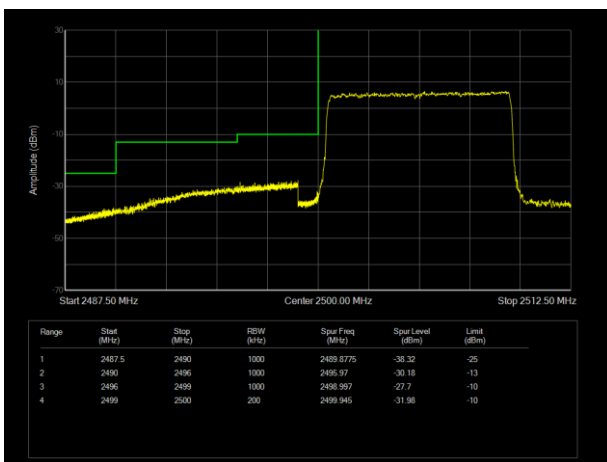
LTE Band7 16QAM BW=10MHz Channel=20800 RB Size=50 Position=#0
