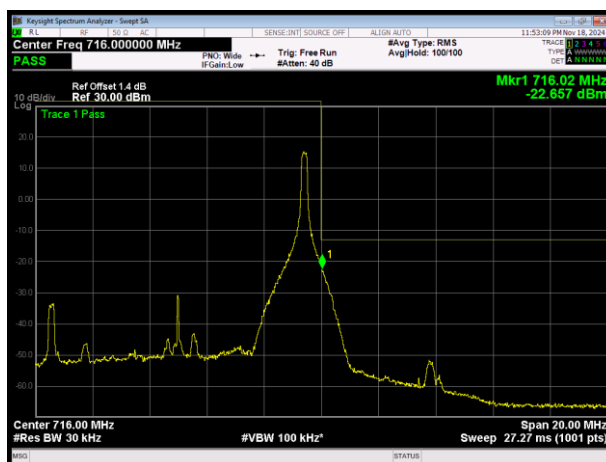
LTE Band12 16QAM BW=10MHz Channel=23130 RB Size=1 Position=#Max
