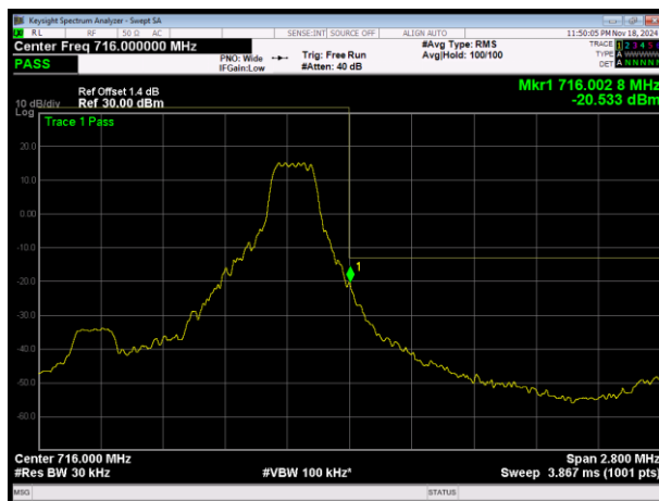
LTE Band12 16QAM BW=1.4MHz Channel=23173 RB Size=1 Position=#Max
