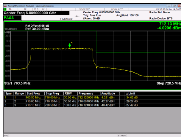
LTE Band12 64QAM BW=10MHz HighChannel=23130 RB Size=50 Position=#0
