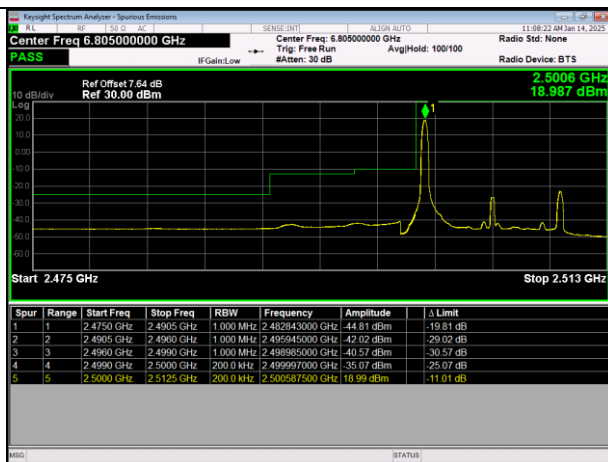
LTE Band7 64QAM BW=10MHz LowChannel=20800 RB Size=1 Position=#0
