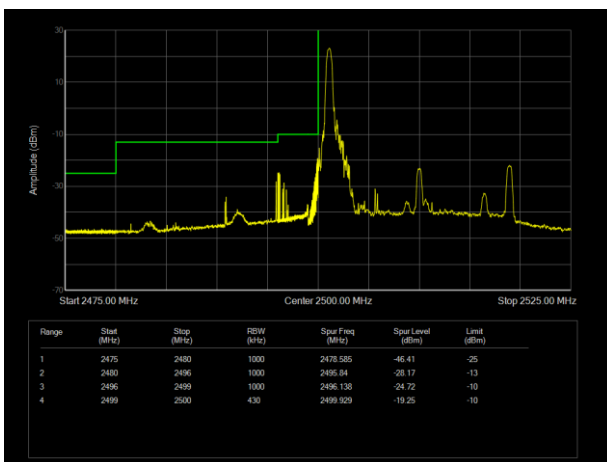
LTE Band7 16QAM BW=20MHz Channel=20850 RB Size=1 Position=#0
