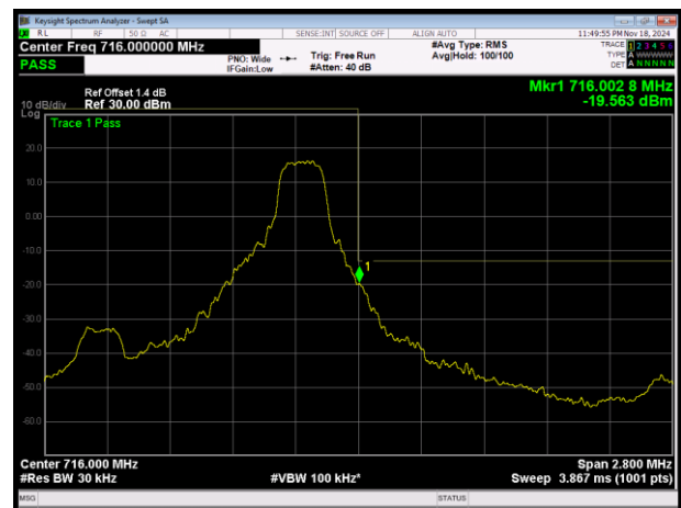
LTE Band12 QPSK BW=1.4MHz Channel=23173 RB Size=1 Position=#Max
