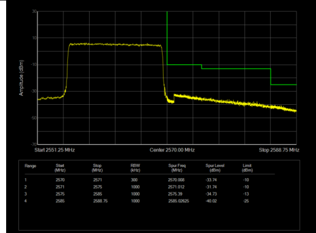
LTE Band7 16QAM BW=15MHz Channel=21375 RB Size=75 Position=#0
