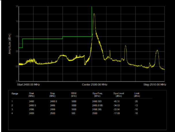
LTE Band7 16QAM BW=5MHz Channel=20775 RB Size=1 Position=#0
