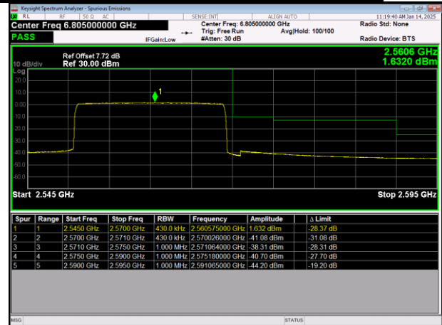
LTE Band7 64QAM BW=20MHz HighChannel=21350 RB Size=100 Position=#0
