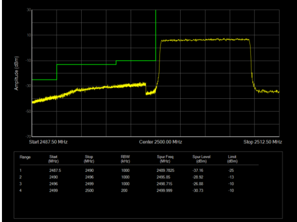
LTE Band7 QPSK BW=10MHz Channel=20800 RB Size=50 Position=#0
