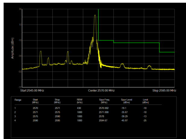
LTE Band7 16QAM BW=20MHz Channel=21350 RB Size=1 Position=#Max
