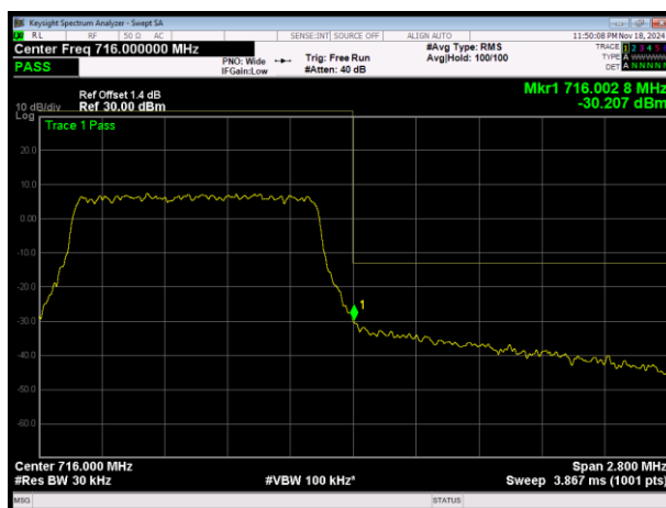
LTE Band12 16QAM BW=1.4MHz Channel=23173 RB Size=6 Position=#0
