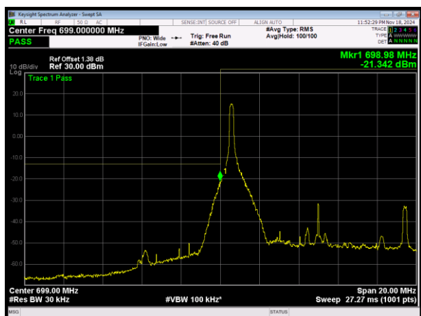
LTE Band12 16QAM BW=10MHz Channel=23060 RB Size=1 Position=#0
