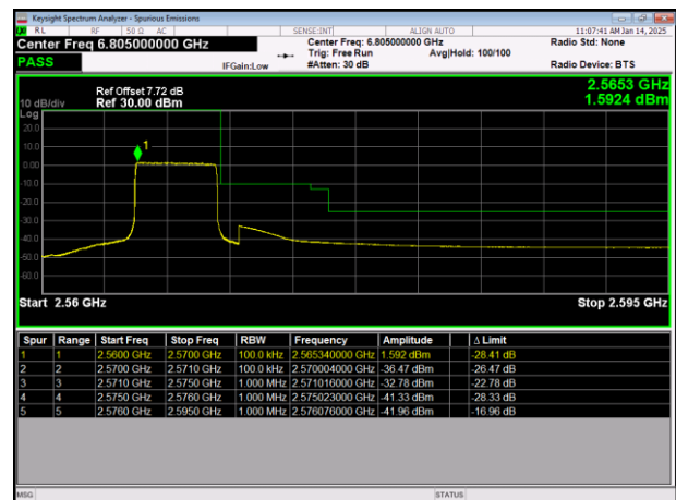
LTE Band7 64QAM BW=5MHz HighChannel=21425 RB Size=25 Position=#0
