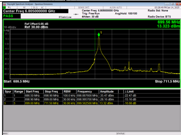
LTE Band12 64QAM BW=10MHz LowChannel=23060 RB Size=1 Position=#0
