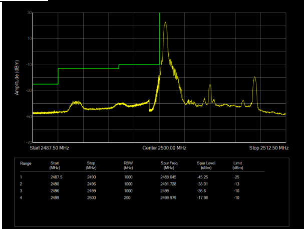
LTE Band7 16QAM BW=10MHz Channel=20800 RB Size=1 Position=#0
