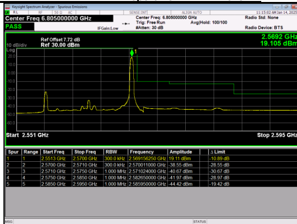
LTE Band7 64QAM BW=15MHz HighChannel=21375 RB Size=1 Position=#Max
