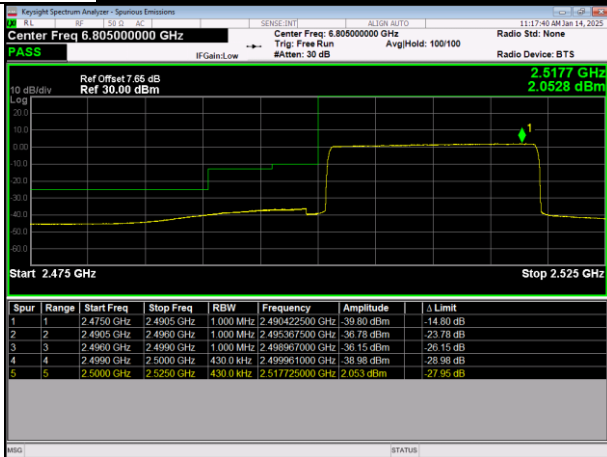
LTE Band7 64QAM BW=20MHz LowChannel=20850 RB Size=100 Position=#0
