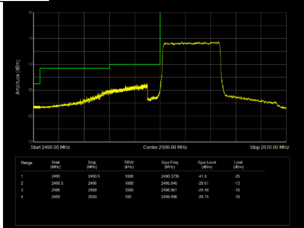
LTE Band7 QPSK BW=5MHz Channel=20775 RB Size=25 Position=#0
