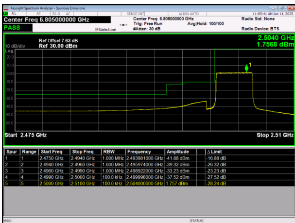
LTE Band7 64QAM BW=5MHz LowChannel=20775 RB Size=25 Position=#0
