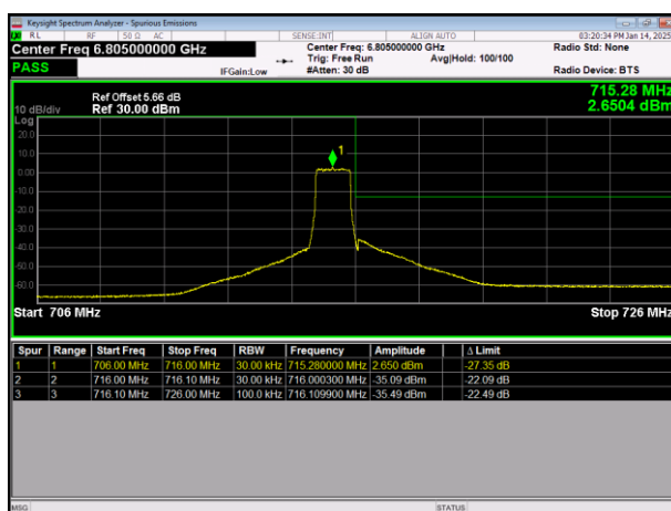
LTE Band12 64QAM BW=1.4MHz HighChannel=23173 RB Size=6 Position=#0
