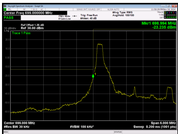
LTE Band12 16QAM BW=3MHz Channel=23025 RB Size=1 Position=#0
