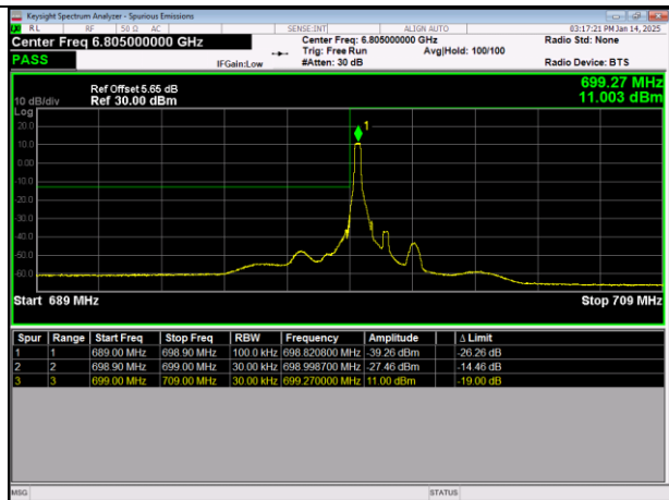
LTE Band12 64QAM BW=1.4MHz LowChannel=23017 RB Size=1 Position=#0
