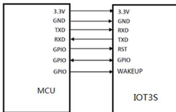
Figure 6-1 IOT3S Reference Design
