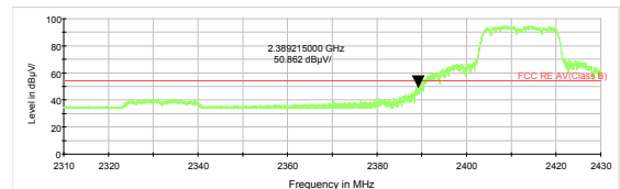
802.11g-Channel 1 Average
