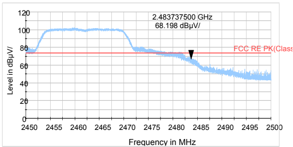
802.11g-Channel 11 Peak
