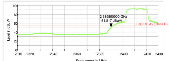
802.11n HT20 -Channel 1 Average
