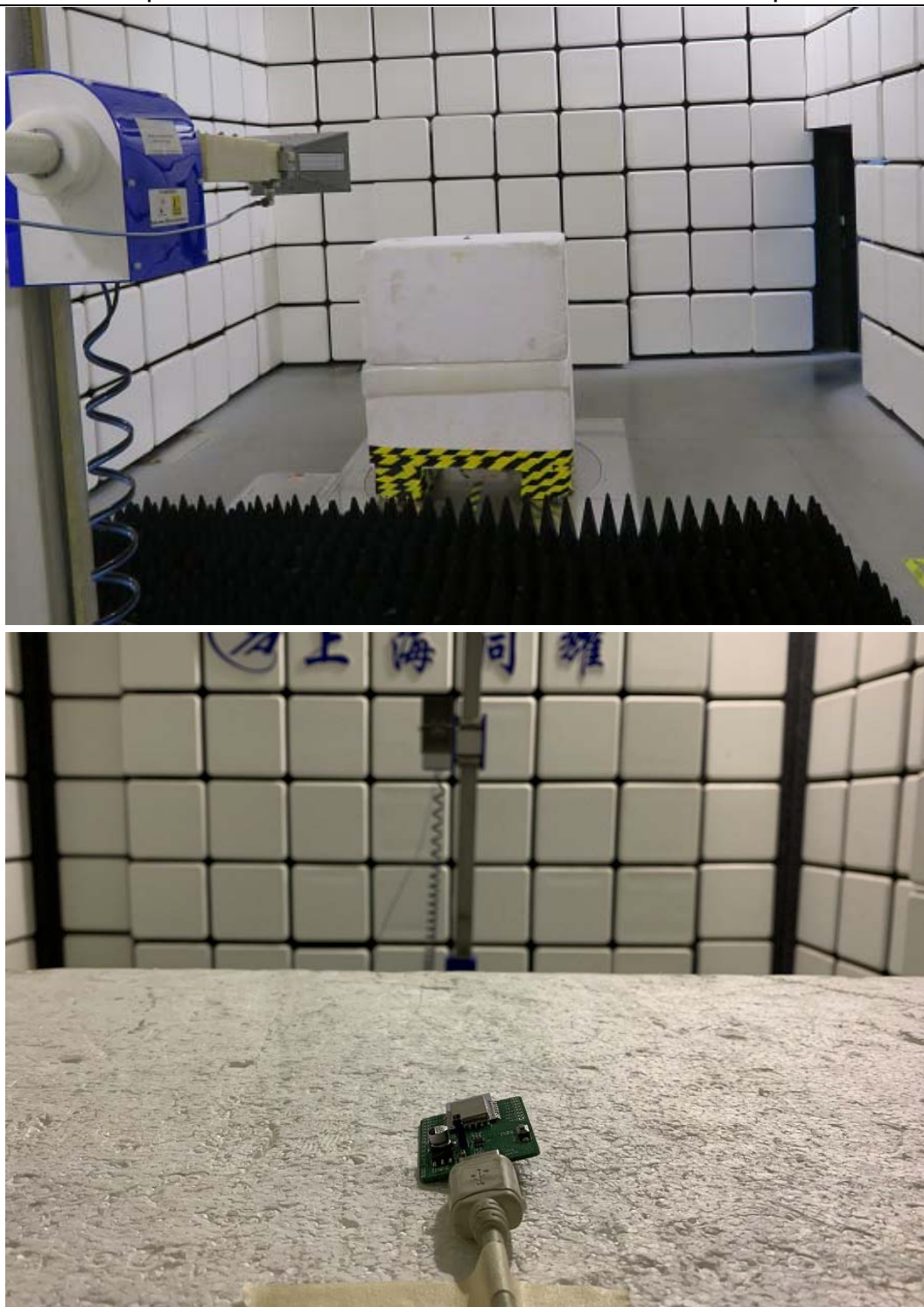
Picture 1 Radiated Emission Test Setup
